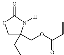
Formula 3. 4-acryloxymethyl-4-ethyl-2-oxazolidinone
