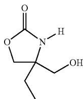
Formula 2. 4-hydroxymethyl-4-ethyl-2-oxazolidinone
