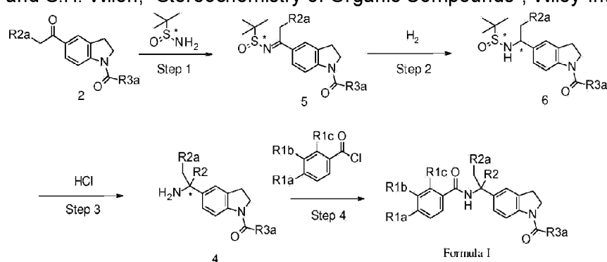
Scheme 2: Synthesis of compounds of Formula I
