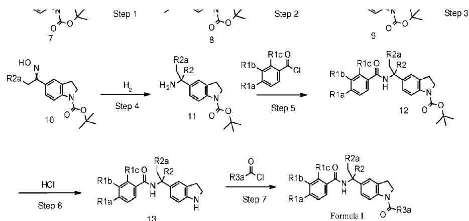
Scheme 3: Synthesis of compounds of Formula I
