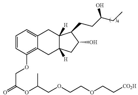
Compound II-21
