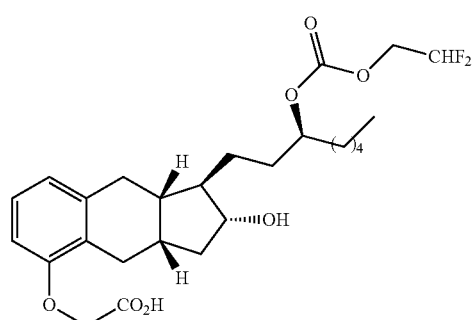
Compound Ib-13
