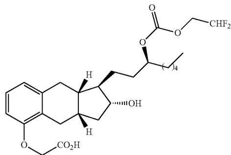
Compound Ib-14
