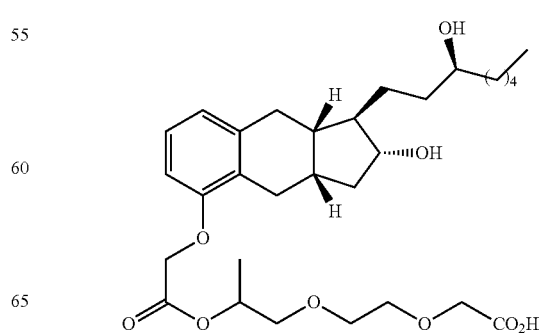
Compound II-18
