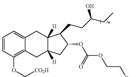
Compound Ib-1
