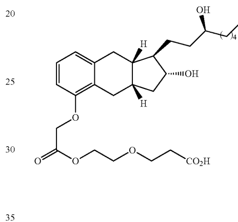
Compound II-11
