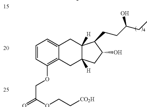
Compound II-4
