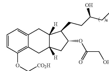
Compound Ia-2 20
