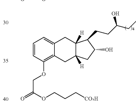
Compound II-5
