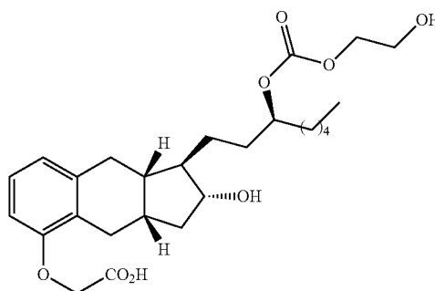
Compound Ib-15
