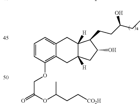
Compound II-1
