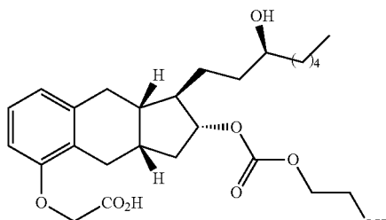
Compound Ia-15
