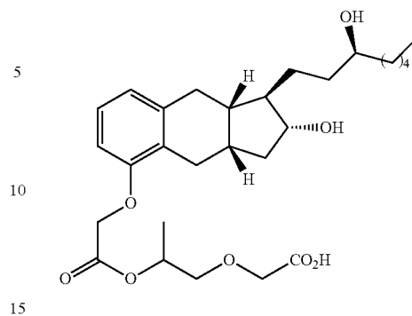
Compound II-10
