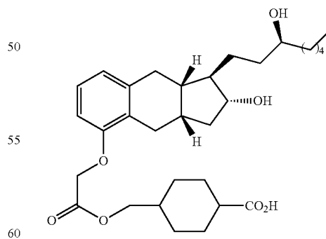
Compound II-22
