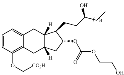
Compound Ia-14
