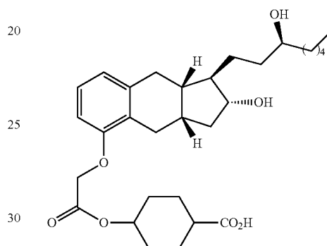
Compound II-20
