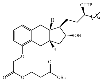
Compound Ib-9
