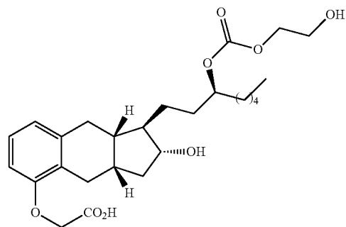
Compound Ib-14
