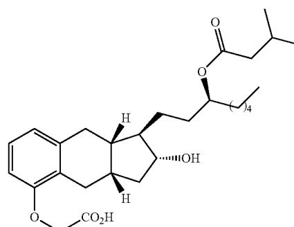
Compound Ib-4
