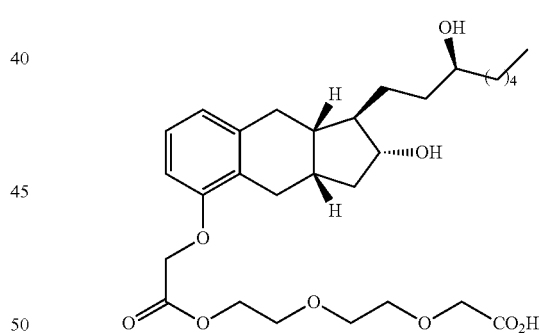
Compound II-17
