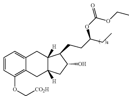
Compound Ib-11
