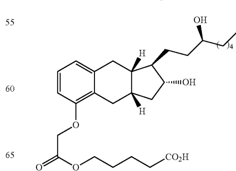
Compound II-2
