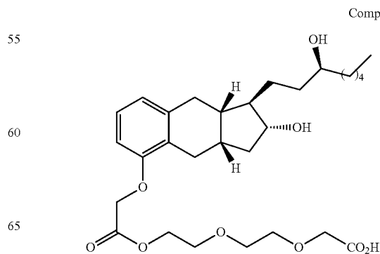
Compound II-17
