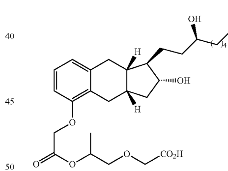
Compound II-14
