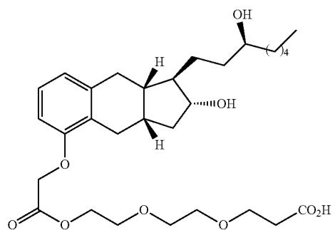
Compound II-19
