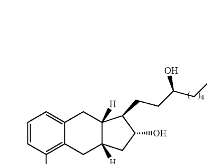
Compound II-8
