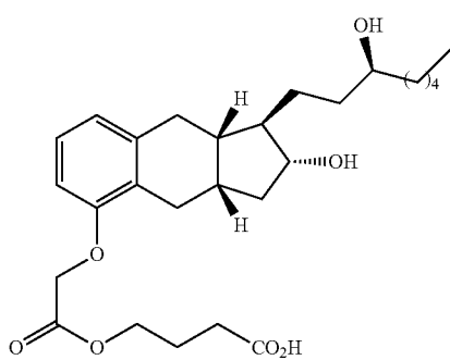
Compound II-5
