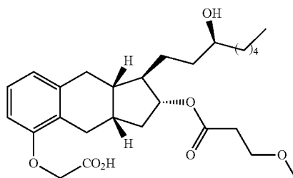
Compound Ia-1 5
