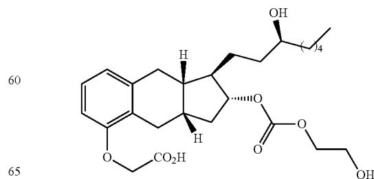
Compound Ia-14
