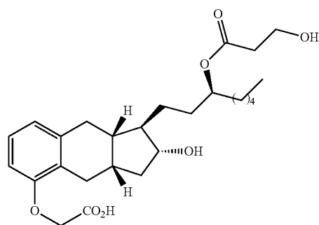
Compound Ib-6
