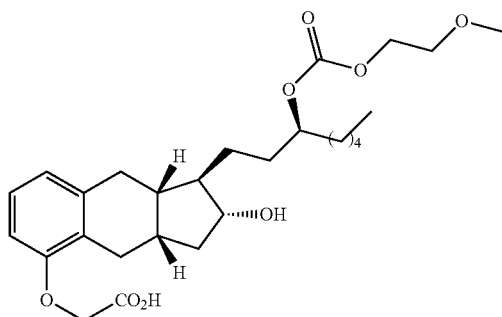
Compound Ib-15
