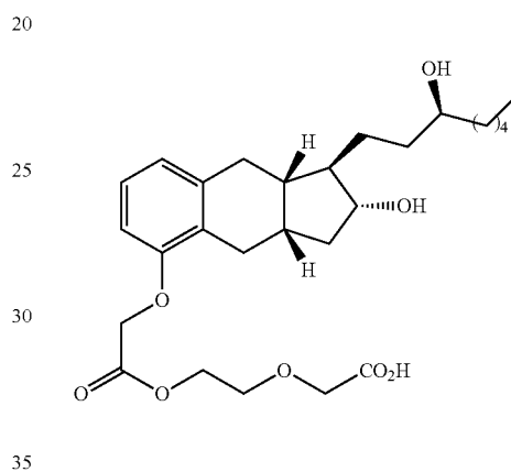
Compound II-13
