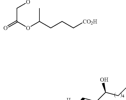
Compound II-9
