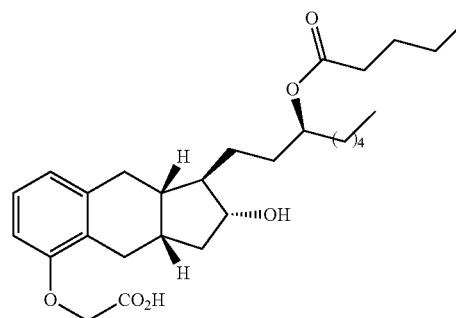
Compound Ib-3
