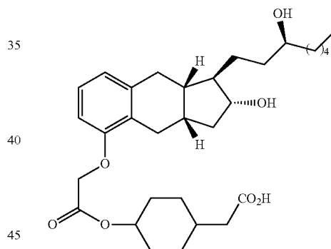
Compound II-21
