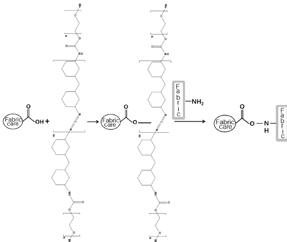
[Reaction Scheme 5]
