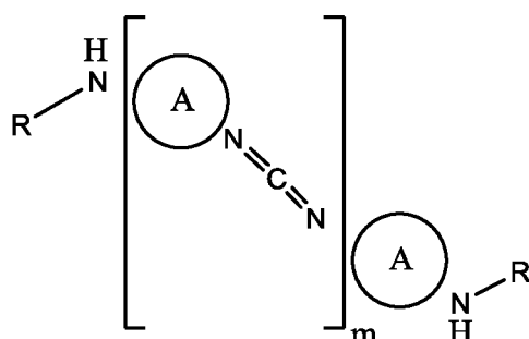
[Chemical Formula 1]
