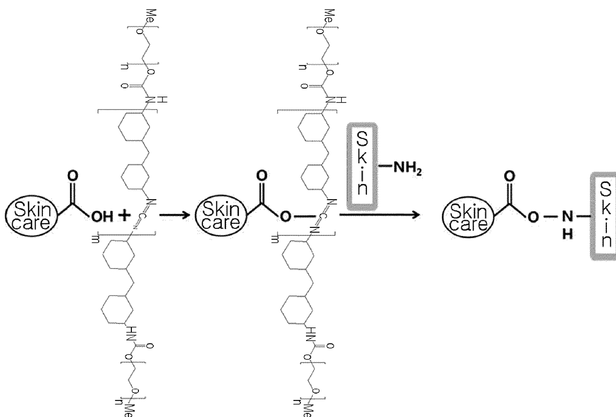
[Reaction Scheme 1]
