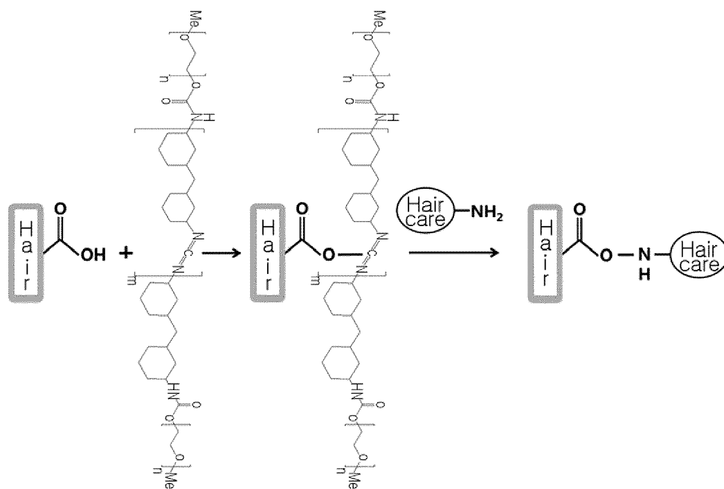
[Reaction Scheme 4]
