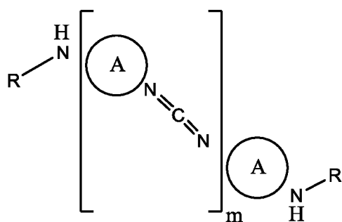
[Chemical Formula 1]
