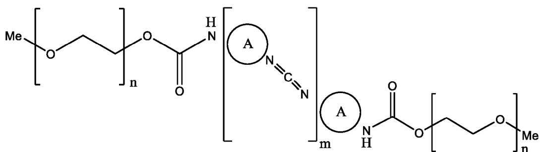
[Chemical Formula 2]
