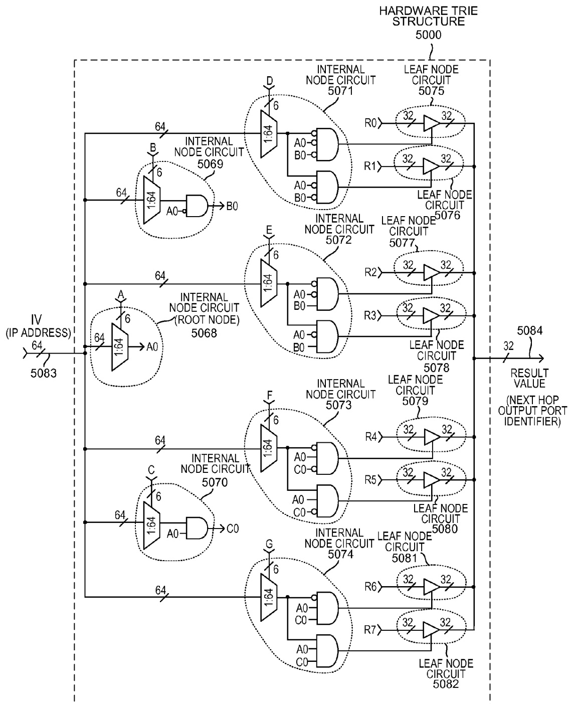
HARDWARE TRIE STRUCTURE
