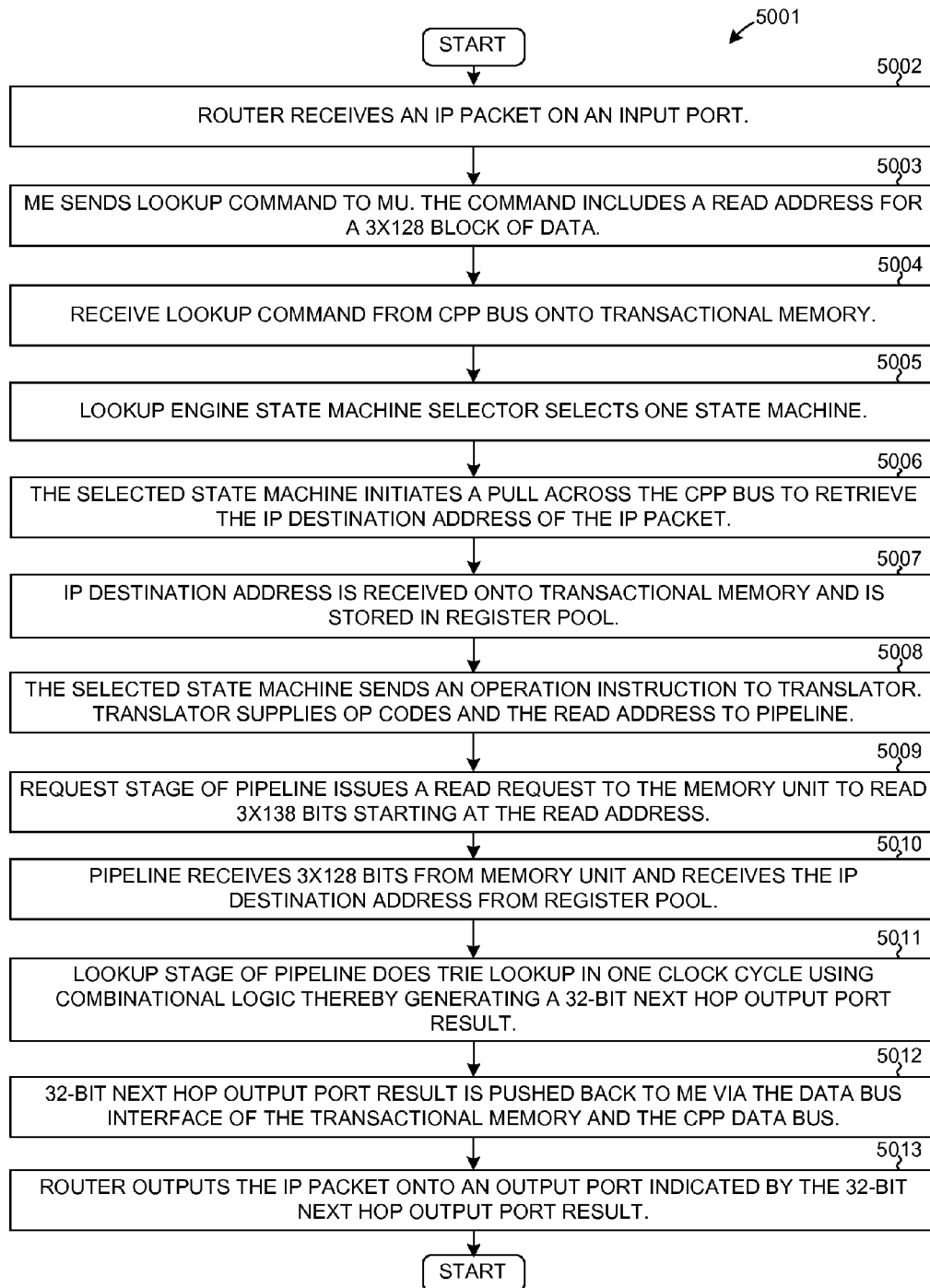
FLOWCHART OF A TRIE MULTI-BIT LOOKUP OPERATION
