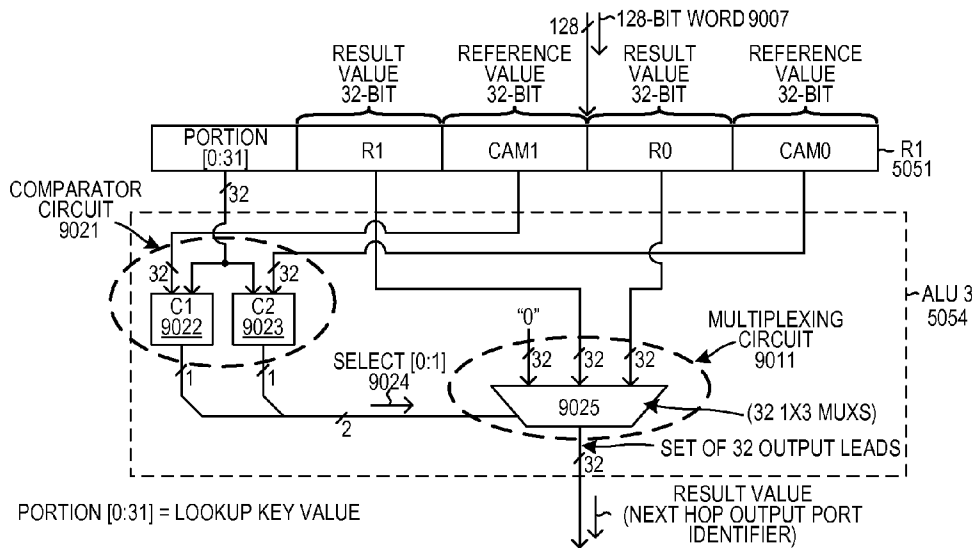
DIRECT CAMR 32-BIT LOOKUP STAGE FIG. 54
