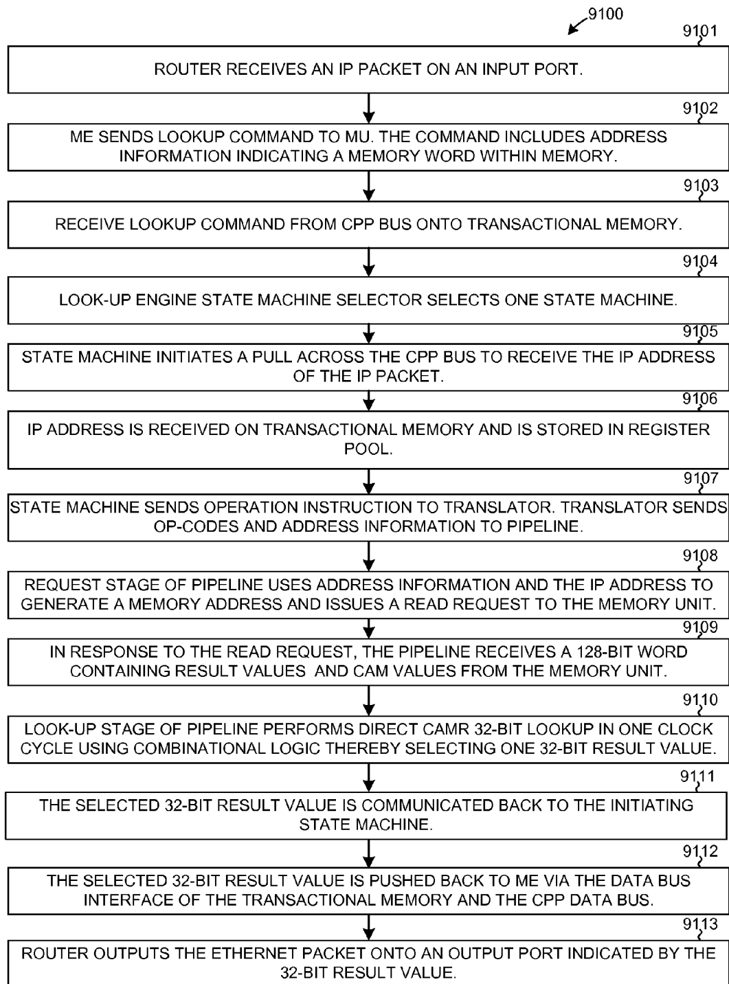
CAMR 32-BIT LOOKUP FLOWCHART FIG. 55
