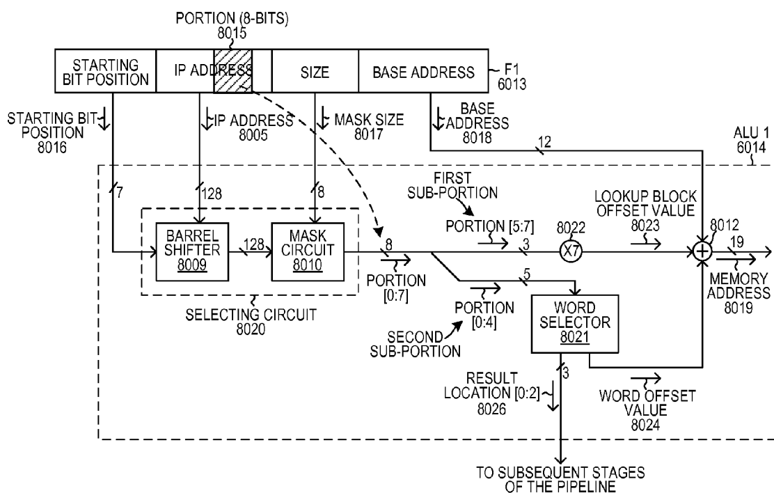
DIRECT 24-BIT REQUEST STAGE FIG. 48
