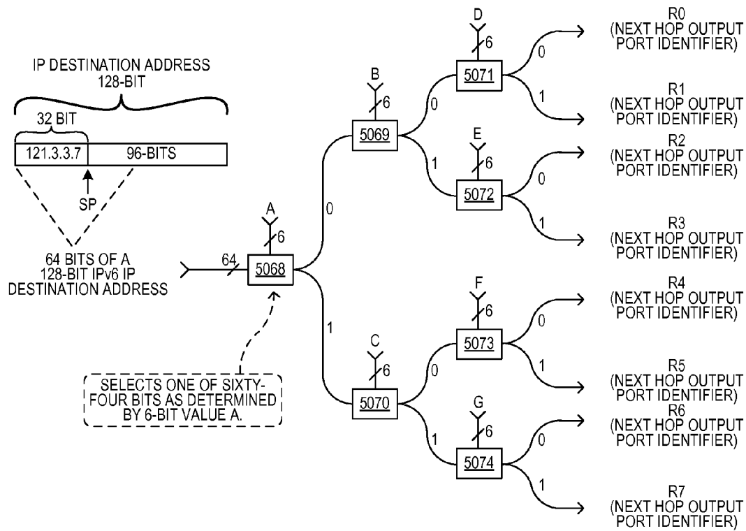
CONCEPTUAL DIAGRAM OF TRIE MULTI-BIT LOOKUP OPERATION
