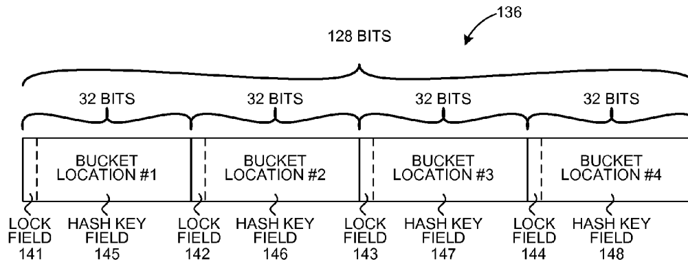
HASH BUCKET FIG. 19
