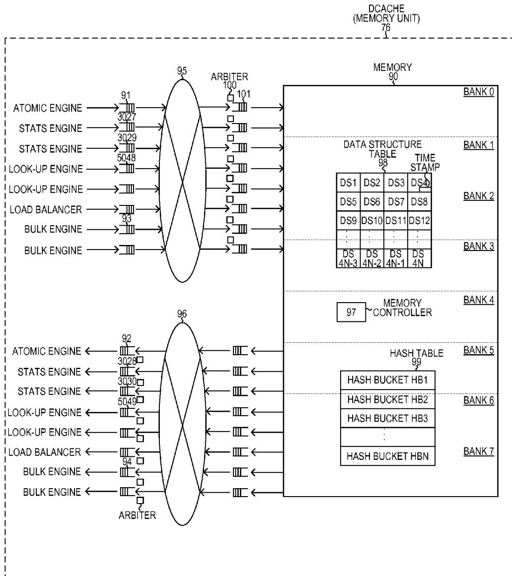
DCACHE EXPANDED DIAGRAM FIG. 12
