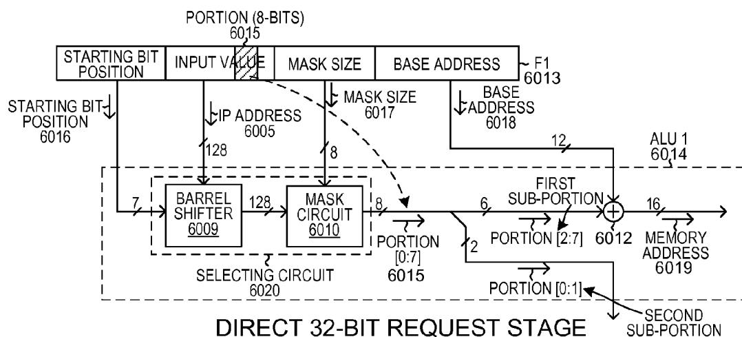
DIRECT 32-BIT MEMORY PACKING SCHEME FIG. 40
