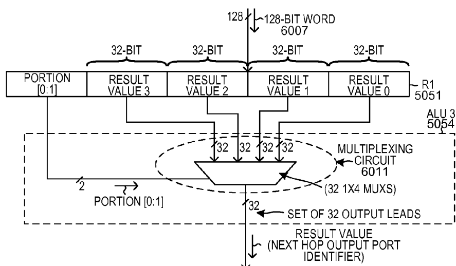
DIRECT 32-BIT LOOKUP STAGE FIG. 42
