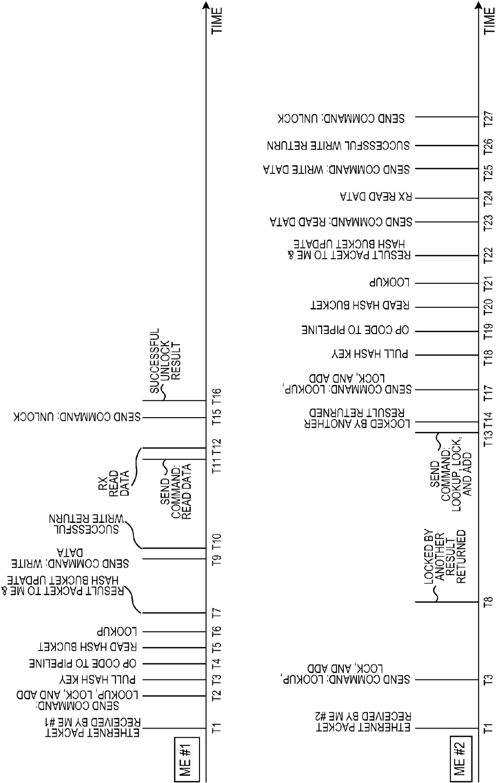
LOOKUP, LOCK, AND ADD TIMING DIAGRAM FIG. 14
