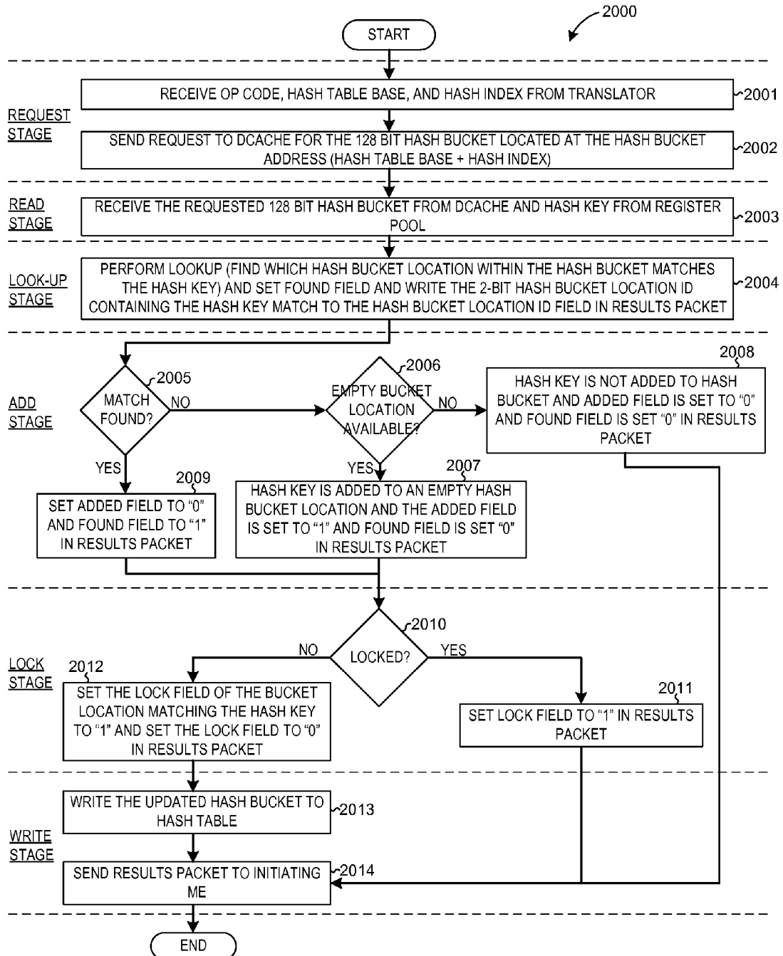
PIPELINE OPERATIONAL FLOW FIG. 24
