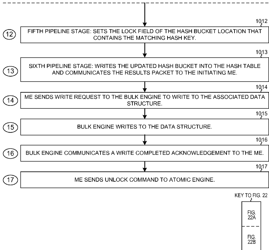
TRANSACTIONAL MEMORY FLOWCHART FIG. 22B
