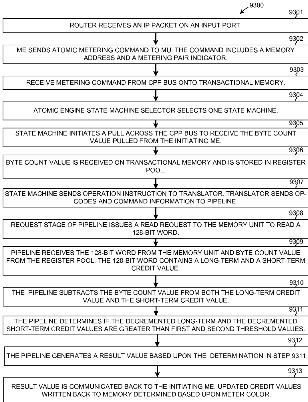
ATOMIC METERING COMMAND FLOWCHART
