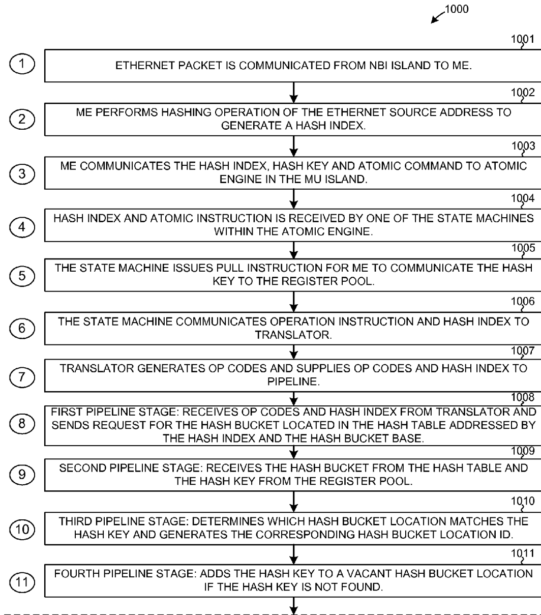
TRANSACTIONAL MEMORY FLOWCHART
