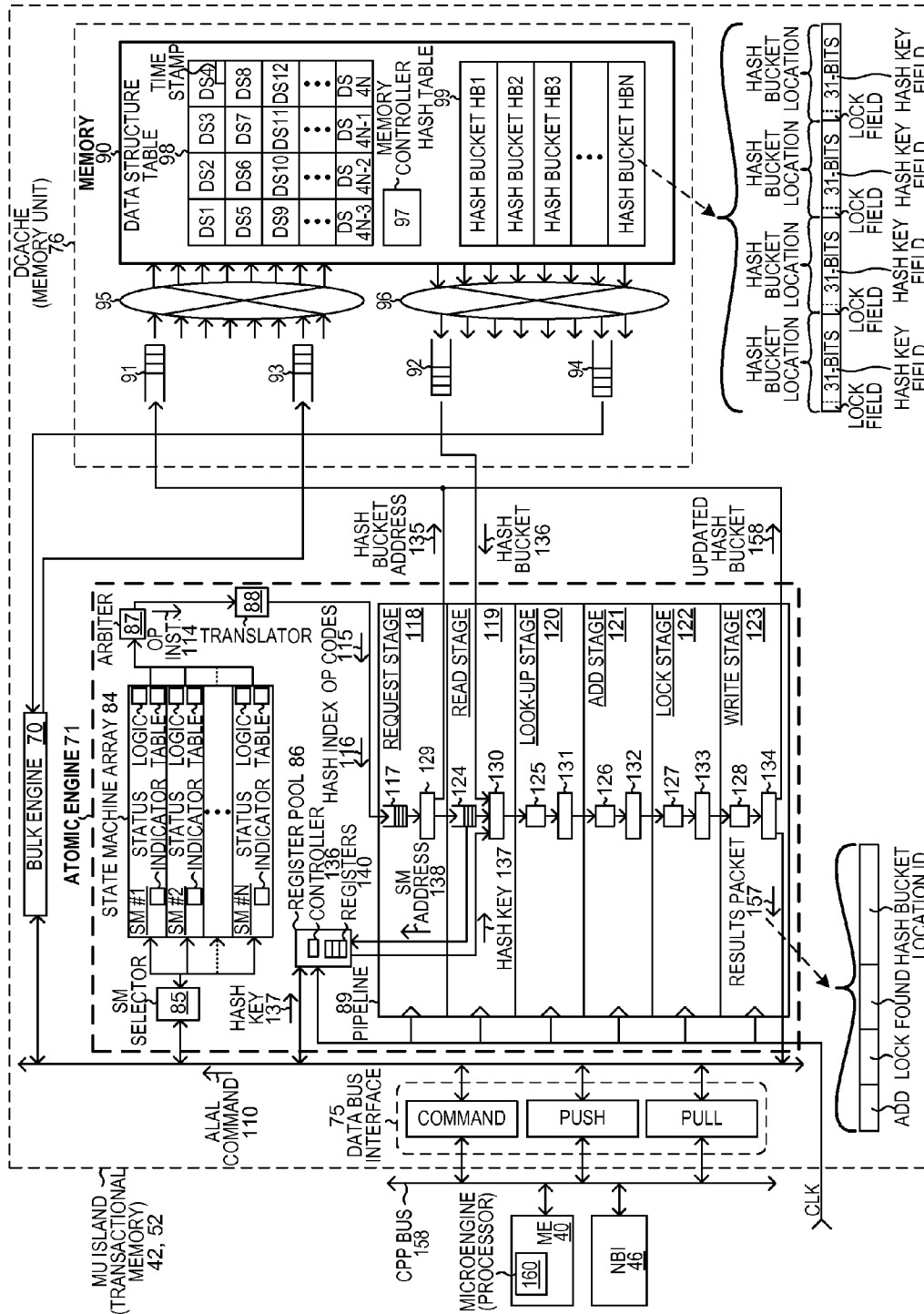
MU ISLAND SHOWING ATOMIC ENGINE IN DETAIL
