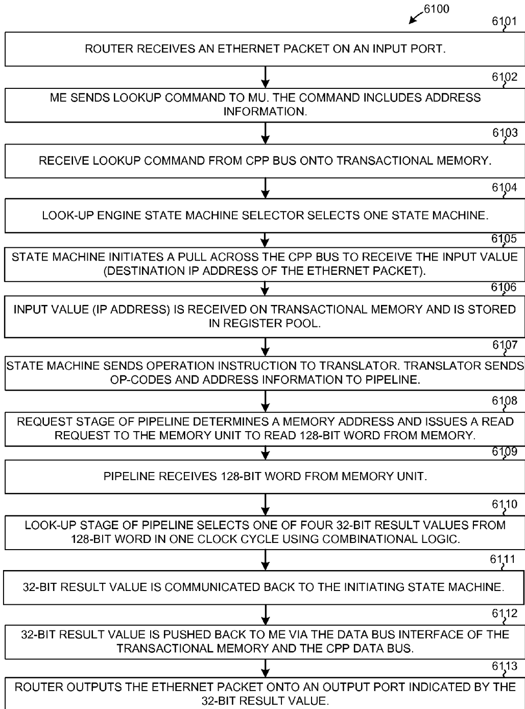
DIRECT 32-BIT LOOKUP FLOWCHART FIG. 44
