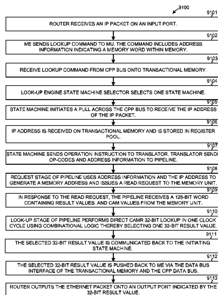
CAMR 32-BIT LOOKUP FLOWCHART
