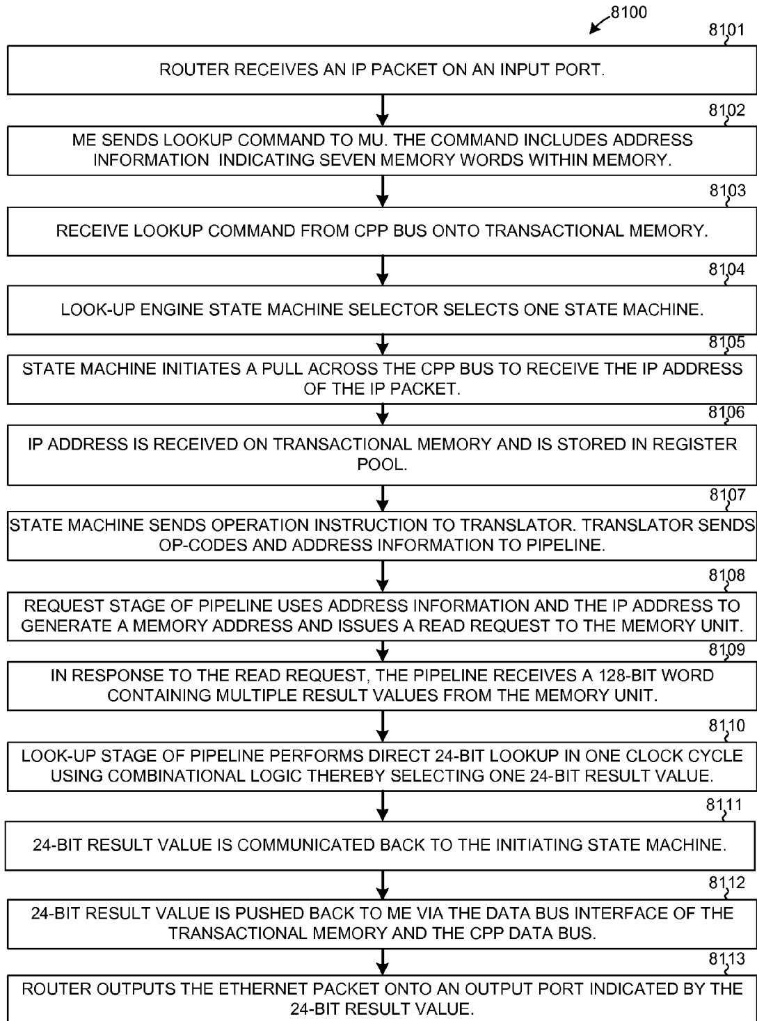
DIRECT 24-BIT LOOK-UP FLOWCHART FIG. 50
