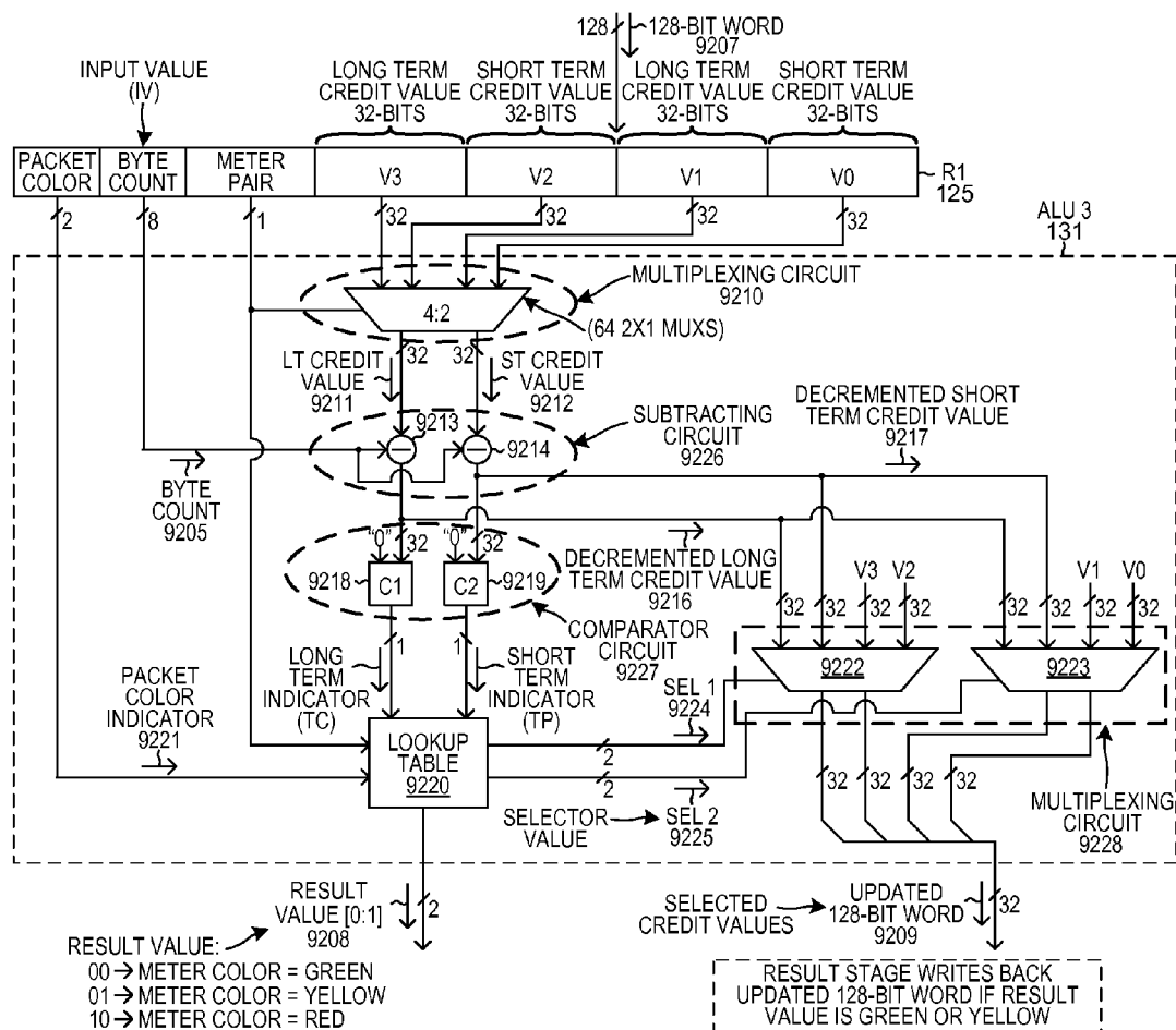
ATOMIC METERING COMMAND LOOKUP STAGE
