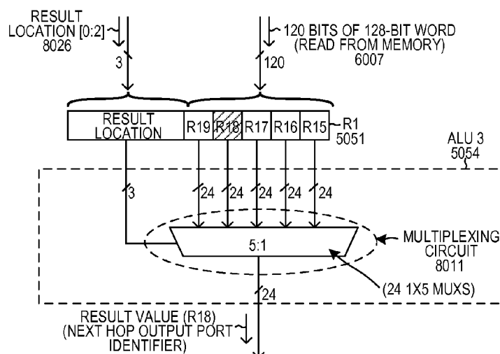
DIRECT 24-BIT LOOK-UP STAGE FIG. 49
