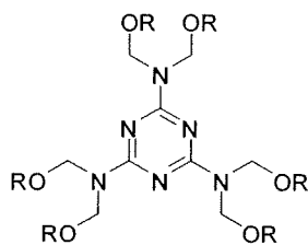
melamine-formaldehyde based
