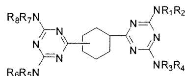
cycloalkanedibisguanamine based
