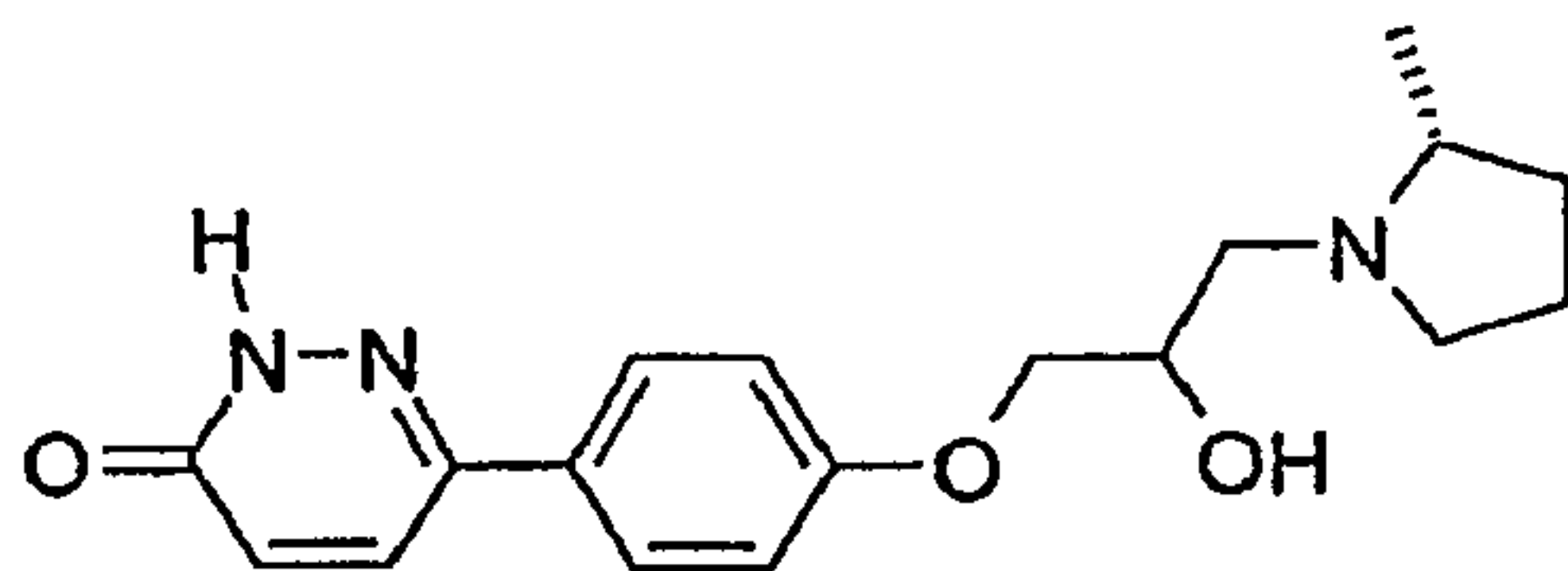
6-{4-[2-Hydroxy-3-((R)-2-methyl-pyrrolidin-1-yl)-propoxy]-phenyl}-2H-pyridazin-3-one
