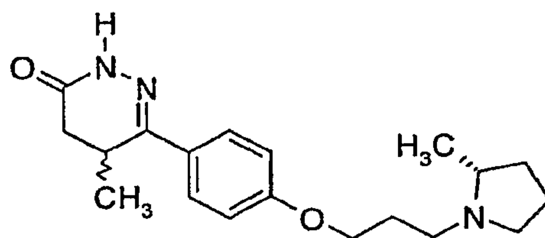
5-Methyl-6-{4-[3-((R)-2-methyl-pyrrolidin-1-yl)-propoxy]-phenyl}-4,5-dihydro-2H-pyridazin-3-one
