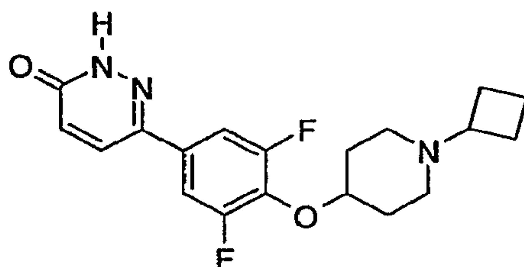
6-[4-(1-Cyclobutyl-piperidin-4-yloxy)-3,5-difluoro-phenyl]-2H-pyridazin-3-one
