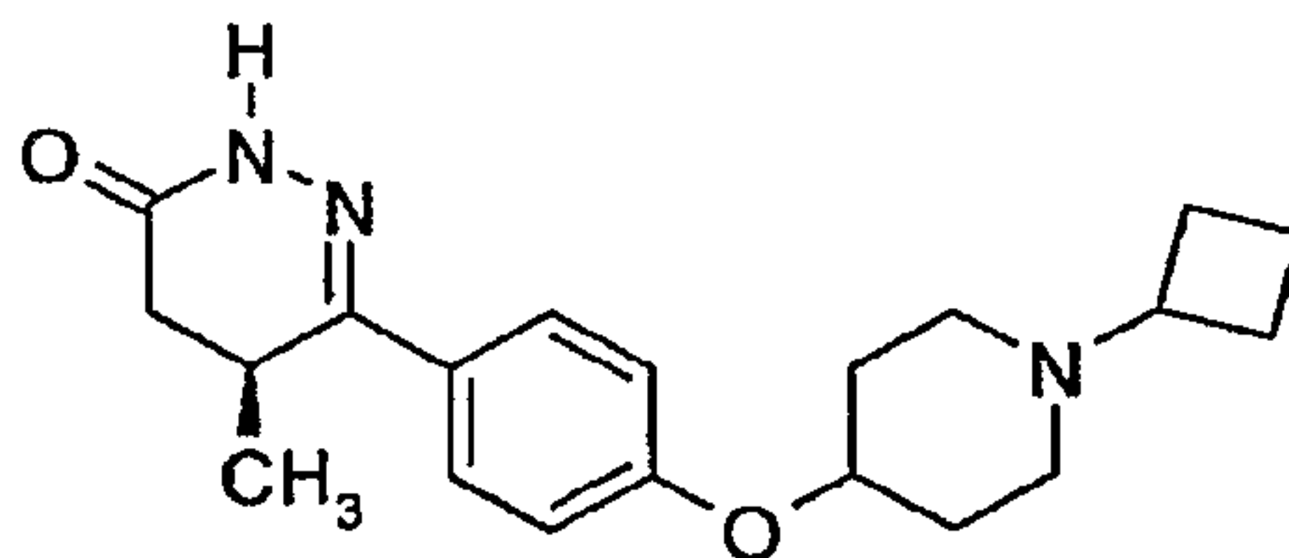
(S)-6-[4-(1-Cyclobutyl-piperidin-4-yloxy)-phenyl]-5-methyl-4,5-dihydro-2H-pyridazin-3-one
