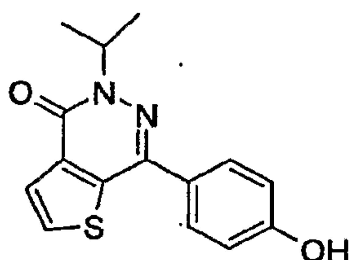
7-(4-Hydroxy-phenyl)-5-isopropyl-5H -thieno[2,3-d]pyridazin-4-one
