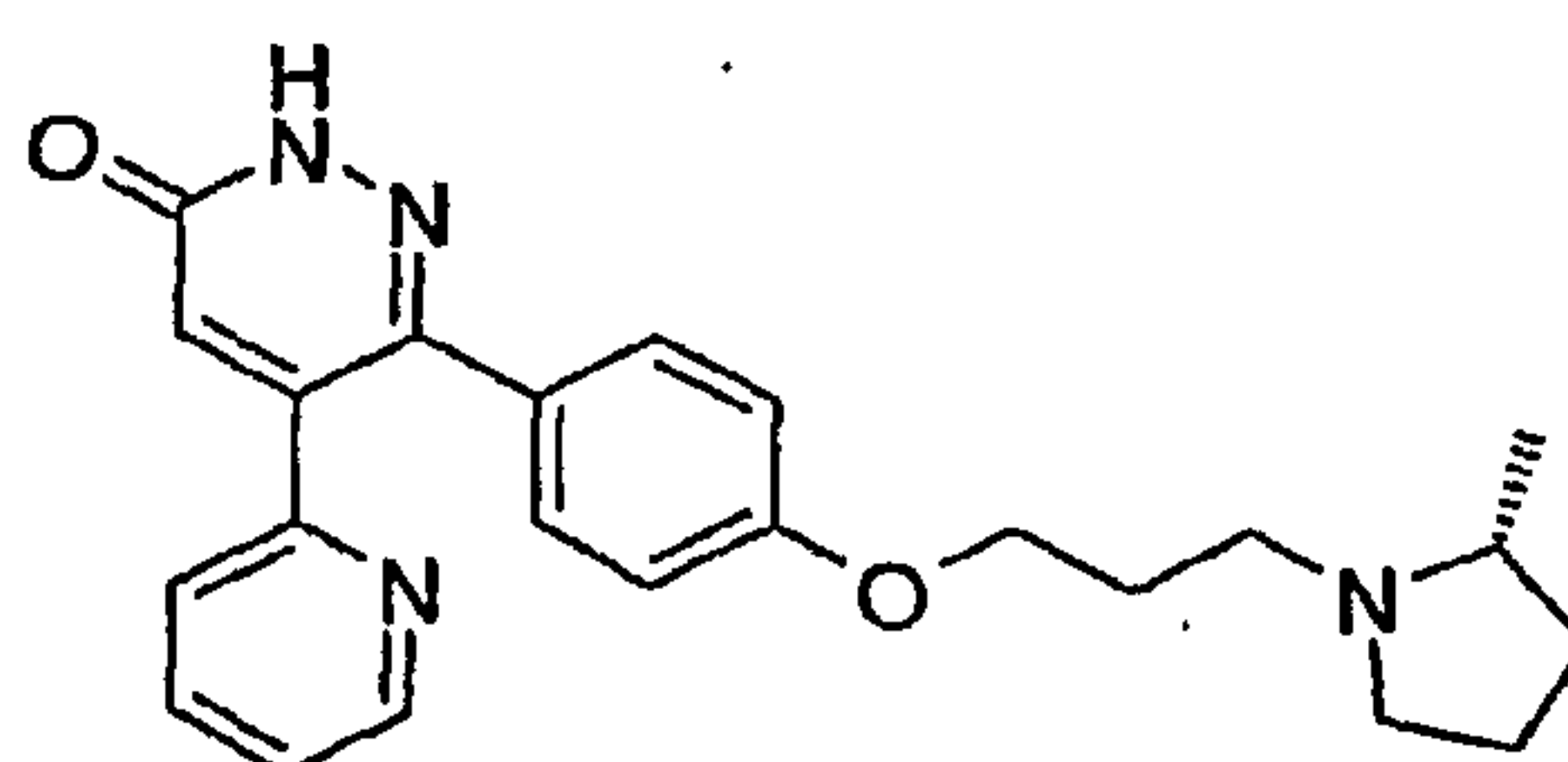
6-{4-[3-((R)-2-Methyl-pyrrolidin-1-yl)-propoxy]-phenyl}-5-pyridin-2-yl-2H-pyridazin-3-one
