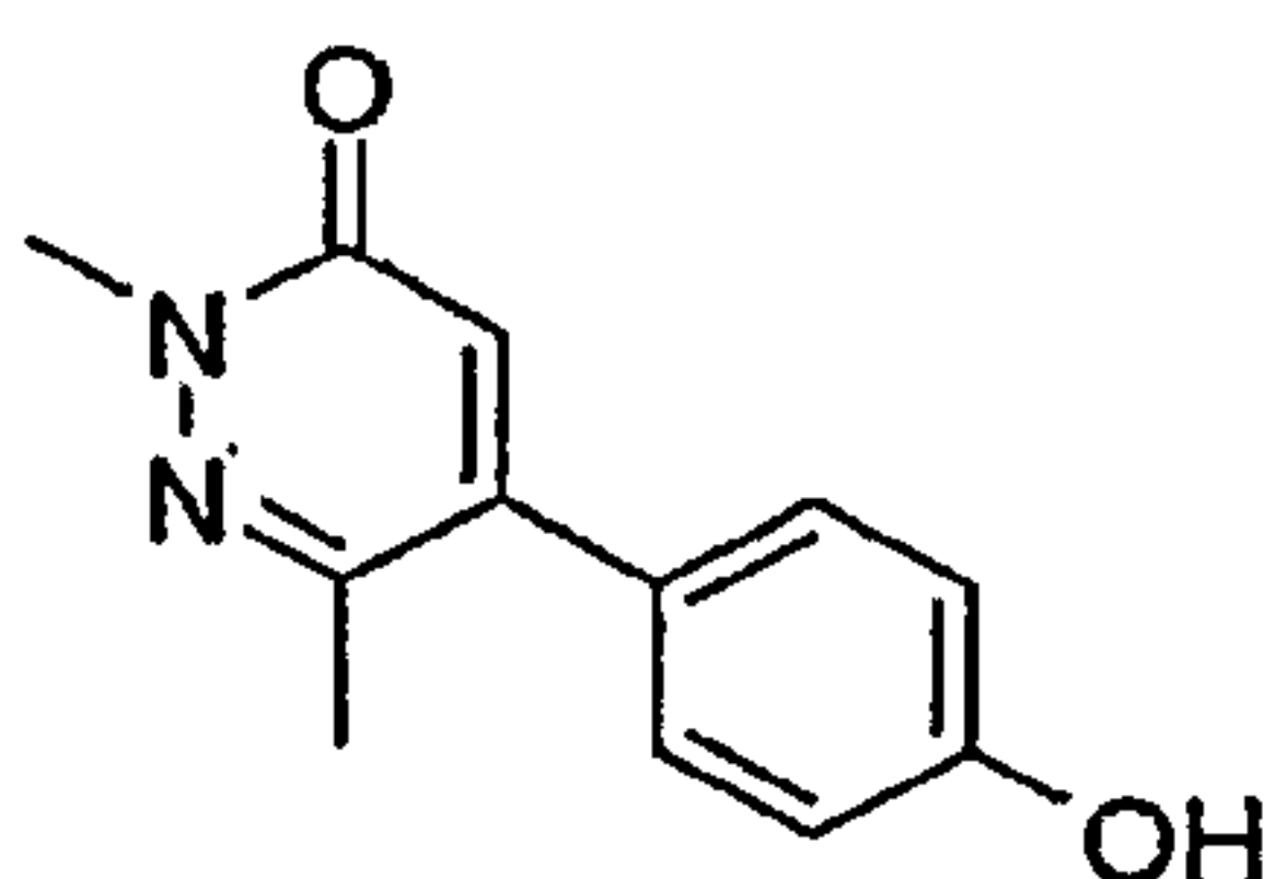
5-(4-Hydroxy-phenyl)-2,6-dimethyl-2H-pyridazin-3-one
