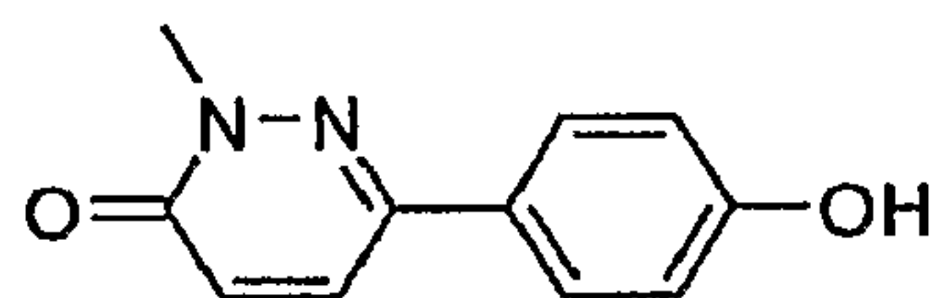
6-(4-Hydroxy-phenyl)-2-methyl-2H-pyridazin-3-one
