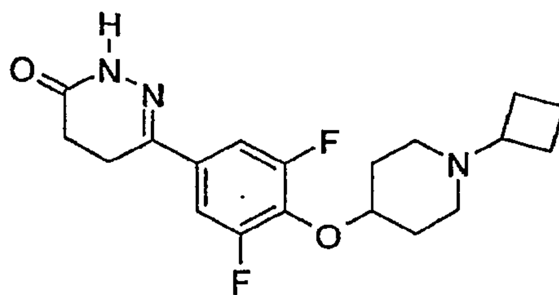
6-[4-(1-Cyclobutyl-piperidin-4-yloxy)-3,5-difluoro-phenyl]-4,5-dihydro-2H-pyridazin-3-one
