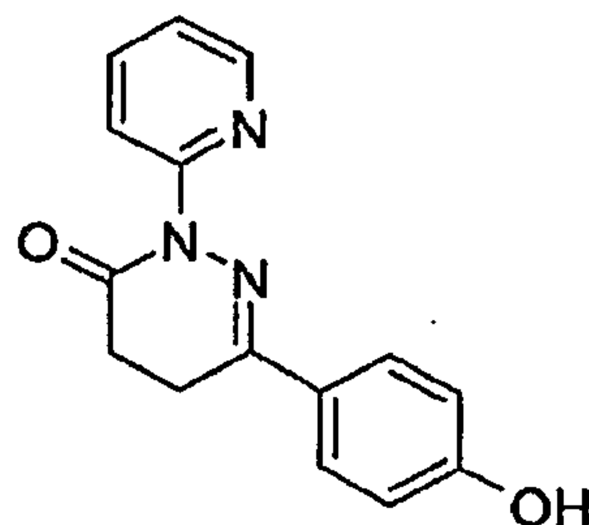
6-(4-Hydroxy-phenyl)-2-pyridin-2-yl-4,5-dihydro-2H-pyridazin-3-one
