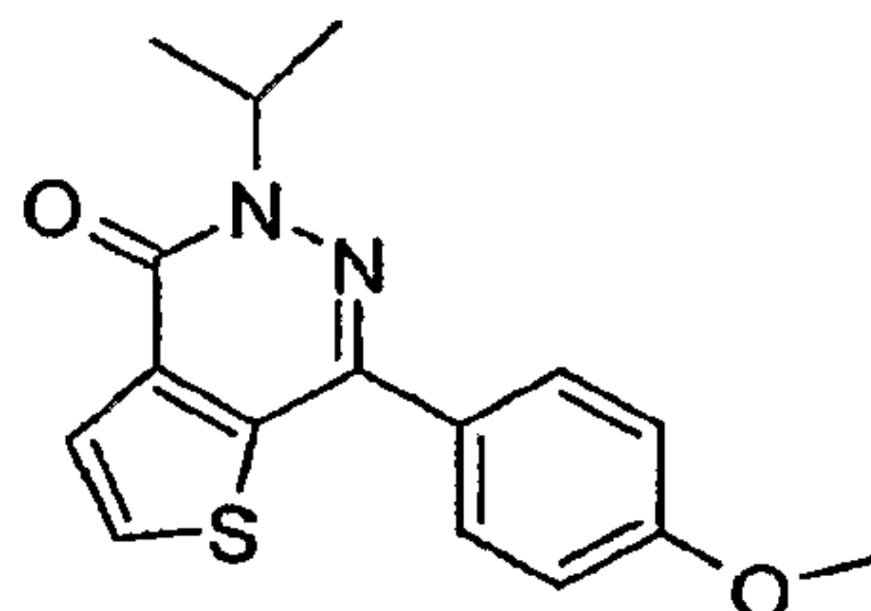
5-Isopropyl-7-(4-methoxy-phenyl)-5H -thieno[2,3-d]pyridazin-4-one
