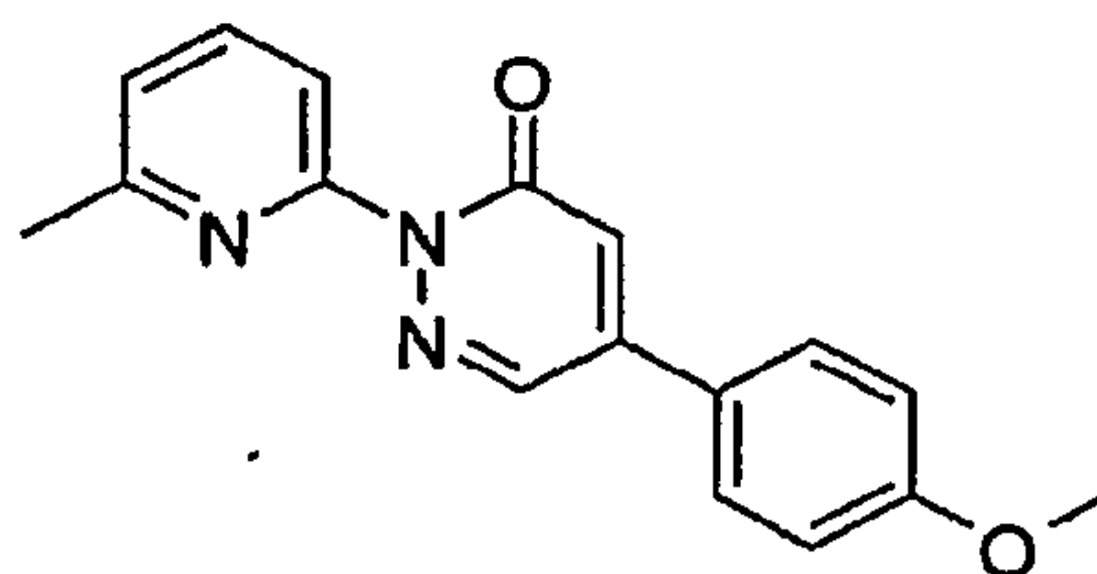
5-(4-Methoxy-phenyl)-2-(6-methyl-pyridin-2-yl)-2H-pyridazin-3-one
