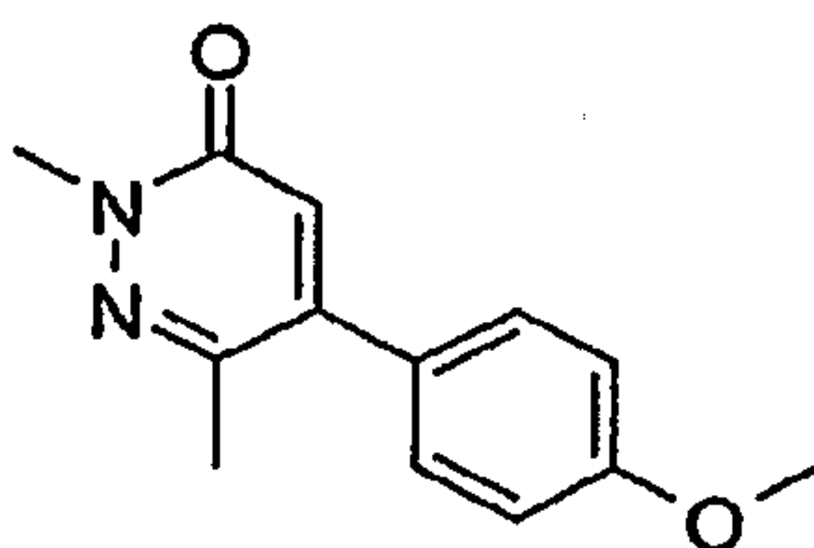
5-(4-Methoxy-phenyl)-2,6-dimethyl-2H-pyridazin-3-one
