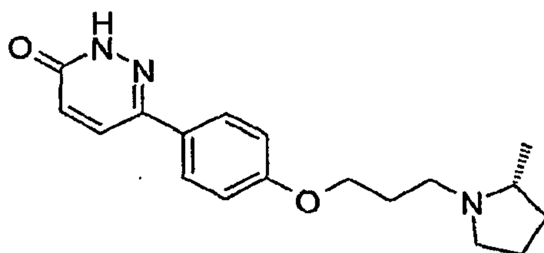
6-[4-[3-((R)-2-Methyl-pyrrolidin-1-yl)-propoxy]-phenyl]-2H-pyridazin-3-one
