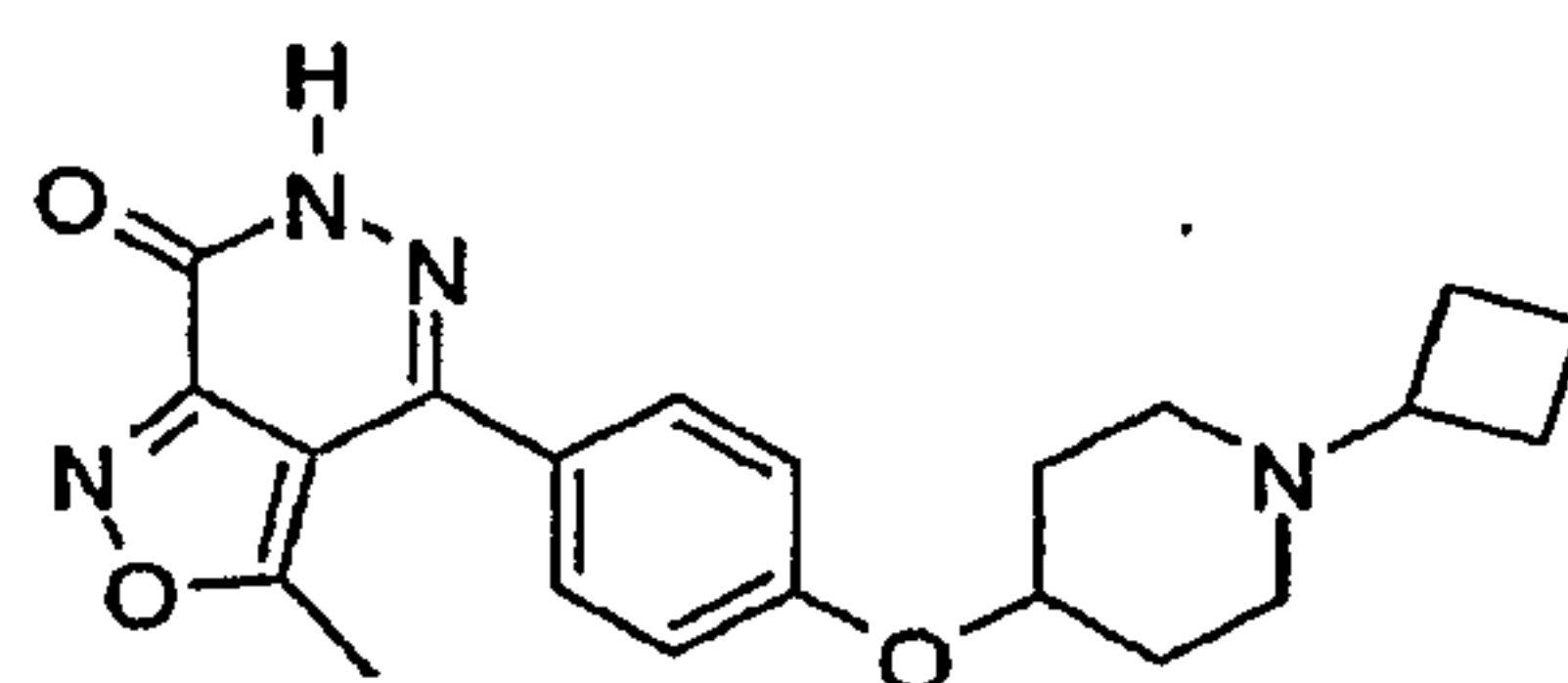
4-[4-(1-Cyclobutyl-piperidin-4-yloxy)-phenyl]-3-methyl-6H-isoxazolo[3,4-d]pyridazin-7-one
