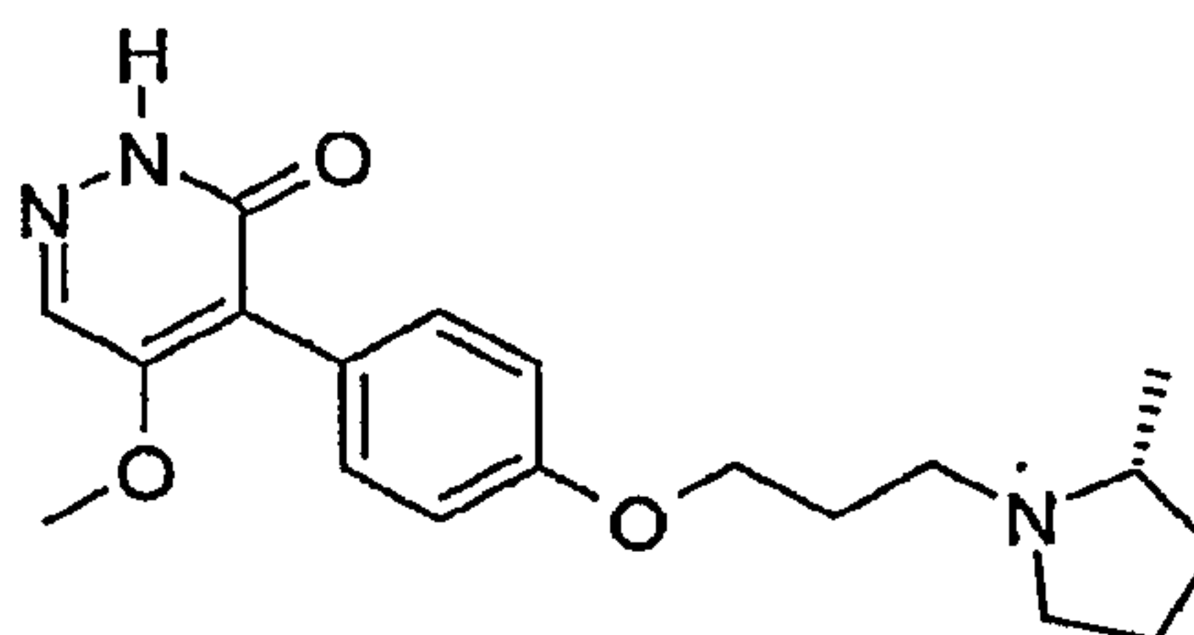
5-Methoxy-4-{4-[3-((R)-2-methyl-pyrrolidin-1-yl)-propoxy]-phenyl}-2H-pyridazin-3-one
