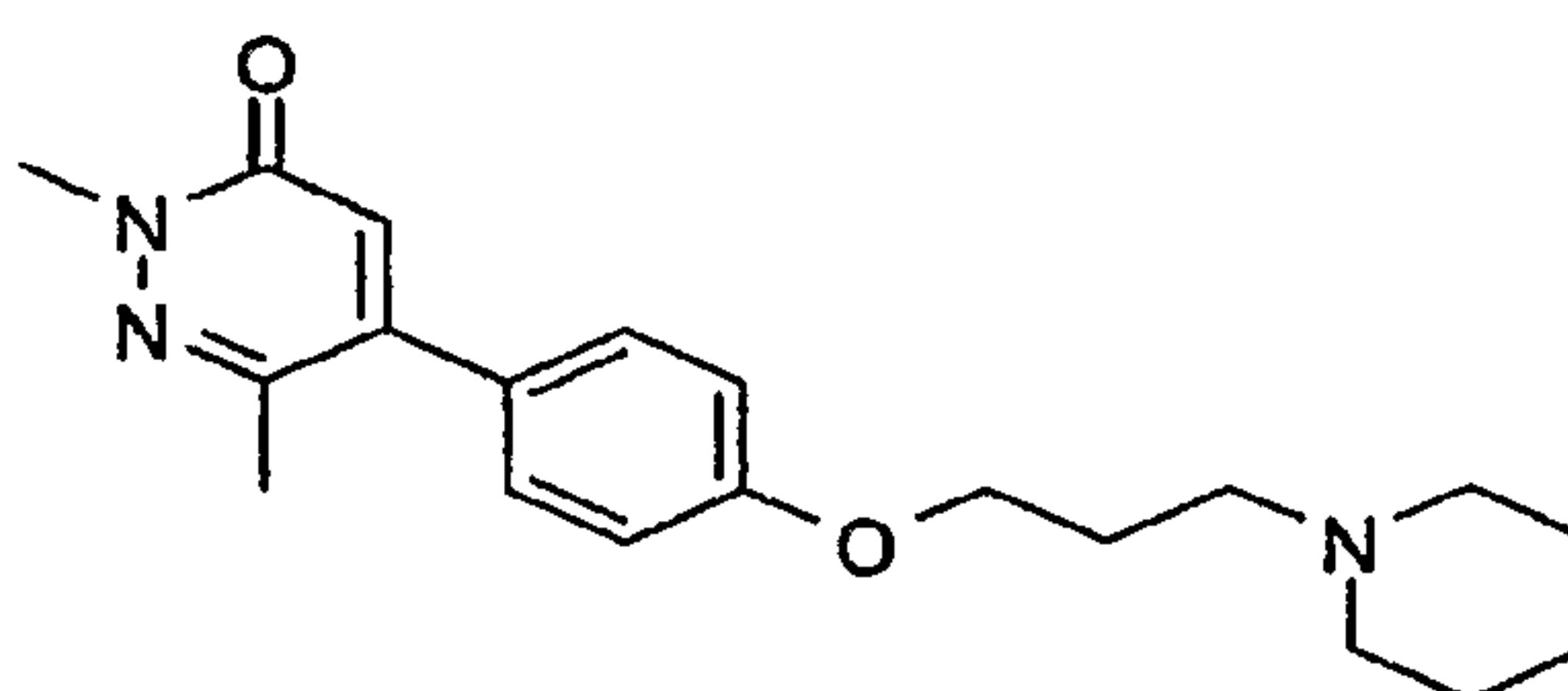
2,6-Dimethyl-5-[4-(3-piperidin-1-yl)-propoxy]-2H-pyridazin-3-one
