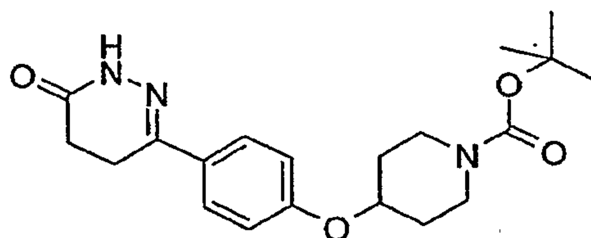
4-[4-(6-Oxo-1,4,5,6-tetrahydro-pyridazin-3-yl)-phenoxy]-piperidine-1-carboxylic acid tert-butyl ester
