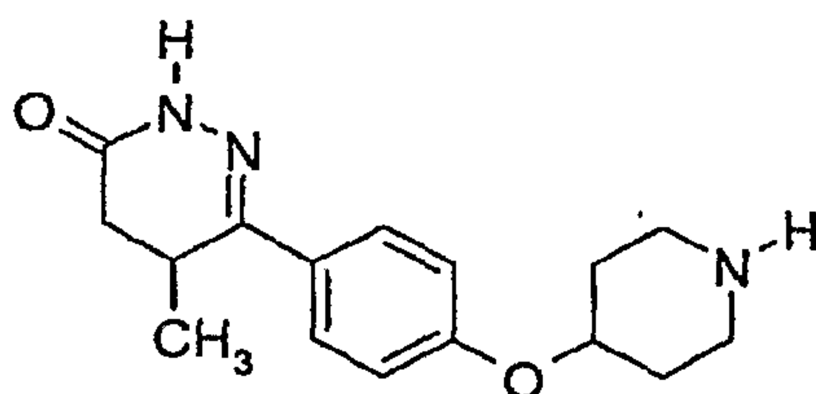
5-Methyl-6-[4-(piperidin-4-yloxy)-phenyl]-4,5-dihydro-2H-pyridazin-3-one
