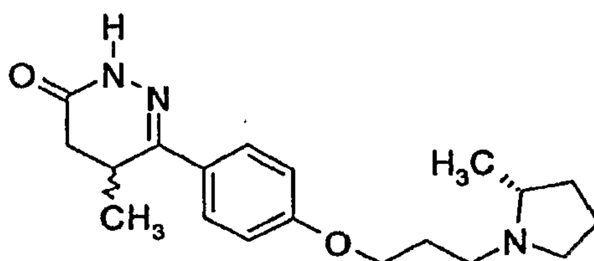
5-Methyl-6-{4-[3-((R)-2-methyl-pyrrolidin-1-yl)-propoxy]-phenyl}-4,5-dihydro-2H-pyridazin-3-one
