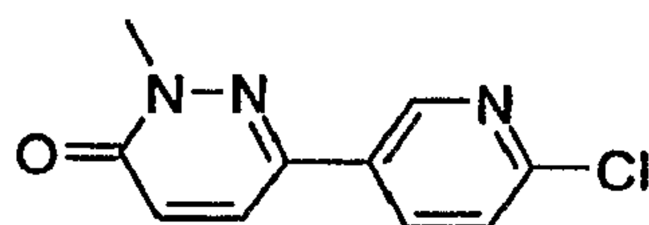
6-(6-Chloro-pyridin-3-yl)-2-methyl-2H-pyridazin-3-one
