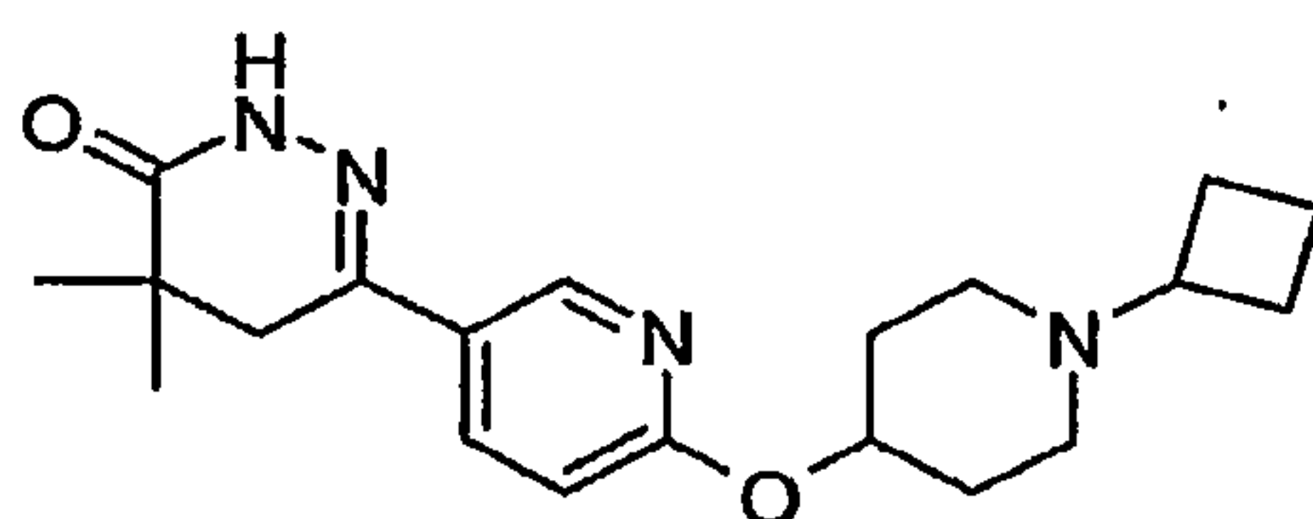
6-[6-(1-Cyclobutyl-piperidin-4-yloxy)-pyridin-3-yl]-4,4-dimethyl-4,5-dihydro-2H-pyridazin-3-one
