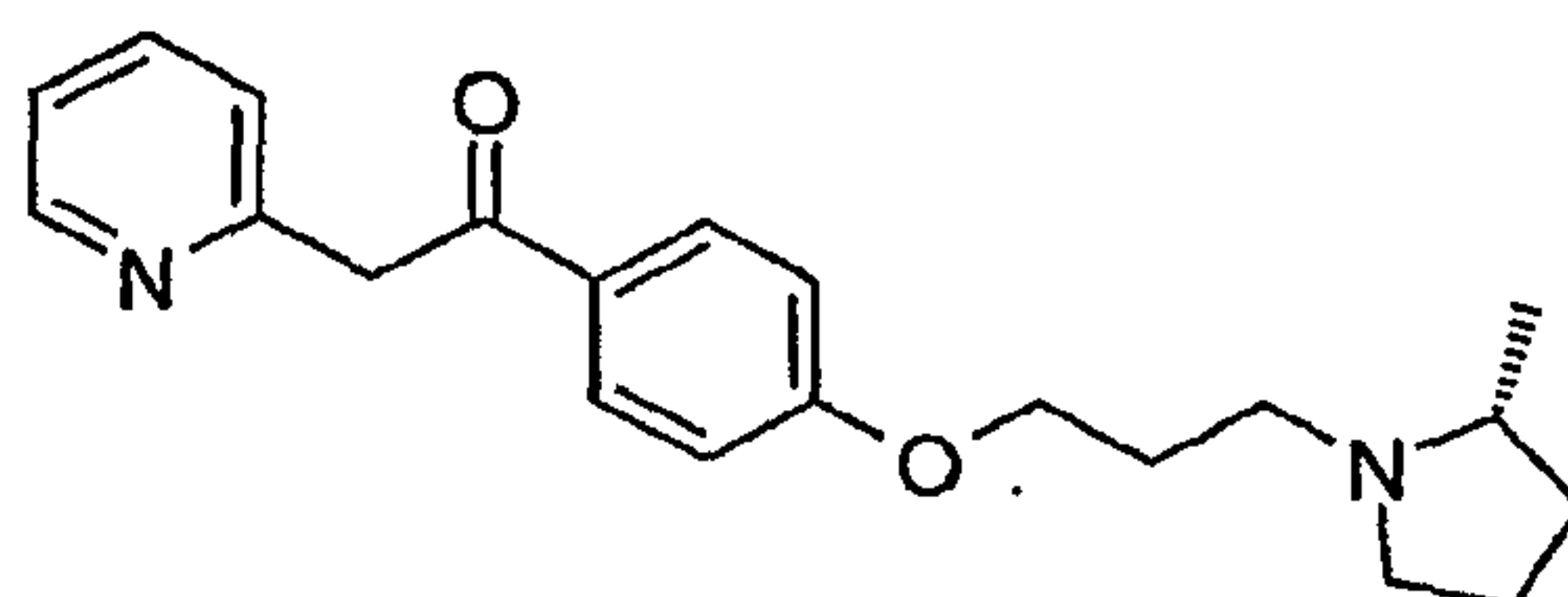
1-{4-[3-((R)-2-Methyl-pyrrolidin-1-yl)-propoxy]-phenyl}-2-pyridin-2-yl-ethanone
