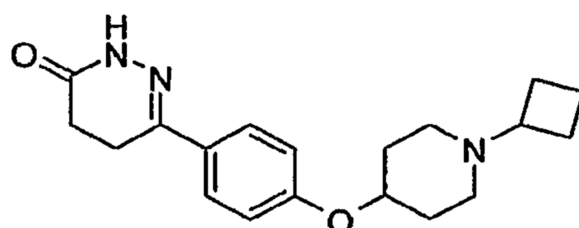
6-[4-(1-Cyclobutyl-piperidin-4-yloxy)-phenyl]-4,5-dihydro-2H-pyridazin-3-one
