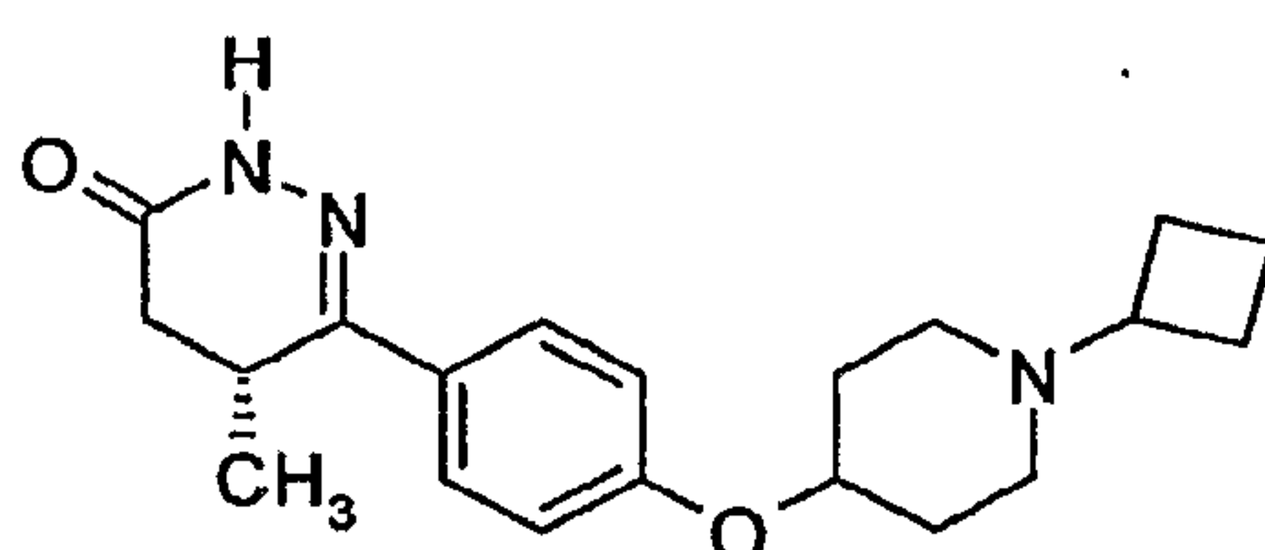
(R)-6-[4-(1-Cyclobutyl-piperidin-4-yloxy)-phenyl]-5-methyl-4,5-dihydro-2H-pyridazin-3-one
