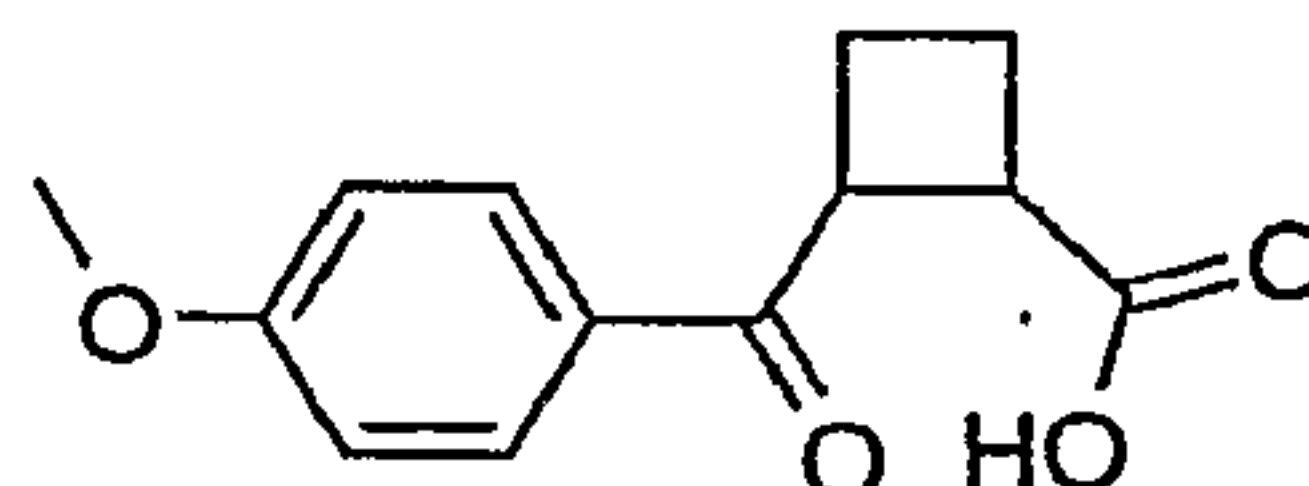
2-(4-Methoxy-benzoyl)-cyclobutanecarboxylic acid
