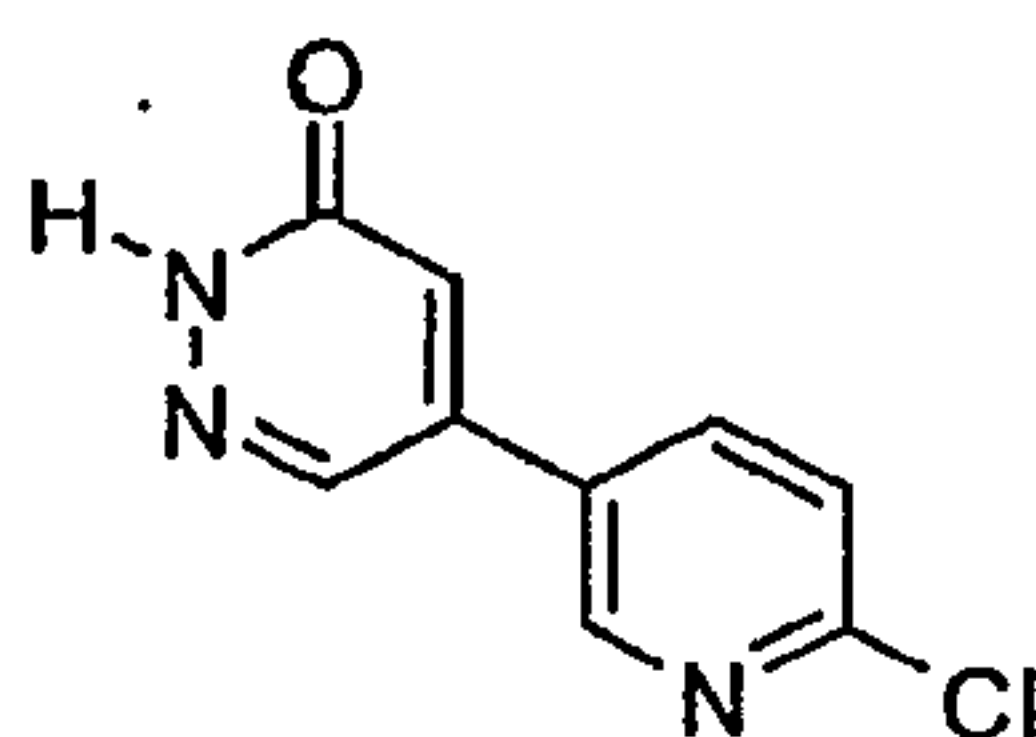
5-(6-Chloro-pyridin-3-yl)-2H- pyridazin-3-one
