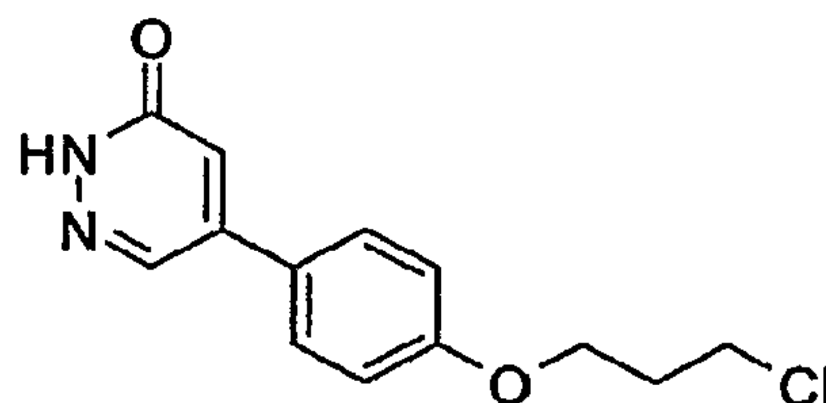
5-[4-(3-Chloro-propoxy)-phenyl]-2H-pyridazin-3-one
