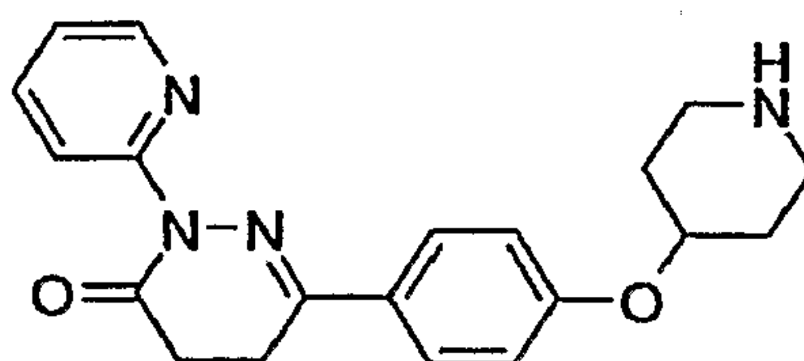
6-[4-(Piperidin-4-yloxy)-phenyl]-2-pyridin-2-yl-4,5-dihydro-2H-pyridazin-3-one
