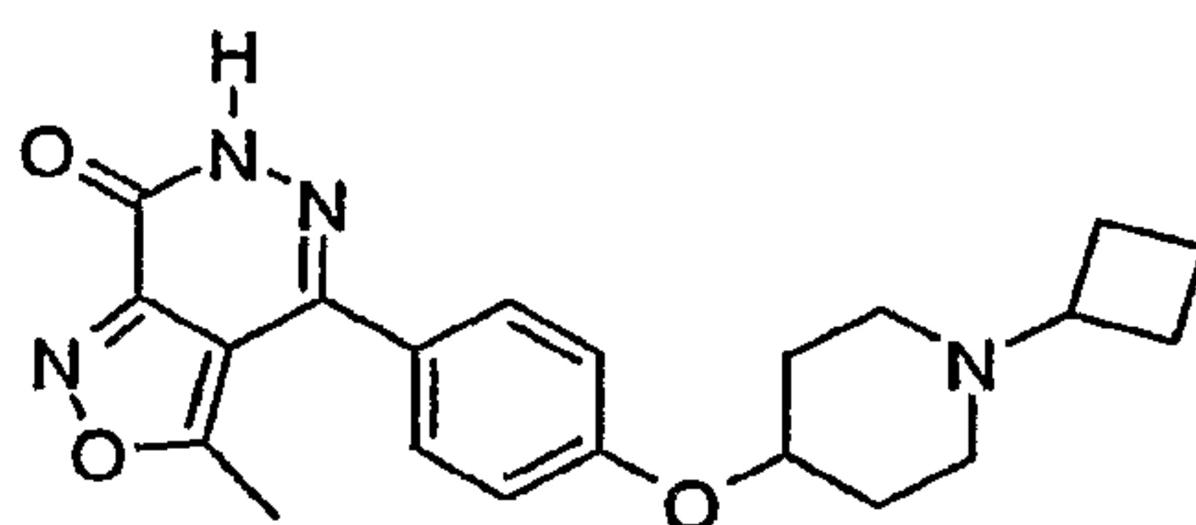
4-[4-(1-Cyclobutyl-piperidin-4-yloxy)-phenyl]-3-methyl-6H-isoxazolo[3,4-d]pyridazin-7-one
