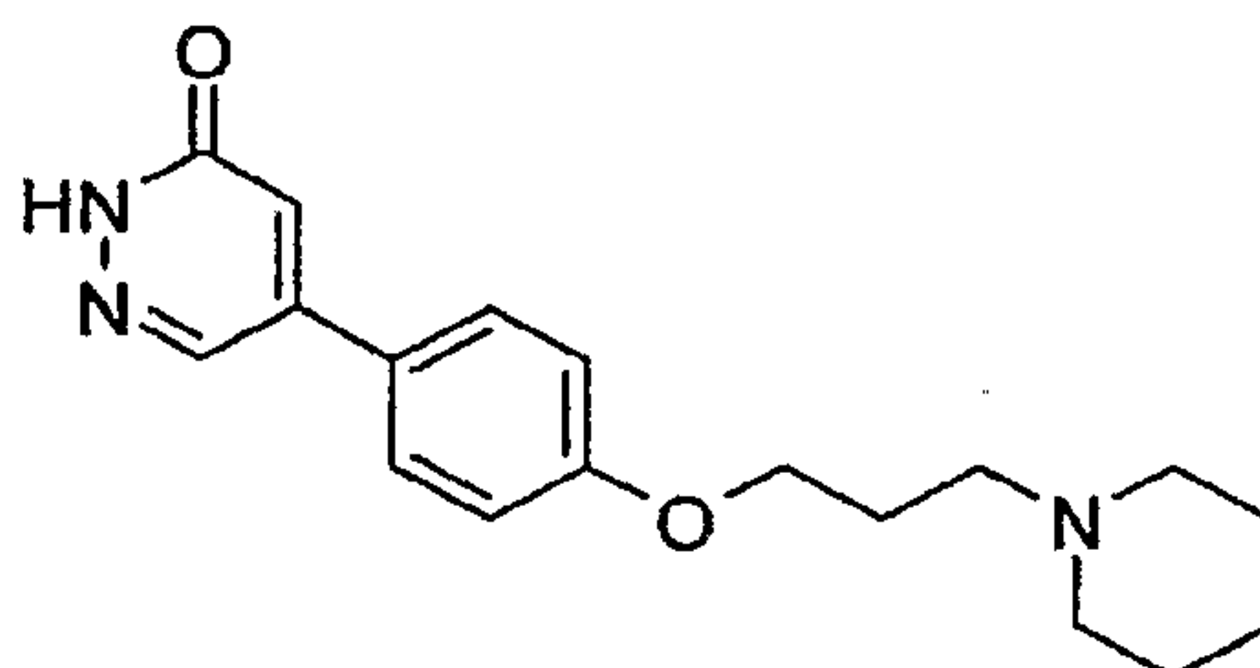
2-Methyl-5-[4-(3-piperidin-1-yl-propoxy)-phenyl]-2H-pyridazin-3-one
