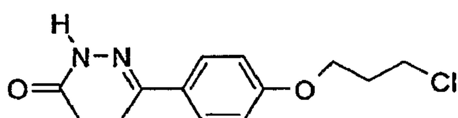
6-[4-(3-Chloro-propoxy)-phenyl]-4,5-dihydro-2H-pyridazin-3-one
