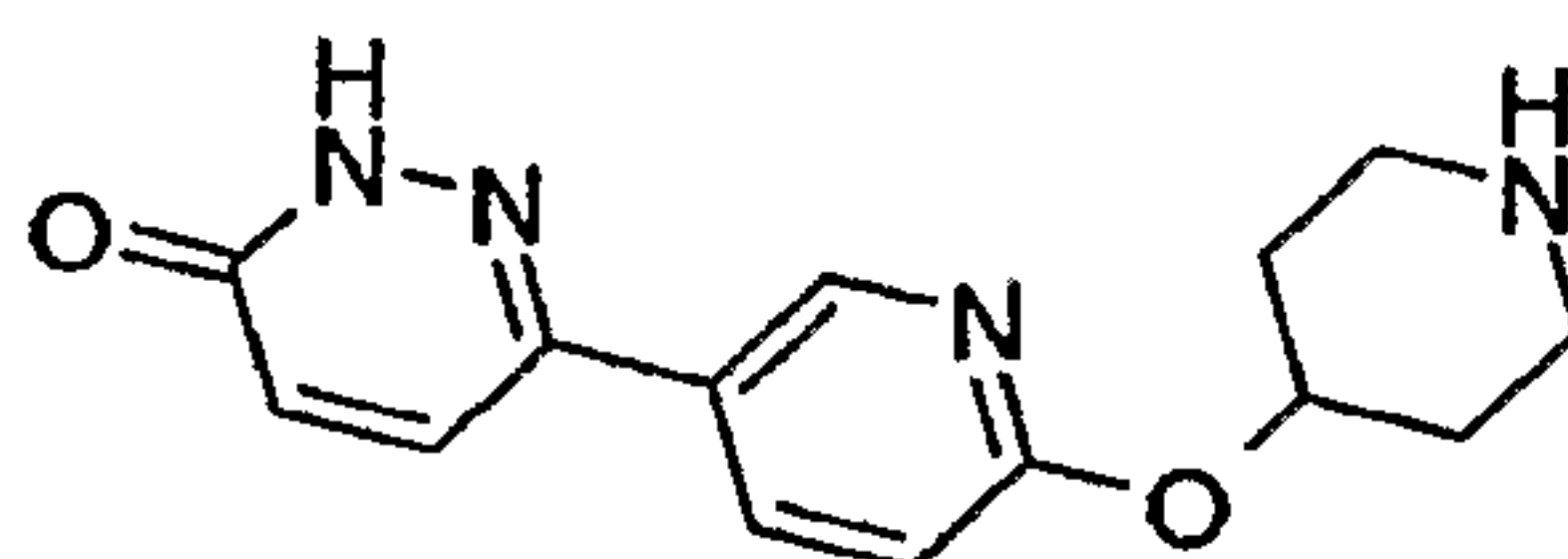
6-[6-(Piperidin-4-yloxy)-pyridin-3-yl]-2H-pyridazin-3-one
