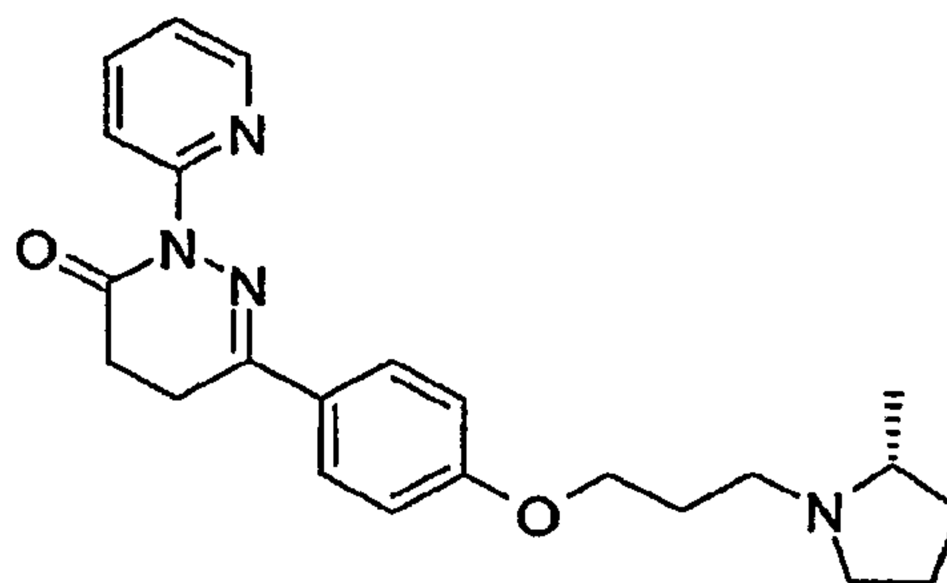
6-[4-[3-((R)-2-Methyl-pyrrolidin-1-yl)-propoxy]-phenyl]-2-pyridin-2-yl-4,5-dihydro-2H-pyridazin-3-one
