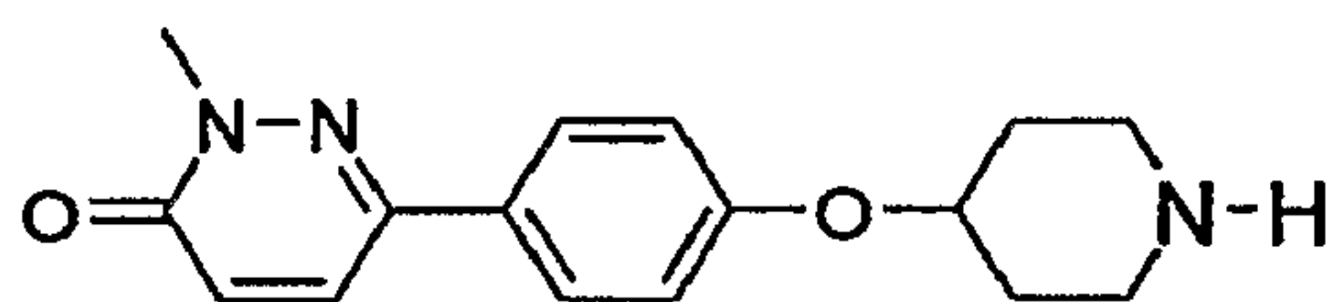
2-Methyl-6-[4-(piperidin-4-yloxy)-phenyl]-2H-pyridazin-3-one
