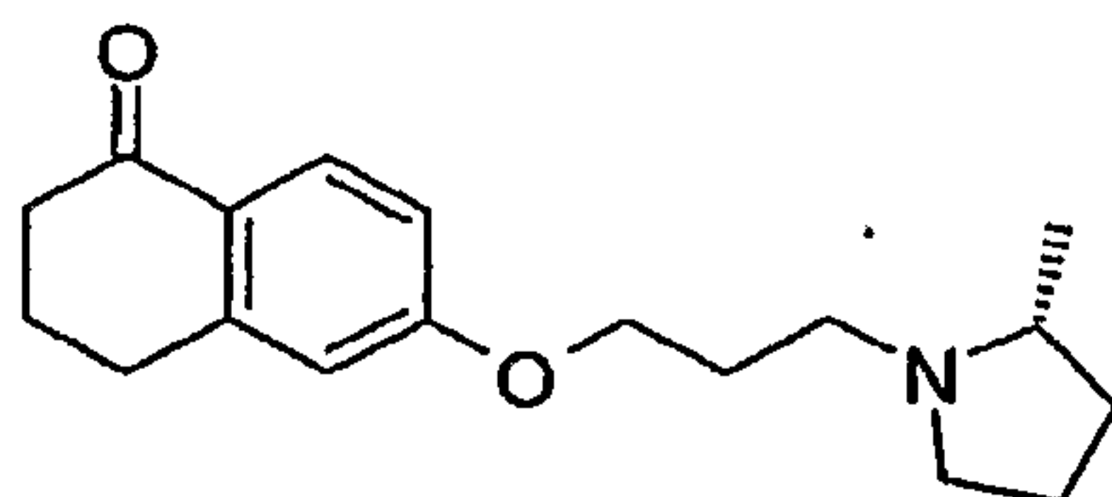
6-[3-((R)-2-Methyl-pyrrolidin-1-yl)-propoxy]-3,4-dihydro-2H-naphthalen-1-one
