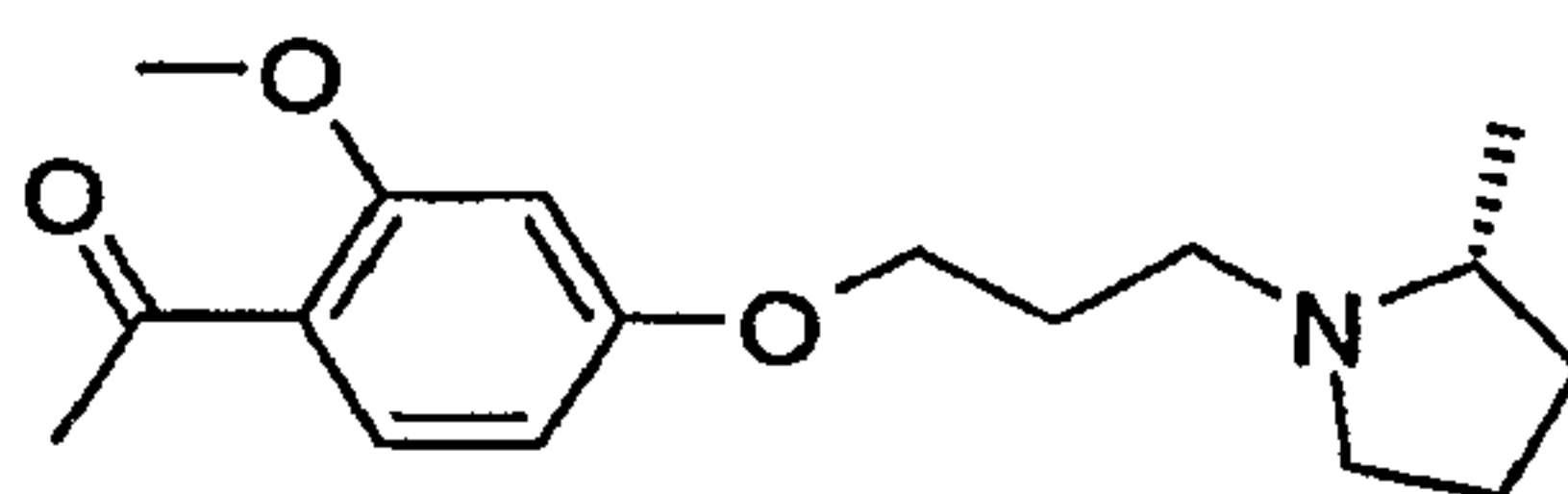
1-[2-Methoxy-4-[3-((R)-2-methyl-pyrrolidin-1-yl)-propoxy]-phenyl]-ethanone
