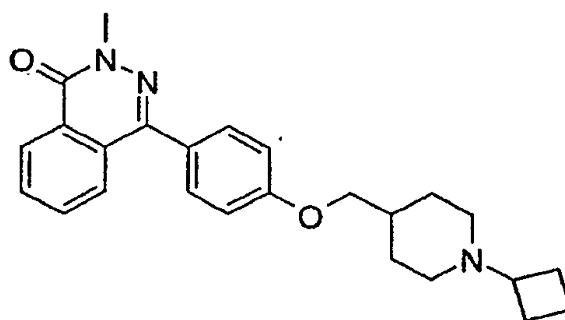
4-[4-(1-Cyclobutyl-piperidin-4-ylmethoxy)-phenyl]-2-methyl-2H-phthalazin-1-one
