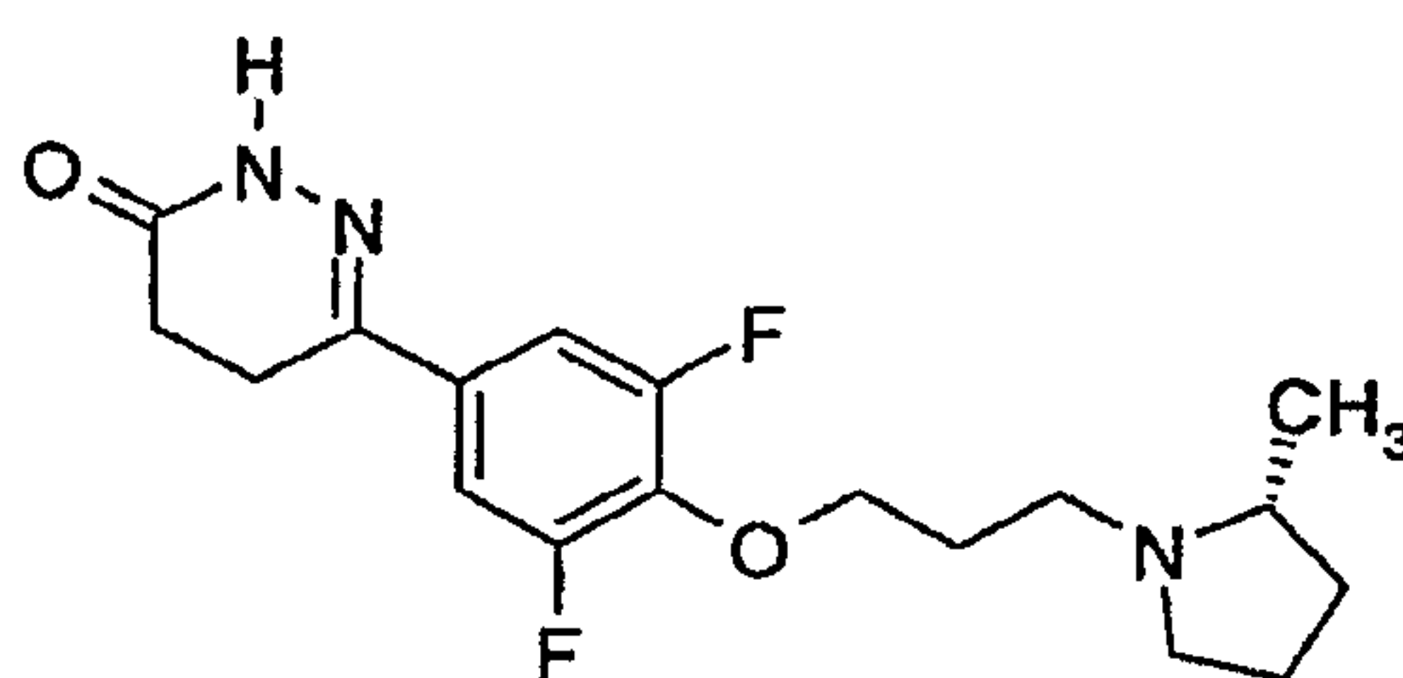
6-{3,5-Difluoro-4-[3-(( R )-2-methyl-pyrrolidin-1-yl)-propoxy]-phenyl}-4,5-dihydro-2H-pyridazin-3-one
