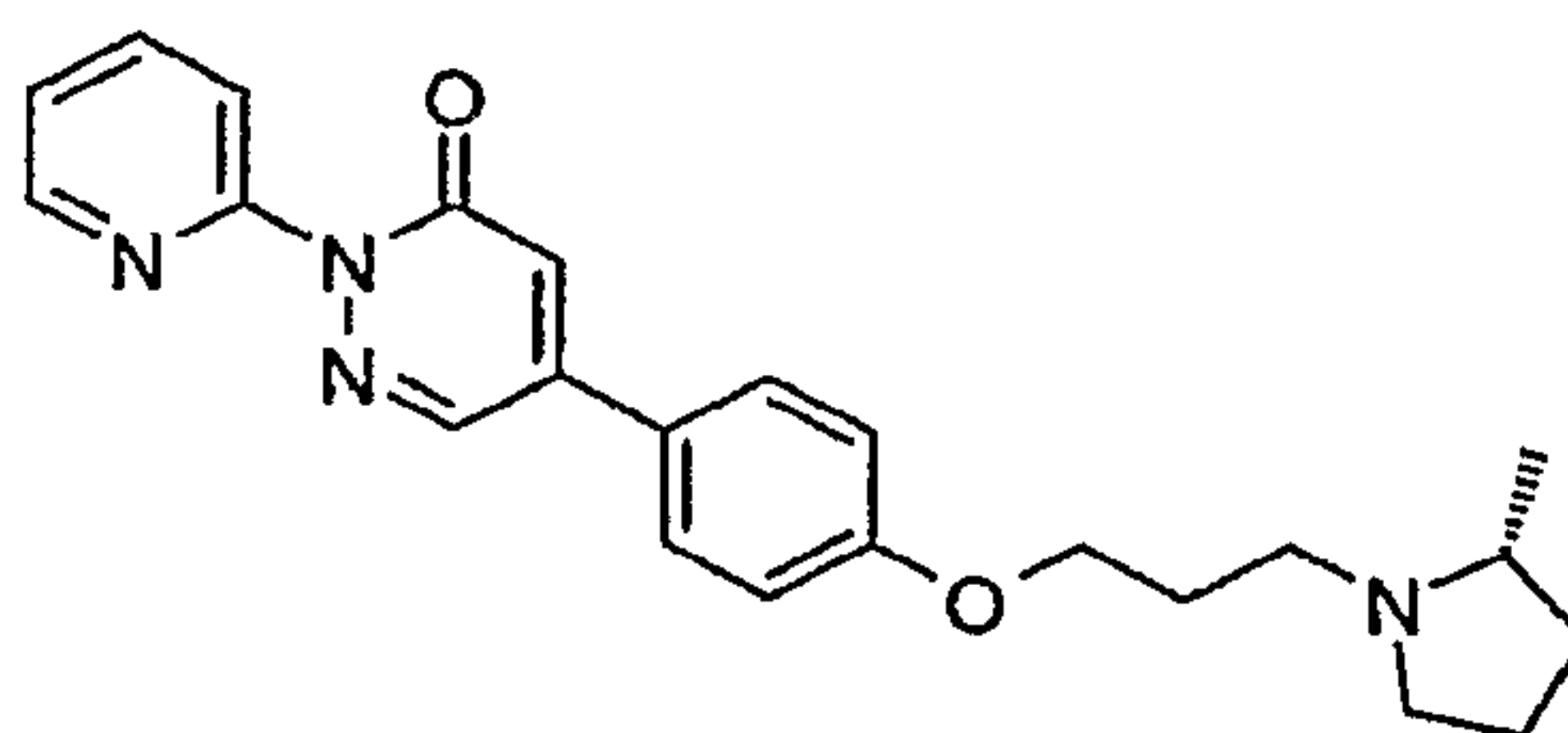
5-{4-[3-((R)-2-Methyl-pyrrolidin-1-yl)-propoxy]-phenyl}-2-pyridin-2-yl-2H-pyridazin-3-one
