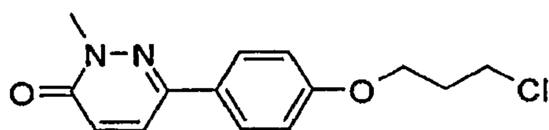
6-[4-(3-Chloro-propoxy)-phenyl]-2-methyl-2H-pyridazin-3-one
