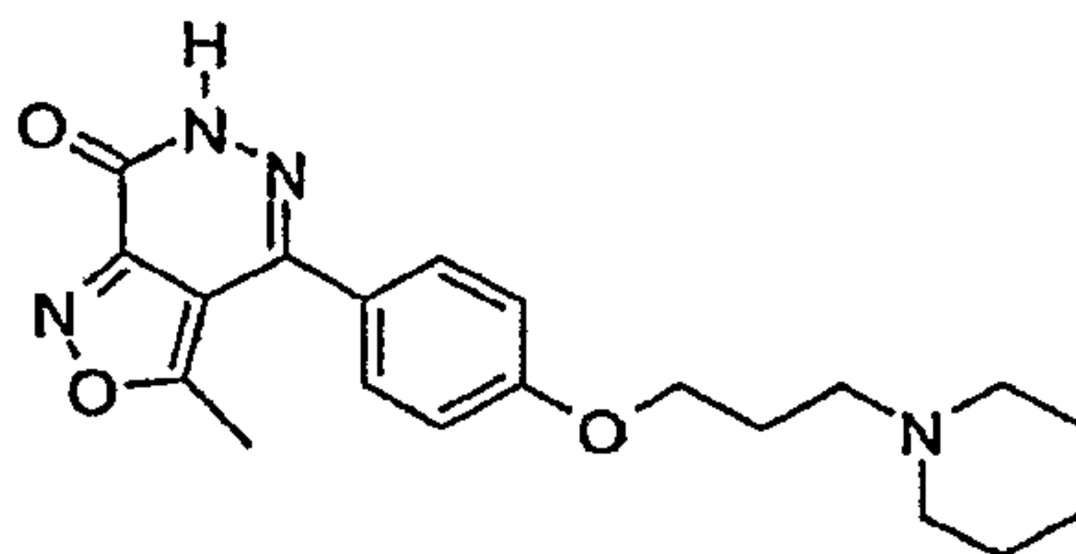
3-Methyl-4-[4-(3-piperidin-1-yl-propoxy)-phenyl]-6H-isoxazolo[3,4-d]pyridazin-7-one
