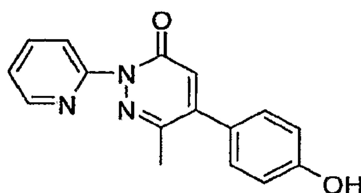
5-(4-Hydroxy-phenyl)-6-methyl-2-pyridin-2-yl-2H-pyridazin-3-one
