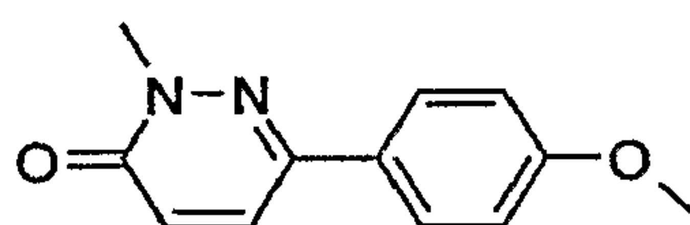
6-(4-Methoxy-phenyl)-2-methyl-2H-pyridazin-3-one
