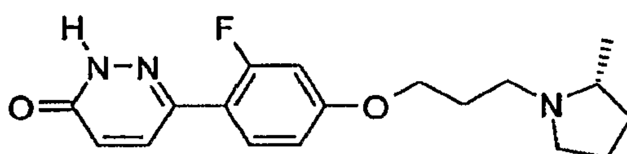
6-{2-Fluoro-4-[3-((R)-2-methyl-pyrrolidin-1-yl)-propoxy]-phenyl}-2H-pyridazin-3-one
