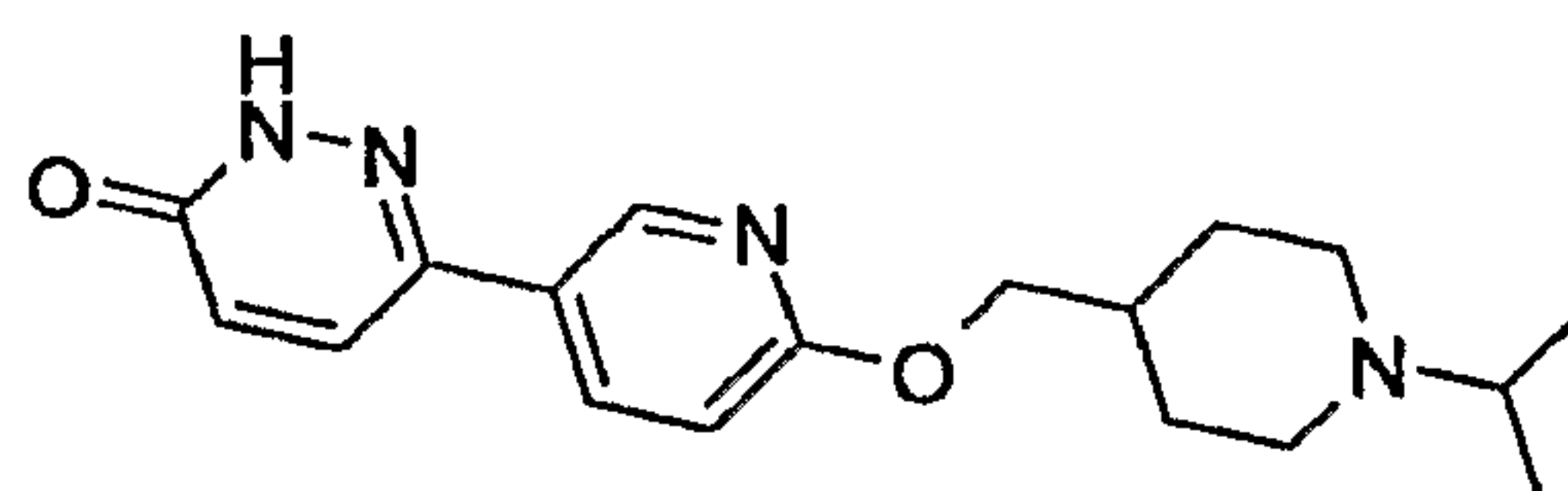
6-[6-(1-isopropyl-piperidin-4-ylmethoxy)-pyridin-3-yl]-2H-pyridazin-3-one
