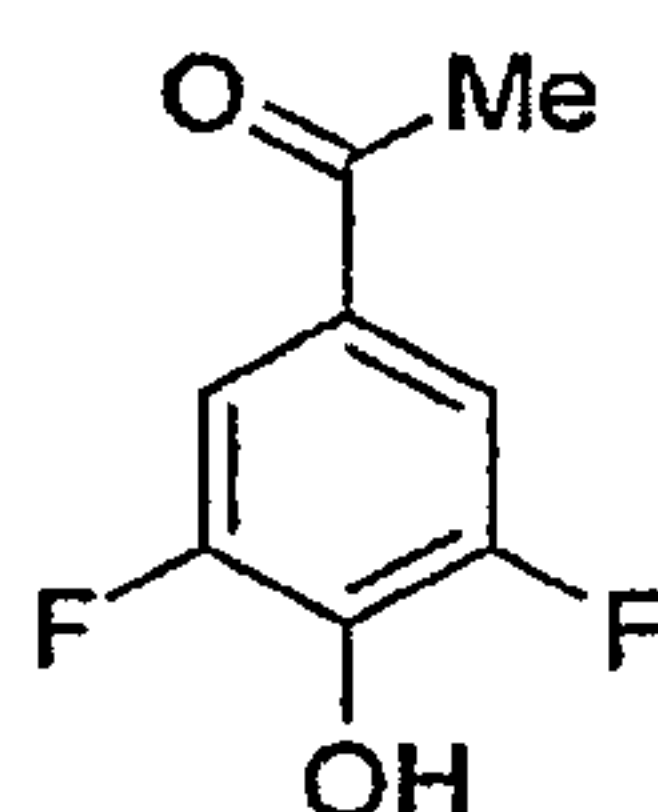
1-(3,5-Difluoro-4-hydroxyphenyl)-ethanone
