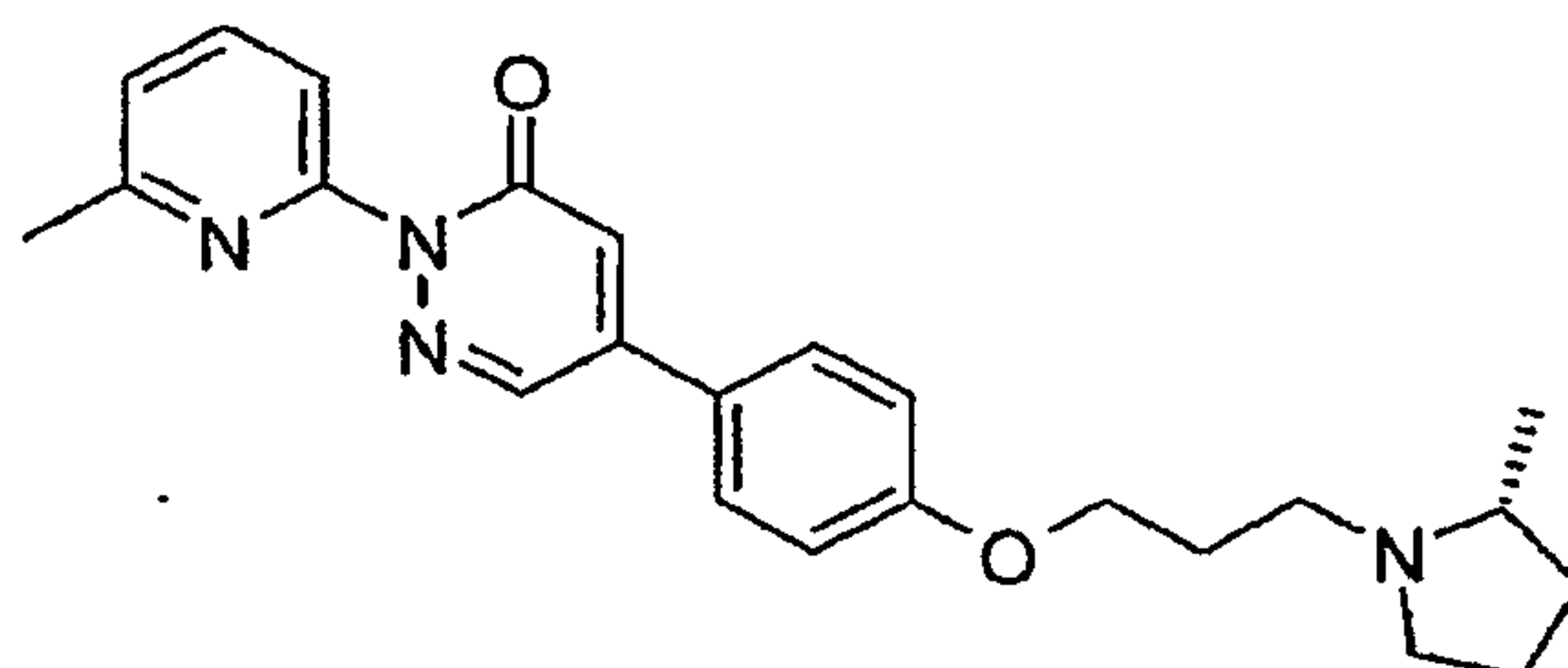
2-(6-Methyl-pyridin-2-yl)-5-{4-[3-((R)-2-methyl-pyrrolidin-1-yl)-propoxy]-phenyl}-2H-pyridazin-3-one
