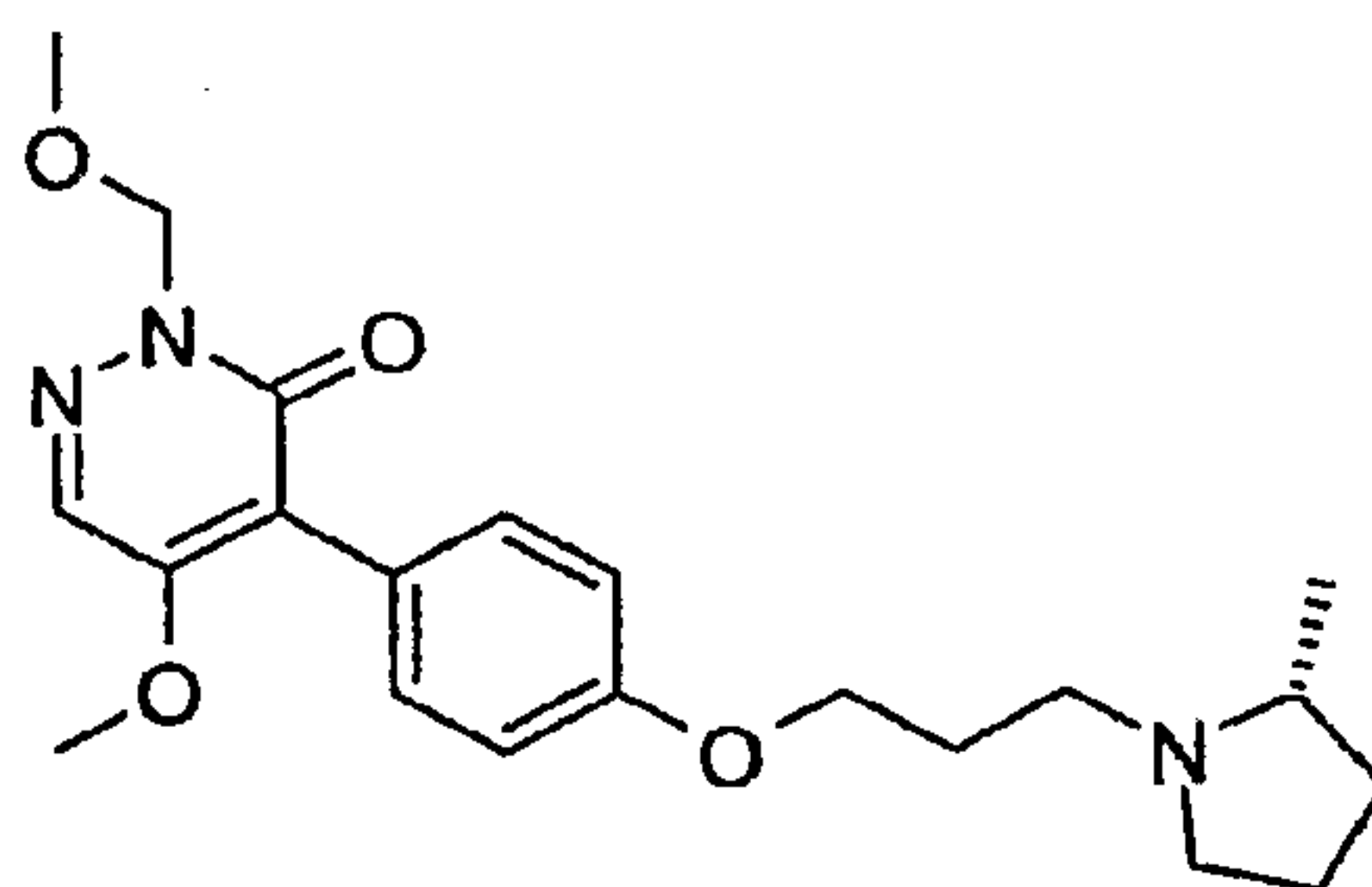
5-Methoxy-2-methoxymethyl-4-{4-[3-((R)-2-methyl-pyrrolidin-1-yl)-propoxy]-phenyl}-2H-pyridazin-3-one
