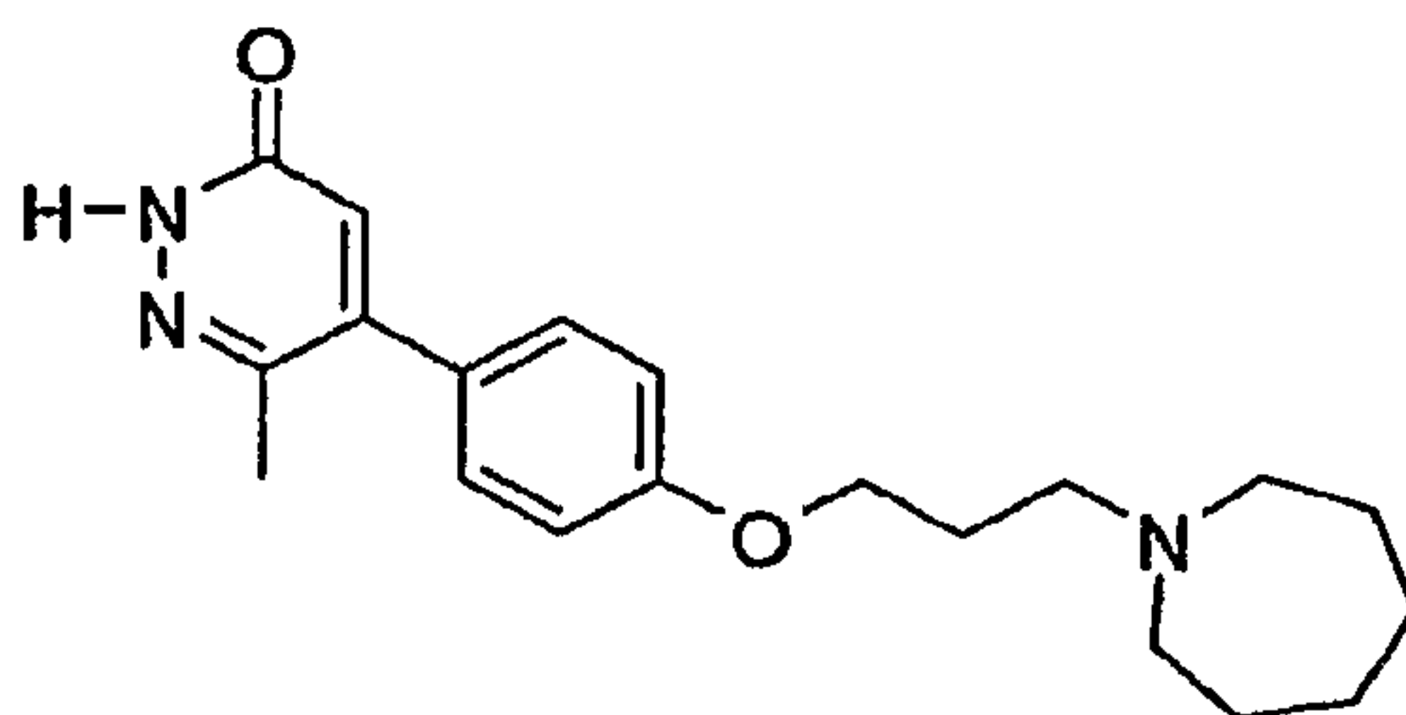
5-[4-(3-Azepan-1-yl-propoxy)-phenyl]-6-methyl-2H-pyridazin-3-one
