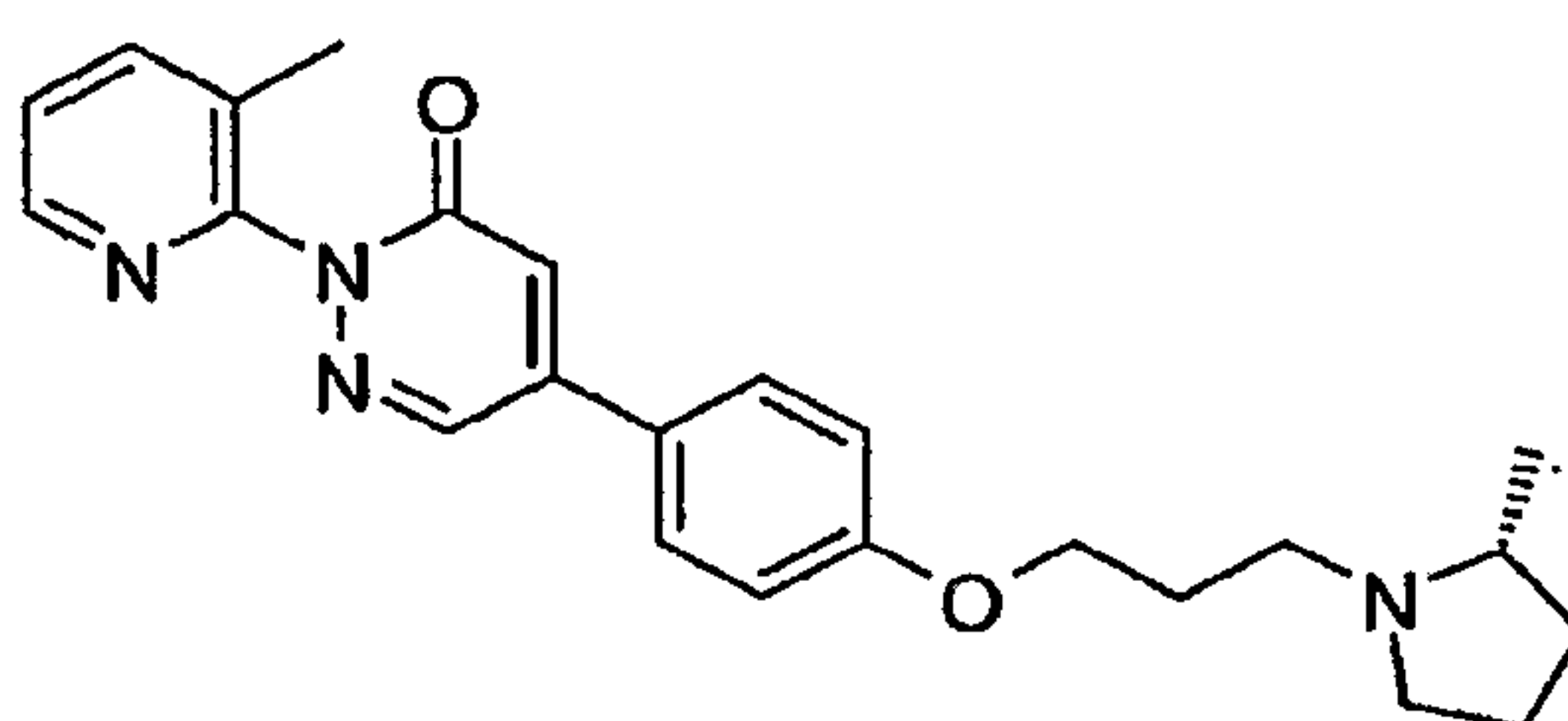
2-(3-Methyl-pyridin-2-yl)-5-{4-[3-((R)-2-methylpyrrolidin-1-yl)-propoxy]-phenyl}-2H-pyridazin-3-one
