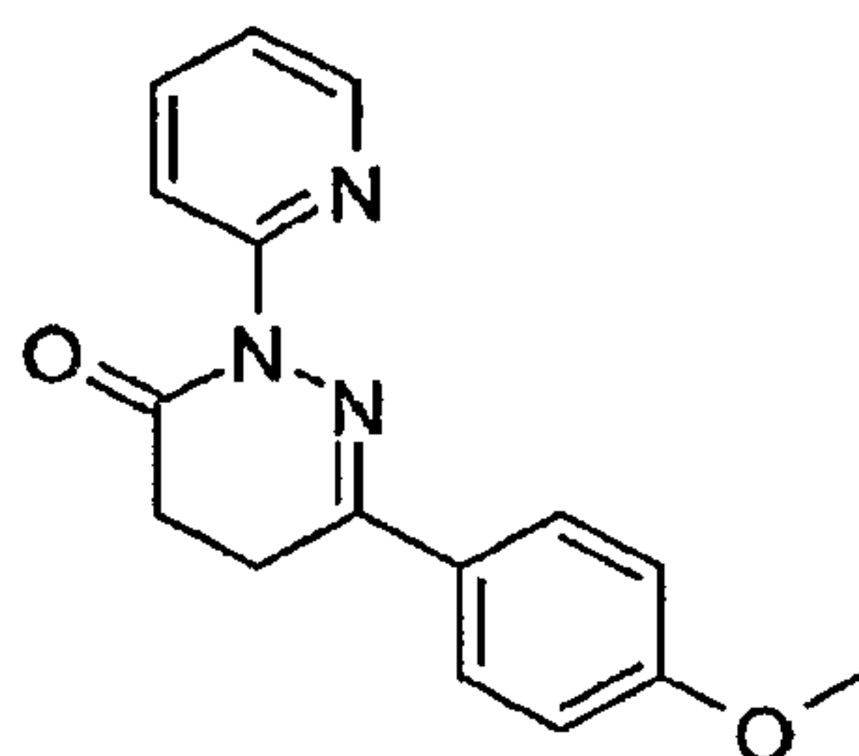
6-(4-Methoxy-phenyl)-2-pyridin-2-yl-4,5-dihydro-2H-pyridazin-3-one
