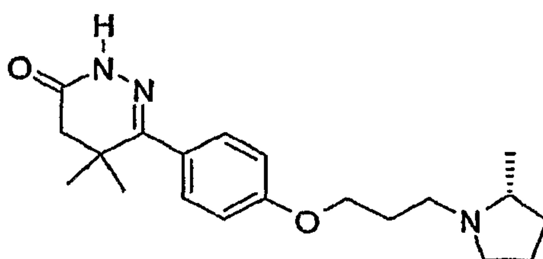
5,5-Dimethyl-6-{4-[3-((R)-2-methylpyrrolidin-1-yl)propoxy]phenyl}-4,5-dihydro-2H-pyridazin-3-one
