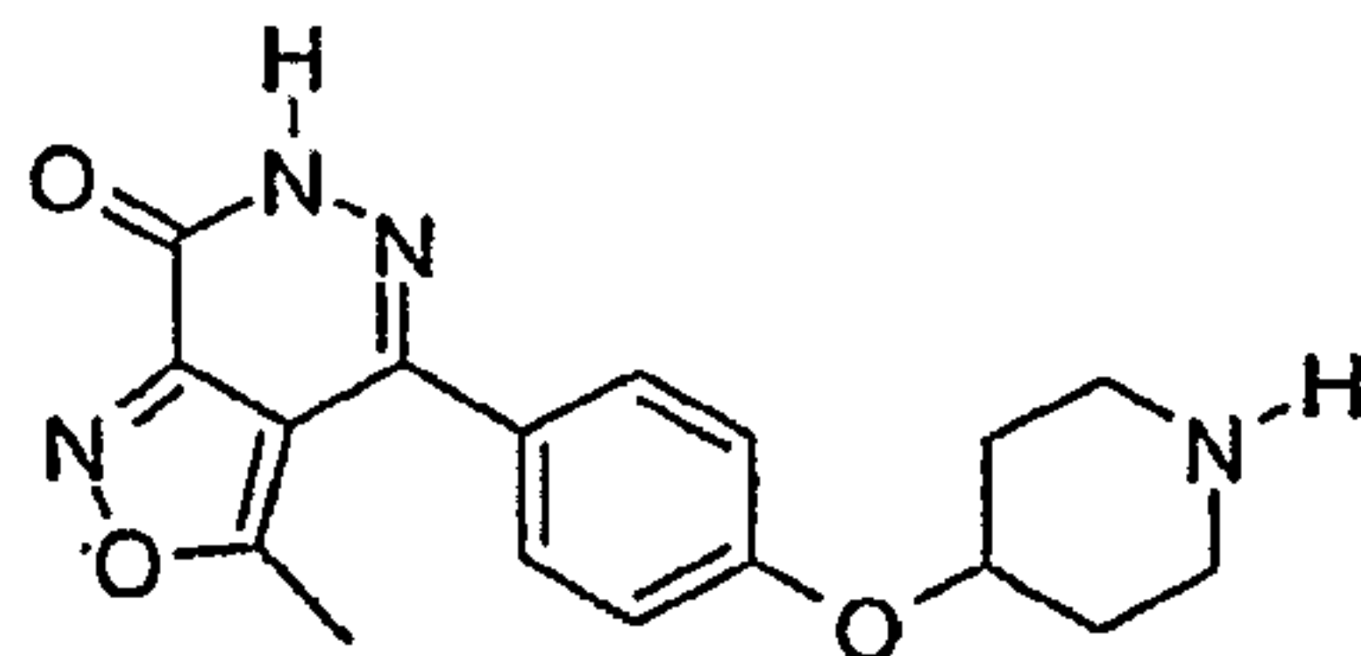
3-Methyl-4-[4-(piperidin-4-yloxy)-phenyl]-6H-isoxazolo[3,4-d]pyridazin-7-one
