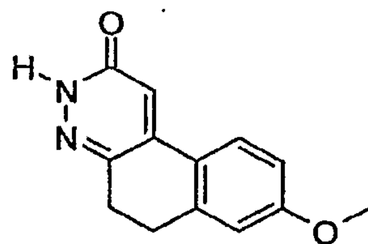
8-Methoxy-5,6-dihydro-3H-benzo[f]cinnolin-2-one
