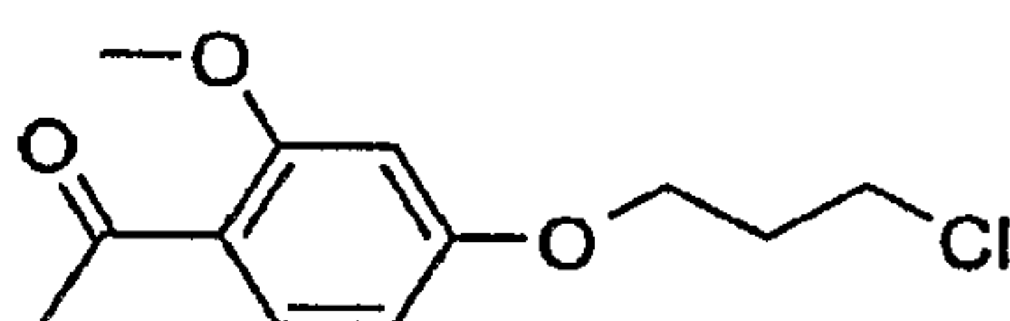
1-[4-(3-Chloro-propoxy)-2-methoxy-phenyl]-ethanone
