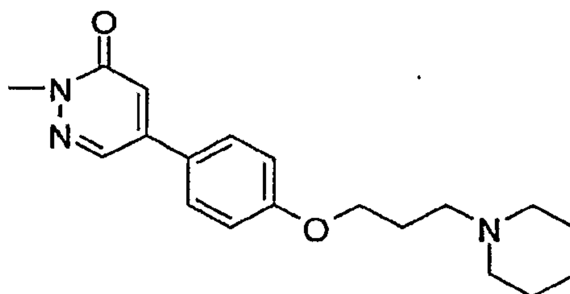
2-Methyl-5-[4-(3-piperidin-1-yl-propoxy)-phenyl]-2H-pyridazin-3-one
