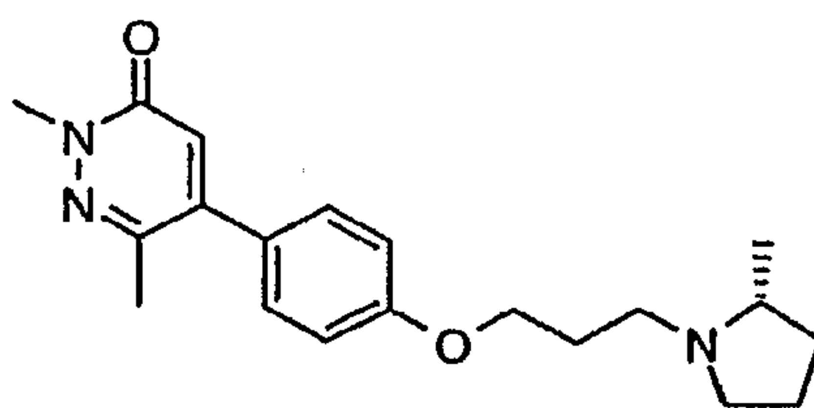
2,6-Dimethyl-5-{4-[3-((R)-2-methylpyrrolidin-1-yl)-propoxy]-phenyl}-2H-pyridazin-3-one
