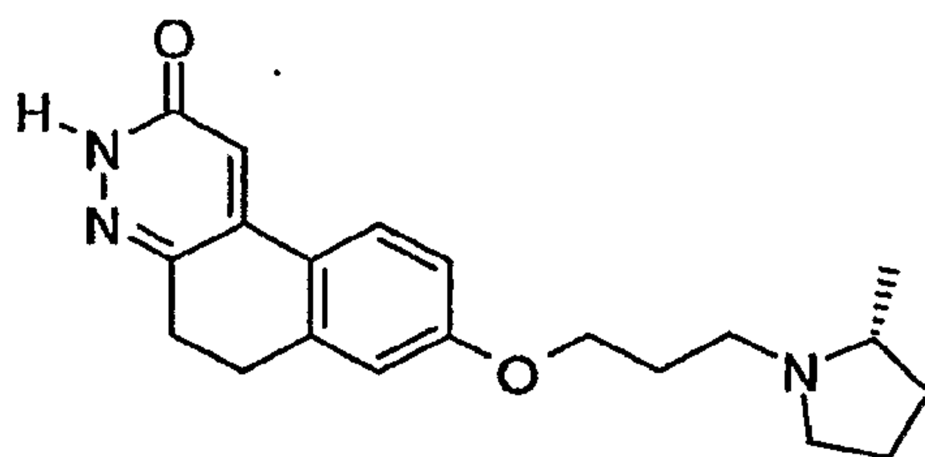
8-[3-((R)-2-Methyl-pyrrolidin-1-yl)-propoxy]-5,6-dihydro-3H-benzo[f]cinnolin-2-one
