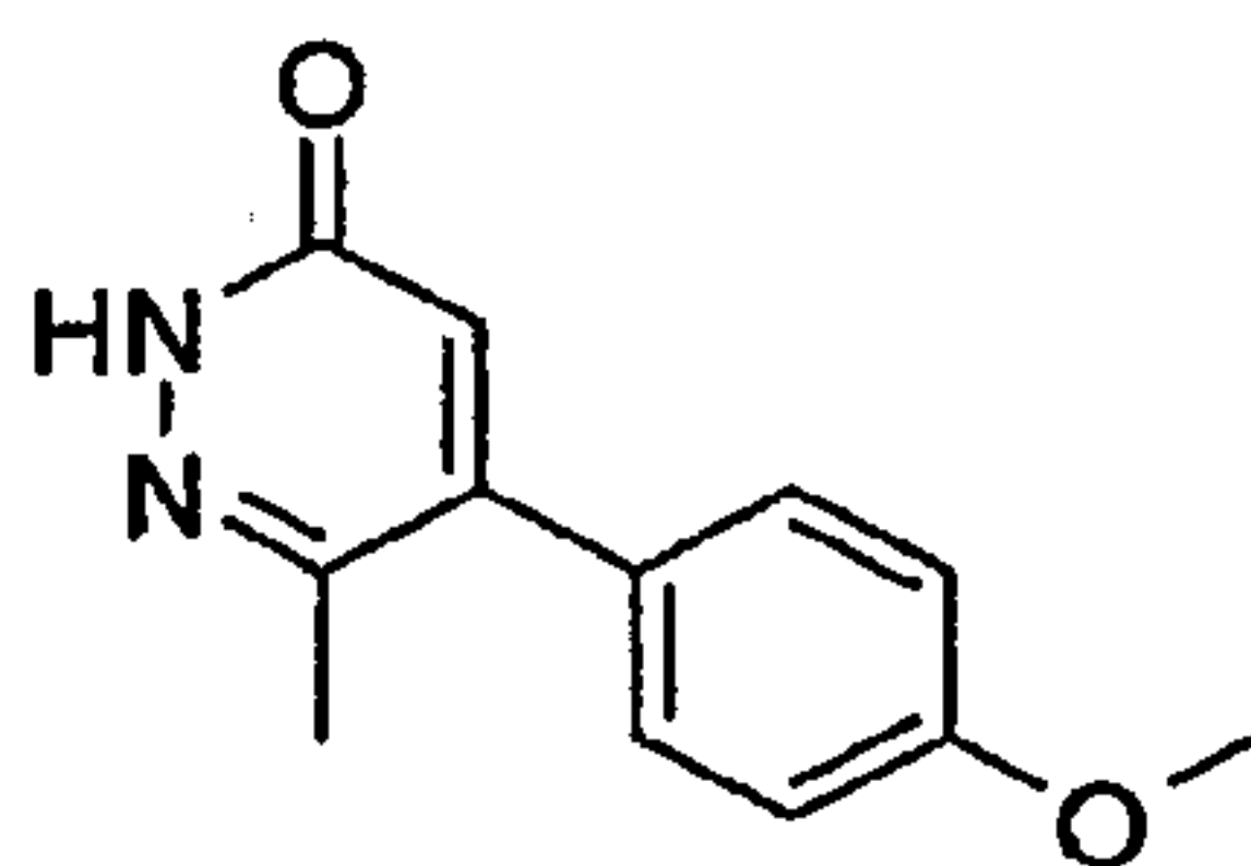
5-(4-Methoxy-phenyl)-6-methyl-2H-pyridazin-3-one
