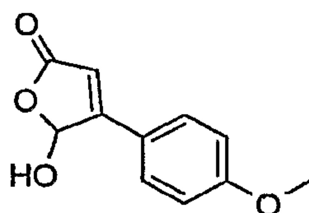
5-Hydroxy-4-(4-methoxy-phenyl)-5H-furan-2-one
