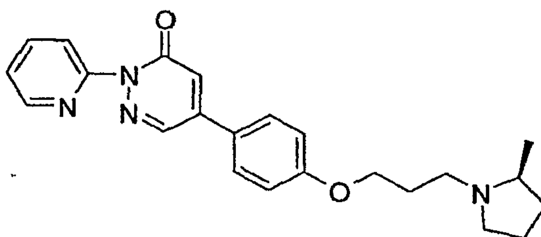
5-{4-[3-((S)-2-Methyl-pyrrolidin-1-yl)-propoxy]-phenyl}-2-pyridin-2-yl-2H-pyridazin-3-one
