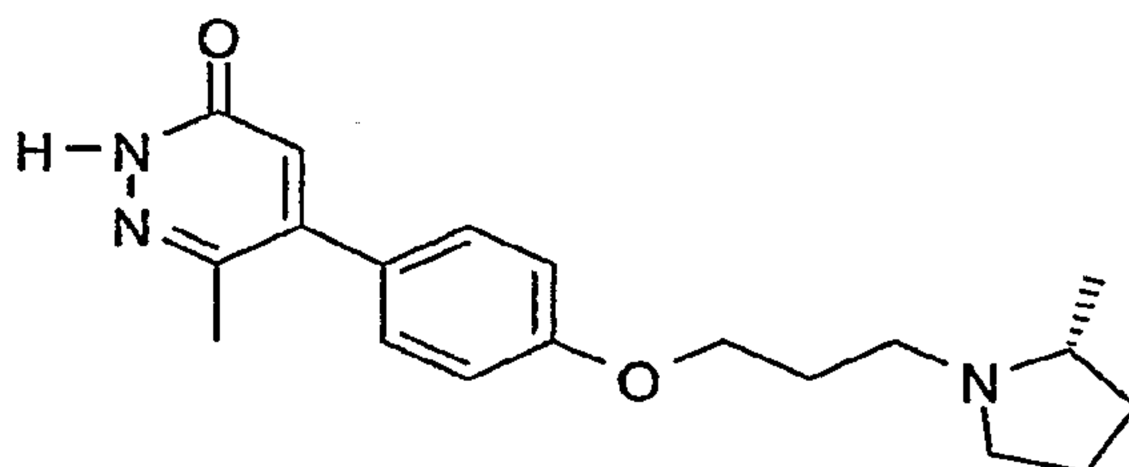
6-Methyl-5-{4-[3-((R)-2-methyl-pyrrolidin-1-yl)-propoxy]-phenyl}-2H-pyridazin-3-one
