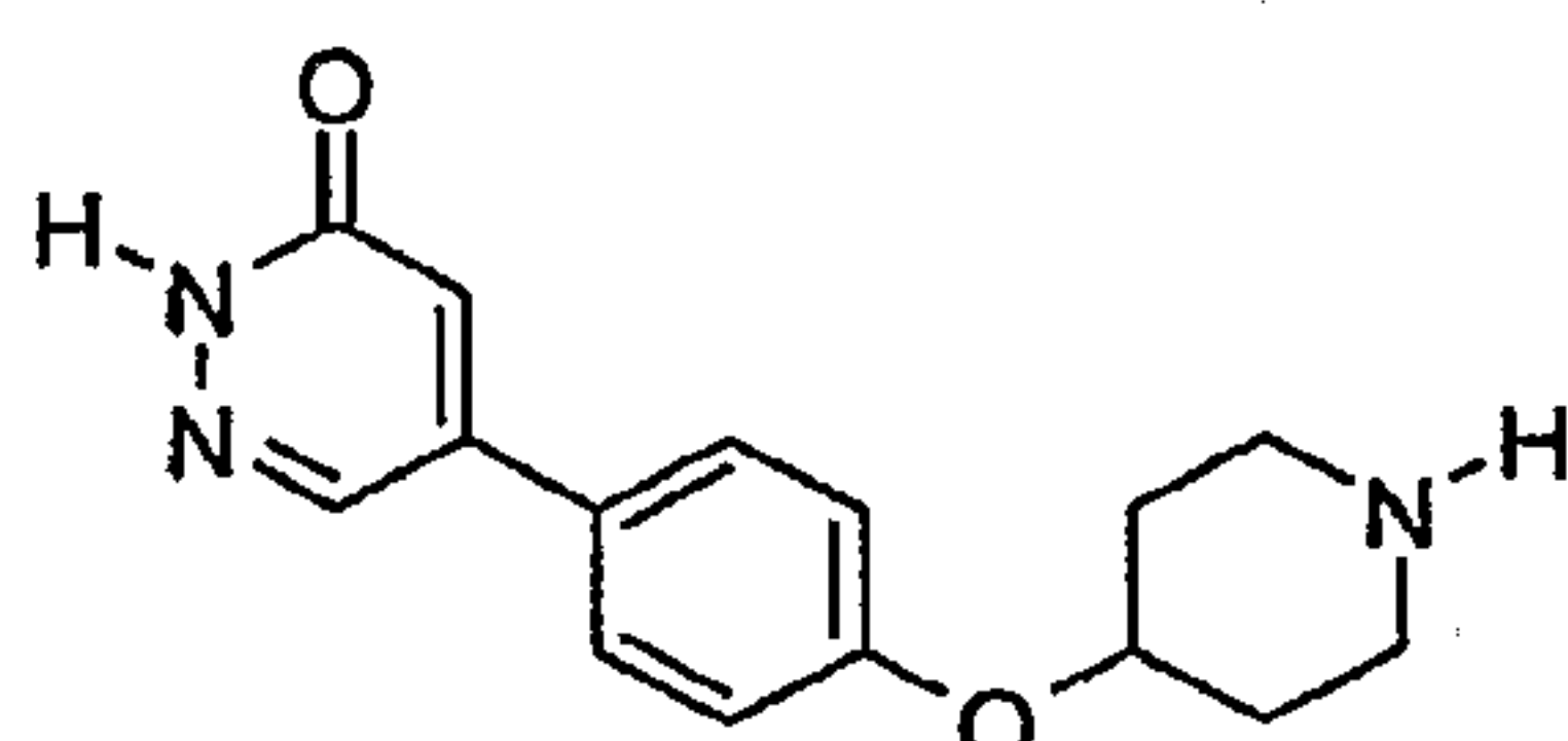
5-[4-(Piperidin-4-yloxy)-phenyl]-2H-pyridazin-3-one
