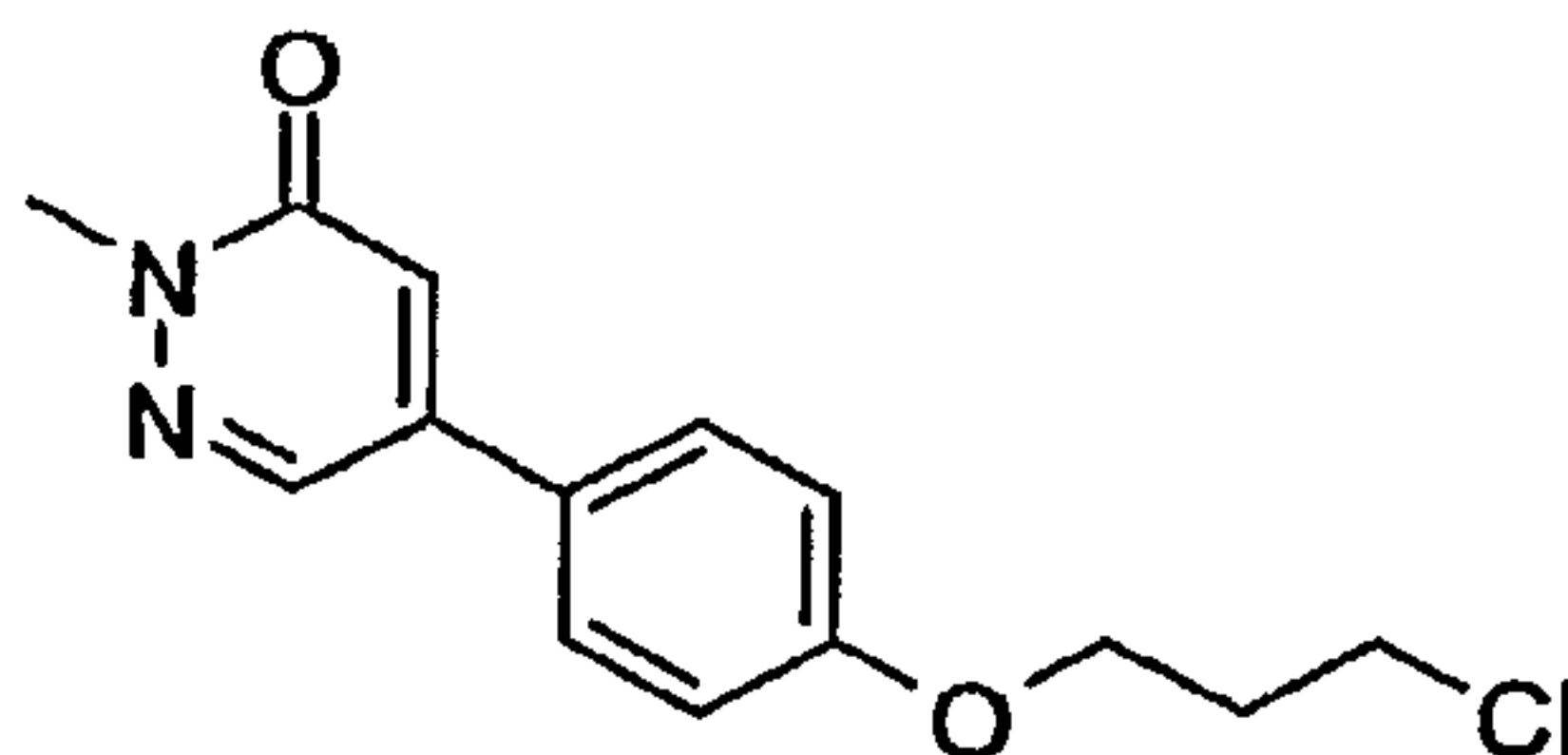
5-[4-(3-Chloro-propoxy)-phenyl]-2-methyl-2H-pyridazin-3-one
