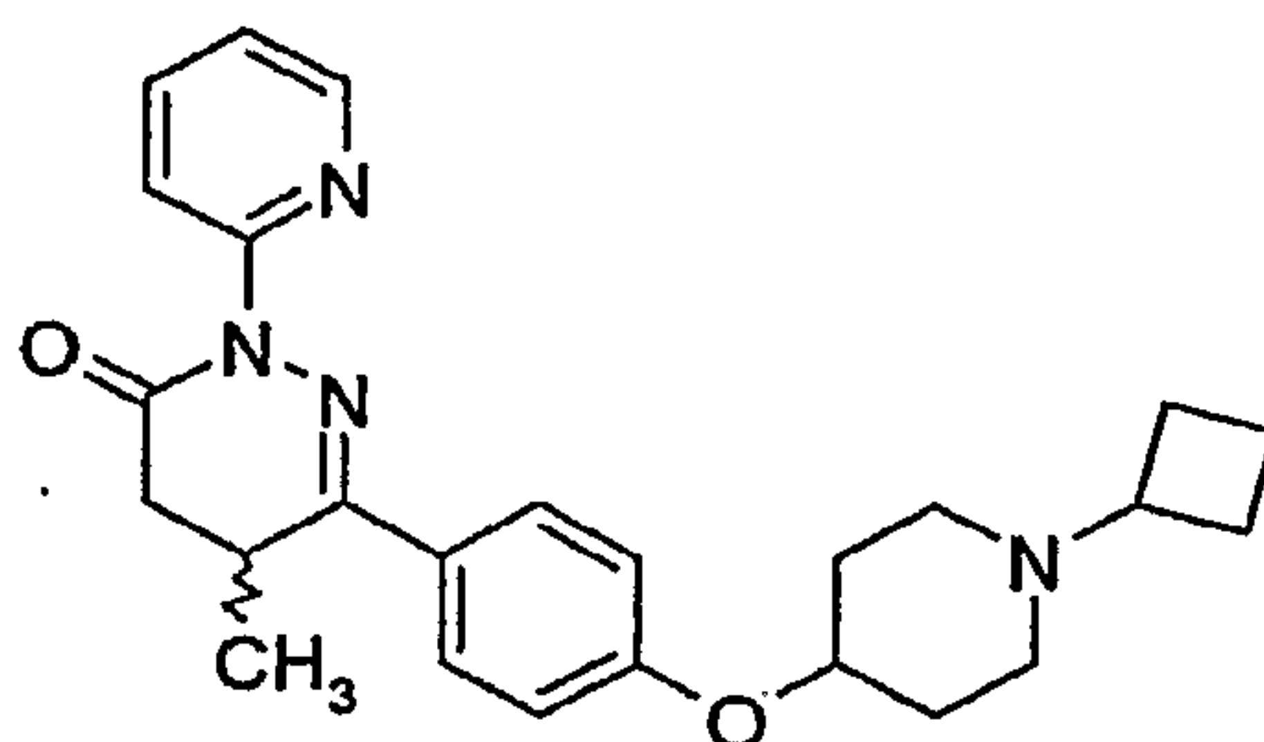
6-[4-(1-Cyclobutyl-piperidin-4-yloxy)-phenyl]-5-methyl-2-pyridin-2-yl-4,5-dihydro-2H-pyridazin-3-one
