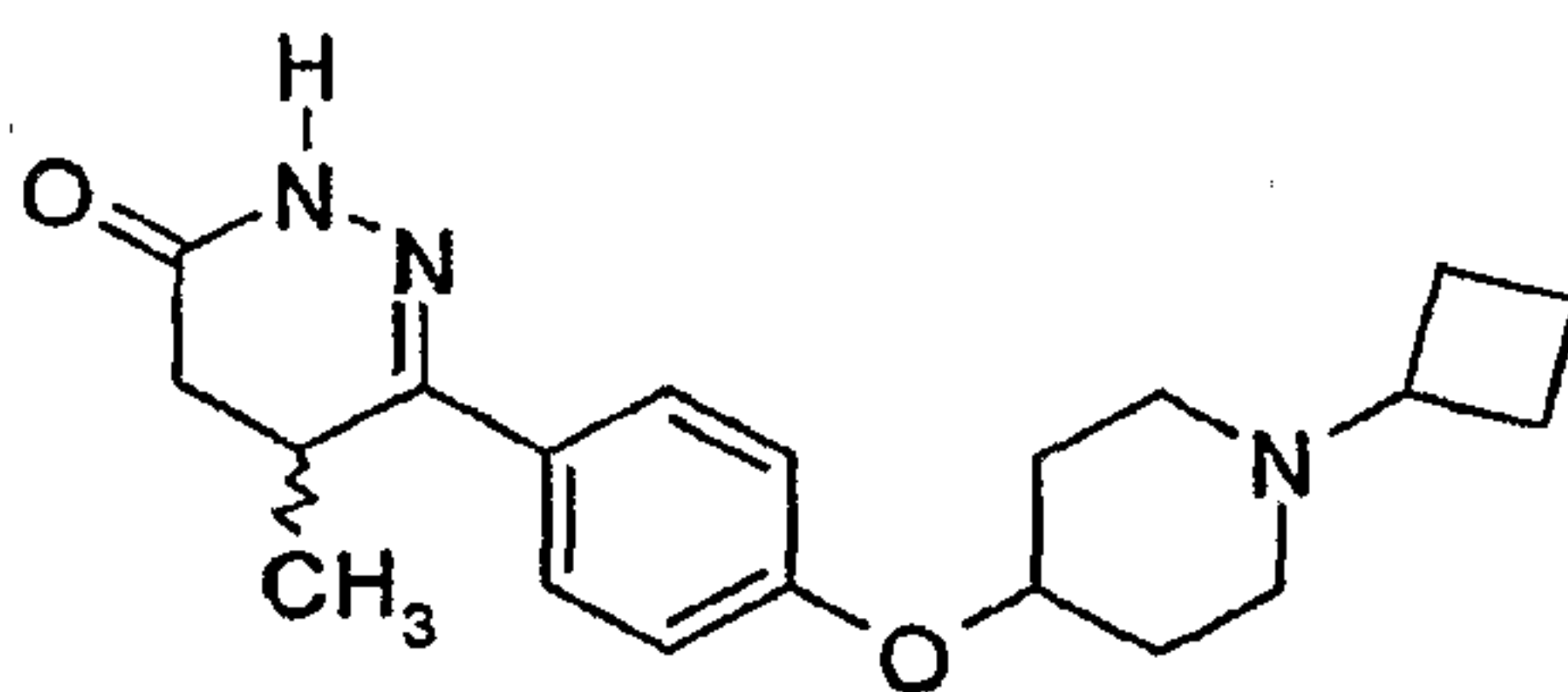
6-[4-(1-Cyclobutyl-piperidin-4-yloxy)-phenyl]-5-methyl-4,5-dihydro-2H-pyridazin-3-one
