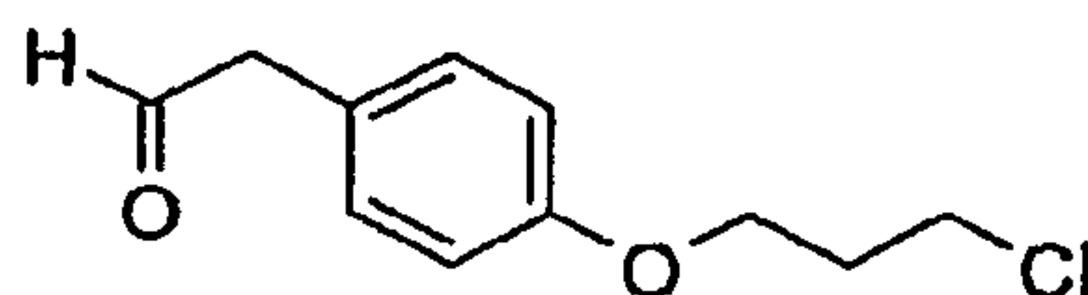
[4-(3-Chloro-propoxy)-phenyl]-acetaldehyde
