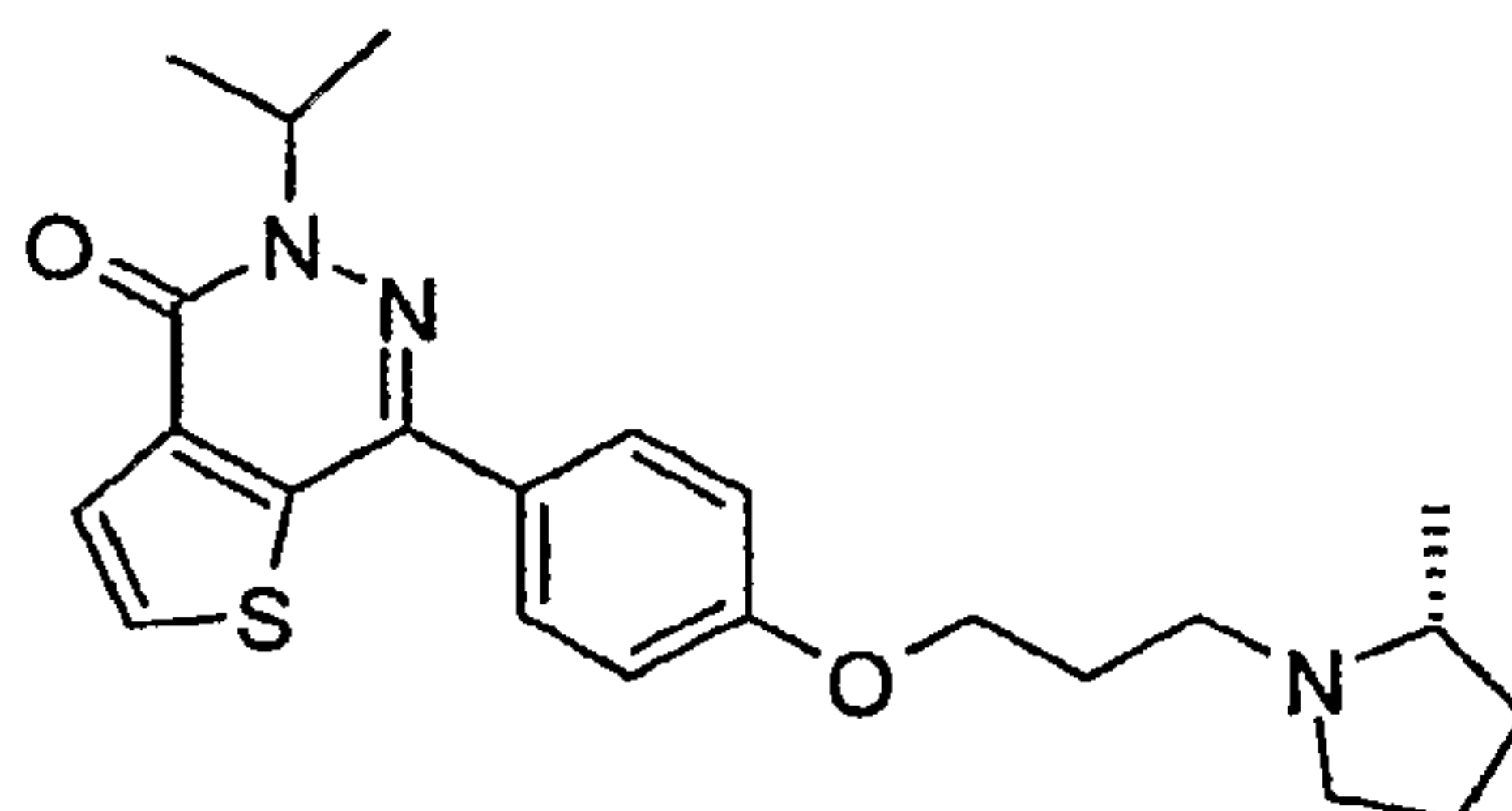
5-Isopropyl-7-{4-[3-((R)-2-methyl-pyrrolidin-1-yl)-propoxy]-phenyl}-5H-thieno[2,3-d]pyridazin-4-one
