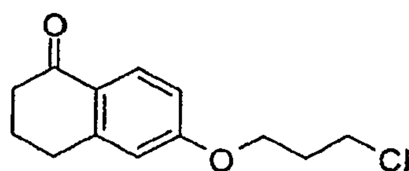
6-(3-Chloro-propoxy)-3,4-dihydro-2H-naphthalen-1-one
