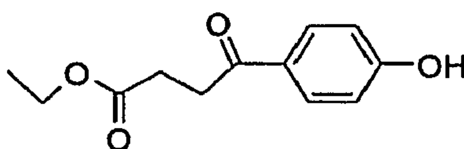
4-(4-Hydroxy-phenyl)-4-oxo-butyric acid ethyl ester
