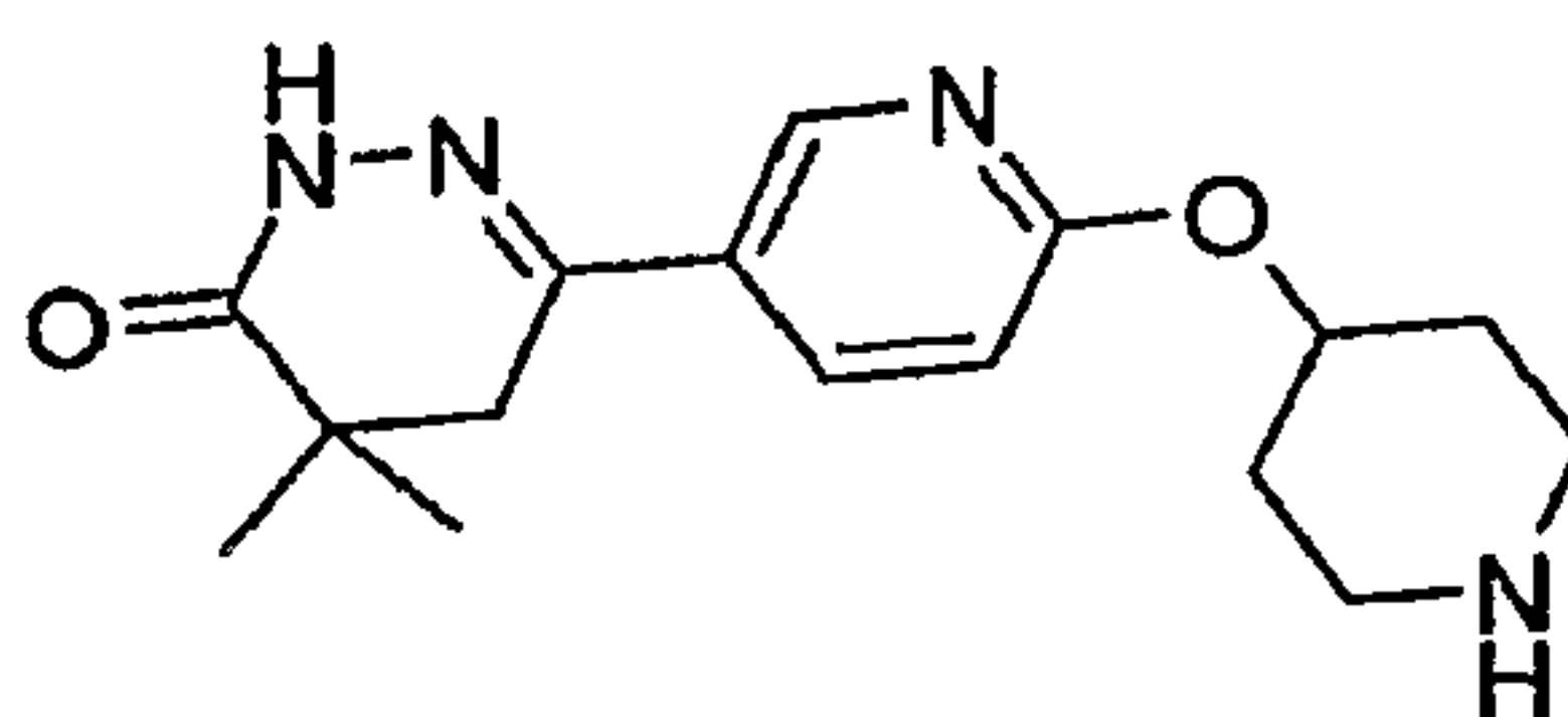
4,4-Dimethyl-6-[6-(piperidin-4-yloxy)-pyridin-3-yl]-4,5-dihydro-2H-pyridazin-3-one
