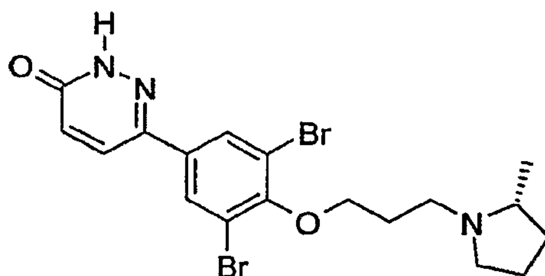
6-{3,5-Dibromo-4-[3-(( R )-2-methyl-pyrrolidin-1-yl)-propoxy]-phenyl}-2H-pyridazin-3-one
