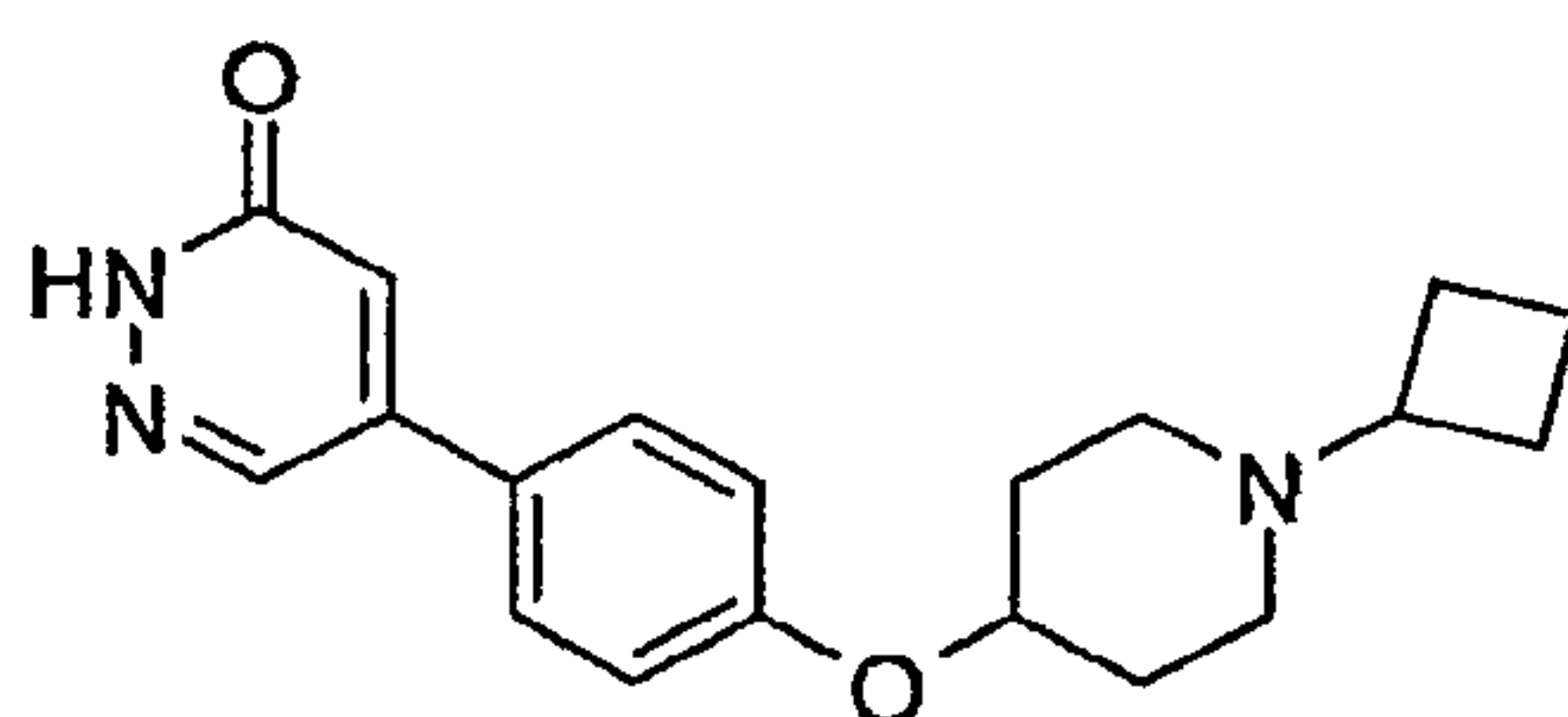
5-[4-(1-Cyclobutyl-piperidin-4-yloxy)-phenyl]-2H-pyridazin-3-one
