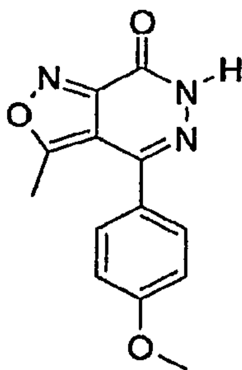
4-(4-Methoxyphenyl)-3-methyl-6H-isoxazolo[3,4-d]pyridazin-7-one
