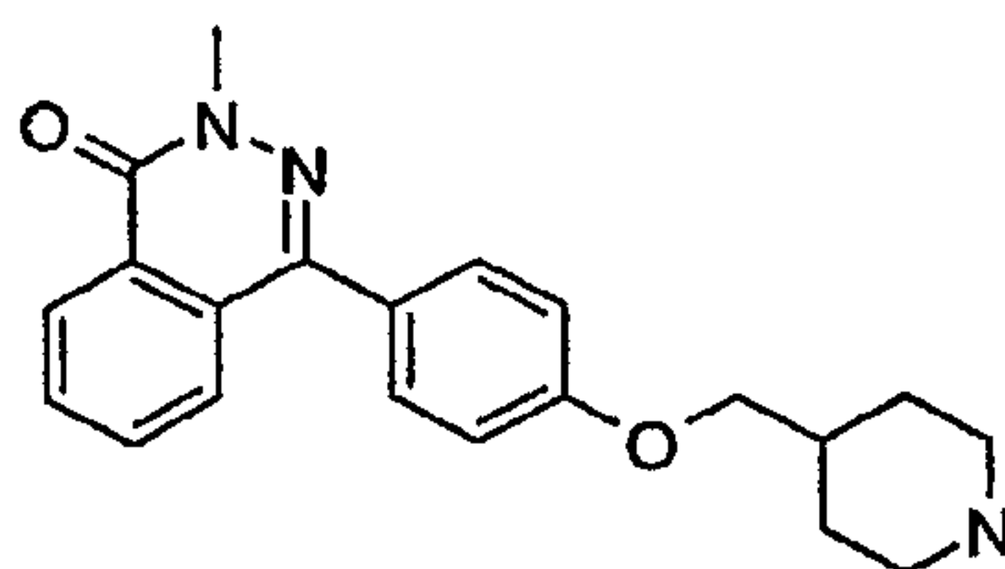
2-Methyl-4-[4-(piperidin-4-ylmethoxy)-phenyl]-2H-phthalazin-1-one
