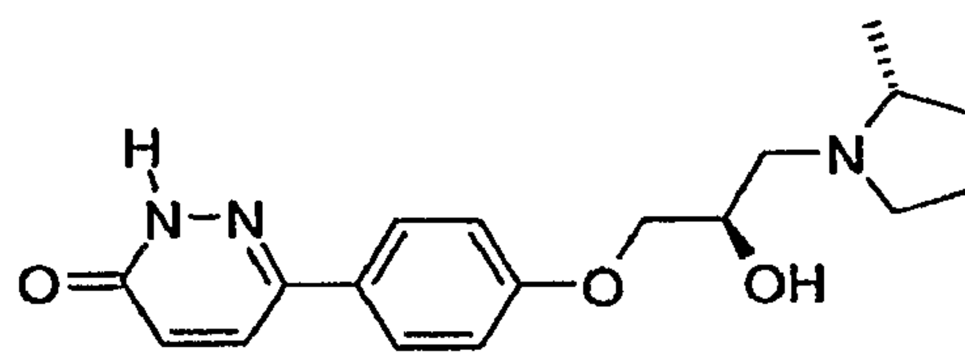
6-{4-[(R)-2-Hydroxy-3-((R)-2-methyl-pyrrolidin-1-yl)-propoxy]-phenyl}-2H-pyridazin-3-one
