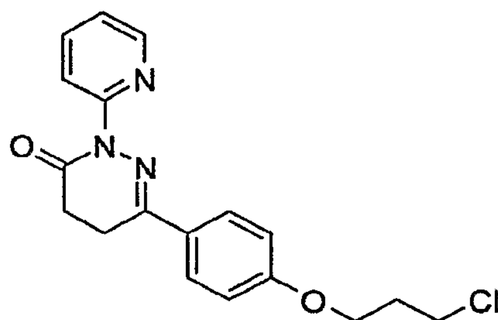
6-[4-(3-Chloropropoxy)-phenyl]-2-pyridin-2-yl-4,5-dihydro-2H-pyridazin-3-one
