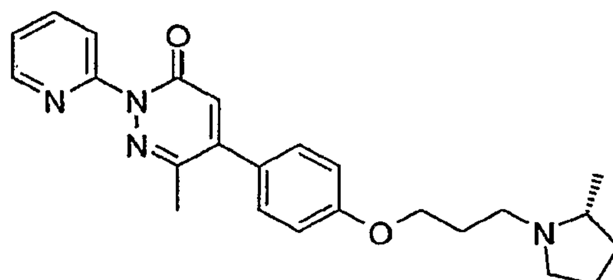
6-Methyl-5-{4-[3-((R)-2-methyl-pyrrolidin-1-yl)-propoxy]-phenyl}-2-pyridin-2-yl-2H-pyridazin-3-one
