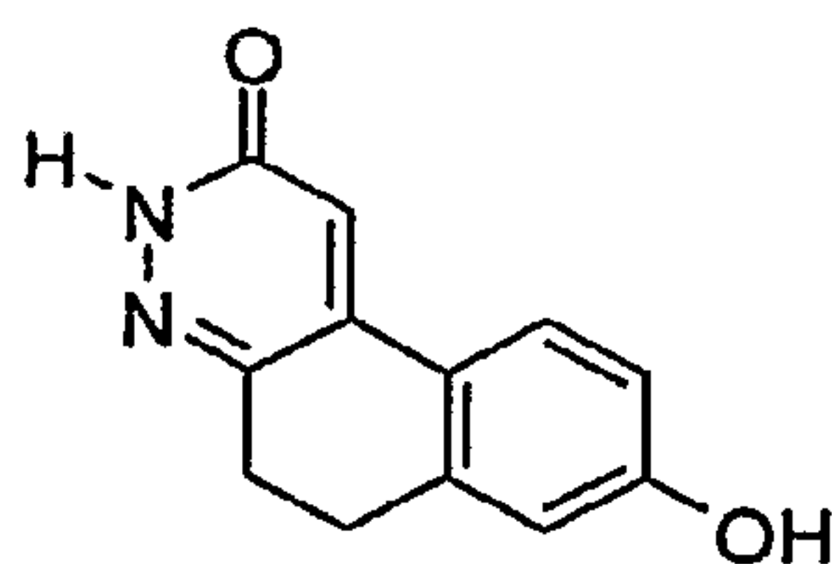
8-Hydroxy-5,6-dihydro-3H-benzo[f]cinnolin-2-one
