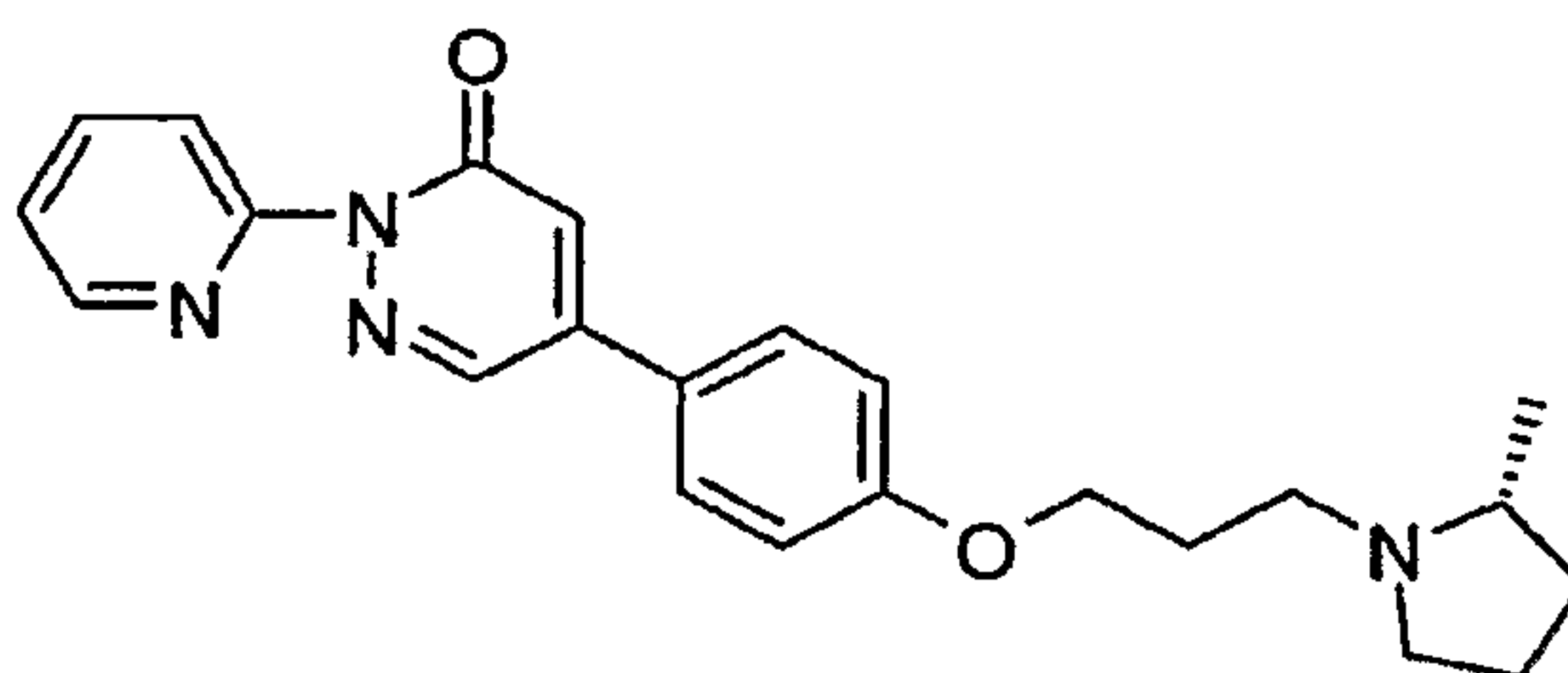
5-{4-[3-((R)-2-Methyl-pyrrolidin-1-yl)-propoxy]-phenyl}-2-pyridin-2-yl-2H-pyridazin-3-one
