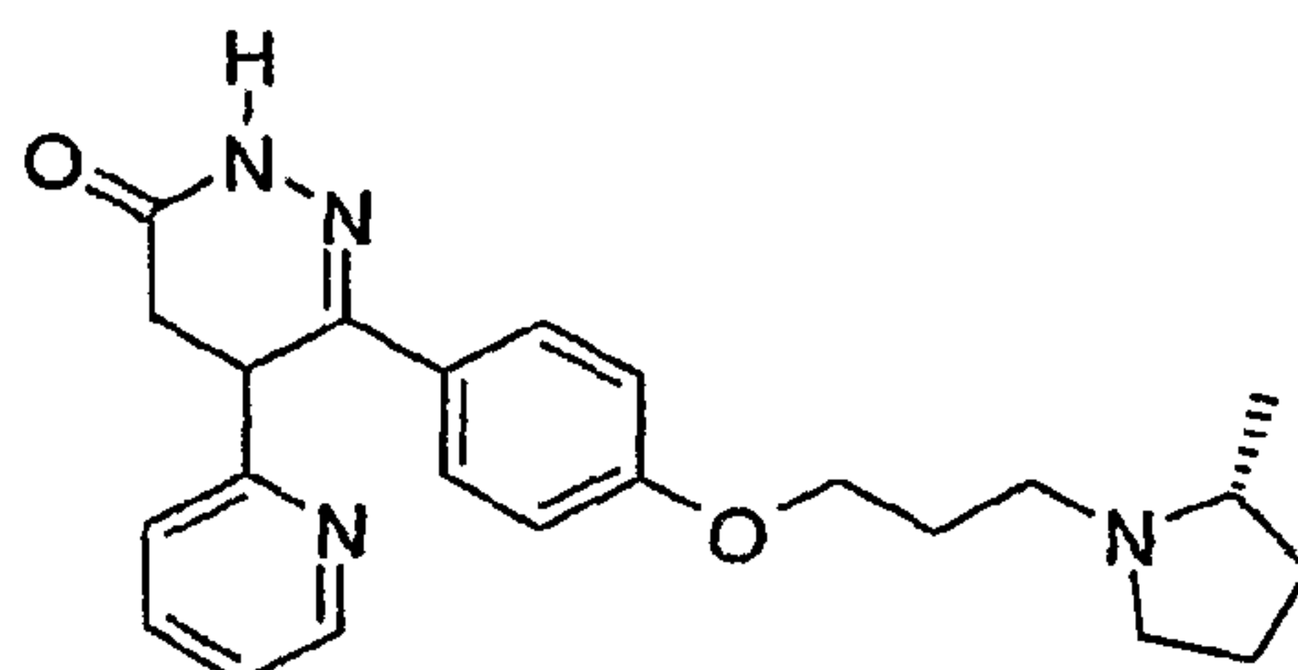
6-{4-[3-((R)-2-Methyl-pyrrolidin-1-yl)-propoxy]-phenyl}-5-pyridin-2-yl-4,5-dihydro-2H-pyridazin-3-one
