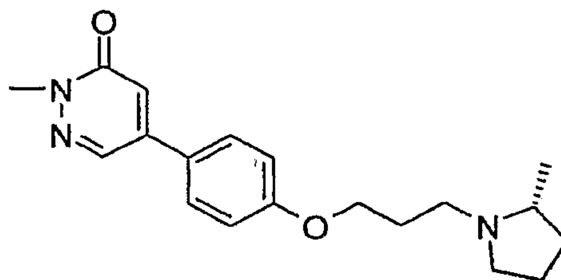
2-Methyl-5-{4-[3-((R)-2-methyl-pyrrolidin-1-yl)-propoxy]-phenyl}-2H-pyridazin-3-one
