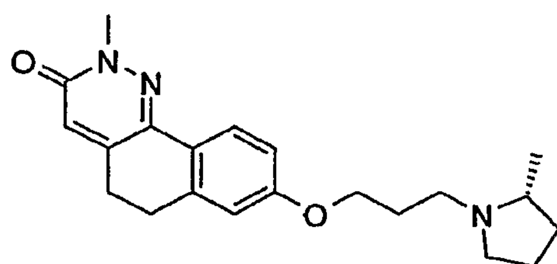
2-Methyl-8-[3-((R)-2-methyl-pyrrolidin-1-yl)-propoxy]-5,6-dihydro-2H-benzo[h]cinnolin-3-one
