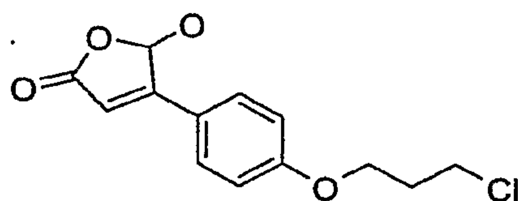
4-[4-(3-Chloro-propoxy)-phenyl]-5-hydroxy-5H-furan-2-one
