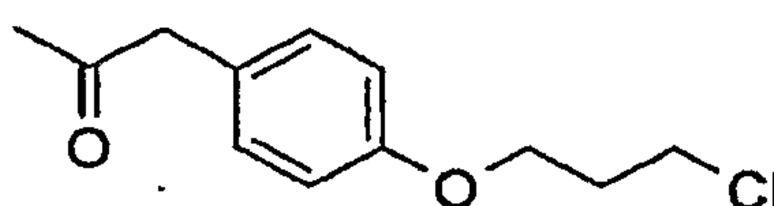
1-[4-(3-Chloropropoxy)-phenyl]-propan-2-one
