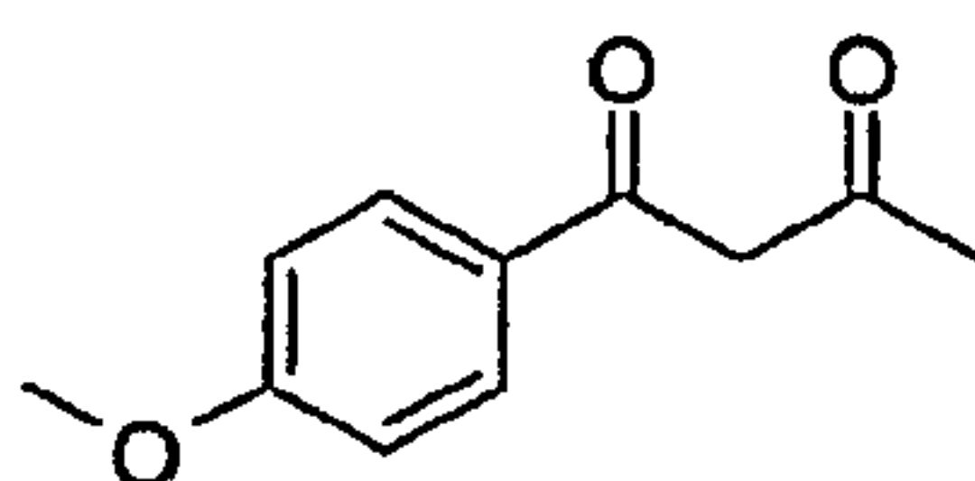
1-(4-Methoxy-phenyl)-butane-1,3-dione
