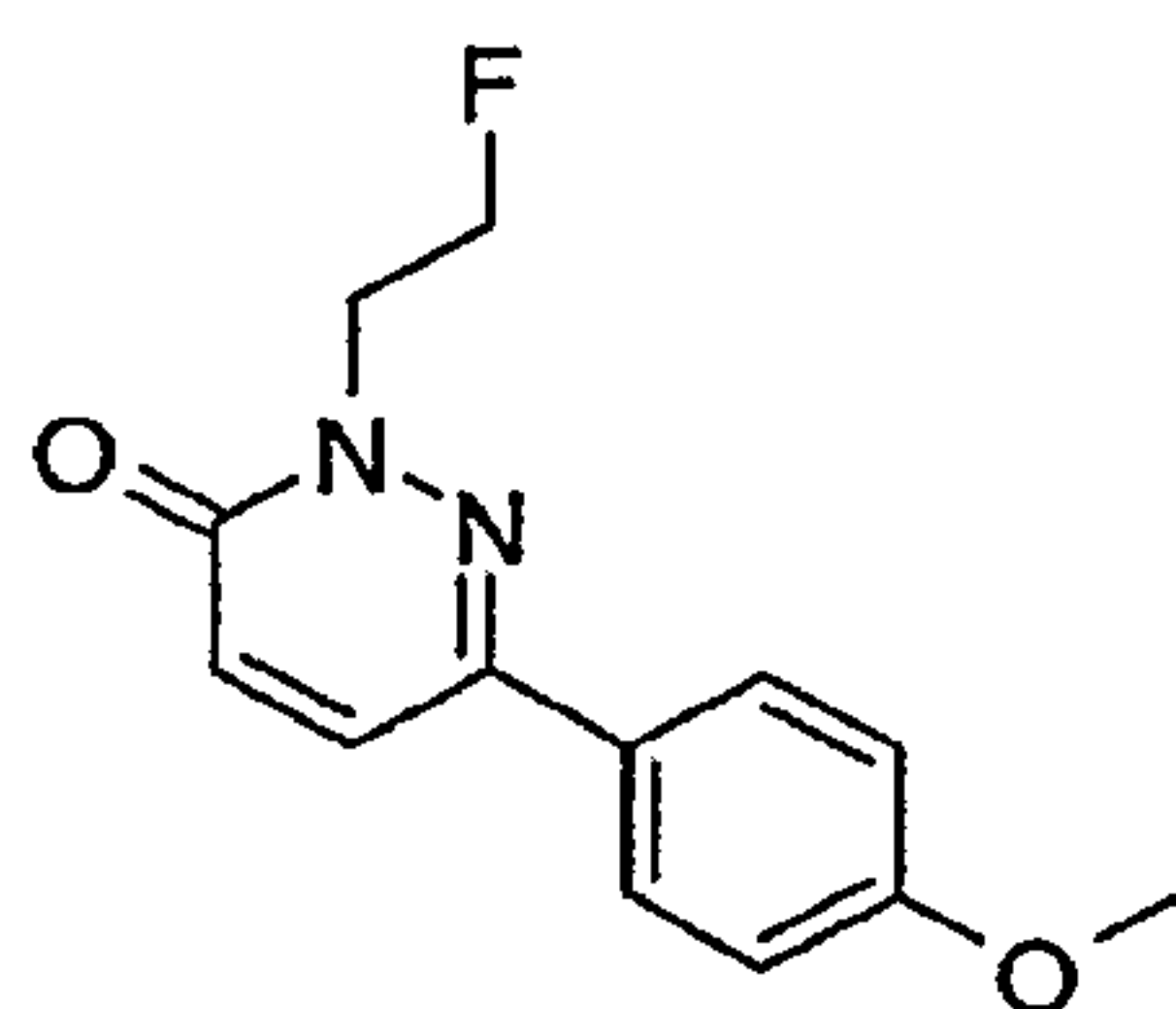
2-(2-Fluoro-ethyl)-6-(4-methoxy-phenyl)-2H-pyridazin-3-one
