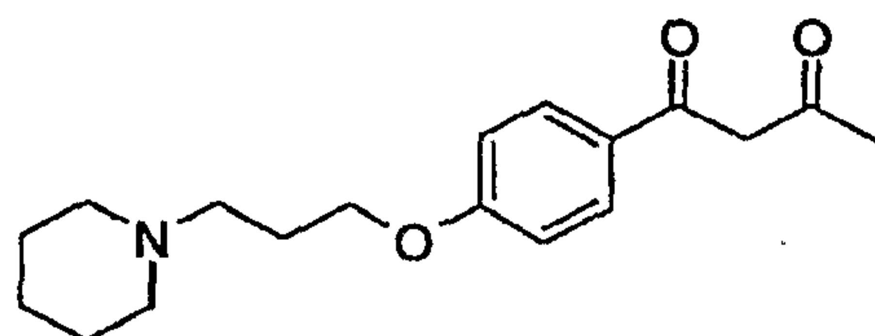
1-[4-(3-Piperidin-1-yl-propoxy)-phenyl]-butane-1,3-dione
