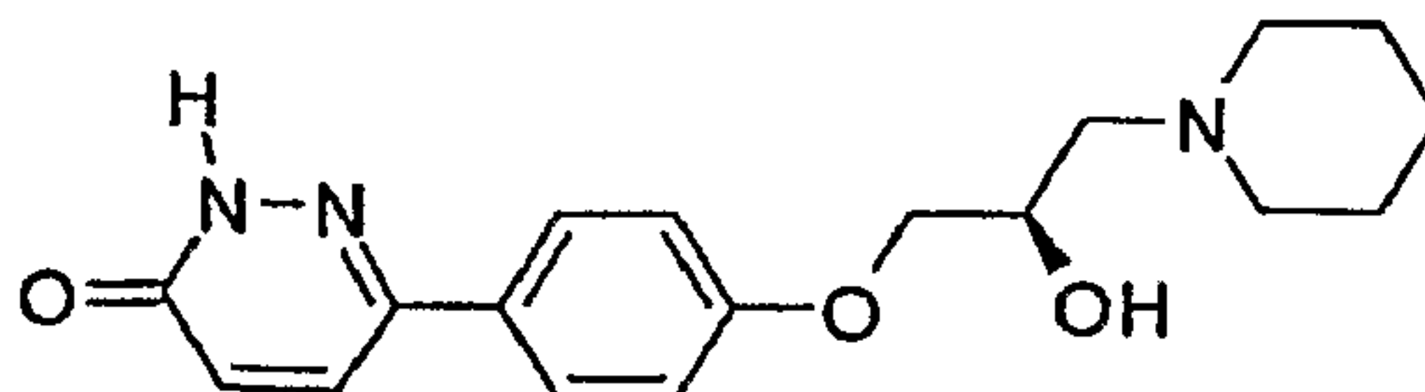
6-[4-((R)-2-Hydroxy-3-piperidin-1-yl-propoxy)-phenyl]-2H-pyridazin-3-one
