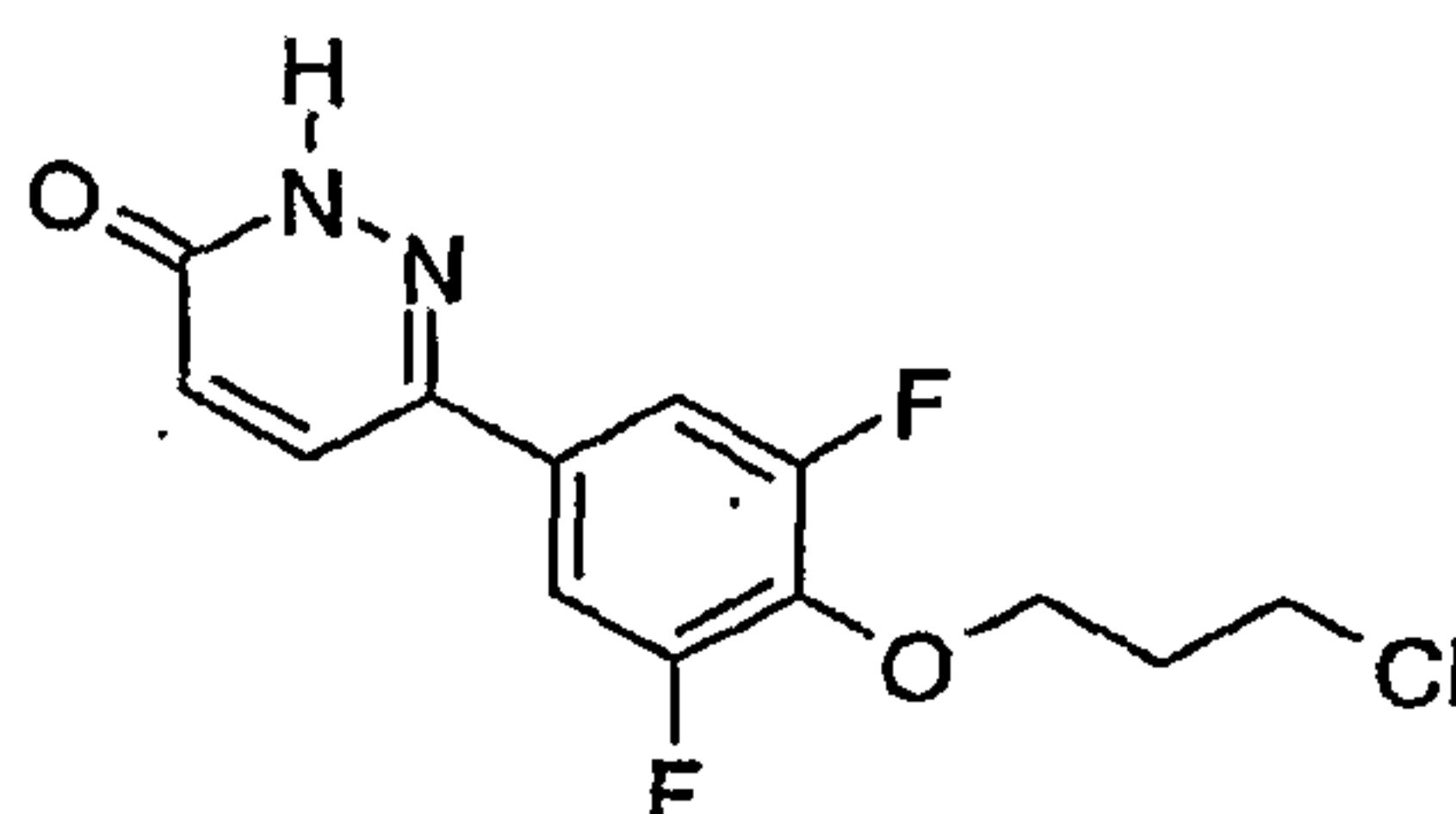
6-[4-(3-Chloro-propoxy)-3,5-difluorophenyl]-2H-pyridazin-3-one
