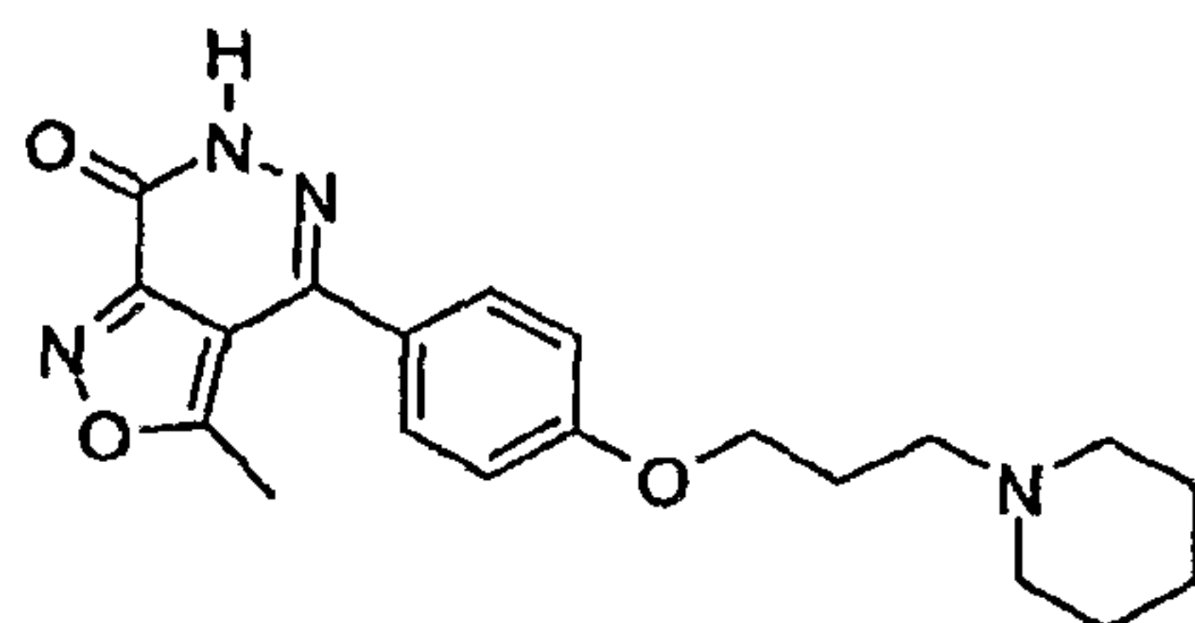
3-Methyl-4-[4-(3-piperidin-1-yl-propoxy)-phenyl]-6H-isoxazolo[3,4-d]pyridazin-7-one
