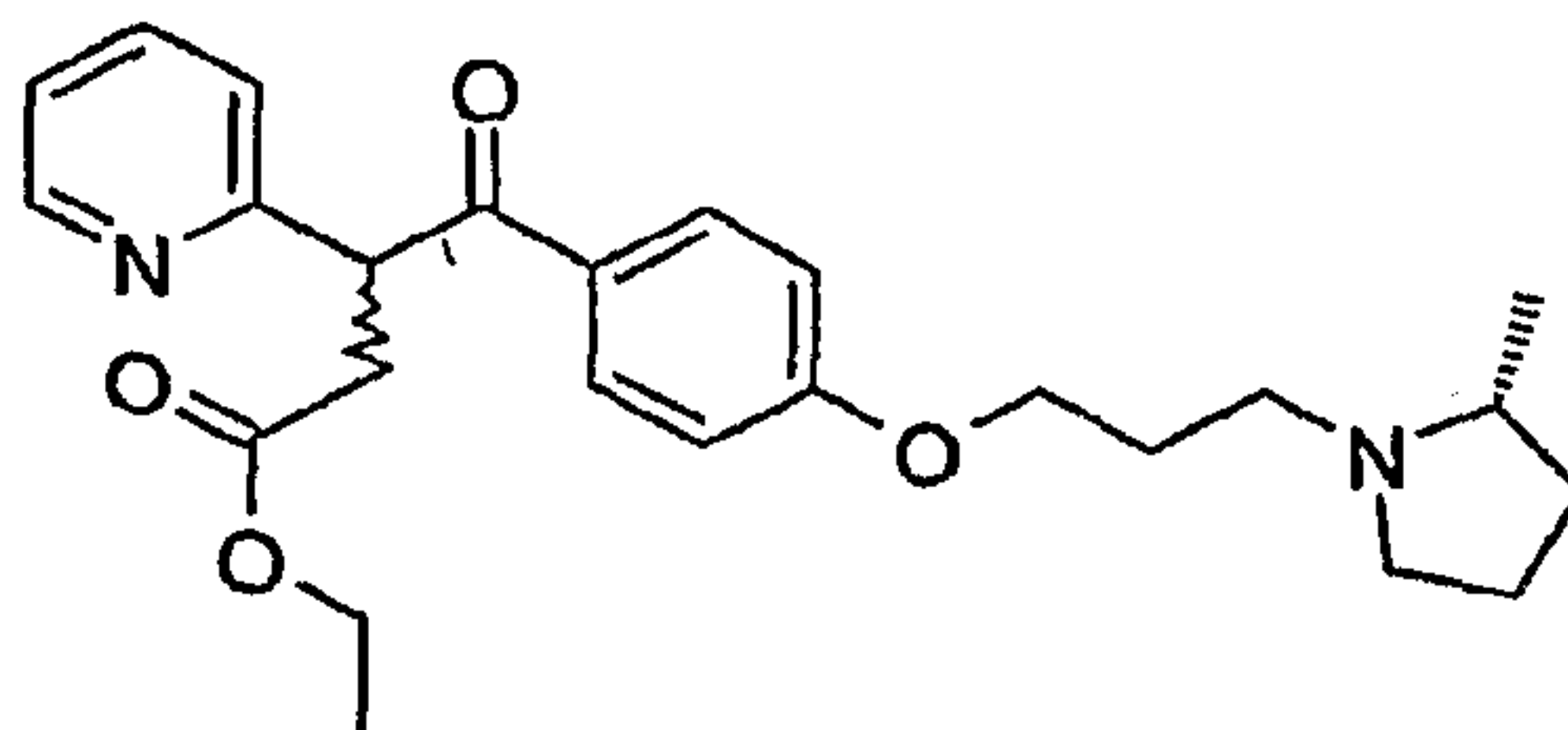
4-{4-[3-((R)-2-Methyl-pyrrolidin-1-yl)-propoxy]-phenyl}-4-oxo-3-pyridin-2-yl-butyrac acid ethyl ester
