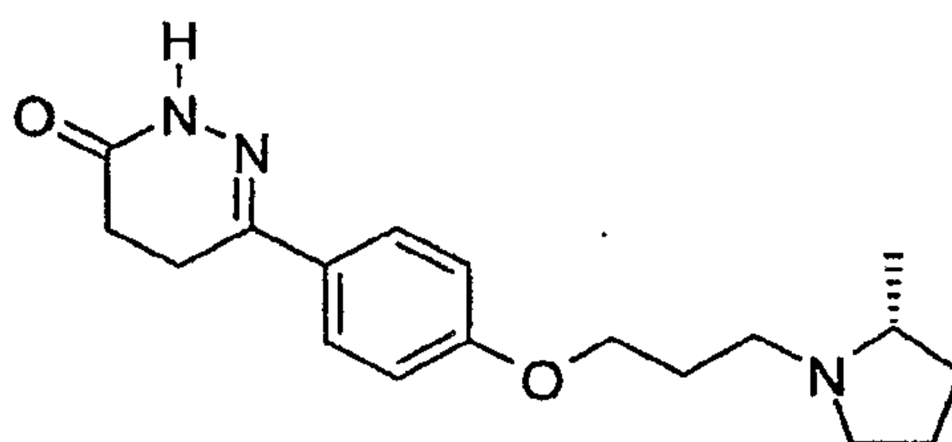
6-{4-[3-((R)-2-Methyl-pyrrolidin-1-yl)-propoxy]-phenyl}-4,5-dihydro-2H-pyridazin-3-one
