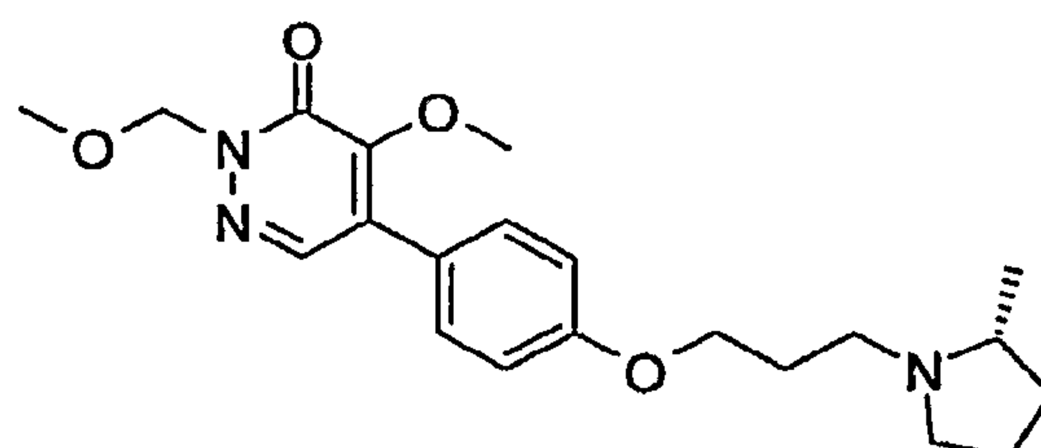
4-Methoxy-2-methoxymethyl-5-{4-[3-(R)-2-methyl-pyrrolidin-1-yl]-propoxy}-phenyl]-2H-pyridazin-3-one
