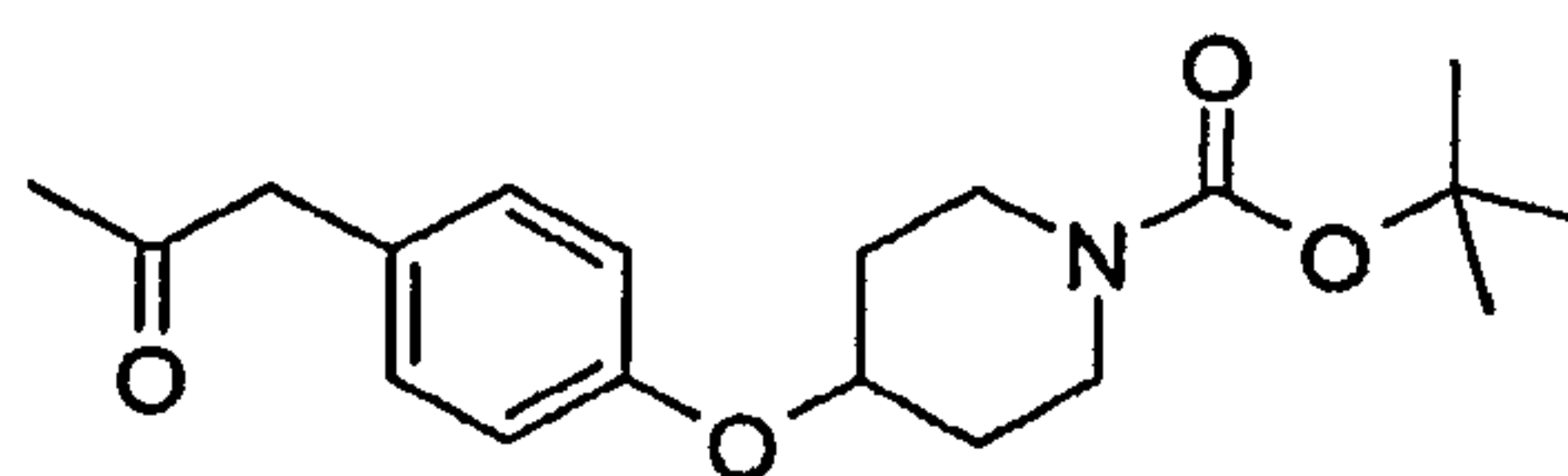
4-[4-(2-Oxo-propyl)-phenoxy]-piperidine-1-carboxylic acid tert-butyl ester
