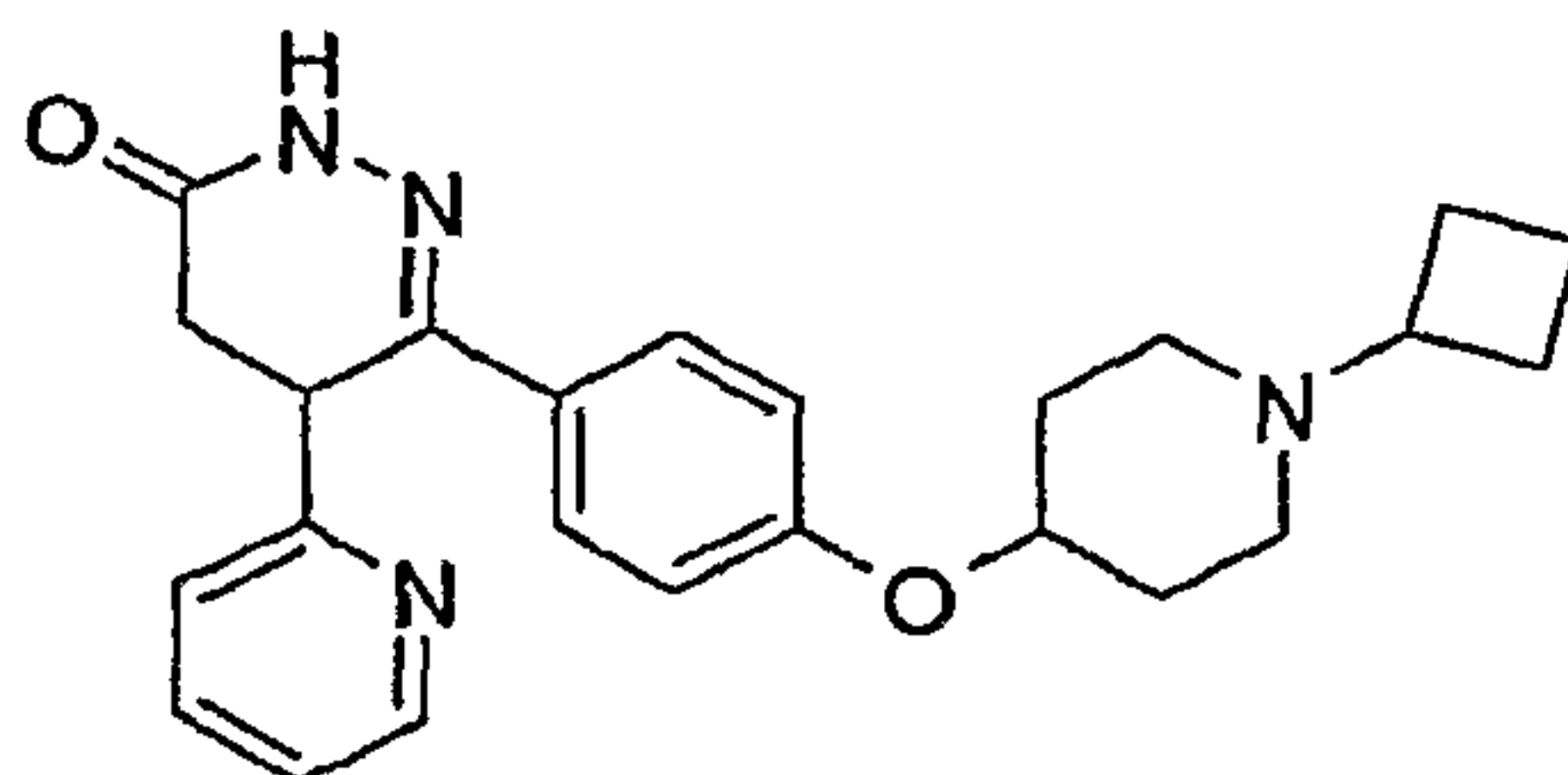
6-[4-(1-Cyclobutyl-piperidin-4-yloxy)-phenyl]-5-pyridin-2-yl-4,5-dihydro-2H-pyridazin-3-one
