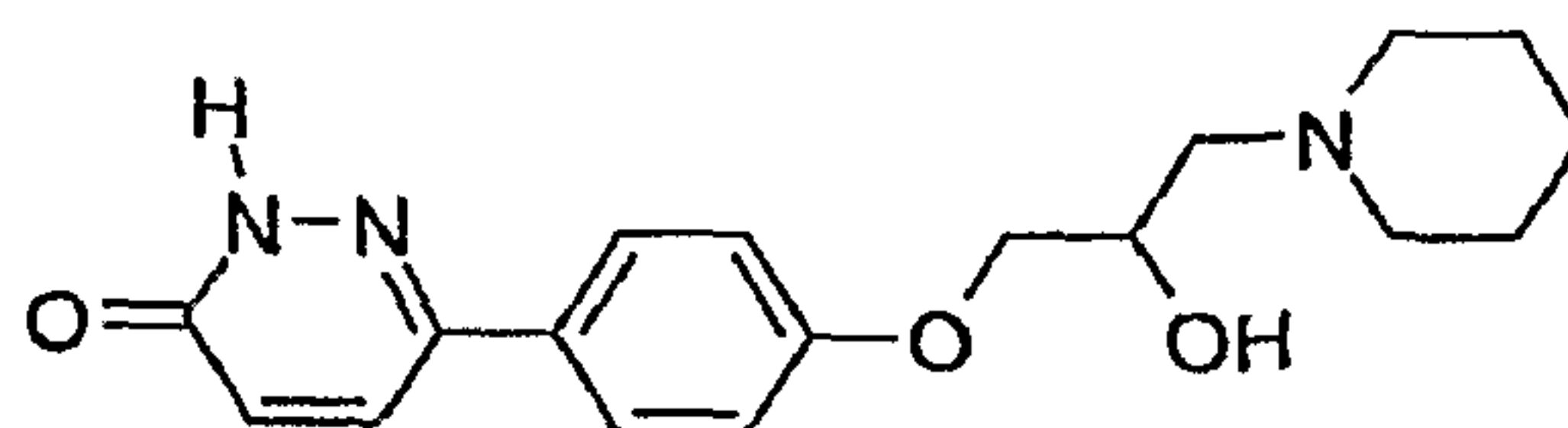
6-[4-(2-Hydroxy-3-piperidin-1-yl-propoxy)-phenyl]-2H-pyridazin-3-one
