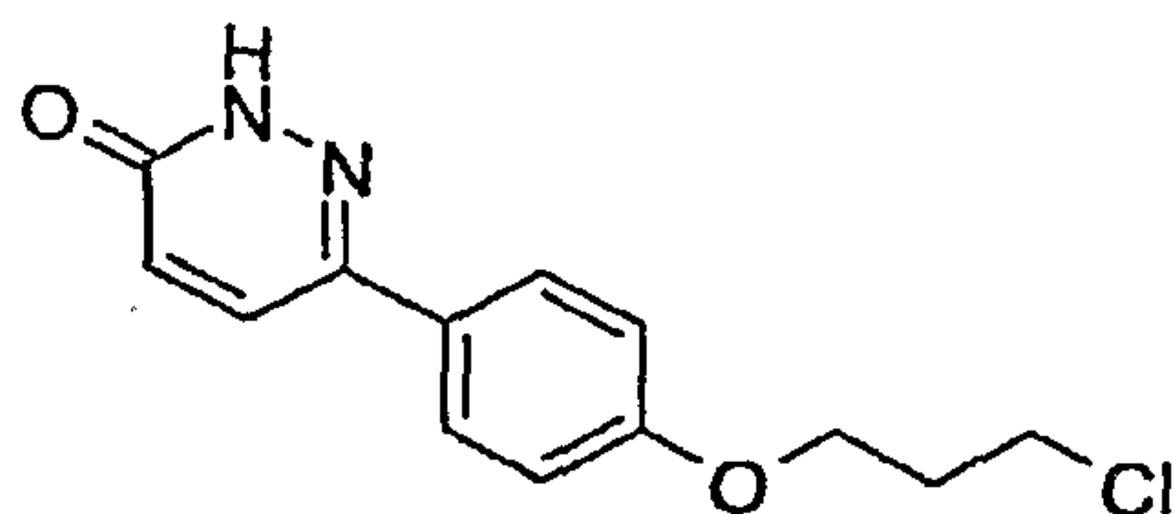
6-[4-(3-Chloro-propoxy)-phenyl]-2H-pyridazin-3-one
