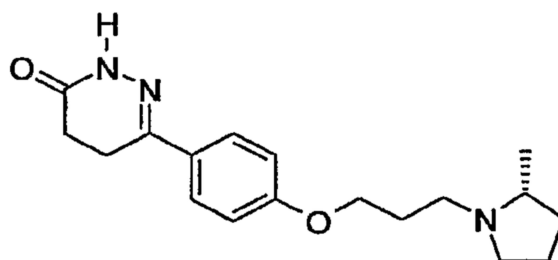
6-{4-[3-((R)-2-Methyl-pyrrolidin-1-yl)-propoxy]-phenyl}-4,5-dihydro-2H-pyridazin-3-one
