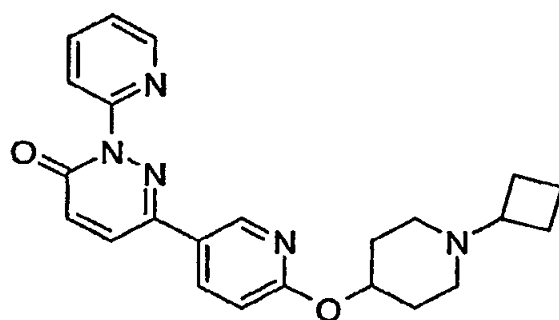
6-[6-(1-Cyclobutyl-piperidin-4-yloxy)-pyridin-3-yl]-2-pyridin-2-yl-2H-pyridazin-3-one
