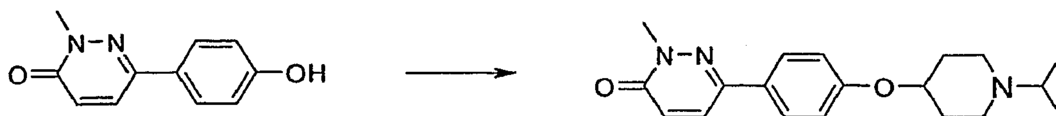
6-(4-Hydroxy-phenyl)-2-methyl-2H-pyridazin-3-one
