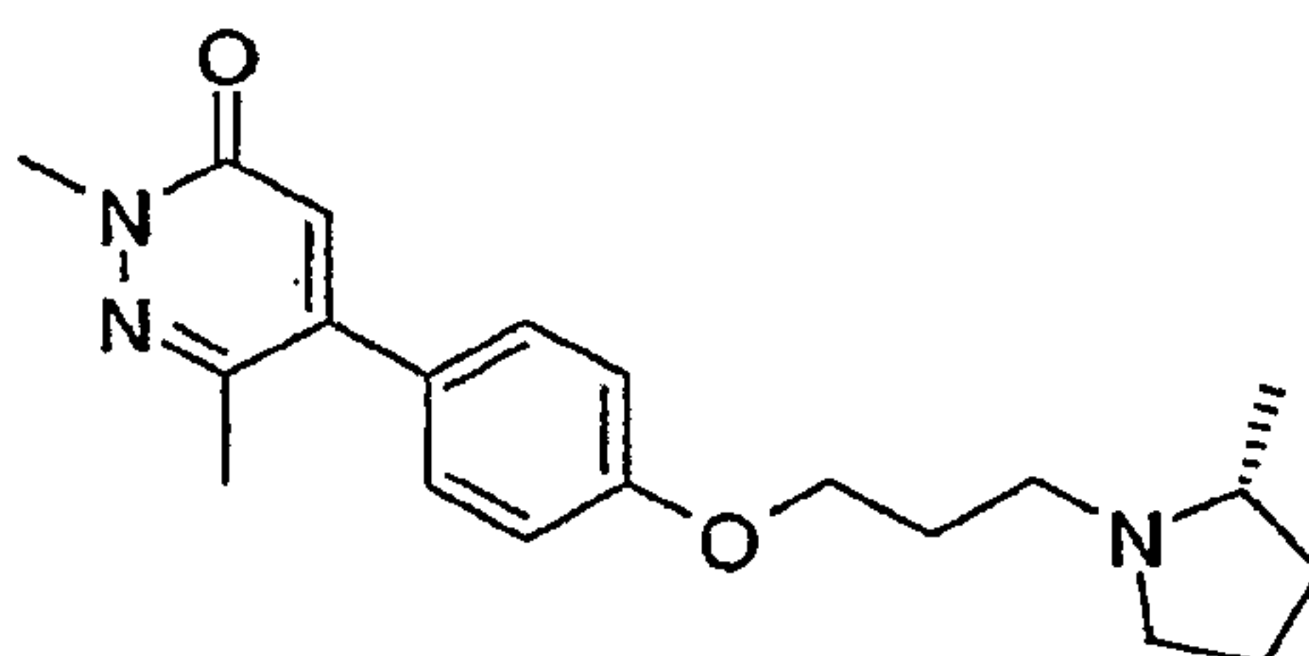
2,6-Dimethyl-5-{4-[3-((R)-2-methylpyrrolidin-1-yl)-propoxy]-phenyl}-2H-pyridazin-3-one
