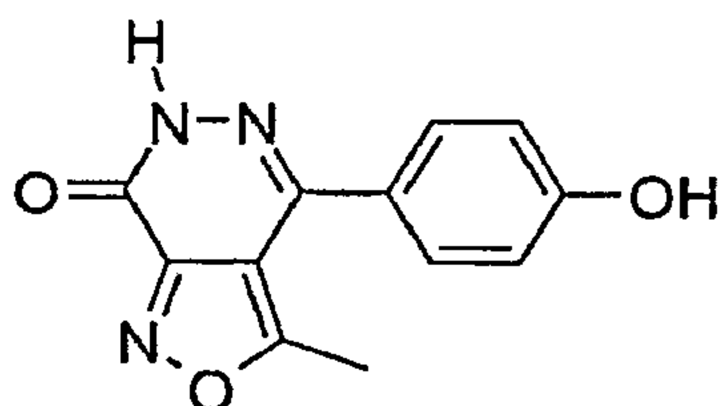
4-(4-Hydroxy-phenyl)-3-methyl-6H-isoxazolo[3,4-d]pyridazin-7-one
