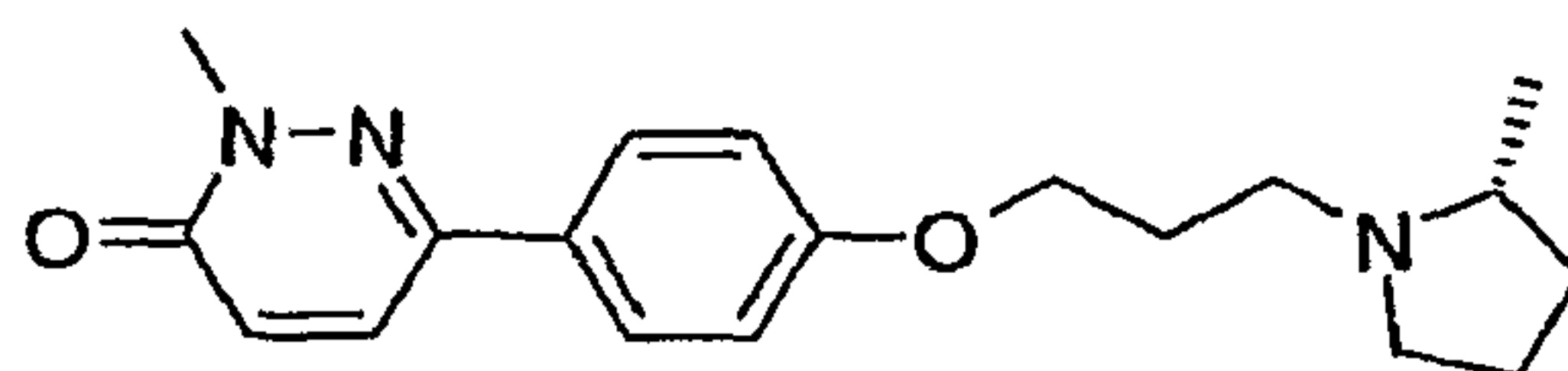
2-Methyl-6-{4-[3-((R)-2-methyl-pyrrolidin-1-yl)-propoxy]-phenyl}-2H-pyridazin-3-one
