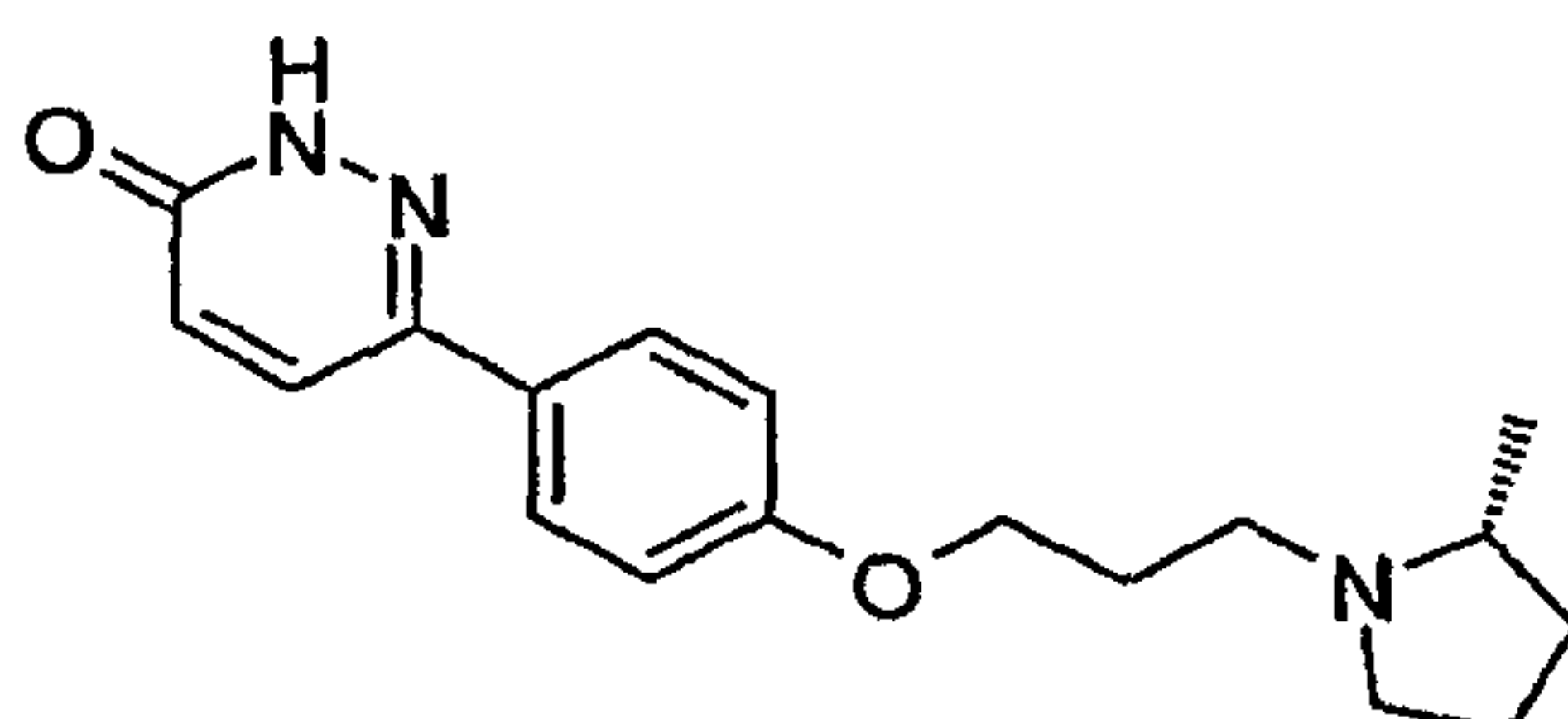
6-{4-[3-((R)-2-Methyl-pyrrolidin-1-yl)-propoxy]-phenyl}-2H-pyridazin-3-one
