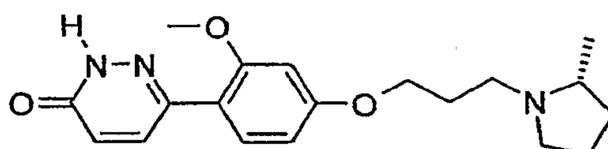
6-{2-Methoxy-4-[3-((R)-2-methyl-pyrrolidin-1-yl)-propoxy]-phenyl}-2H-pyridazin-3-one
