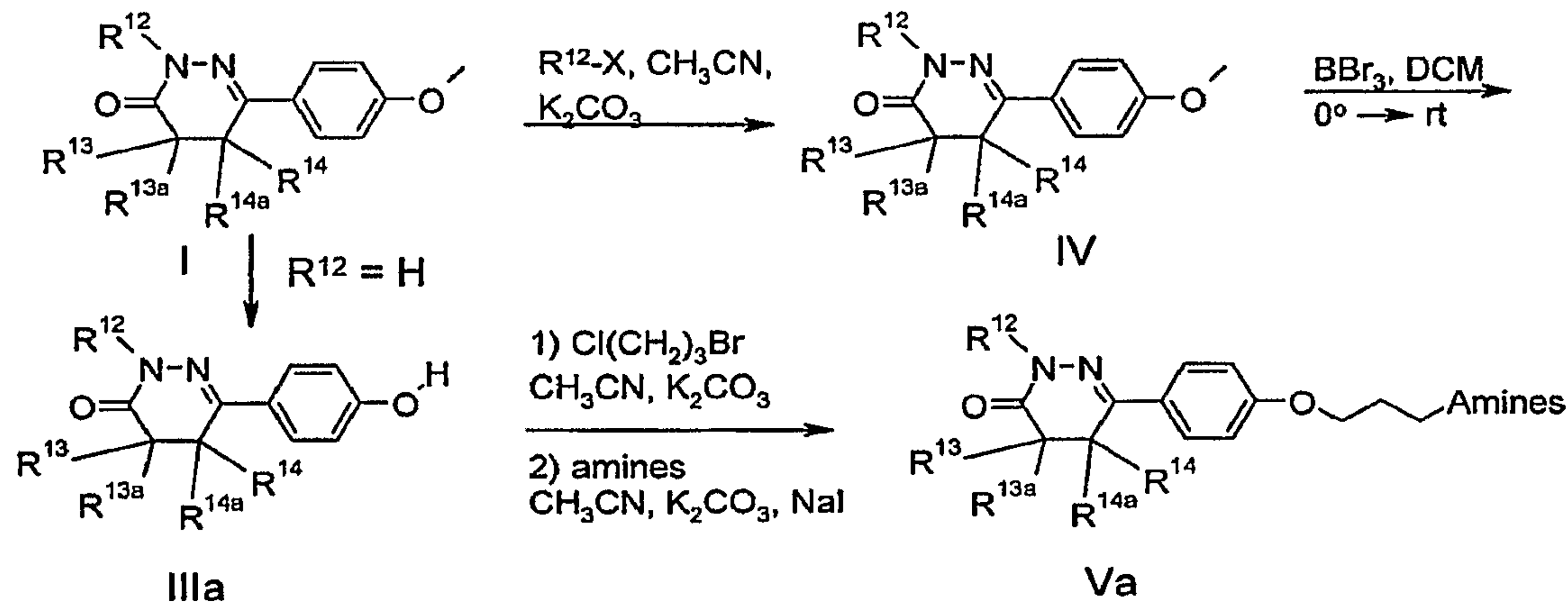
Scheme 4. General synthesis of 4,5-dihydro examples
