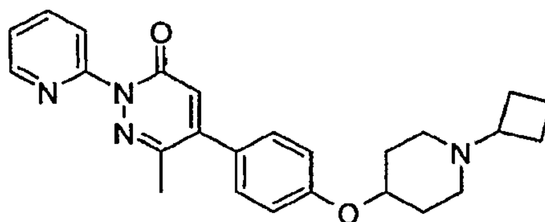
5-[4-(1-Cyclobutyl-piperidin-4-yloxy)-phenyl]-6-methyl-2-pyridin-2-yl-2H-pyridazin-3-one
