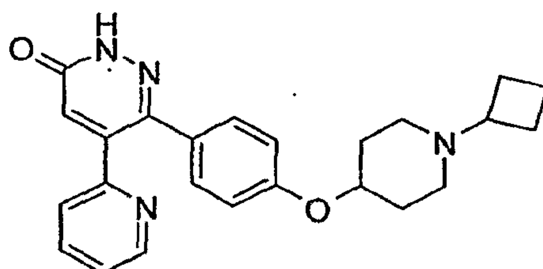
6-[4-(1-Cyclobutyl-piperidin-4-yloxy)-phenyl]-5-pyridin-2-yl-2H-pyridazin-3-one
