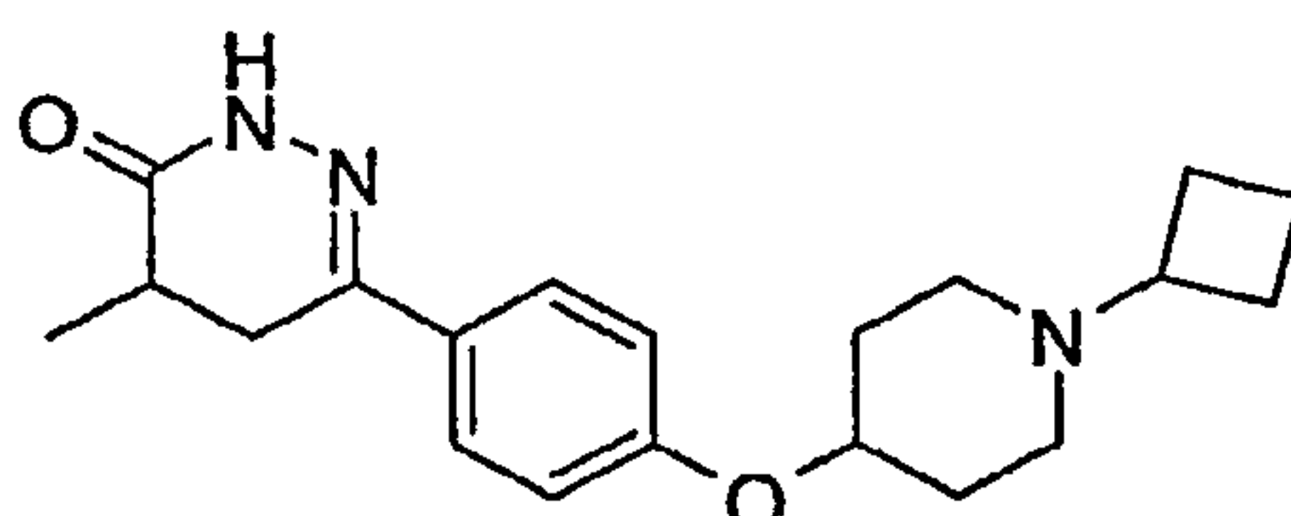
6-[4-(1-Cyclobutyl-piperidin-4-yloxy)-phenyl]-4-methyl-4,5-dihydro-2H-pyridazin-3-one
