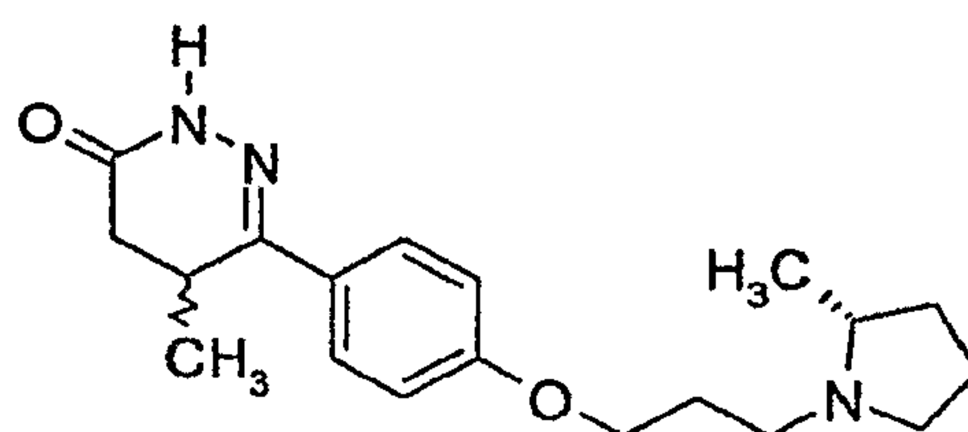
5-Methyl-6-{4-[3-((R)-2-methyl-pyrrolidin-1-yl)-propoxy]-phenyl}-4,5-dihydro-2H-pyridazin-3-one
