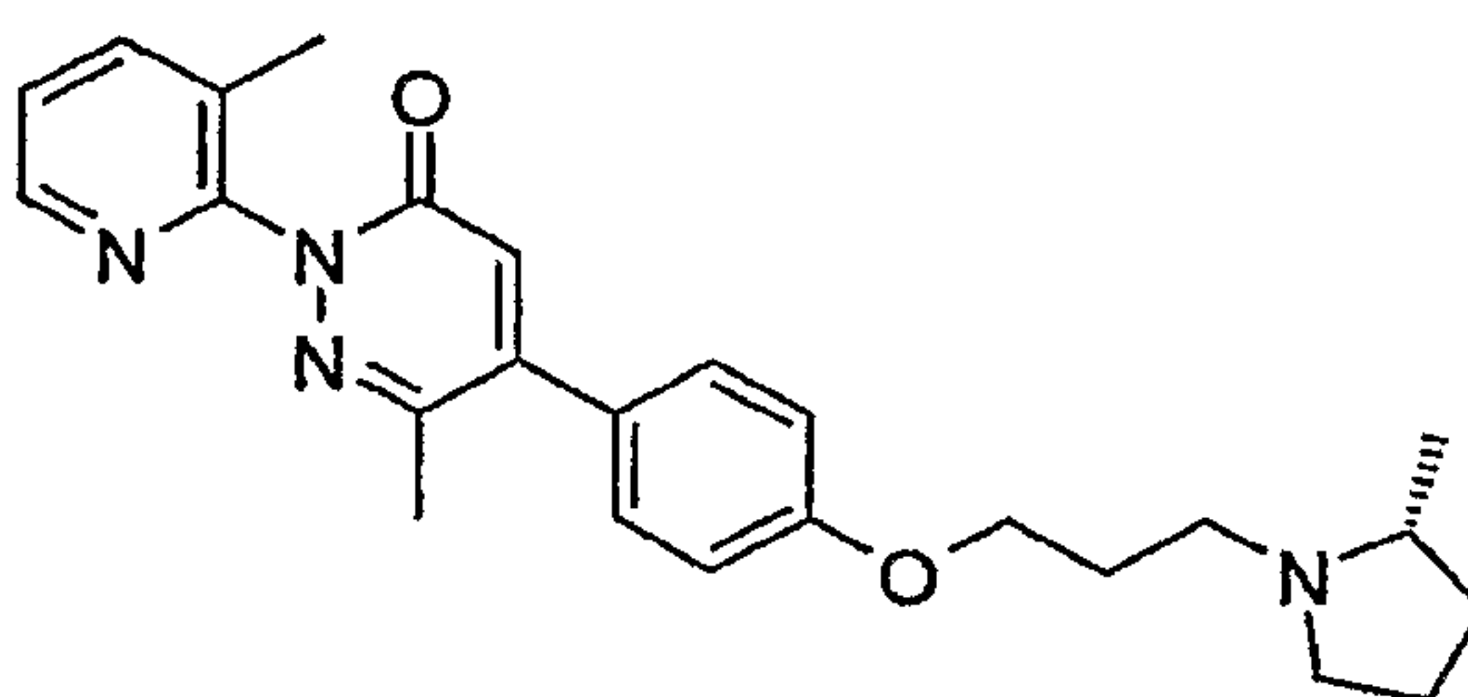
6-Methyl-2-(3-methyl-pyridin-2-yl)-5-{4-[3-((R)-2-methyl-pyrrolidin-1-yl)-propoxy]-phenyl}-2H-pyridazin-3-one
