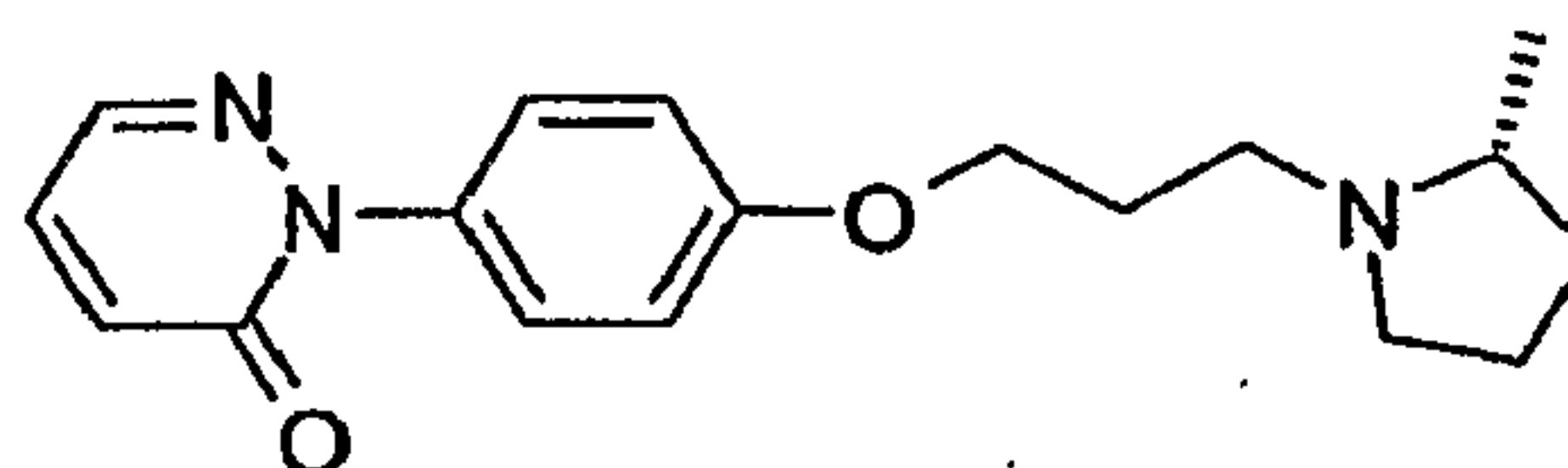
2-{4-[3-((R)-2-Methyl-pyrrolidin-1-yl)-propoxy]-phenyl}-2H-pyridazin-3-one
