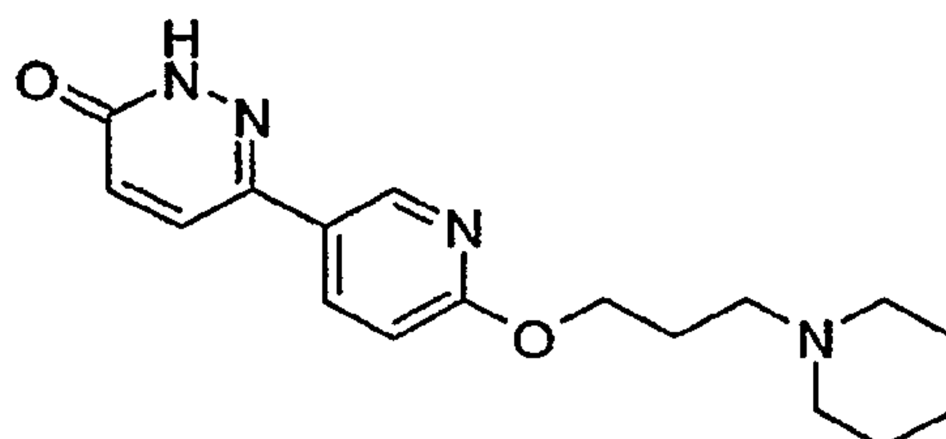
6-[6-(3-Piperidin-1-yl-propoxy)-pyridin-3-yl]-2H-pyridazin-3-one
