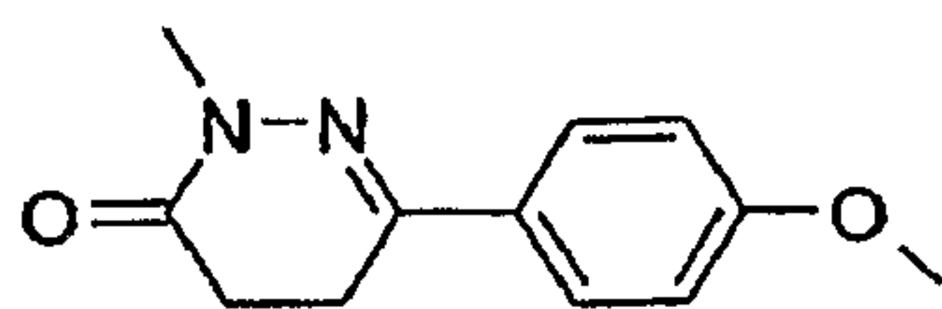
6-(4-Methoxy-phenyl)-2-methyl-4,5-dihydro-2H-pyridazin-3-one
