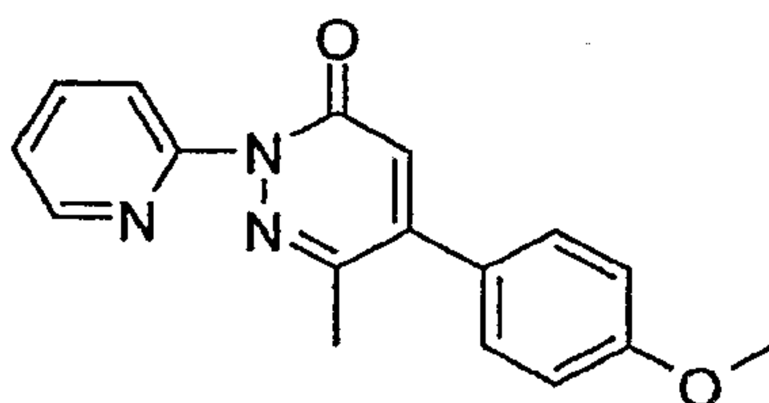
5-(4-Methoxy-phenyl)-6-methyl-2-pyridin-2-yl-2H-pyridazin-3-one
