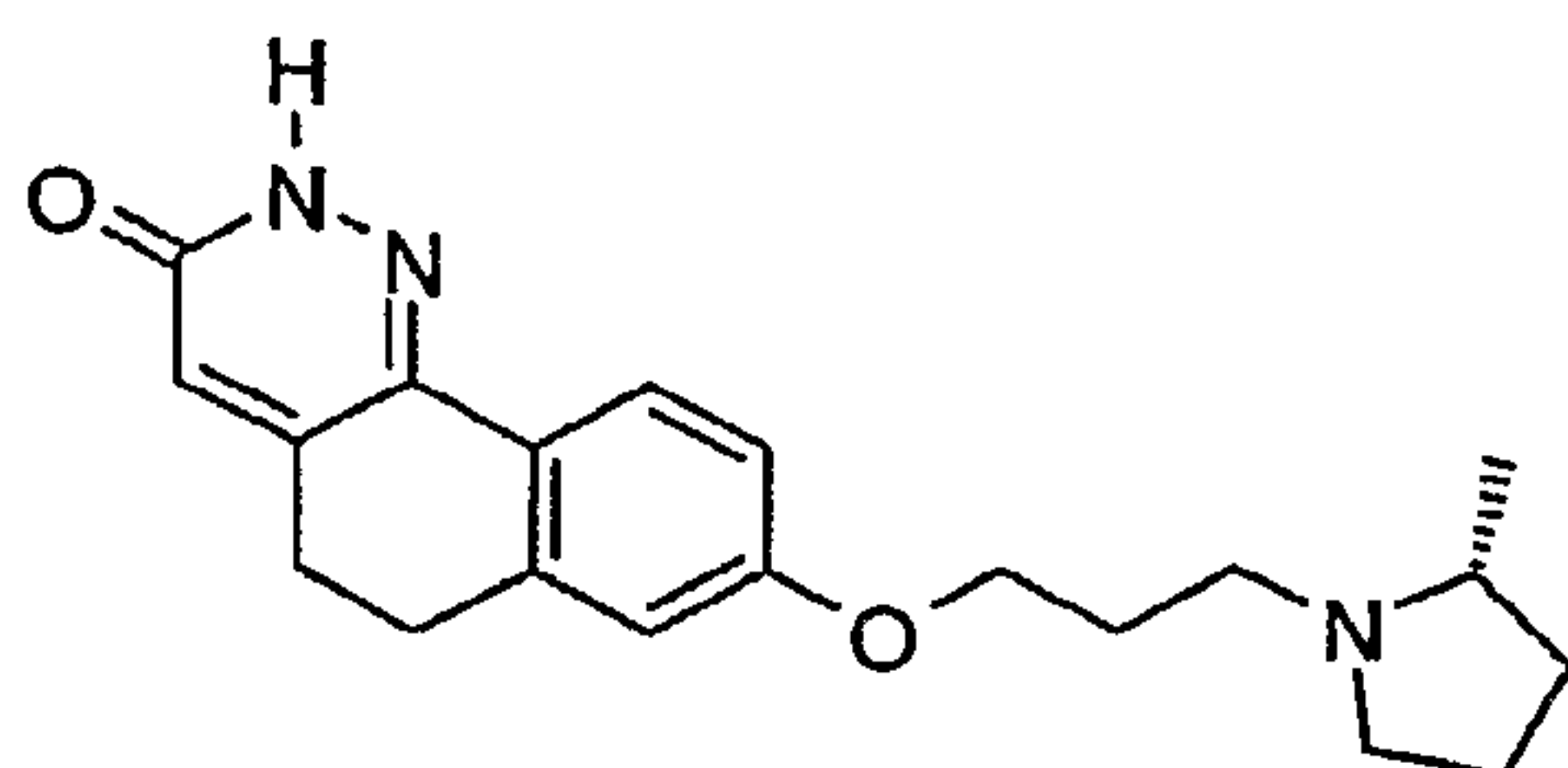
8-[3-((R)-2-Methyl-pyrrolidin-1-yl)-propoxy]-5,6-dihydro-2H-benzo[h]cinnolin-3-one
