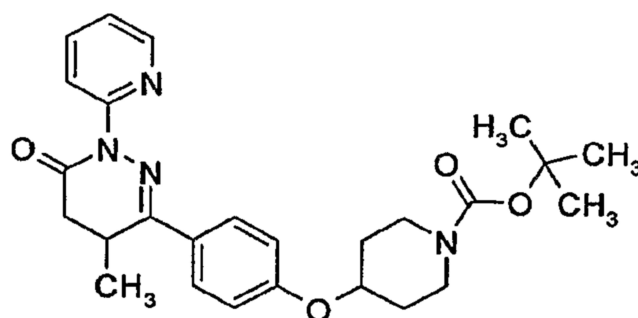
4-[4-(4-Methyl-6-oxo-1-pyridin-2-yl -1,4,5,6-tetrahydro-pyridazin-3-yl)- -phenoxy]-piperidine-1-carboxylic a cid tert-butyl ester
