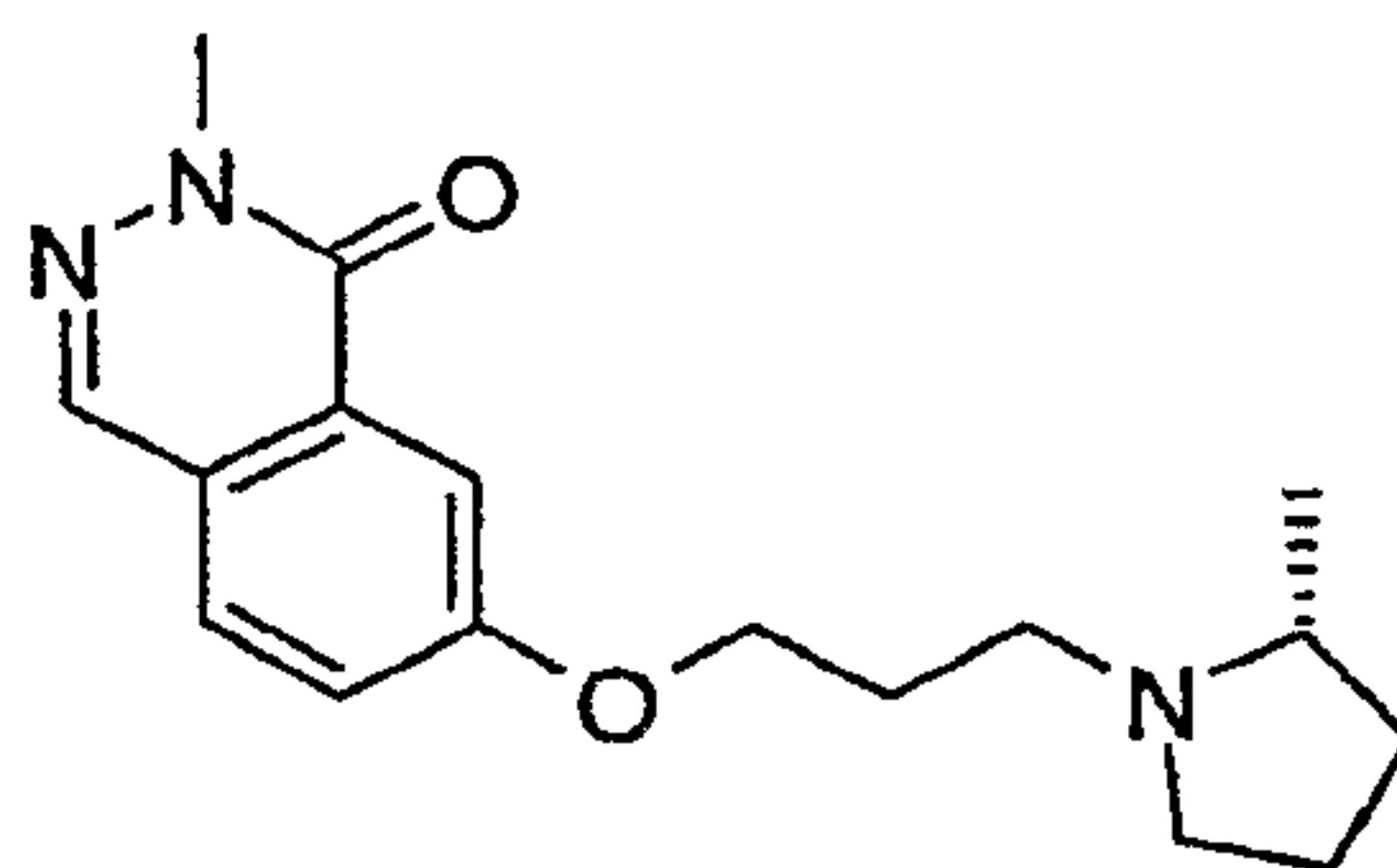
2-Methyl-7-[3-((R)-2-methyl-pyrrolidin-1-yl)-propoxy]-2H-phthalazin-1-one
