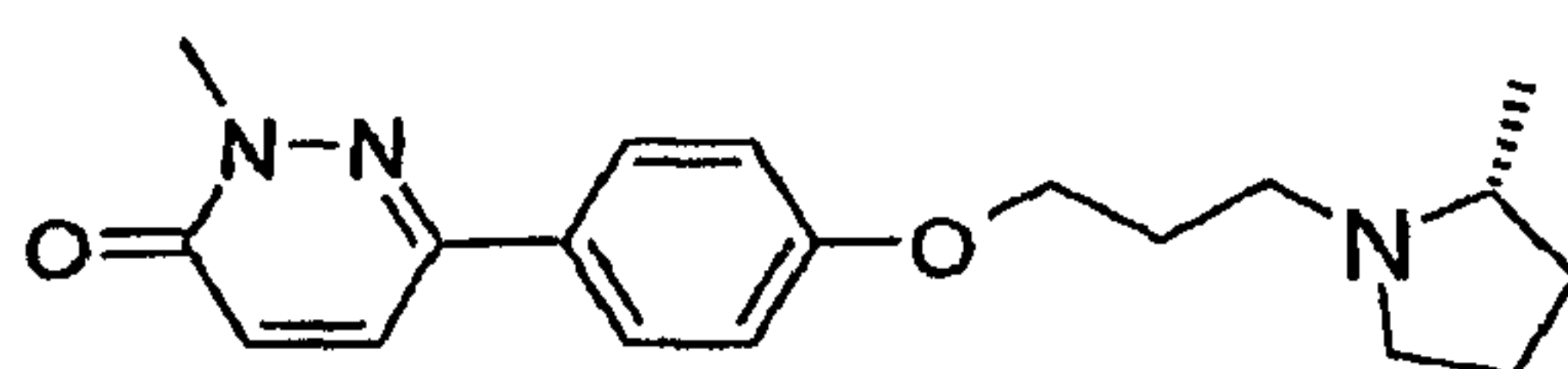
2-Methyl-6-{4-[3-((R)-2-methyl-pyrrolidin-1-yl)-propoxy]-phenyl}-2H-pyridazin-3-one
