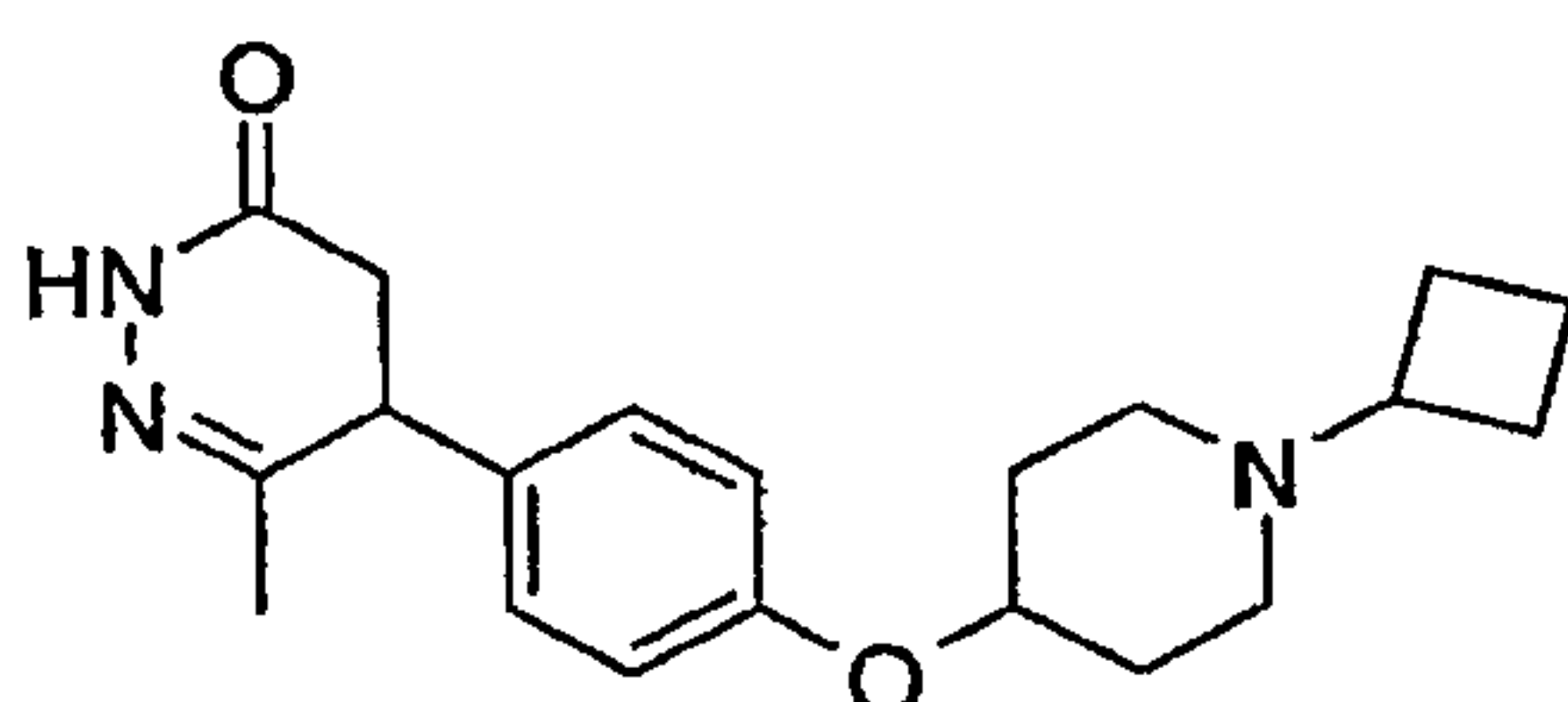
5-[4-(1-Cyclobutyl-piperidin-4-yloxy)-phenyl]-6-methyl-4,5-dihydro-2H-pyridazin-3-one
