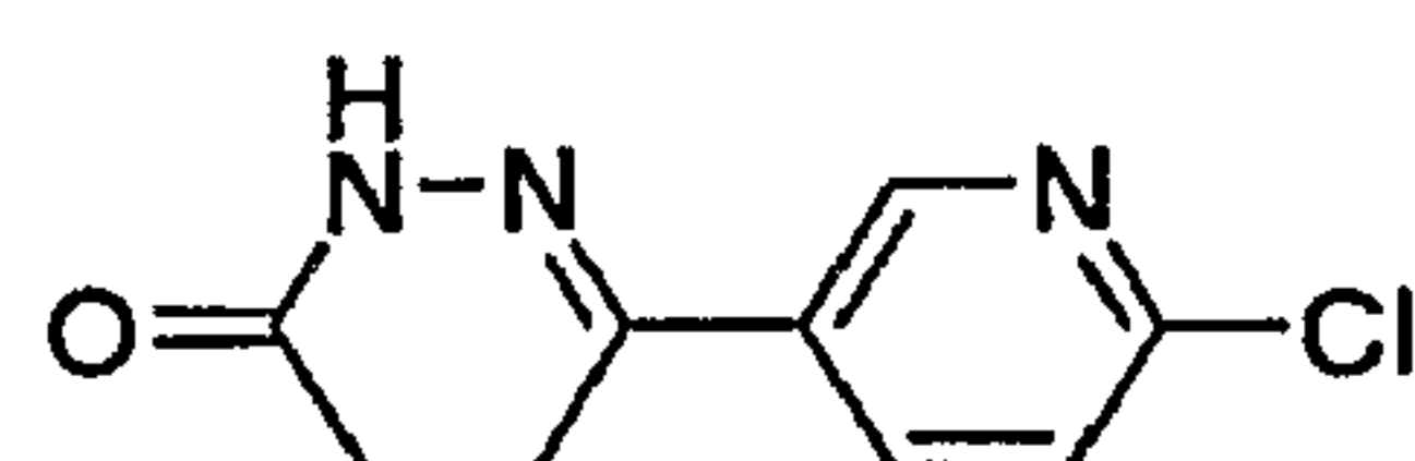
6-(6-Chloro-pyridin-3-yl)-4,5-dihydro-2H-pyridazin-3-one
