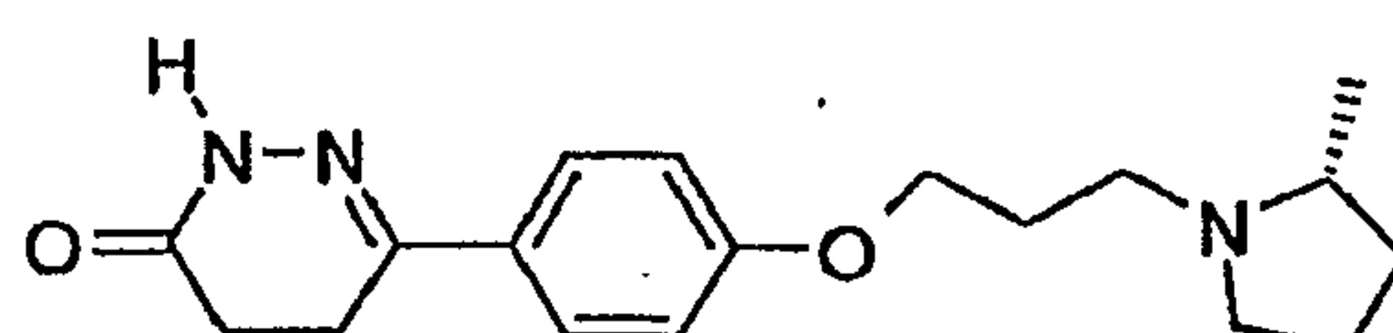
6-[4-[3-((R)-2-Methyl-pyrrolidin-1-yl)-propoxy]-phenyl]-4,5-dihydro-2H-pyridazin-3-one
