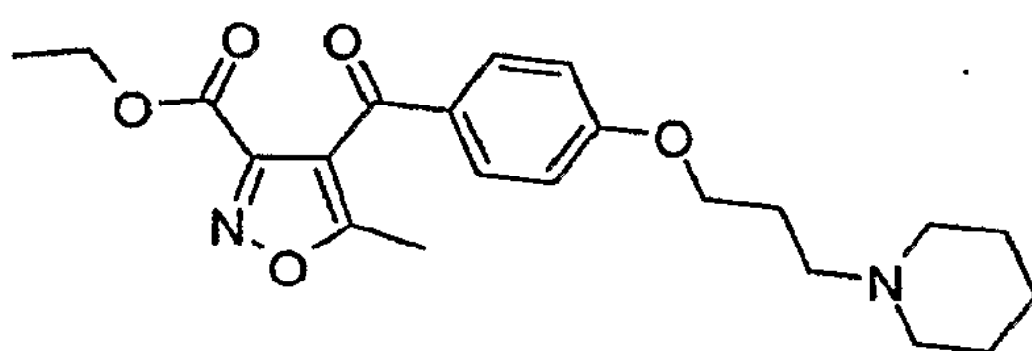
5-Methyl-4-[4-(3-piperidin-1-yl-propoxy)-benzoyl]-isoxazole-3-carboxylic acid ethyl ester
