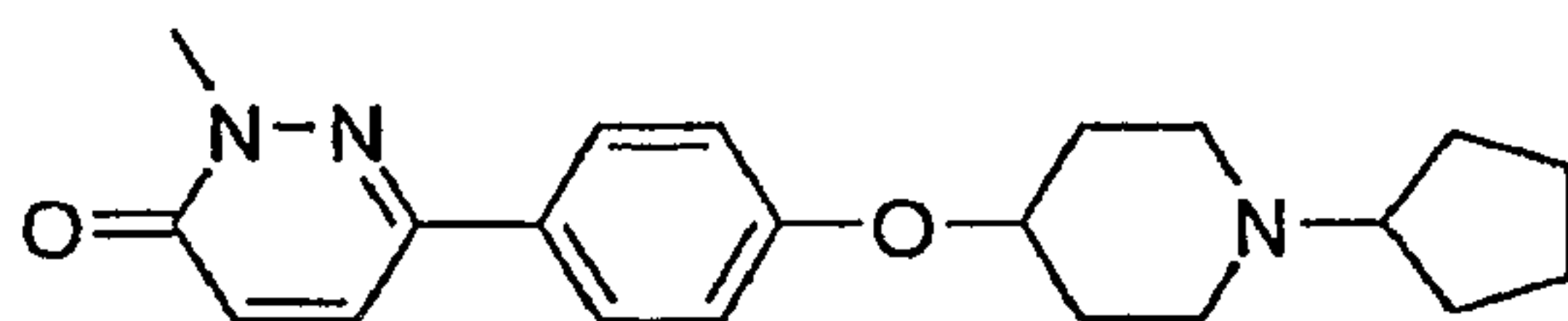
6-[4-(1-Cyclopentyl-piperidin-4-yloxy)-phenyl]- 2-methyl-2H-pyridazin-3-one
