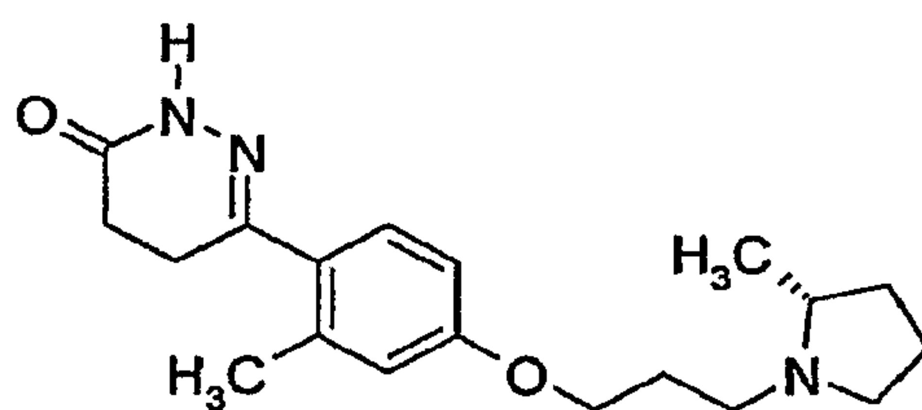
6-((R)-2-Methyl-4-[3-(2-methyl-pyrrolidin-1-yl)-propoxy]-phenyl)-4,5-dihydro-2H-pyridazin-3-one
