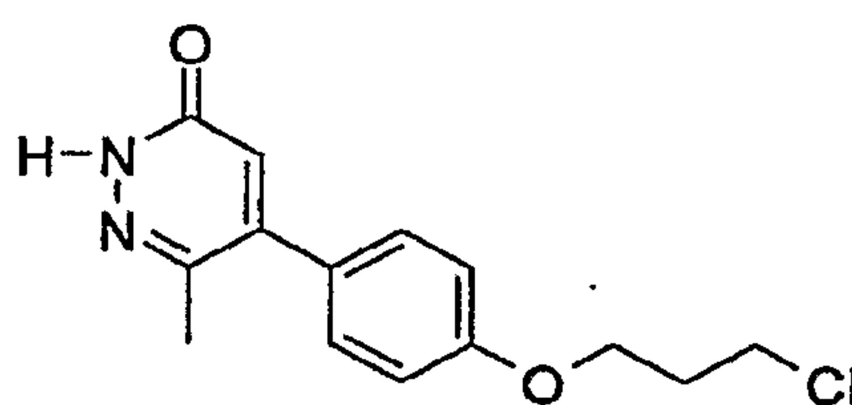
5-[4-(3-Chloropropoxy)phenyl]-6-methyl-2H-pyridazin-3-one
