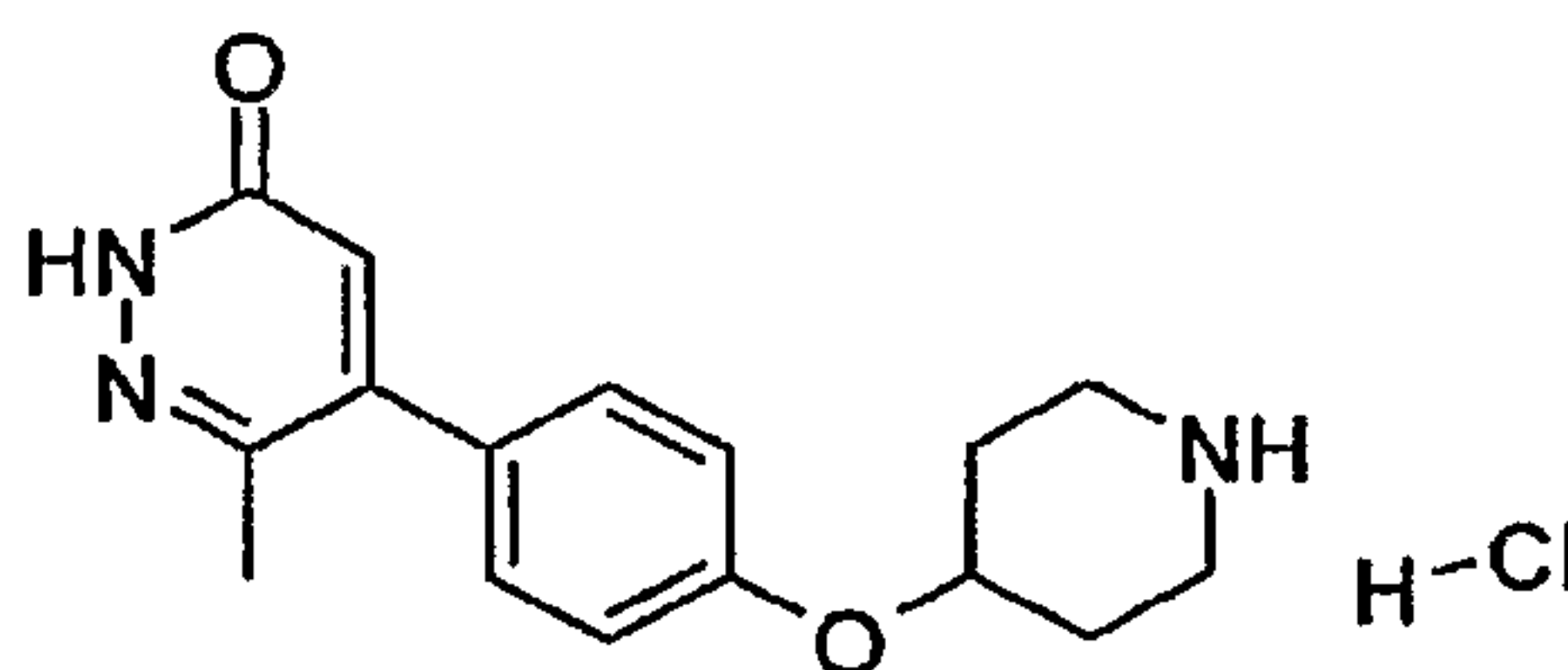
6-Methyl-5-[4-(piperidin-4-yloxy)-phenyl]-2H-pyridazin-3-one; hydrochloride
