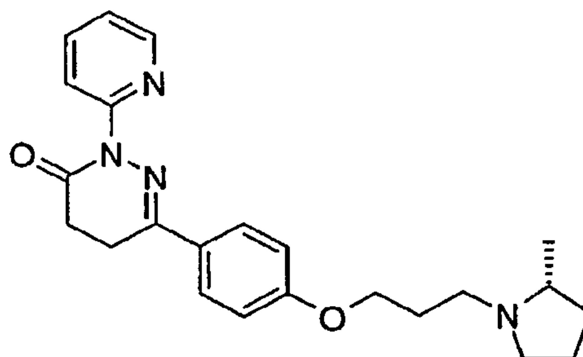
6-{4-[3-((R)-2-Methyl-pyrrolidin-1-yl)-propoxy]-phenyl}-2-pyridin-2-yl-4,5-dihydro-2H-pyridazin-3-one
