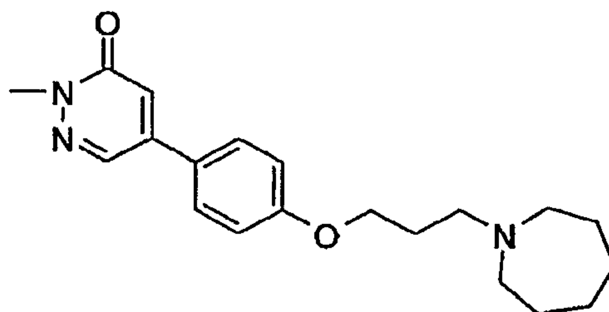
5-[4-(3-Azepan-1-yl-propoxy)-phenyl]-2-methyl-2H-pyridazin-3-one
