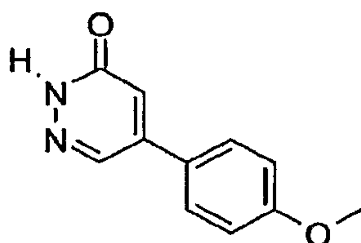
5-(4-Methoxy-phenyl)-2H-pyridazin-3-one
