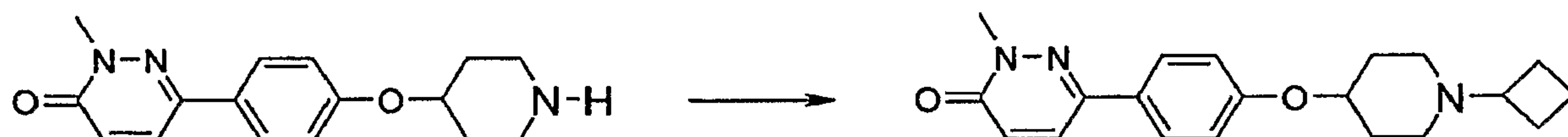
2-Methyl-6-[4-(piperidin-4-yloxy)-phenyl]-2H-pyridazin-3-one
