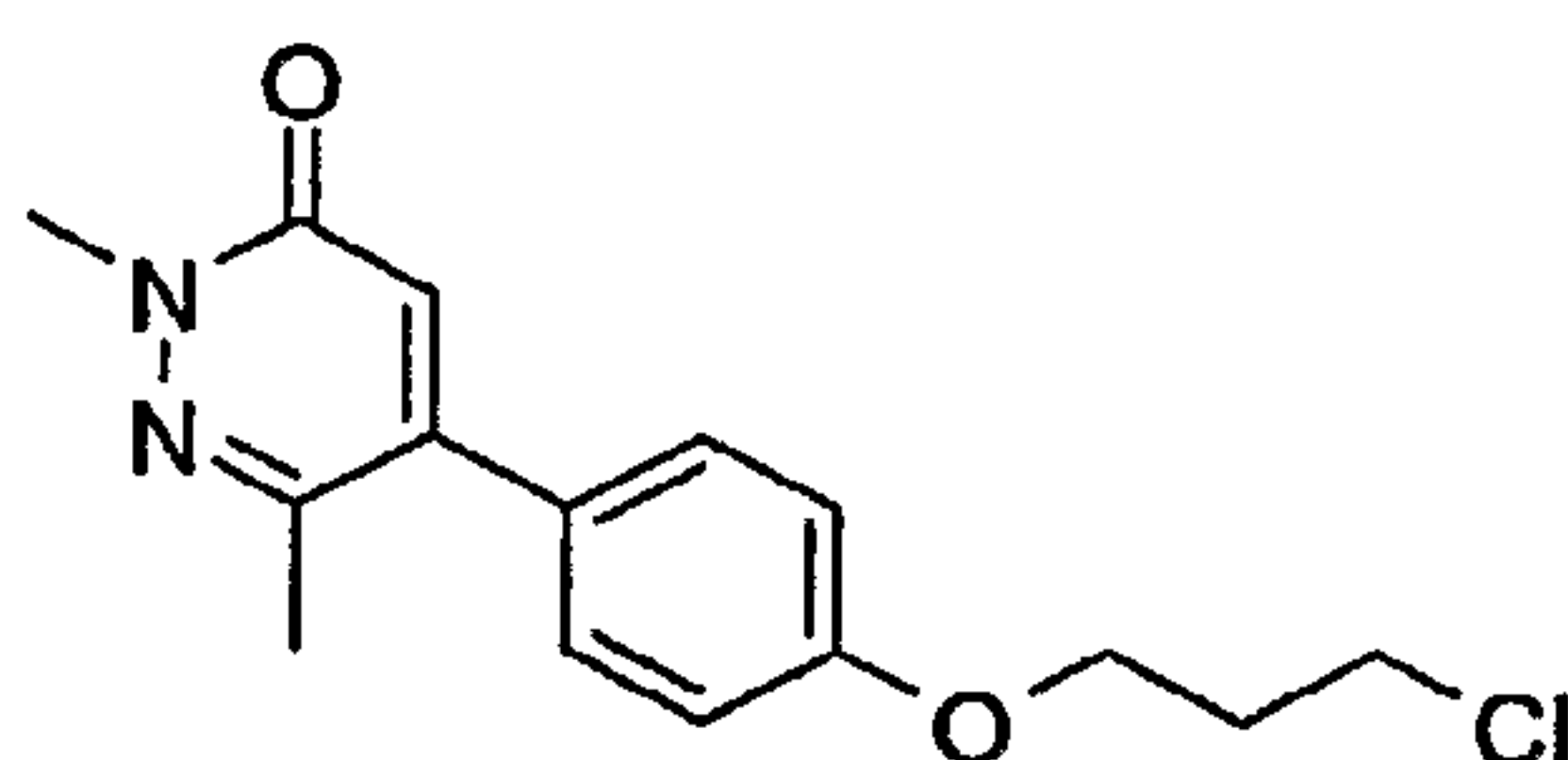
5-[4-(3-Chloro-propoxy)-phenyl]-2,6-dimethyl-2H-pyridazin-3-one
