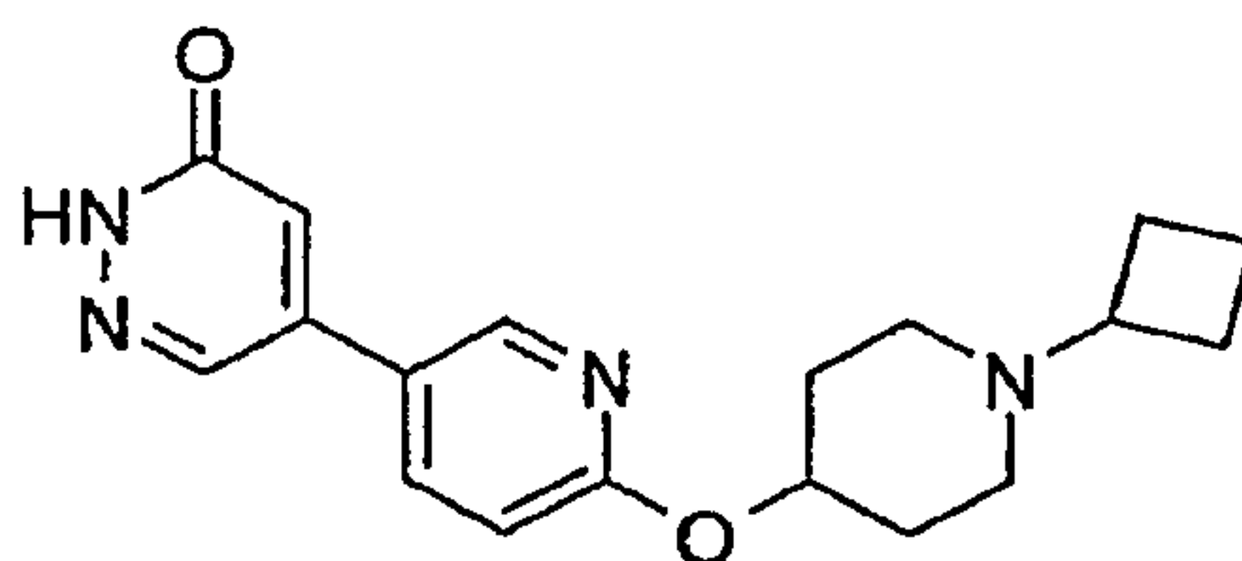
5-[6-(1-Cyclobutyl-piperidin-4-yloxy)- pyridin-3-yl]-2H-pyridazin-3-one
