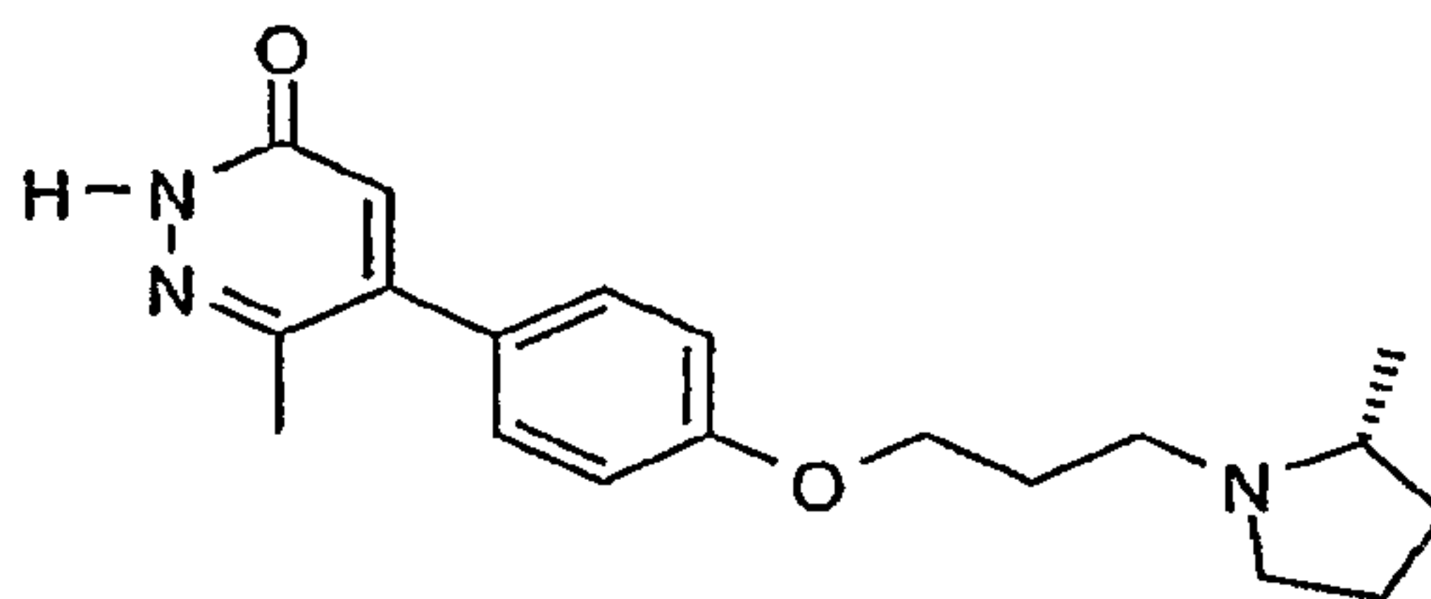
6-Methyl-5-{4-[3-((R)-2-methyl-pyrrolidin-1-yl)-propoxy]-phenyl}-2H-pyridazin-3-one
