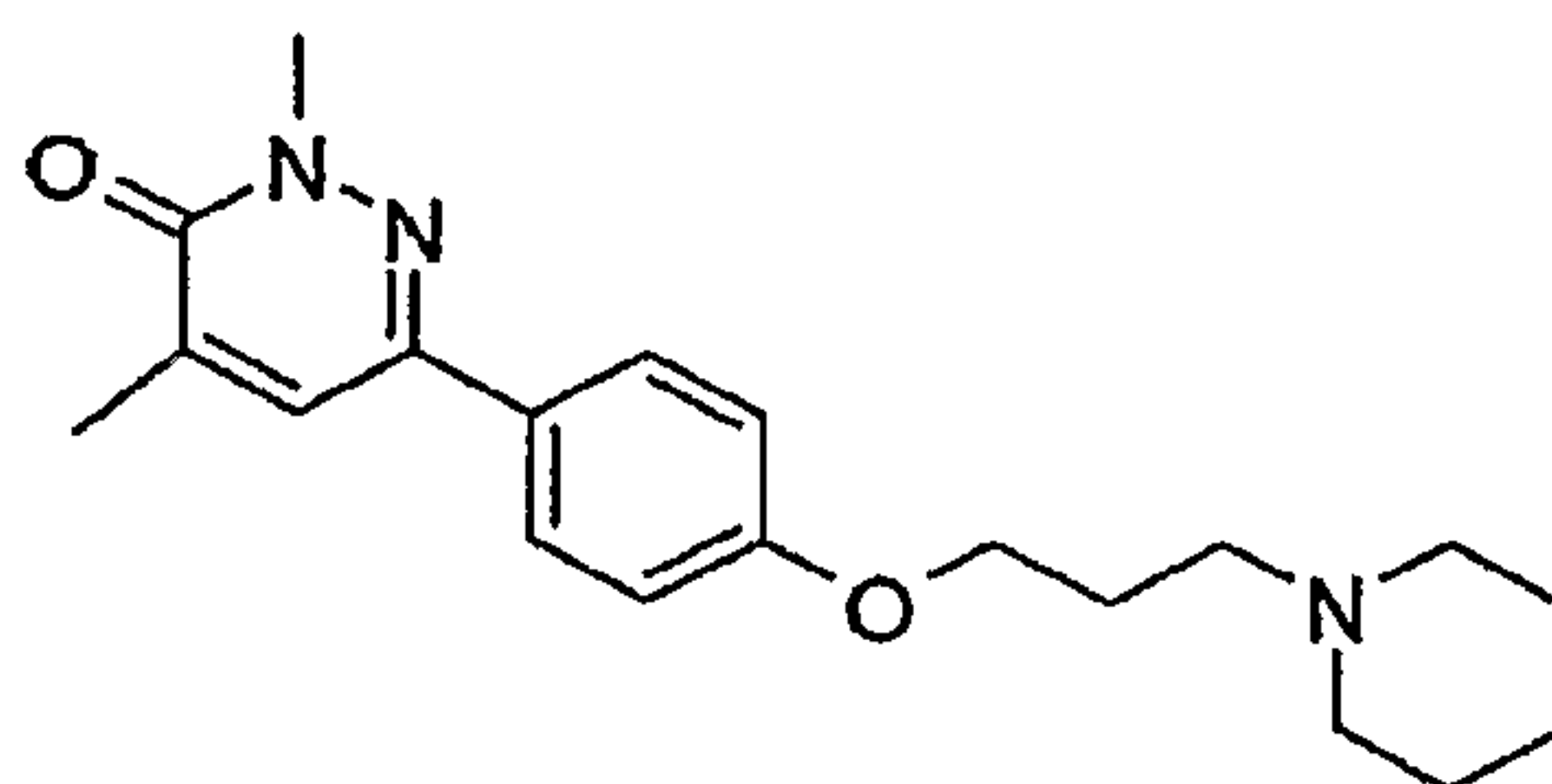
2,4-Dimethyl-6-[4-(3-piperidin-1-yl-propoxy)-phenyl]-2H-pyridazin-3-one
