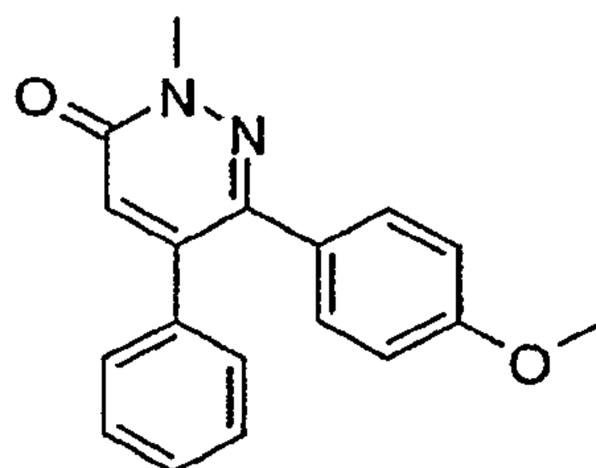
6-(4-Methoxy-phenyl)-2-methyl-5-phenyl-2H-pyridazin-3-one
