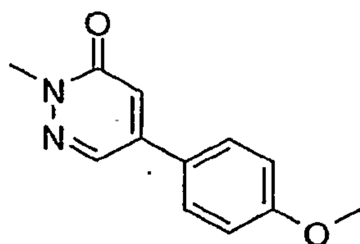
5-(4-Methoxy-phenyl)-2-methyl-2H-pyridazin-3-one
