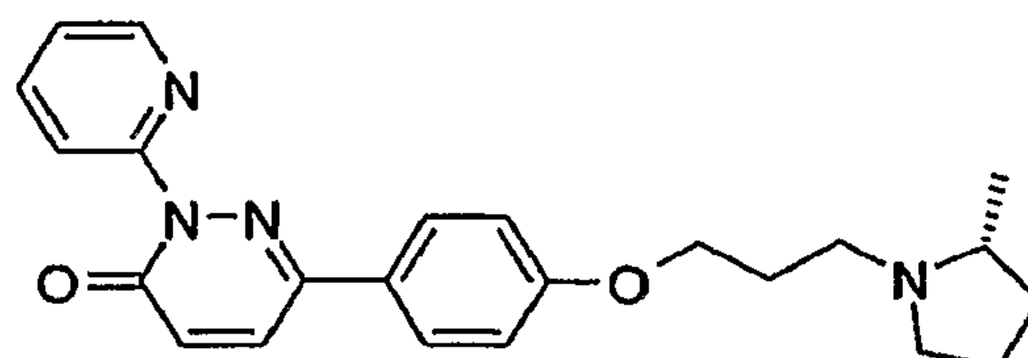
6-{4-[3-((R)-2-Methyl-pyrrolidin-1-yl)-propoxy]-phenyl}-2-pyridin-2-yl-2H-pyridazin-3-one
