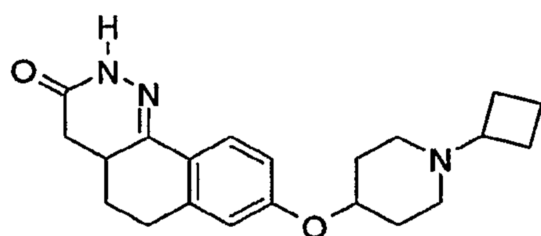
8-(1-Cyclobutyl-piperidin-4-yloxy)- 4,4a,5,6-tetrahydro-2H-benzo[h]cinn olin-3-one
