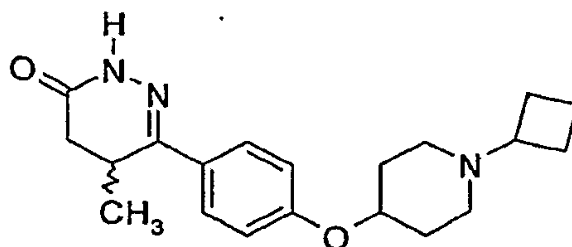
6-[4-(1-Cyclobutyl-piperidin-4-yloxy)-phenyl] -5-methyl-4,5-dihydro-2H-pyridazin-3-one
