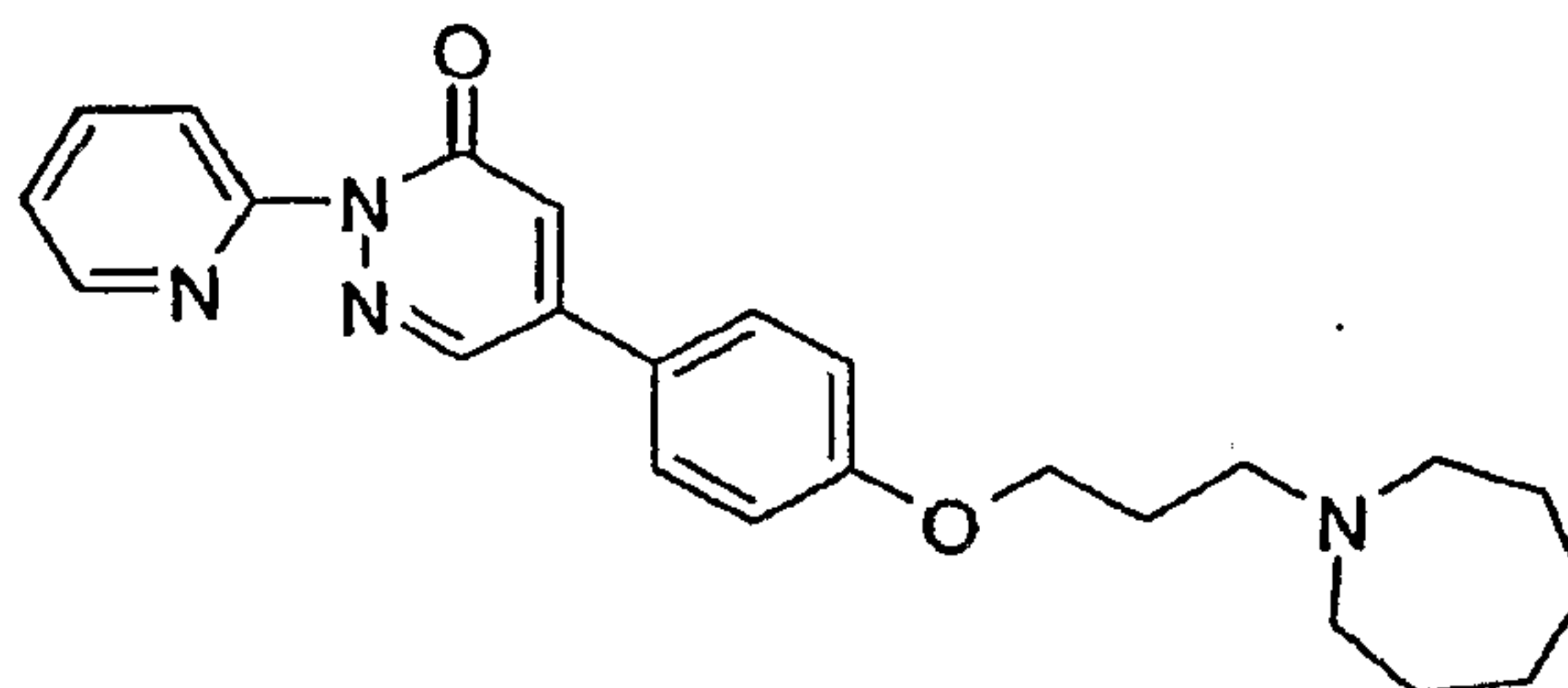
5-[4-(3-Azepan-1-yl-propoxy)-phenyl] 2-pyridin-2-yl-2H-pyridazin-3-one
