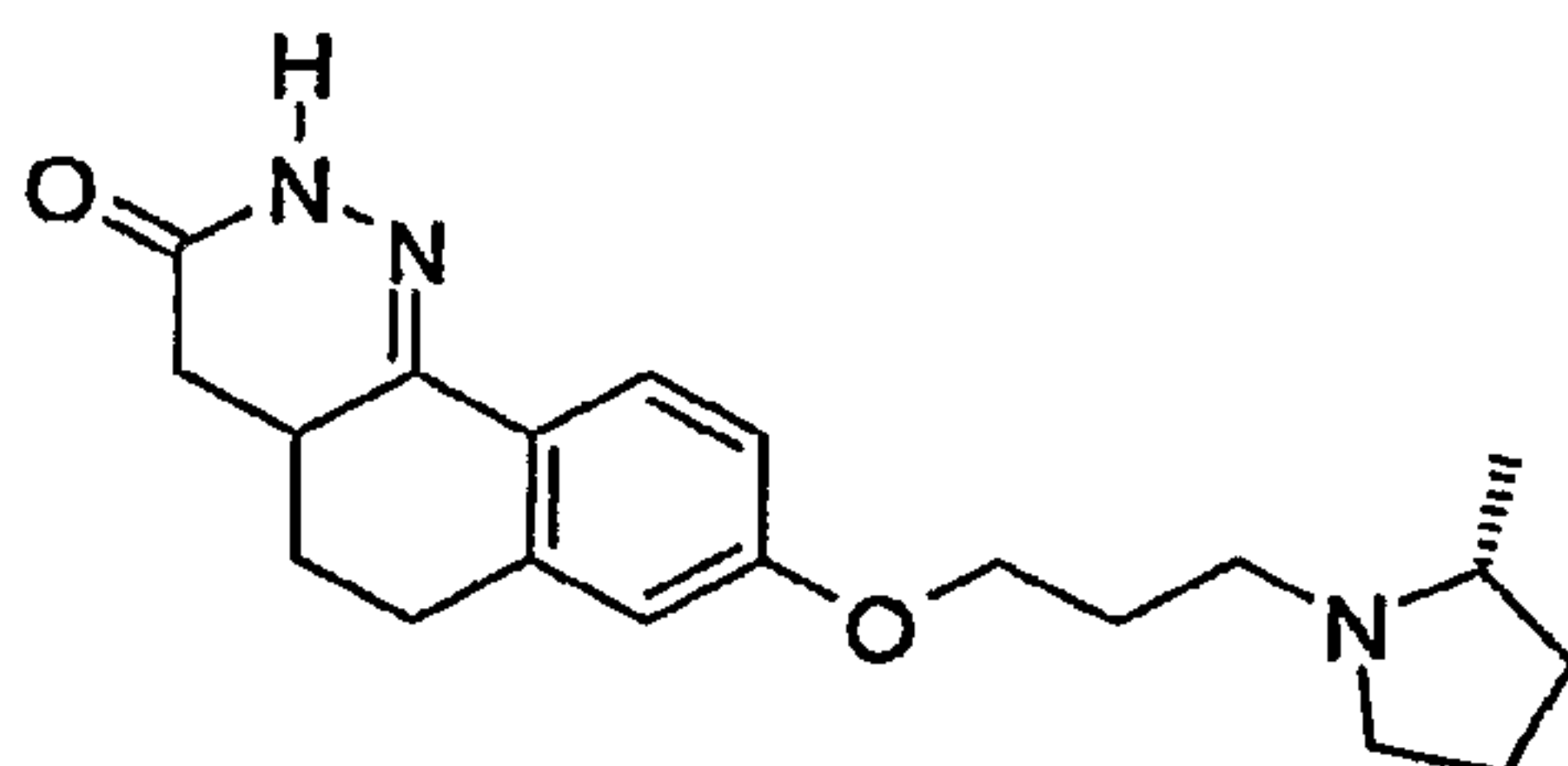
8-[3-(2-Methyl-pyrrolidin-1-yl)-propoxy]-4,4a,5,6-tetrahydro-2H-benzo[h]cinnolin-3-one
