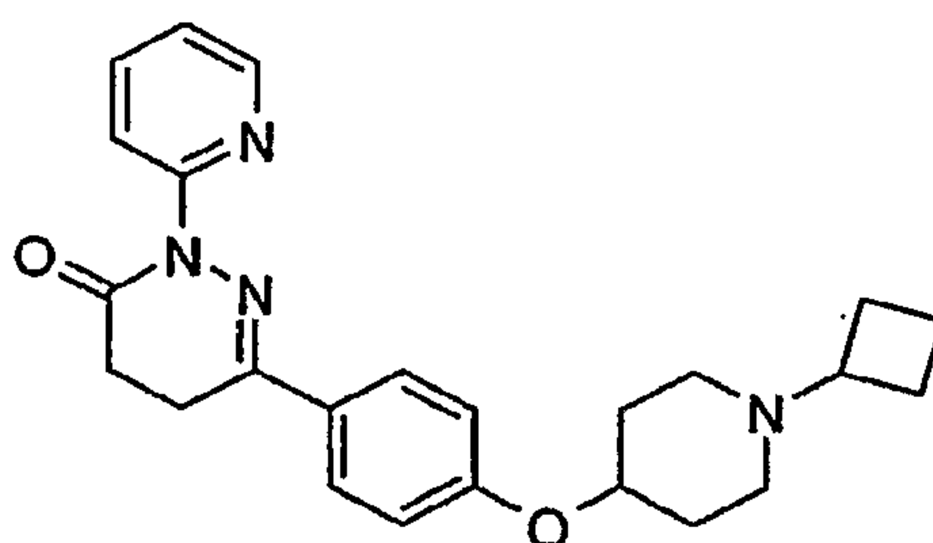
6-[4-(1-Cyclobutyl-piperidin-4-yloxy)-phenyl]-2-pyridin-2-yl-4,5-dihydro-2H-pyridazin-3-one
