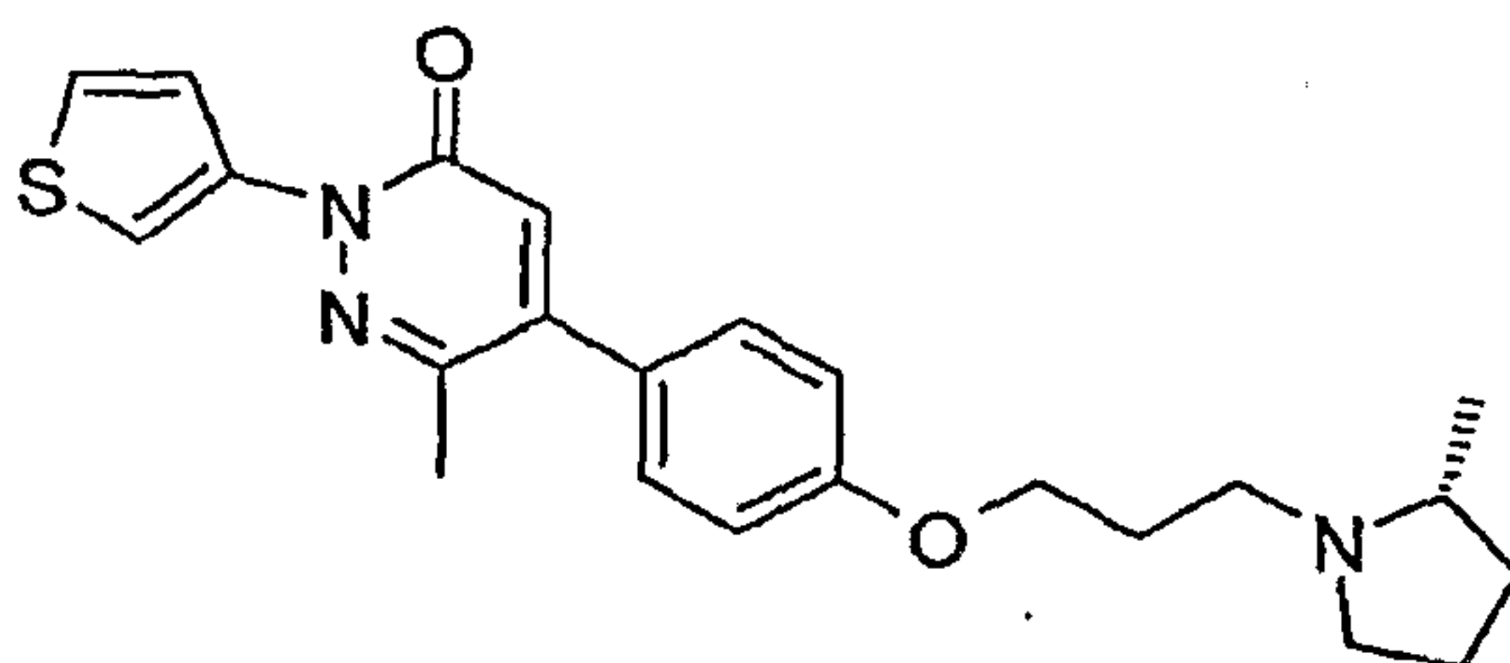
6-Methyl-5-{4-[3-((R)-2-methyl-pyrrolidin-1-yl)-propoxy]-phenyl}-2-thiophen-3-yl-2H-pyridazin-3-one
