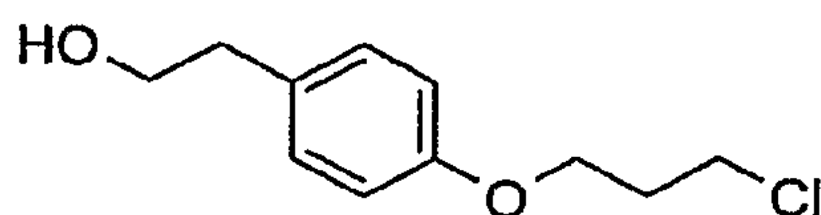
2-[4-(3-Chloro-propoxy)-phenyl]-ethanol
