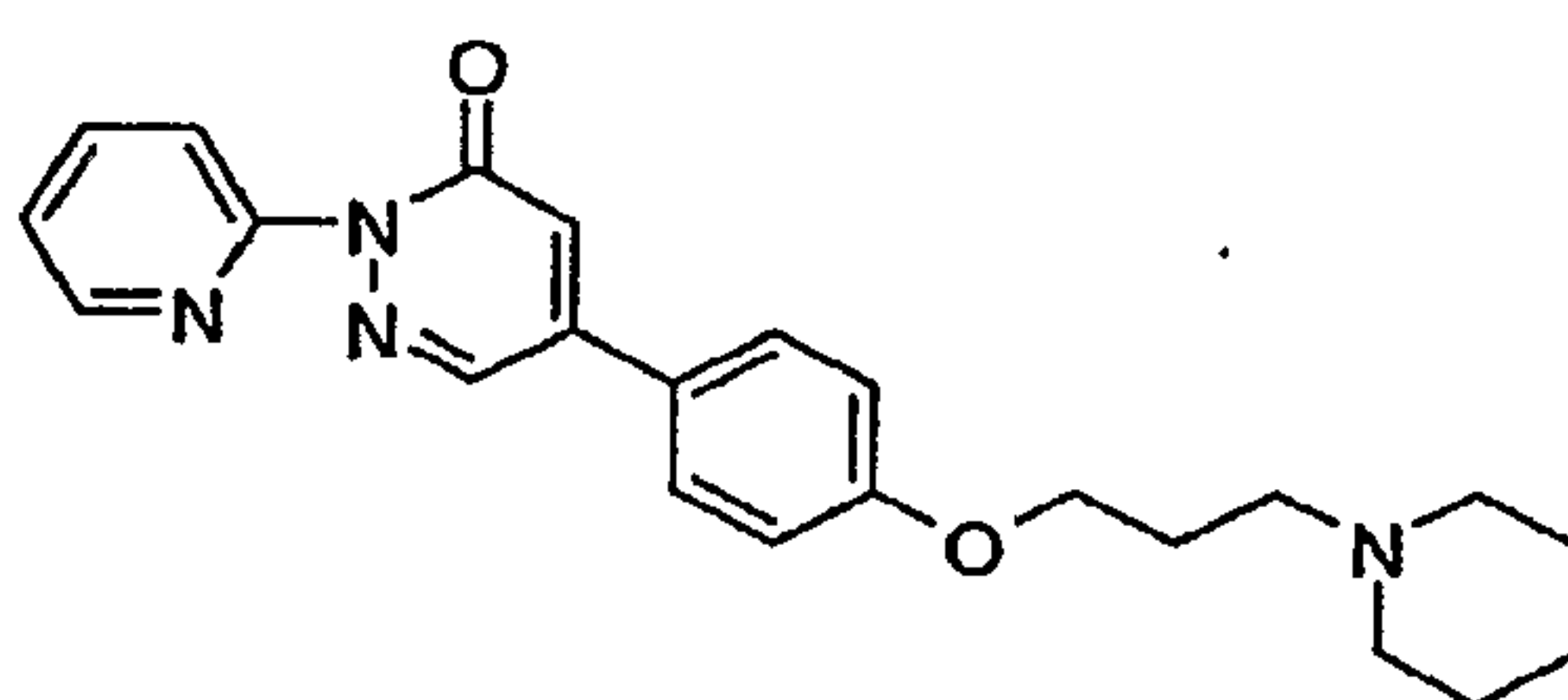
5-[4-(3-Piperidin-1-yl-propoxy)-phenyl]-2-pyridin-2-yl-2H-pyridazin-3-one
