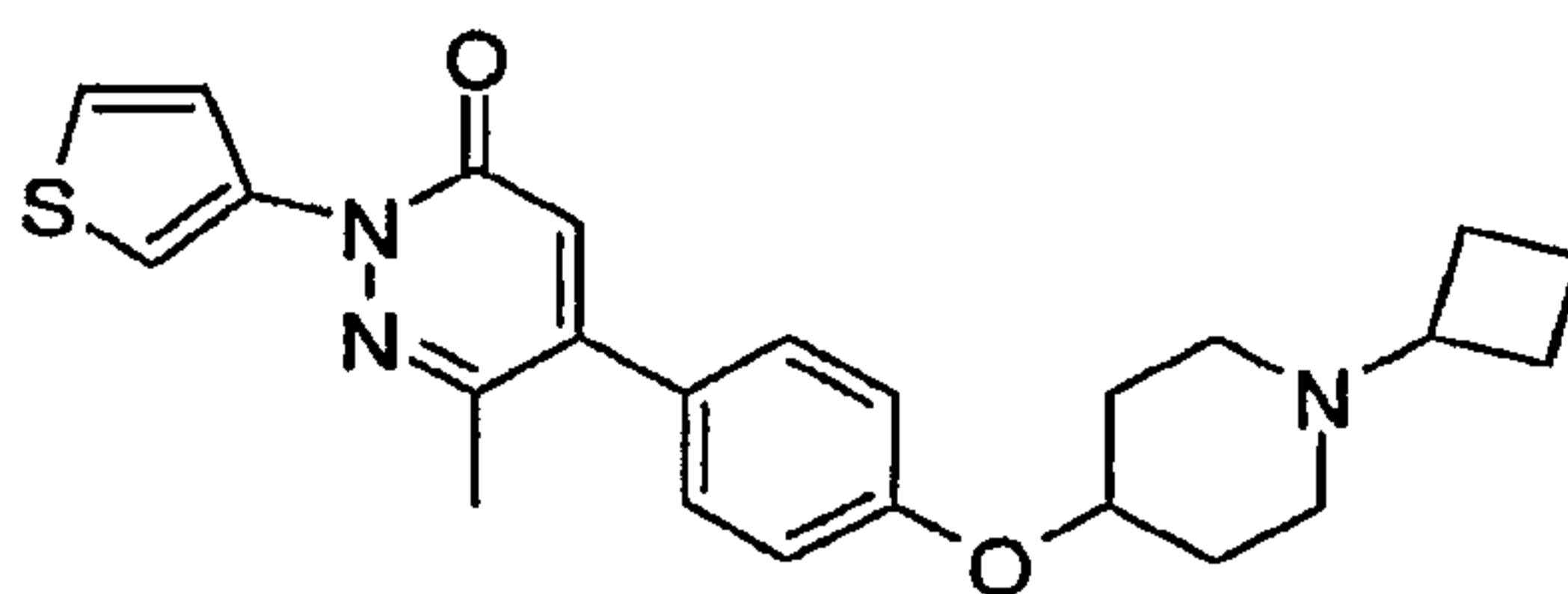
5-[4-(1-Cyclobutyl-piperidin-4-yloxy)-phenyl]-6-methyl-2-thiophen-3-yl-2H-pyridazin-3-one
