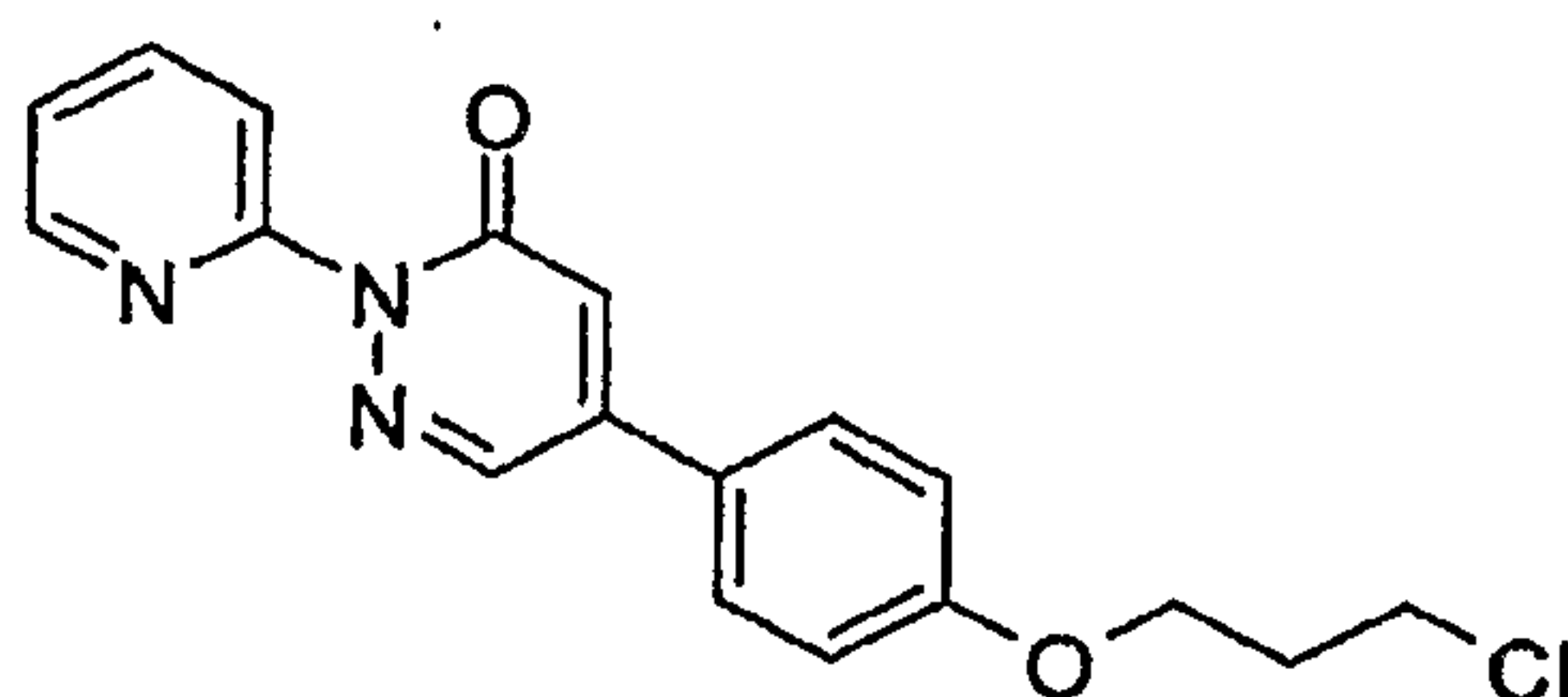
5-[4-(3-Chloro-propoxy)-phenyl]-2-pyridin-2-yl-2H-pyridazin-3-one
