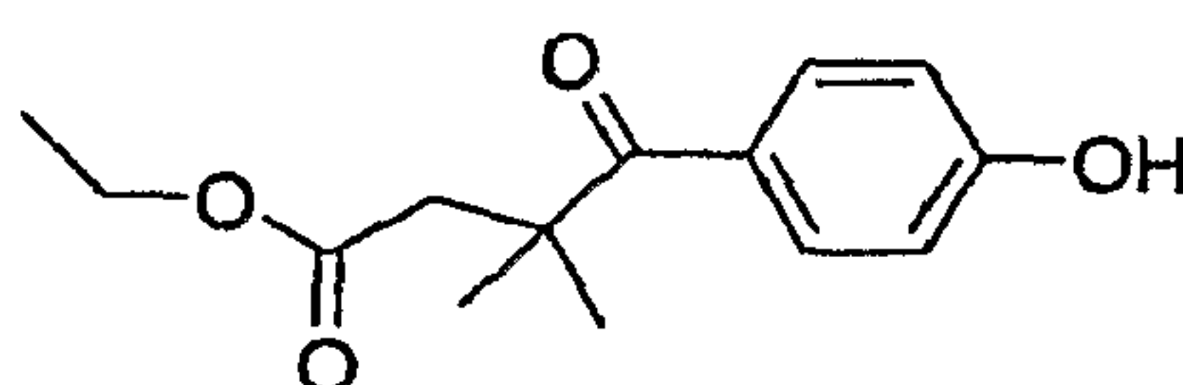
4-(4-Hydroxy-phenyl)-3,3-dimethyl-4 -oxo-butyl ethyl ester
