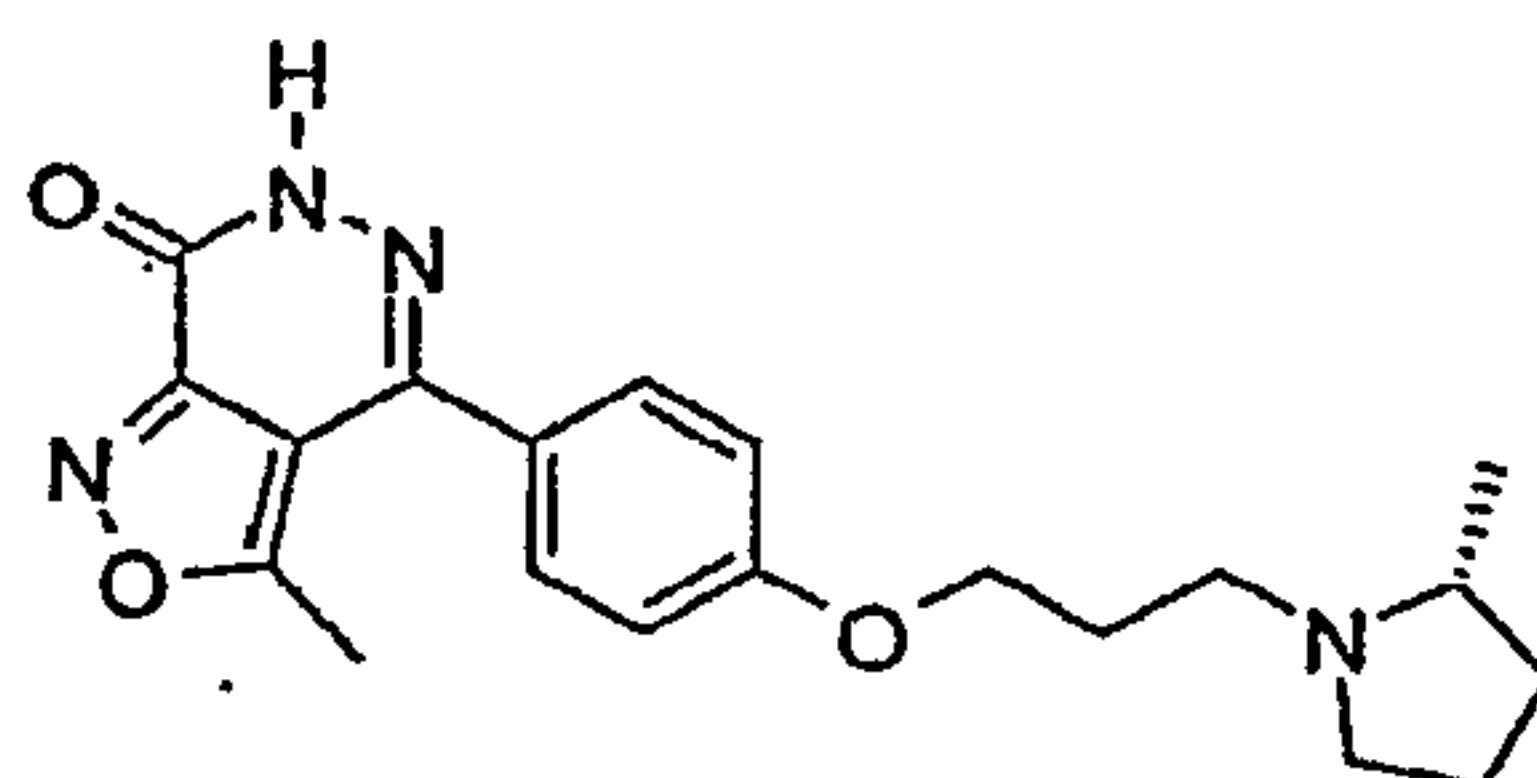
3-Methyl-4-[4-[3-((R)-2-methyl-pyrrolidin-1-yl)-propoxy]-phenyl]-6H-isoxazolo[3,4-d]pyridazin-7-one
