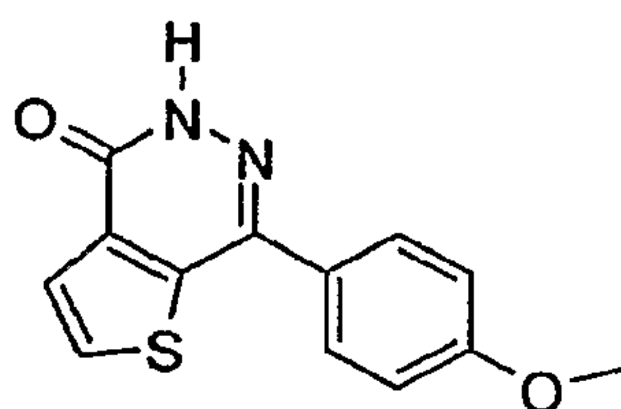
7-(4-Methoxy-phenyl)-5H-thieno[2,3-d]pyridazin-4-one
