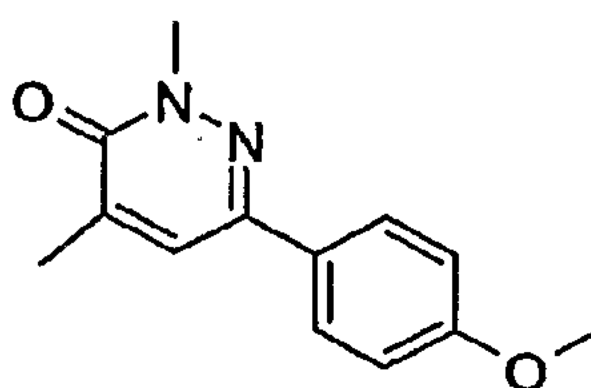
6-(4-Methoxy-phenyl)-2,4-dimethyl-2H-pyridazin-3-one
