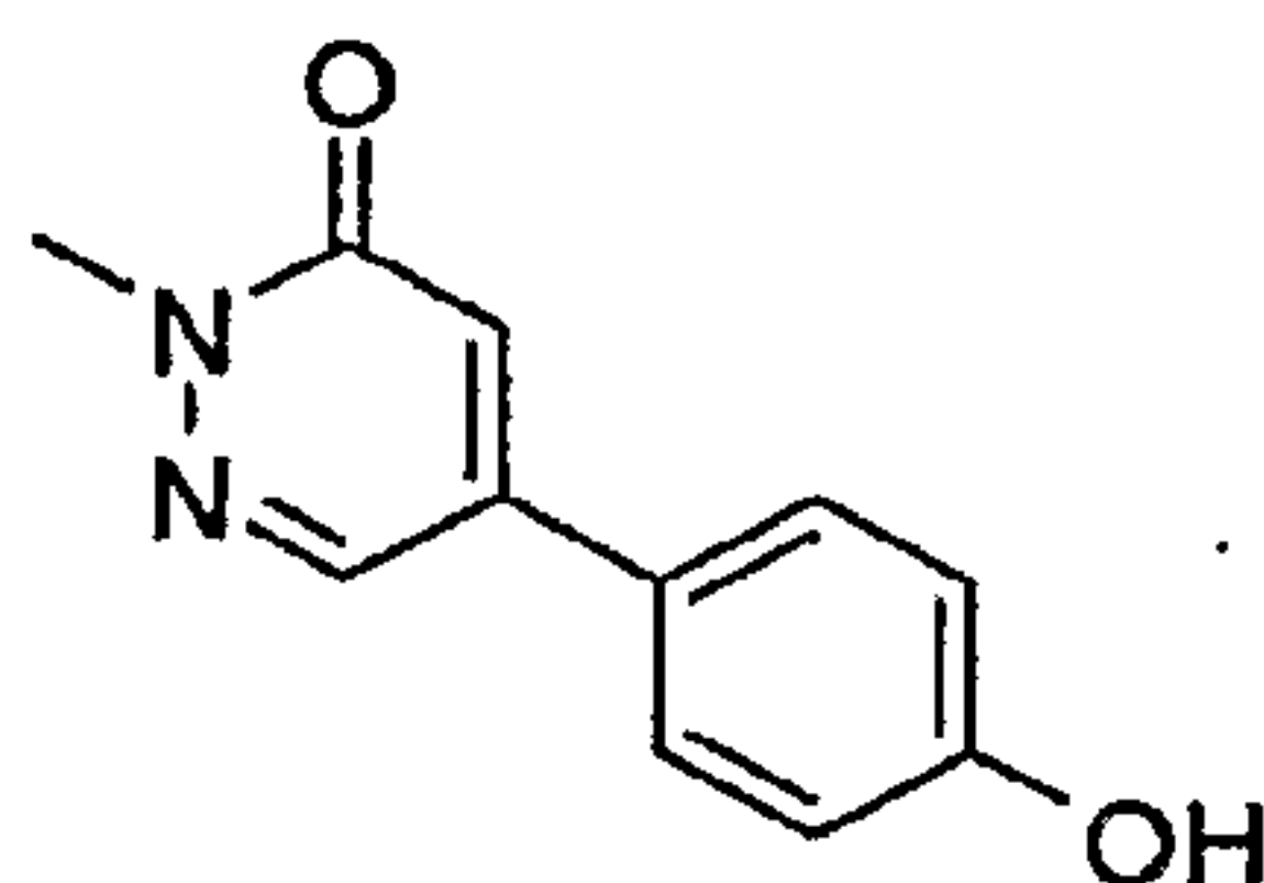
5-(4-Hydroxy-phenyl)-2-methyl-2H-pyridazin-3-one
