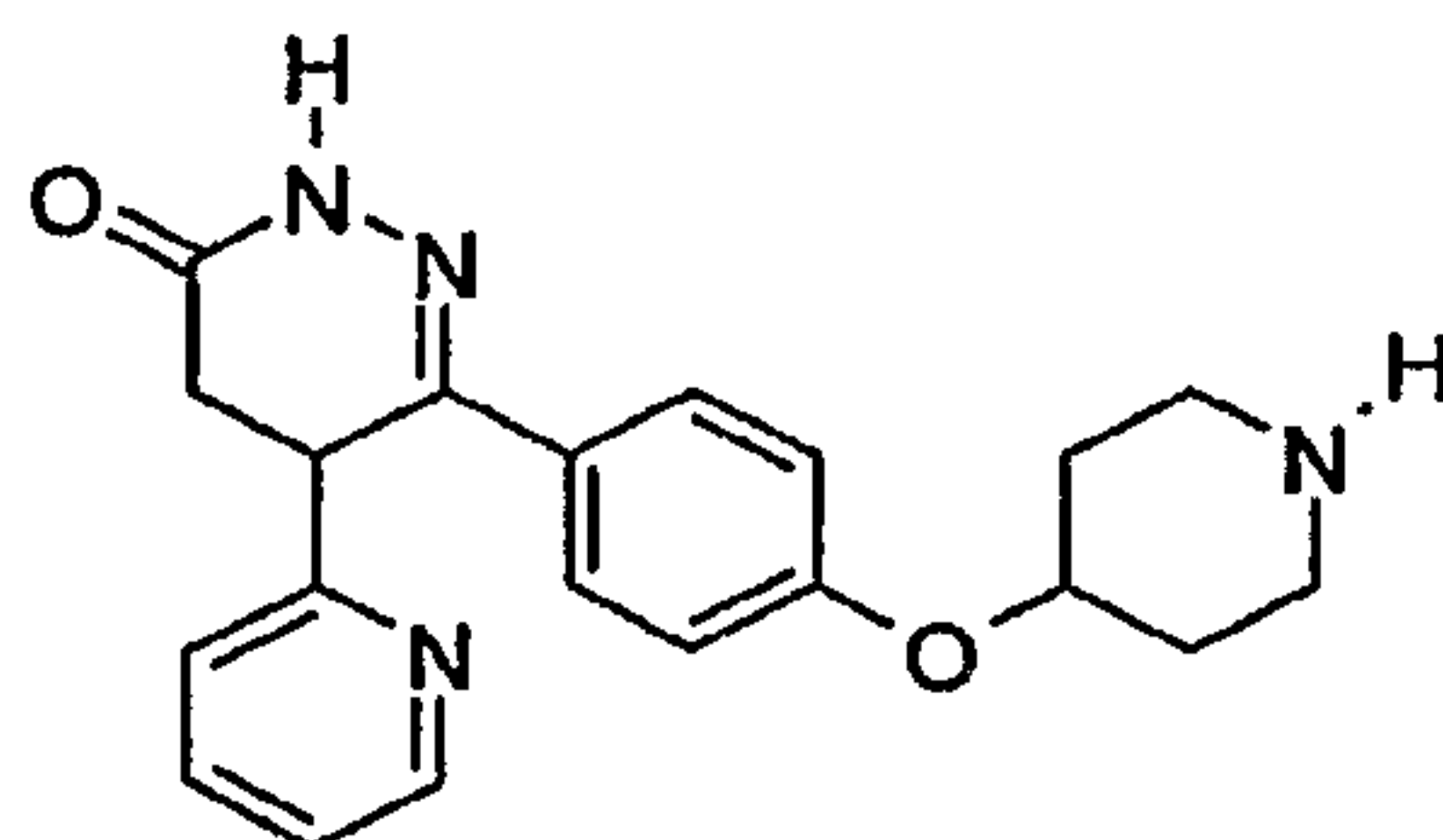
6-[4-(Piperidin-4-yloxy)-phenyl]-5-pyridin-2-yl-4,5-dihydro-2H-pyridazin-3-one
