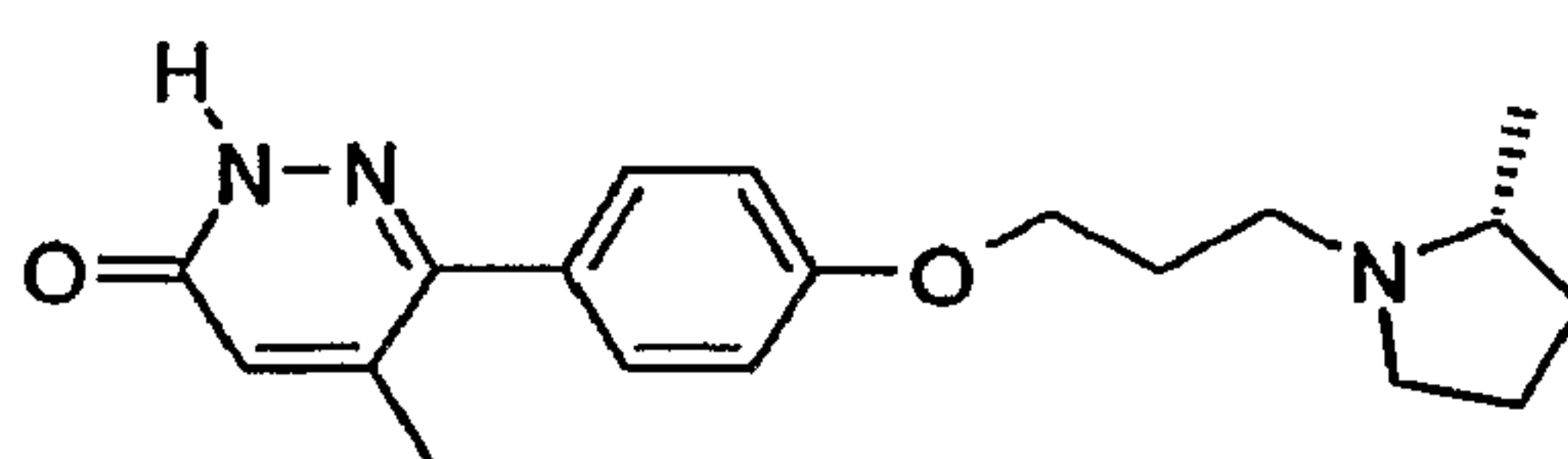
5-Methyl-6-{4-[3-((R)-2-methyl-pyrrolidin-1-yl)-propoxy]-phenyl}-2H-pyridazin-3-one
