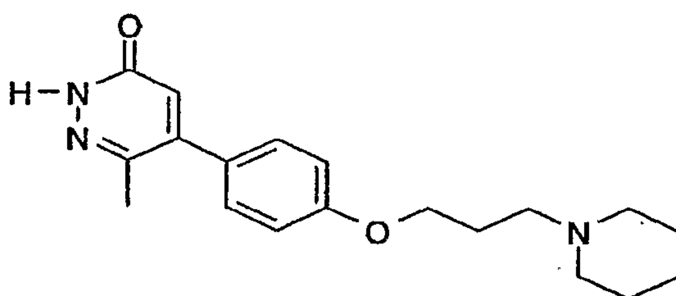
6-Methyl-5-[4-(3-piperidin-1-yl-propoxy)-phenyl]-2H-pyridazin-3-one
