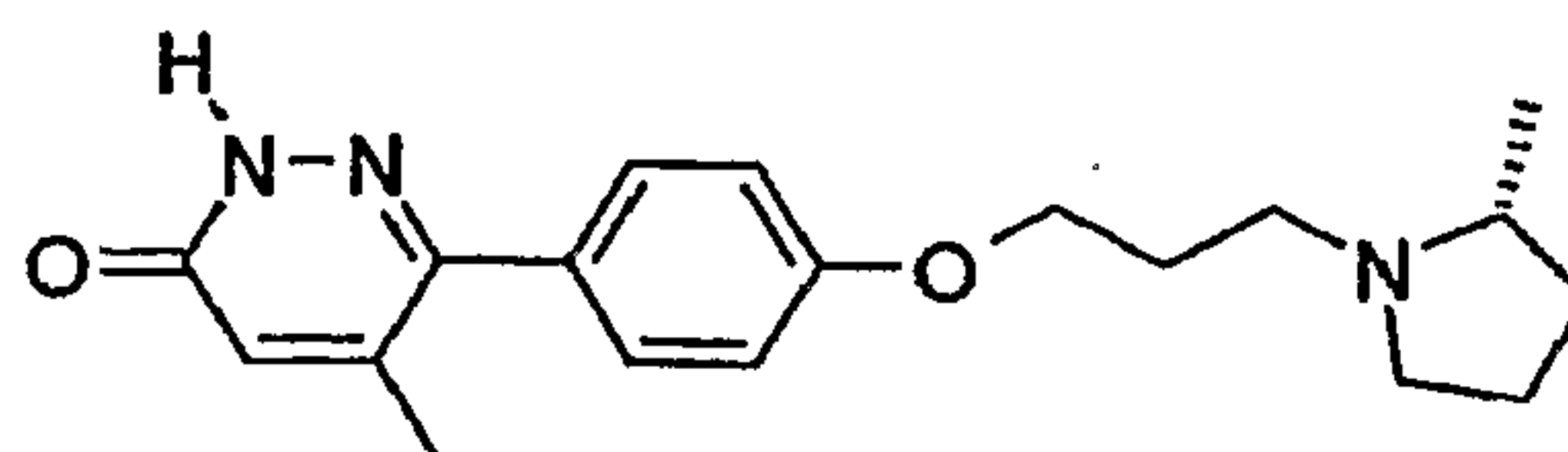
5-Ethyl-6-{4-[3-((R)-2-methyl-pyrrolidin-1-yl)-propoxy]-phenyl}-2H-pyridazin-3-one
