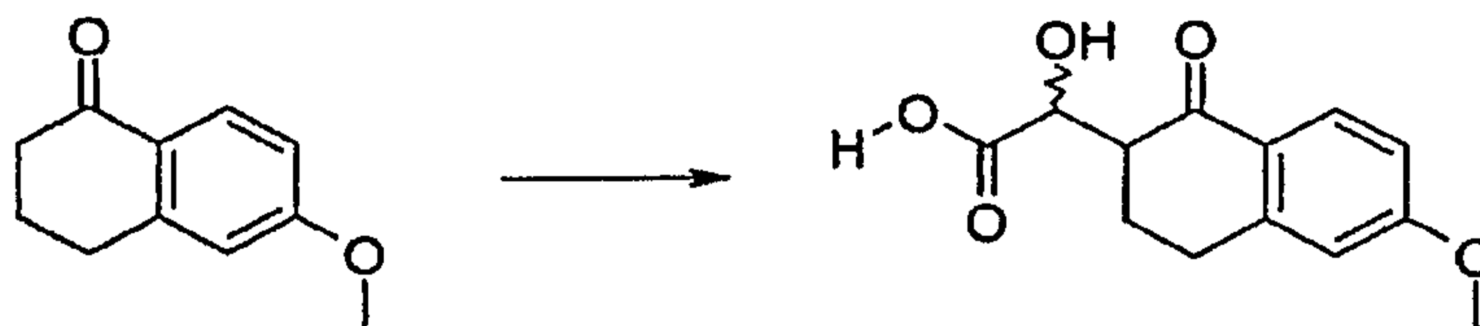
Hydroxy-(6-methoxy-1-oxo-1,2,3,4-tetrahydro-naphthalen-2-yl)-acetic acid
