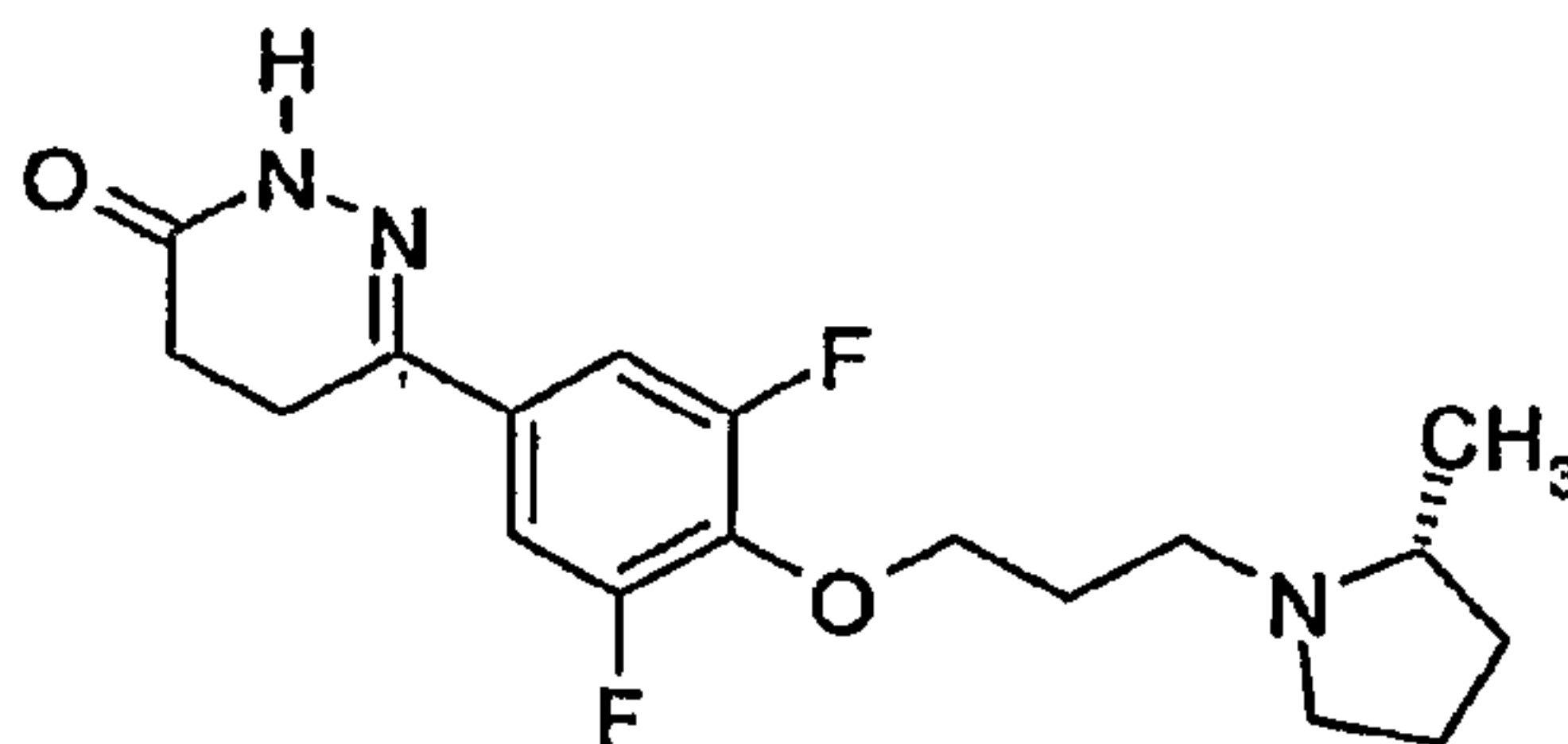
6-{3,5-Difluoro-4-[3-(( R )-2-methyl-pyrrolidin-1-yl)-propoxy]-phenyl}-4,5-dihydro-2H-pyridazin-3-one
