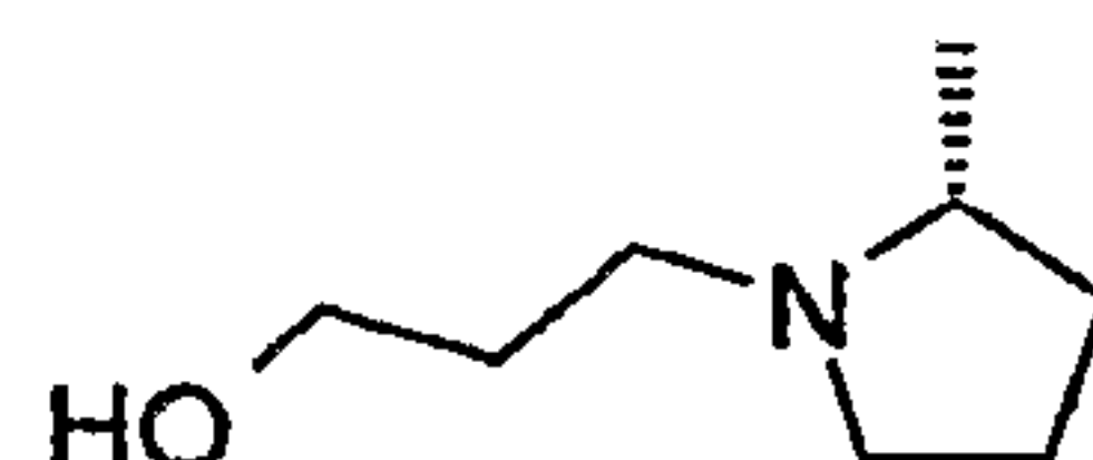
3-((R)-2-Methyl-pyrrolidin-1-yl)-propan-1-ol
