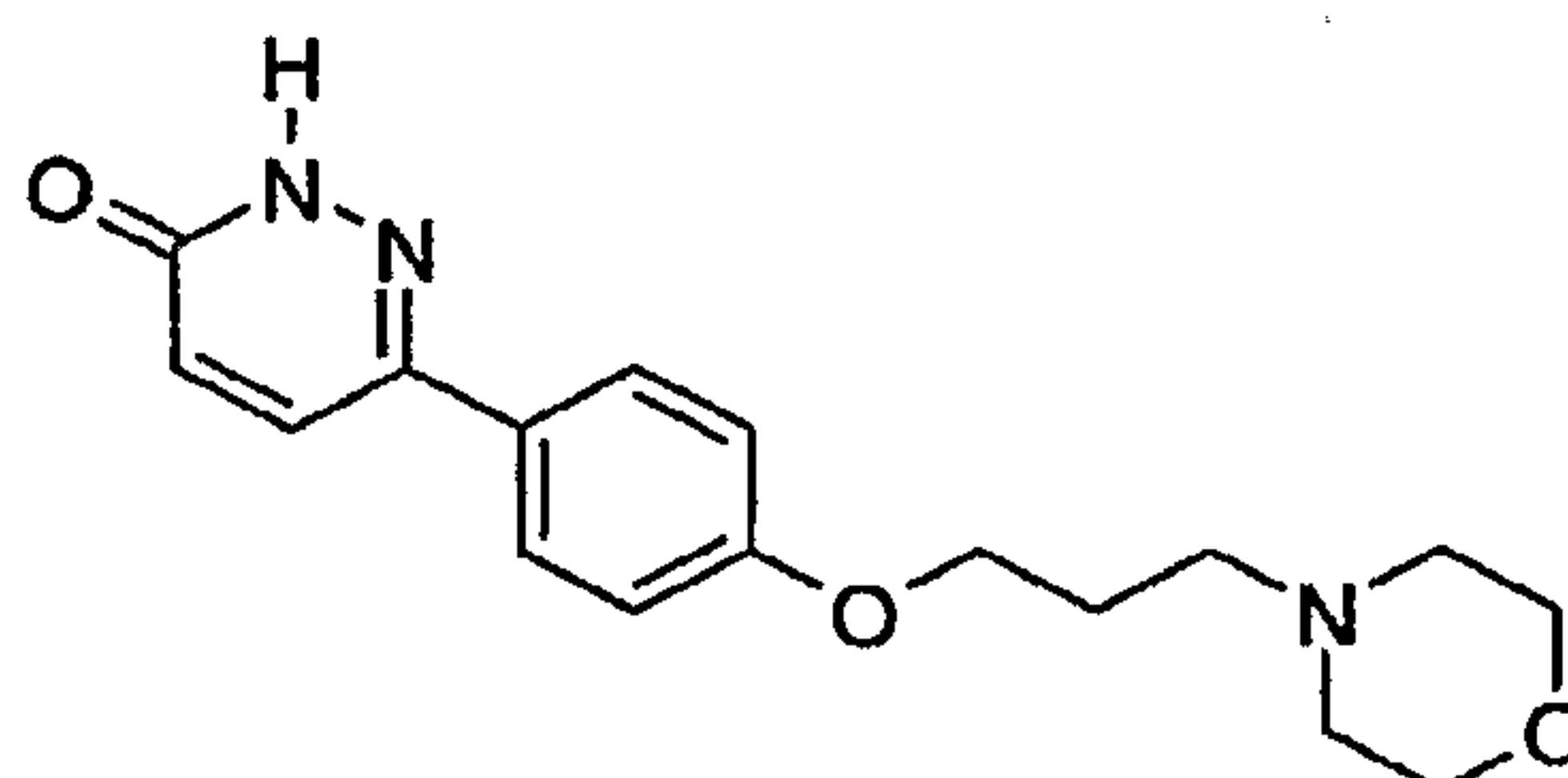
6-[4-(3-Morpholin-4-yl-propoxy)-phenyl]-2H-pyridazin-3-one
