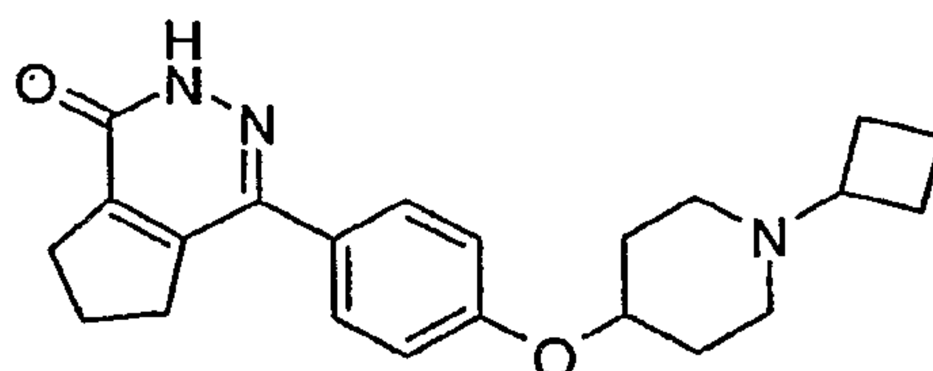
4-[4-(1-Cyclobutyl-piperidin-4-yloxy)-phenyl]-2,5,6,7-tetrahydro-cyclopenta[d]pyridazin-1-one
