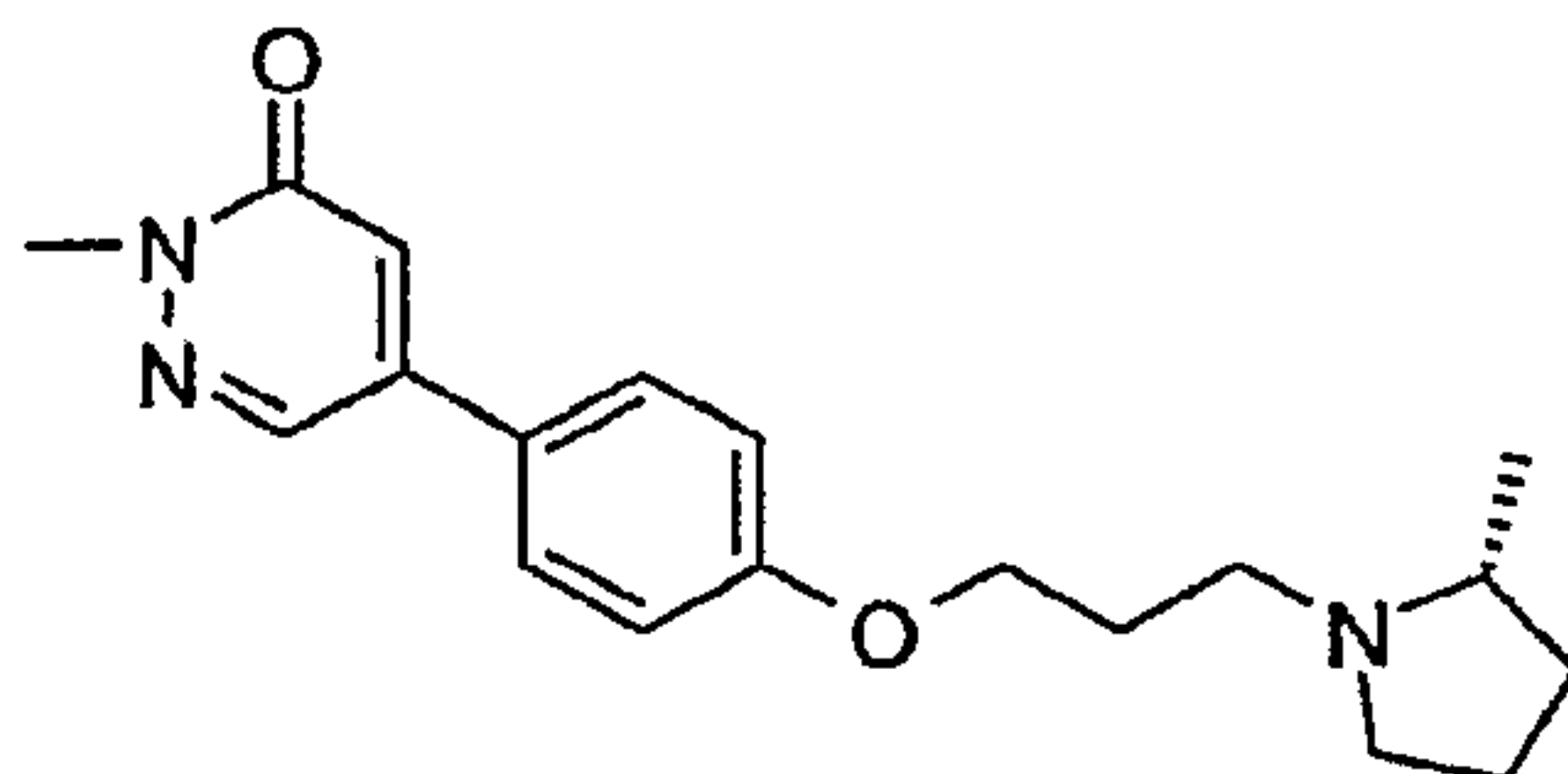
2-Methyl-5-{4-[3-((R)-2-methyl-pyrrolidin-1-yl)-propoxy]-phenyl}-2H-pyridazin-3-one
