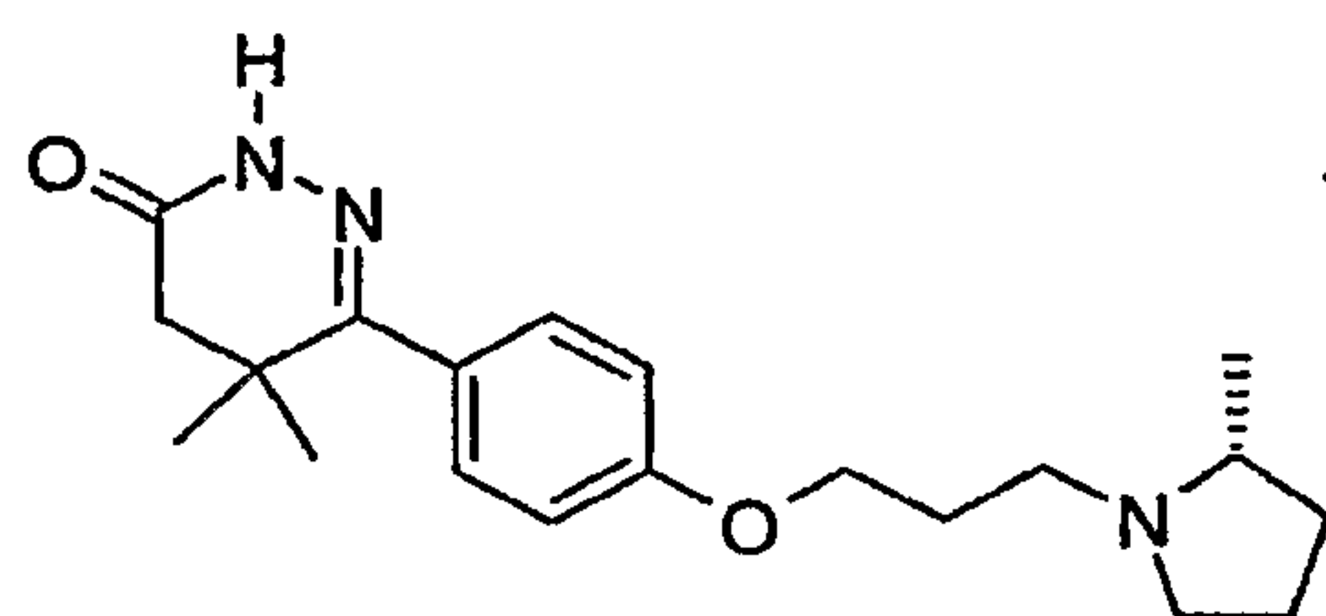
5,5-Dimethyl-6-{4-[3-((R)-2-methyl-pyrrolidin-1-yl)-propoxy]-phenyl}-4,5-dihydro-2H-pyridazin-3-one
