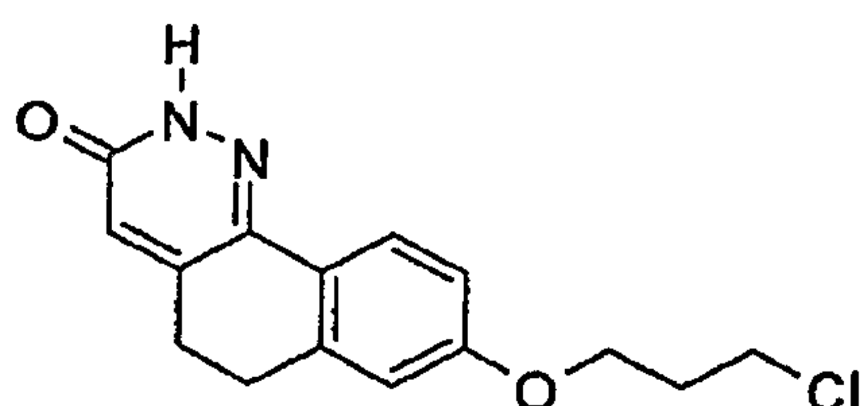
8-(3-Chloro-propoxy)-5,6-dihydro-2H-benzo[h]cinnolin-3-one
