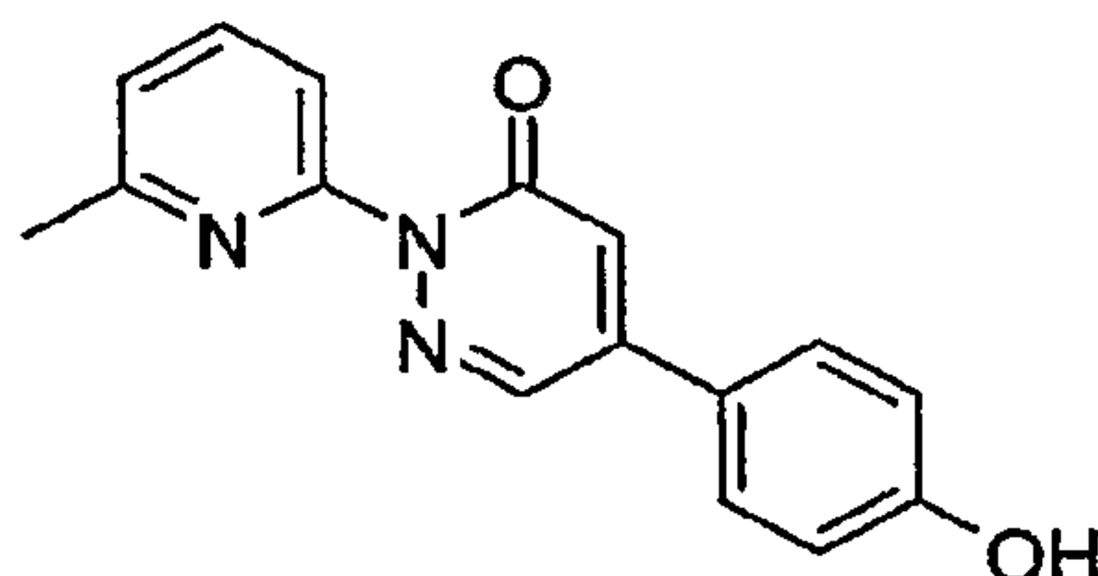
5-(4-Hydroxy-phenyl)-2-(6-methyl-pyridin-2-yl)-2H-pyridazin-3-one
