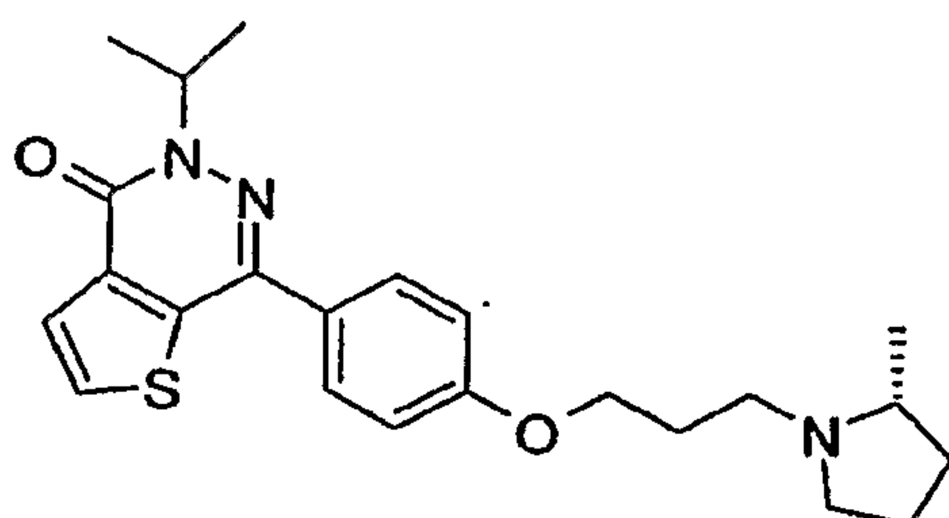
5-Isopropyl-7-{4-[3-((R)-2-methylpyrrolidin-1-yl)propoxy]-phenyl}-5H-thieno[2,3-d]pyridazin-4-one
