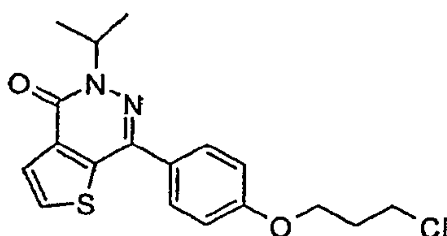
7-[4-(3-Chloro-propoxy)-phenyl]-5-isopropyl-5H-thieno[2,3-d]pyridazin-4-one
