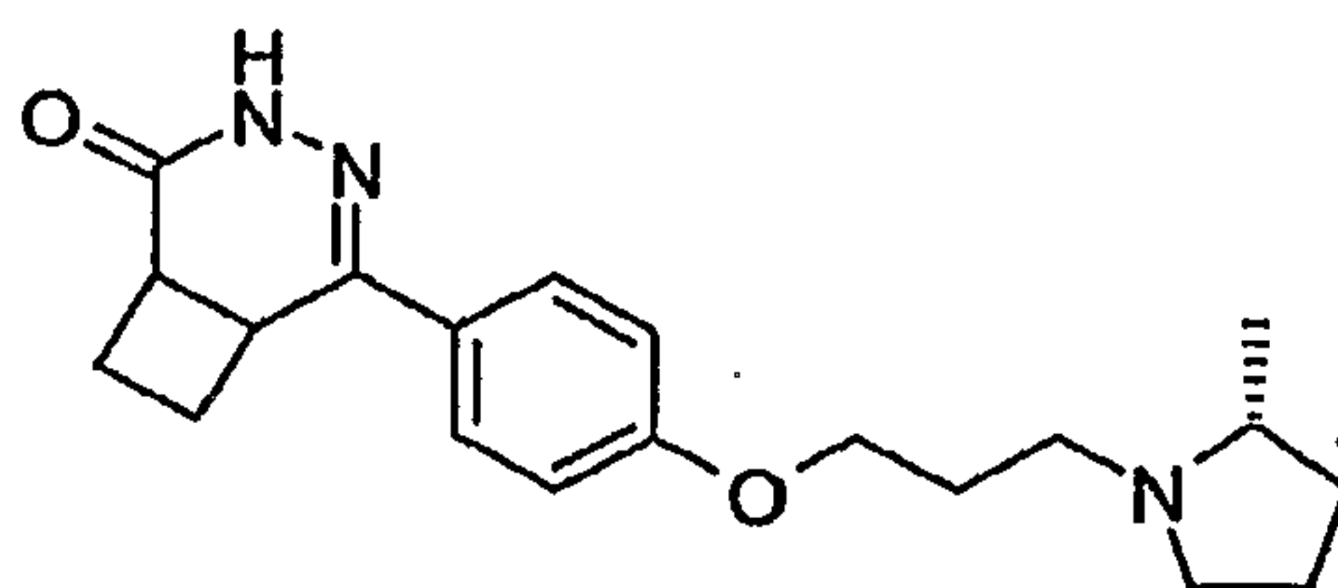
5-{4-[3-((R)-2-Methyl-pyrrolidin-1-yl)-propoxy]-phenyl}-3,4-diazabicyclo[4.2.0]oct-4-en-2-one
