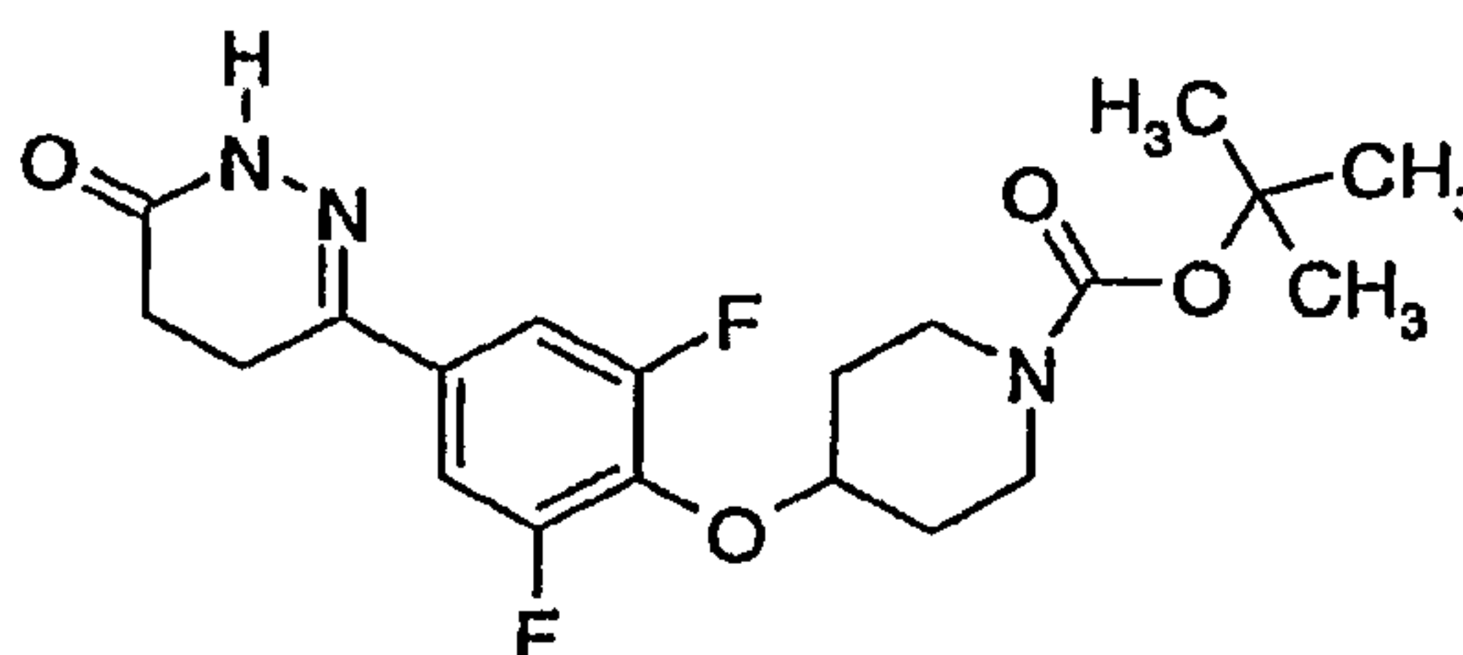
4-[2,6-Difluoro-4-(6-oxo-1,4,5,6-tetrahydro-pyridazin-3-yl)-phenoxy]-piperidine-1-carboxylic acid tert-butyl ester
