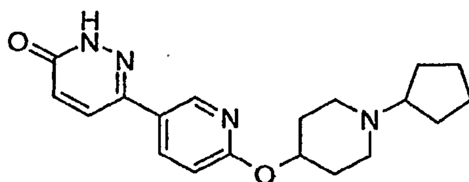
6-[6-(1-Cyclopentyl-piperidin-4-yloxy)-pyridin-3-yl]-2H-pyridazin-3-one
