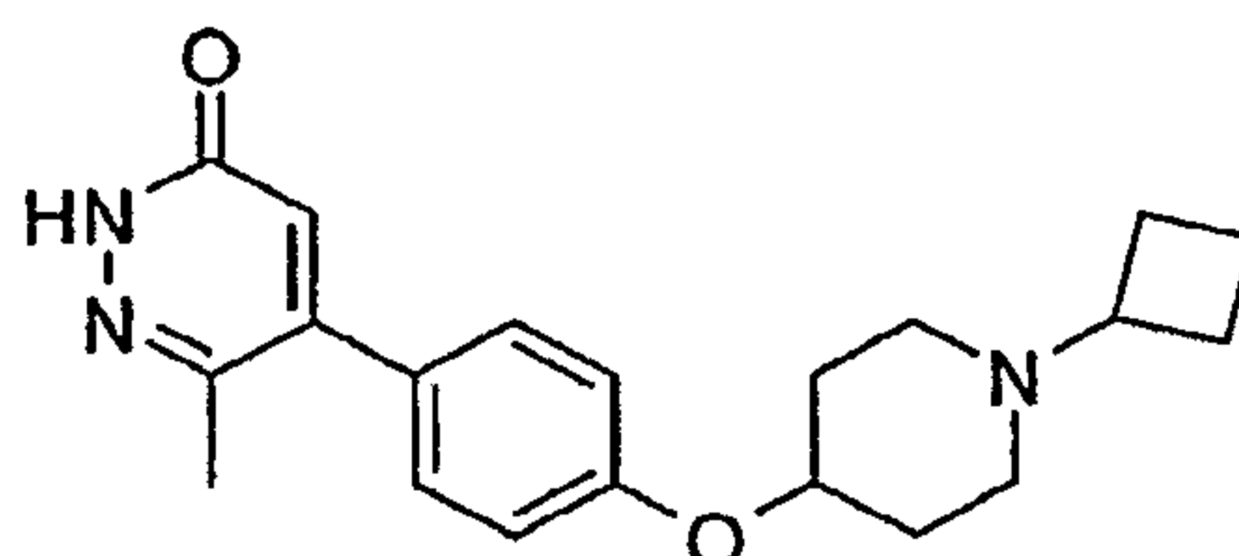
5-[4-(1-Cyclobutyl-piperidin-4-yloxy)-phenyl]-6-methyl-2H-pyridazin-3-one
