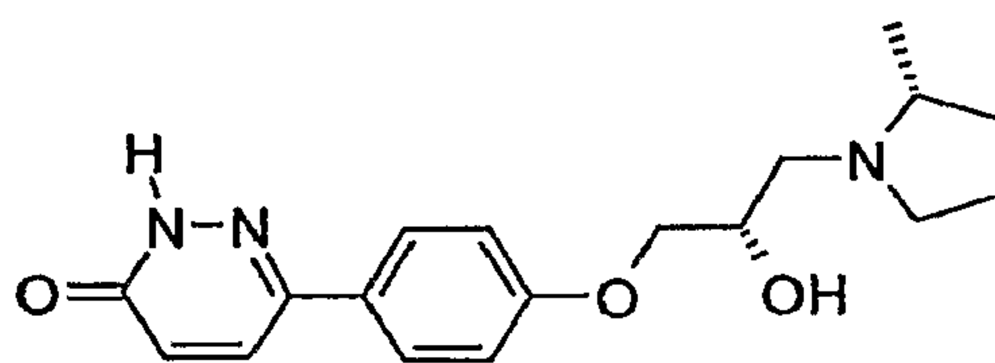
6-{4-[(S)-2-Hydroxy-3-((R)-2-methyl-pyrrolidin-1-yl)-propoxy]-phenyl}-2H-pyridazin-3-one
