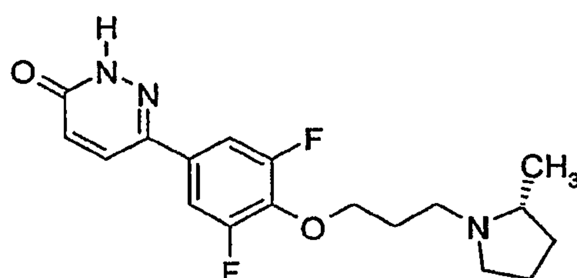
6-{3,5-Difluoro-4-[3-((R)-2-methylpyrrolidin-1-yl)-propoxy]-phenyl}-2H-pyridazin-3-one
