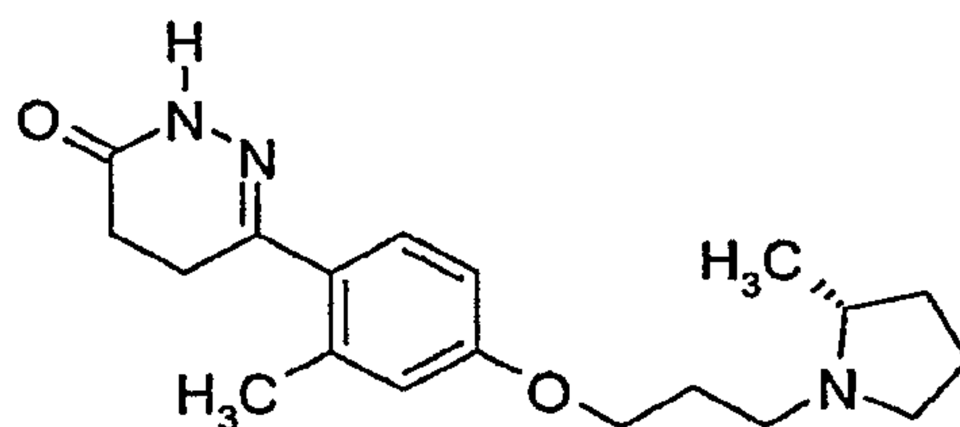
6-((R)-2-Methyl-4-[3-(2-methyl-pyrrolidin-1-yl)-propoxy]-phenyl)-4,5-dihydro-2H-pyriazin-3-one
