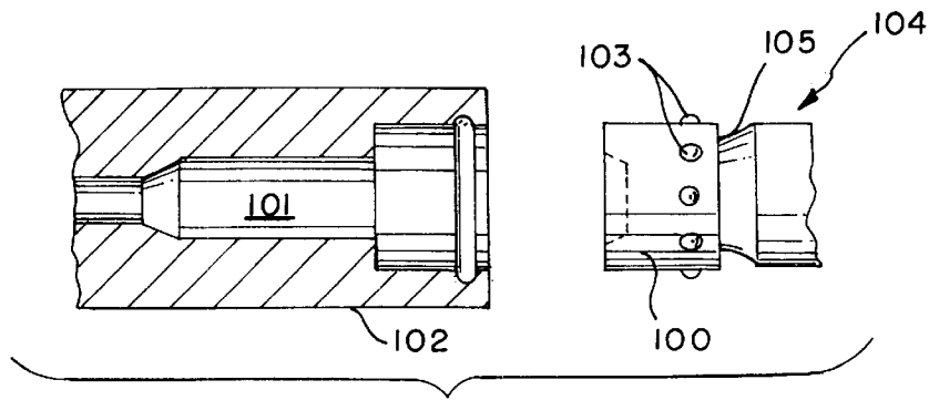
FIG. 11 BACKGROUND ART
