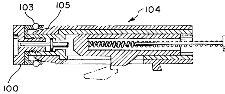
FIG. 10 BACKGROUND ART
