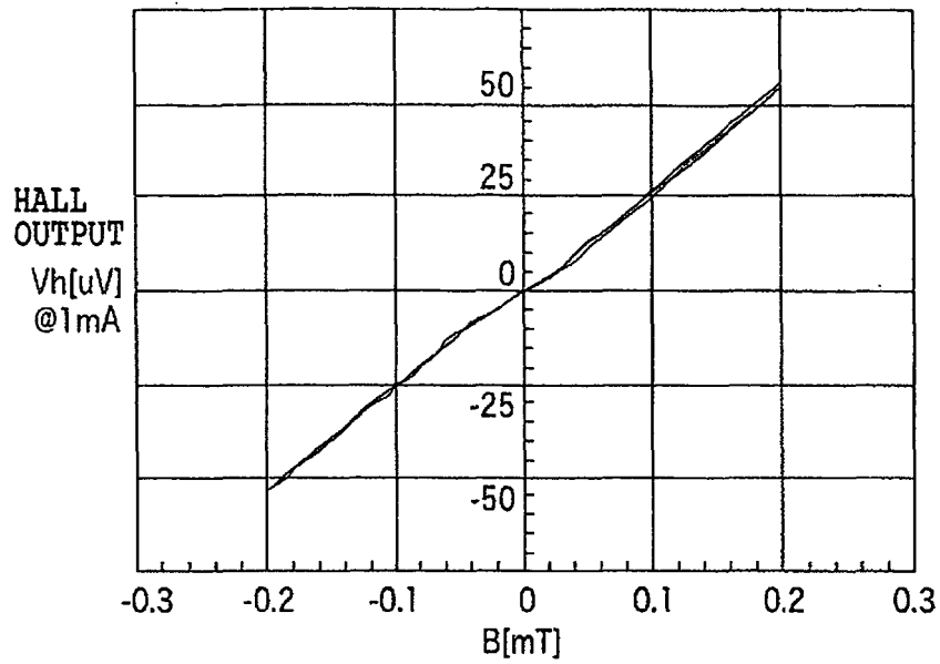
MAGNETIC CHARACTERISTICS OF HALL ELEMENT WHEN THERE IS STRAIN IN THE MAGNETIC SUBSTANCE
