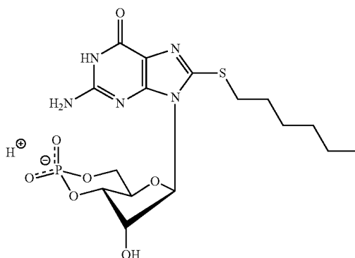
8-Hexylthioguanosine-3',5'-cyclic monophosphate (8-HT-cGMP)
