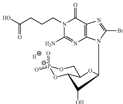
8-Bromo-1-(3-carboxypropyl)guanosine-3',5'-cyclic monophosphate (8-Br-1-CPr-cGMP)
