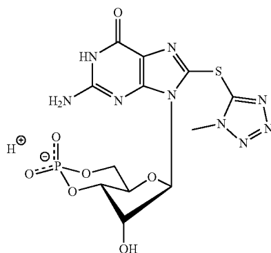
8-(5-(1-Methyl)tetrazolyl)thioguanosine-3',5'-cyclic monophosphate (8-(5-(1-Me)-Tet)T-cGMP)
