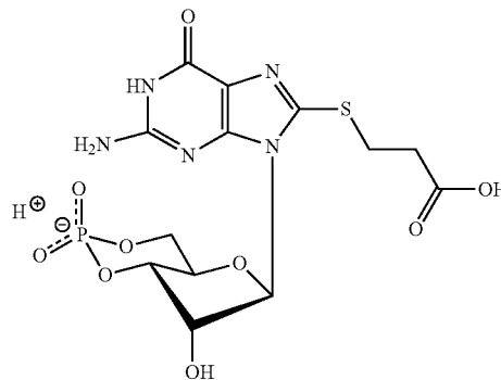
8-Carboxyethylthioguanosine-3', 5'-cyclic Monophosphate (8-CET-cGMP)
