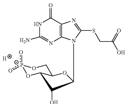
8-Carboxymethylthioguanosine-3', 5'-cyclic Monophosphate (8-CMT-cGMP)
