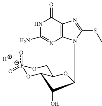
8-Methylthioguanosine-3', 5'-cyclic Monophosphate (8-MeS-cGMP)
