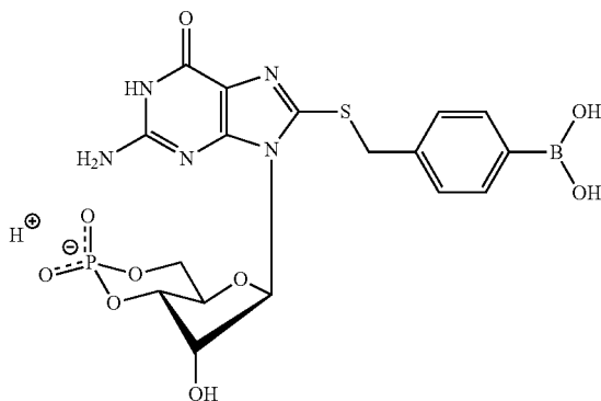
8-(4-Boronatebenzylthio)guanosine-3',5'-cyclic monophosphate (8-(pB(OH) 2 Bn)T-cGMP)
