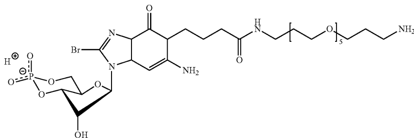
1-[Aminomethyl-(pentaethoxy)-propylamidopropyl]-8-bromoguanosine-3',5'-cyclic monophosphate (1-AM-(EO) 5 -PrAmdPr-8-Br-cGMP)
