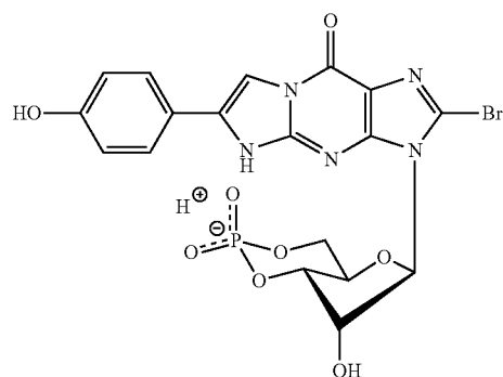
8-Bromo-(4-hydroxy-β-phenyl-1,N 2 -etheno)guanosine-3',5'-cyclic monophosphate (8-Br-pHPET-cGMP)
