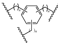
Trimeric Linkers
