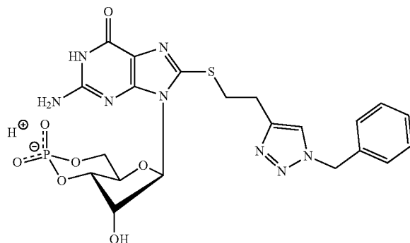
8-(2-(1-Benzyl-[1,2,3]-triazole-4-yl)-ethylthio)guanosine-3',5'-cyclic monophosphate (8-(1-Bn-[1,2,3]-Tz-4)-ET-cGMP)
