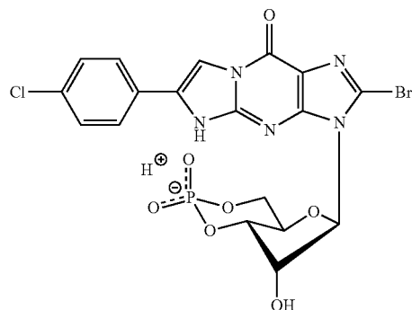
8-Bromo-(4-chloro-β-phenyl-1,N2-etheno)guanosine-3',5'-cyclic monophosphate (8-Br-pCl-PET-cGMP)
