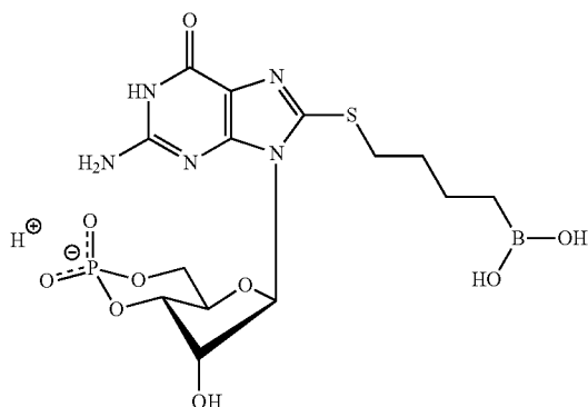
8-(4-Boronatebutylthio)guanosine-3',5'-cyclic monophosphate (8-(pB(OH) 2 Bu)T-cGMP)
