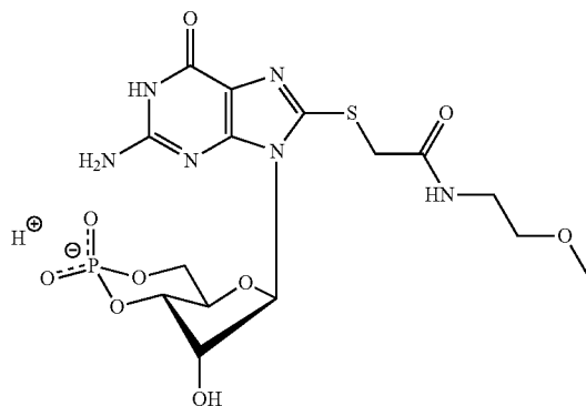
8-Methoxyethylamidomethylthio-guanosine-3',5'-cyclic monophosphate (8-MeOEAmMT-cGMP)
