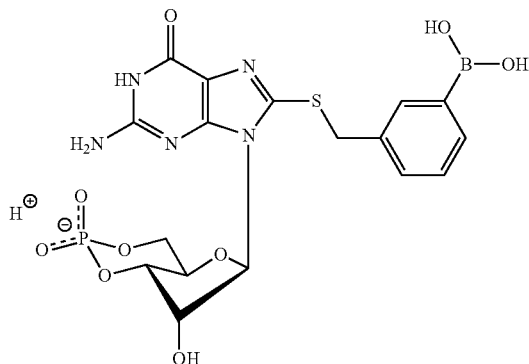
8-(3-Boronatebenzylthio)guanosine-3',5'-cyclic monophosphate (8-(mB(OH) 2 Bn)T-cGMP)
