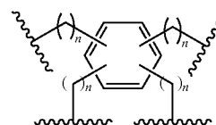
Tetrameric linkers
