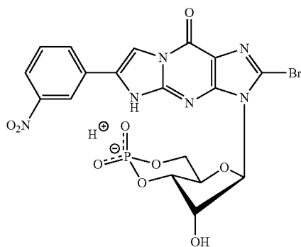
8-Bromo-(3-nitro-β-phenyl-1,N2-etheno)guanosine-3',5'-cyclic monophosphate (8-Br-mN-PET-cGMP)
