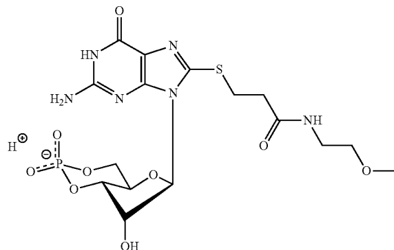
8-Methoxyethylamidoethylthio-guanosine-3',5'-cyclic monophosphate (8-MeOEAmEt-cGMP)
