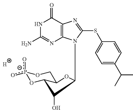
8-(4-Isopropylphenylthio)guanosine-3',5'-cyclic monophosphate (8-pIPrPT-cGMP)
