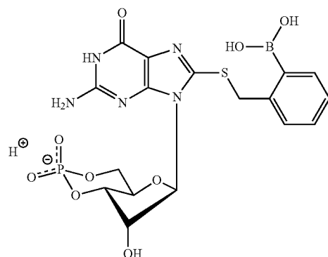
8-(2-Boronatebenzylthio)guanosine-3',5'-cyclic monophosphate (8-(oB(OH) 2 Bn)T-cGMP)
