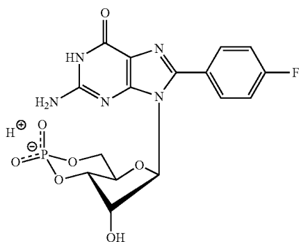
8-(4-Fluorophenyl)guanosine-3',5'-cyclic monophosphate (8-pFP-cGMP)
