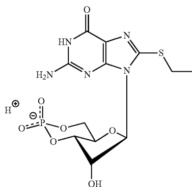
8-Ethylthioguanosine-3',5'-cyclic monophosphate (8-ET-cGMP)
