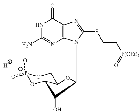
8-Diethylphosphonoethylthio-guanosine-3',5'-cyclic monophosphate (8-DEPET-cGMP)
