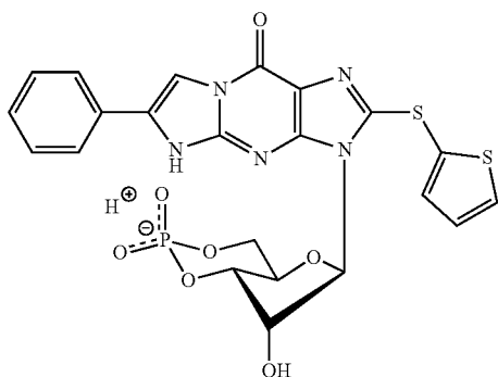
\beta -Phenyl-1,N 2 -etheno-8-(2-thiophenyl)thioguanosine-3',5'-cyclic monophosphate (PET-8-(2-Tp)T-cGMP)
