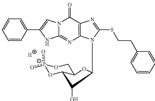
\beta -Phenyl-1,N 2 -etheno-8-(2-phenylethyl)thioguanosine-3',5'-cyclic monophosphate (PET-8-PhEtT-cGMP)
