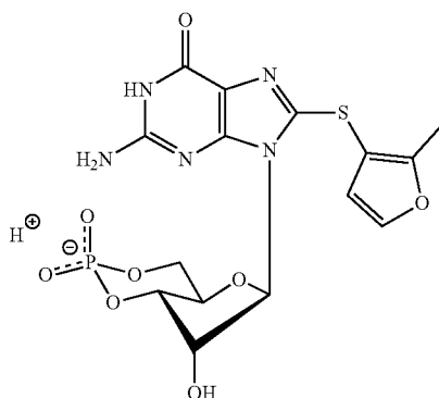
8-(3-(2-Methyl)furanyl)thioguanosine-3',5'-cyclic monophosphate (8-(3-(2-Me)-FU)T-cGMP)
