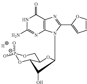
8-(2-Furyl)guanosine-3',5'-cyclic monophosphate (8-(2-Fur)-cGMP)
