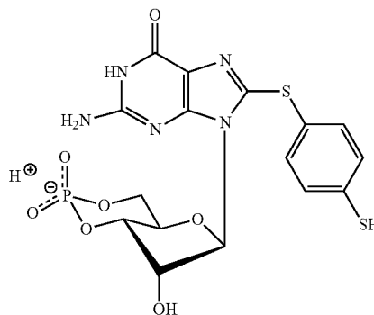
8-(4-Thiophenylthio)guanosine-3', 5'-cyclic Monophosphate (8-pTPT-cGMP)
