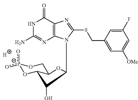
8-(3-Fluoro-5-methoxybenzylthio)guanosine-3',5'-cyclic monophosphate (8-(3-F-5- MeO)BT-cGMP)
