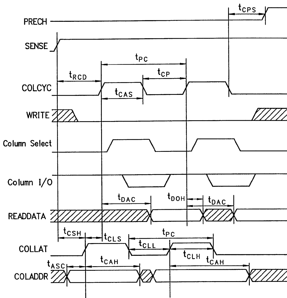
FIG. 5 (Prior Art)
