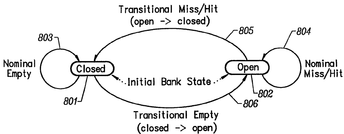
FIG. 8 (Prior Art)
