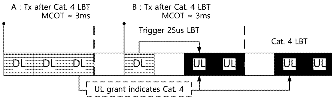
(b) Receive Cat. 4 LBT signaling by signaling of UL grant, and signaling related change of LBT type through recent DL
