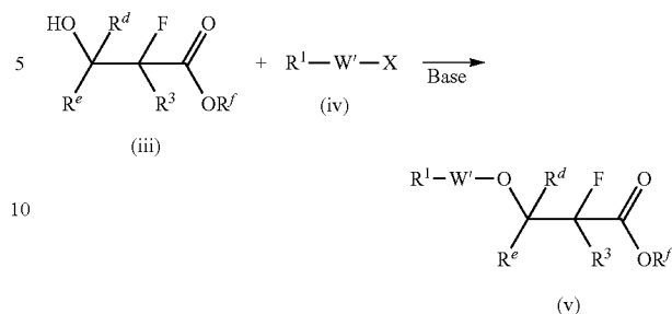
Reaction Formula (2)
