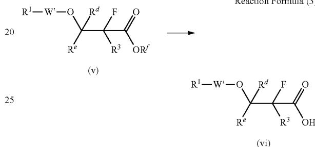
Reaction Formula (3)
