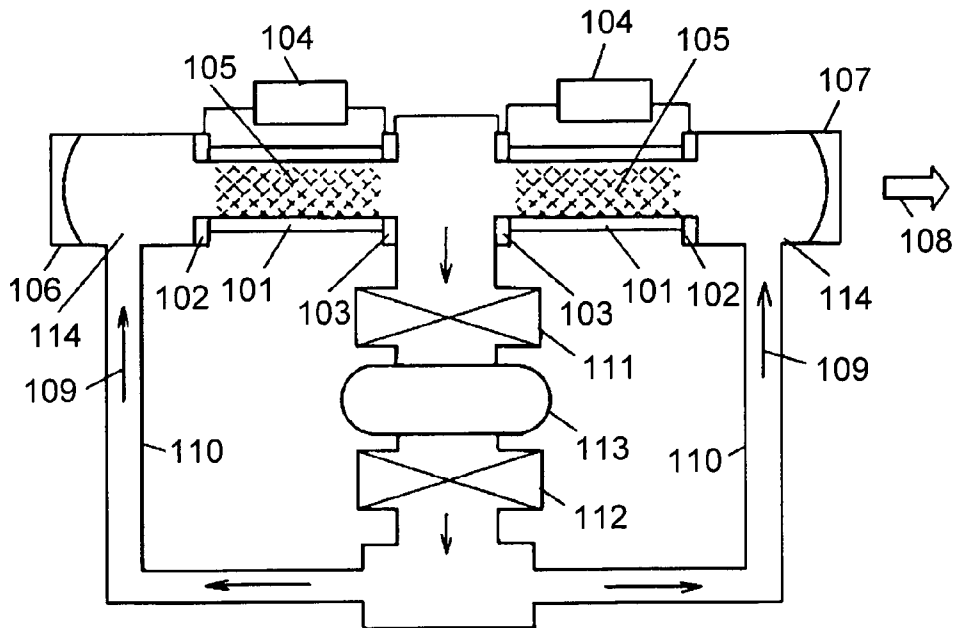
FIG. 12 – PRIOR ART
