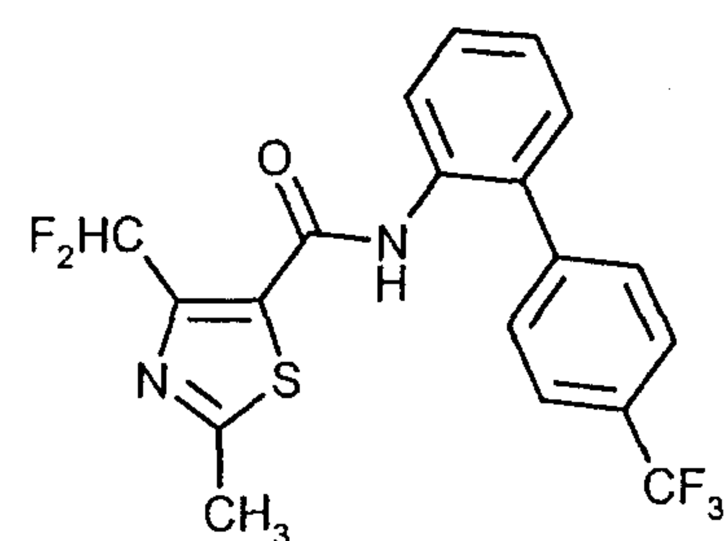
(24-8) 4-(difluoromethyl)-2-methyl- N -[4'-(trifluoromethyl)-1,1'-biphenyl-2-yl]-1,3-thiazole-5-carboxamide (known from WO 03/066610) of the formula
