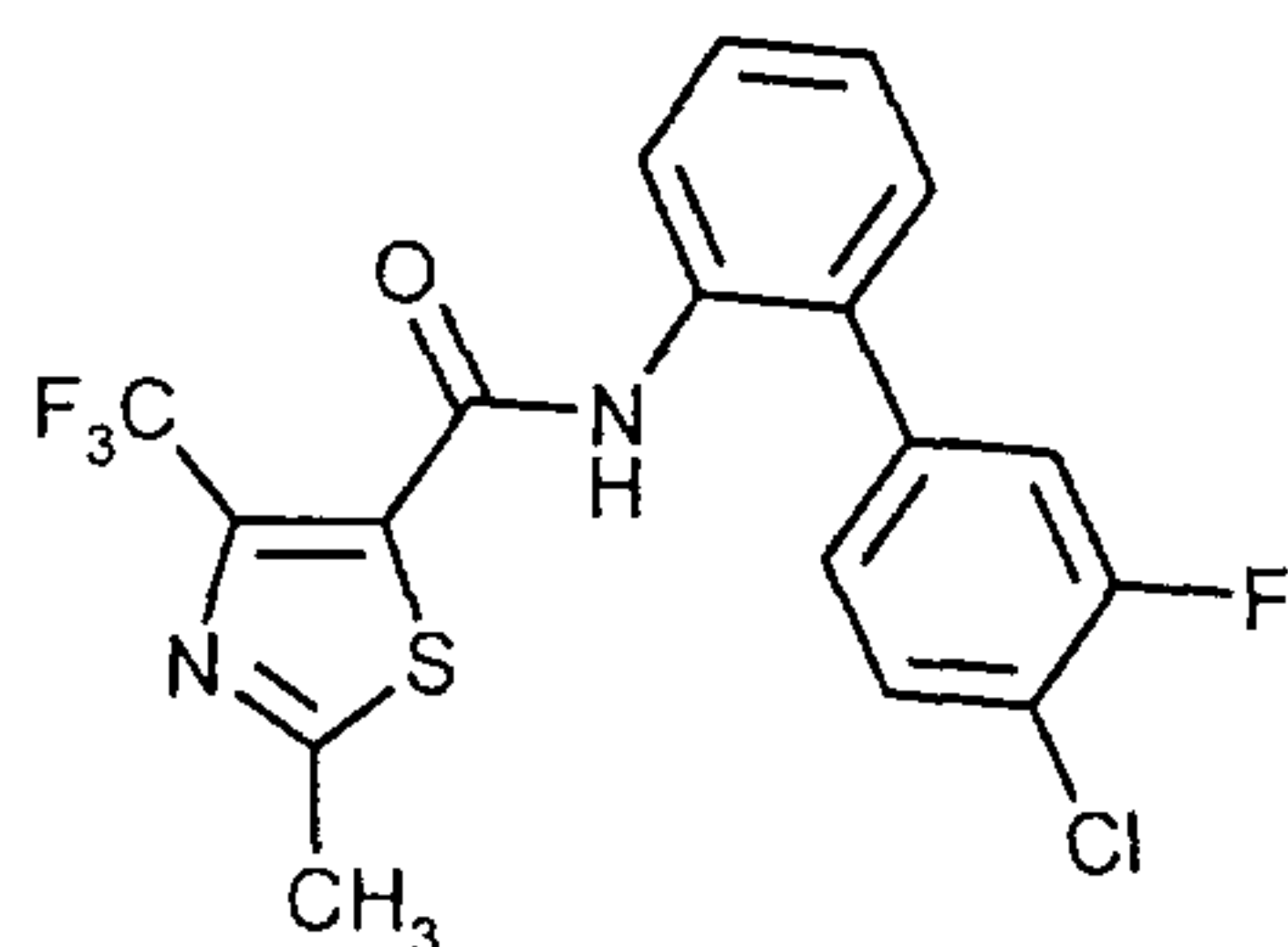
(24-6) N -(4'-chloro-1,1'-biphenyl-2-yl)-4-(difluoromethyl)-2-methyl-1,3-thiazole-5-carboxamide (known from WO 03/066610) of the formula
