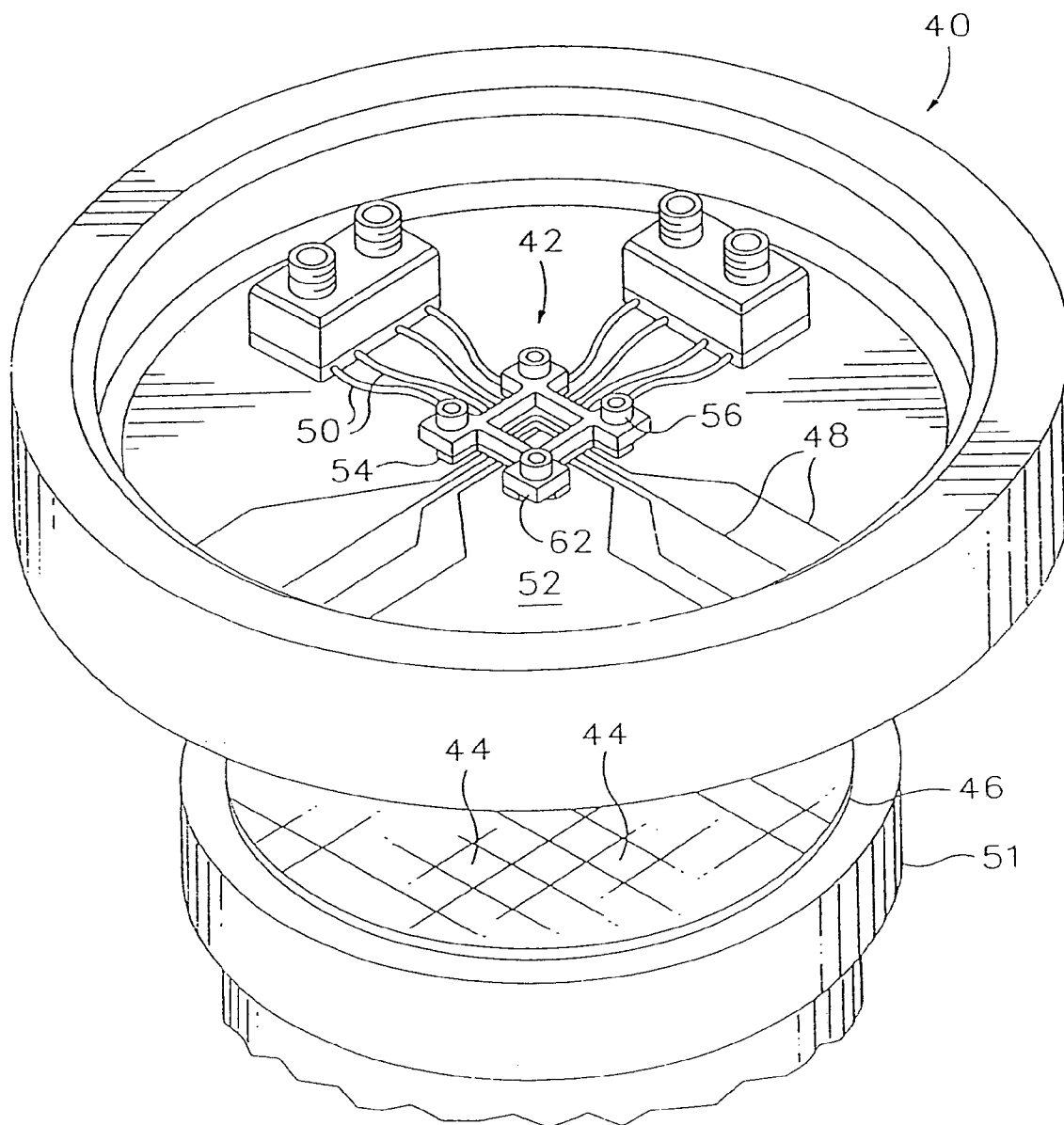
FIG.1 PRIOR ART
