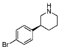
(S)-3-(4-bromophenyl)piperidine
