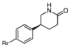
(S)-5-(4-bromophenyl)piperidin-2-one
