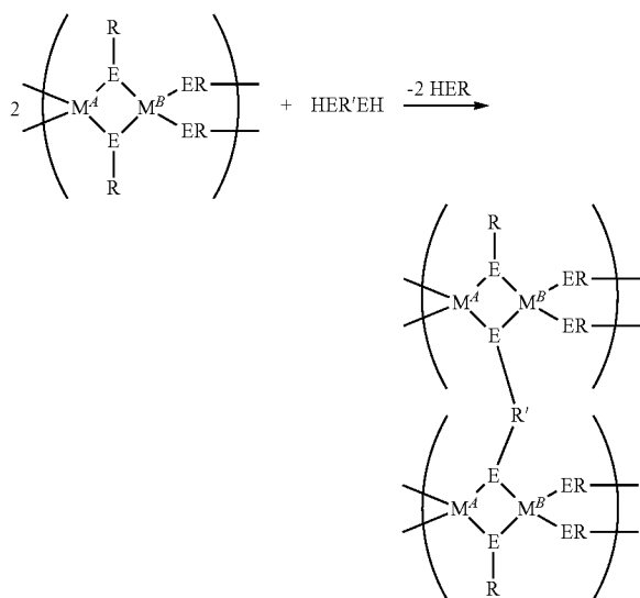
REACTION SCHEME 14
