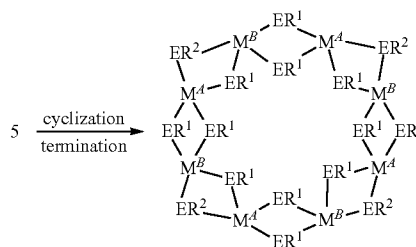
REACTION SCHEME 7:
