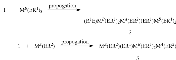
REACTION SCHEME 2:
