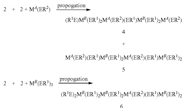
REACTION SCHEME 3:
