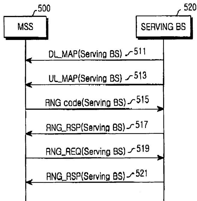
FIG.5 (PRIOR ART)
