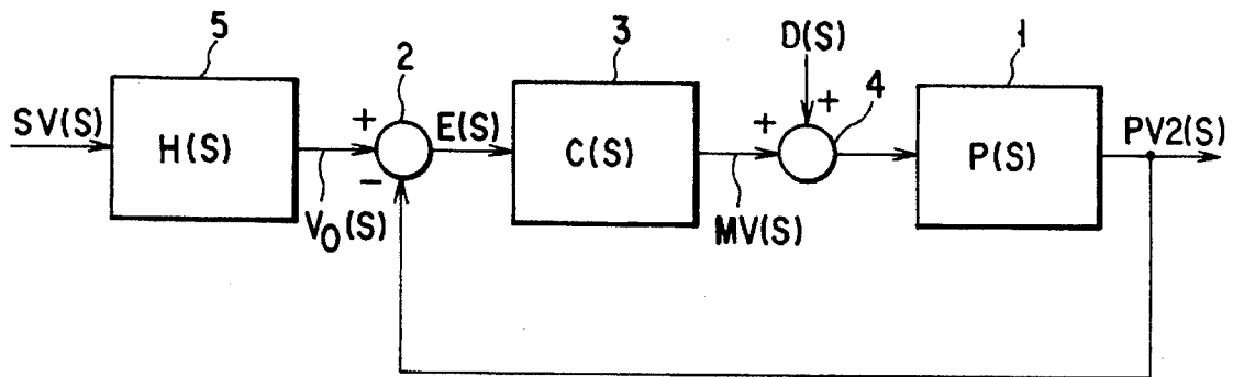
FIG. 2 (PRIOR ART)
