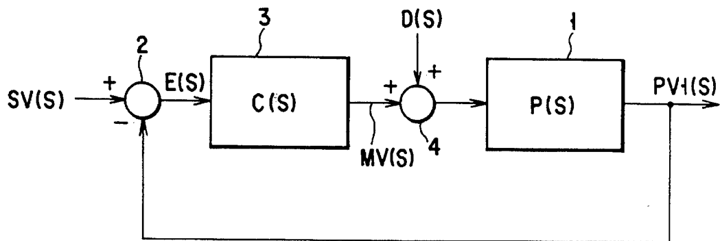
FIG. 1 (PRIOR ART)
