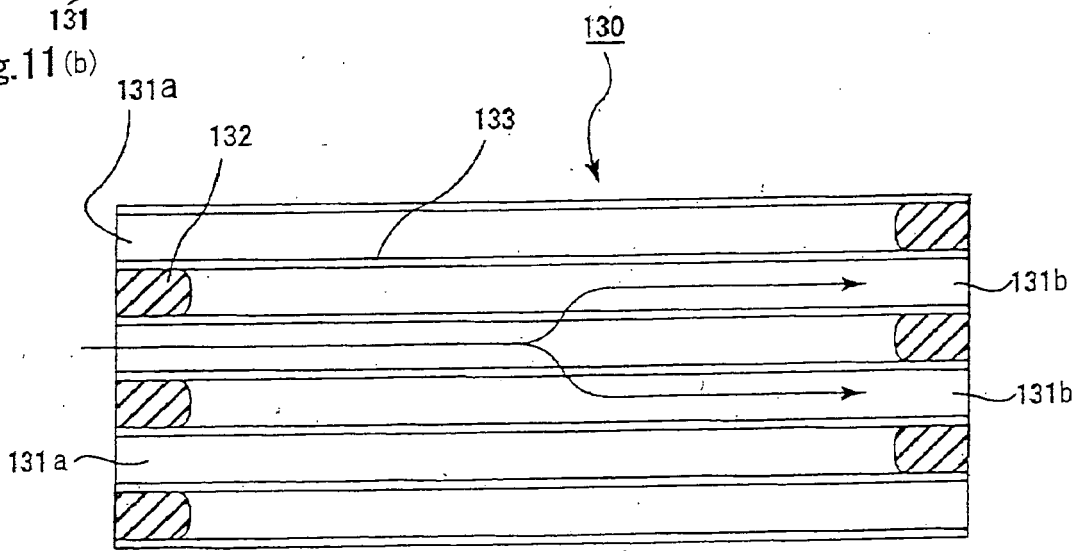
Section at C-C line
