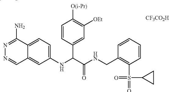
134A: 4-Bromo-N-diethylbenzamide
