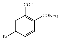
134B: 4-Bromo-N,N-diethyl-2-formylbenzamide
