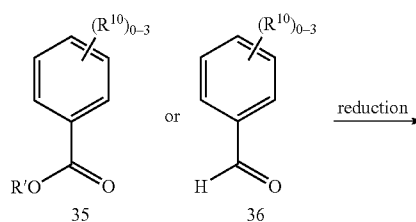
Scheme 9
