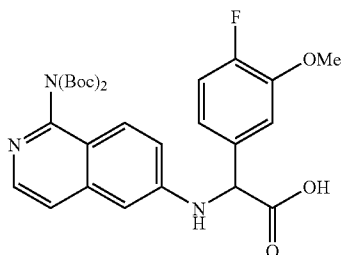
69C: 2-(1-di-tert-Butoxycarbonylaminoisoquinolin-6-ylamino)-2-(4-fluoro-3-methoxyphenyl)acetic acid
