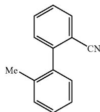
175A: 2-(o-Tolyl)benzonitrile
