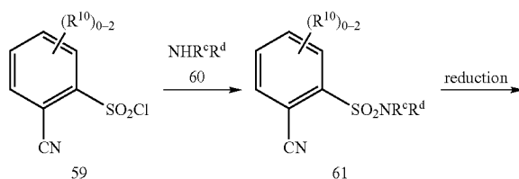
Scheme 18
