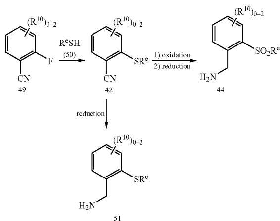
Scheme 15
