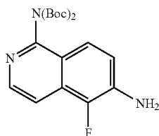
261A: 5-Fluoro-6-Amino-1-di-tert-butoxycarbonylaminoisoquinoline
