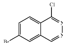
134E: 6-Bromo-1-chlorophthalazine
