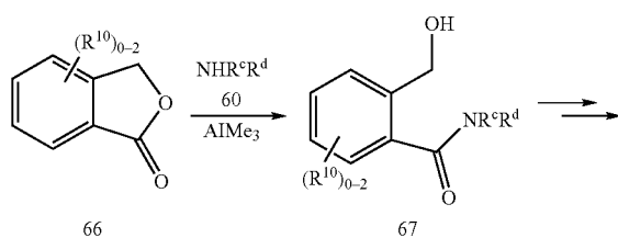
Scheme 20
