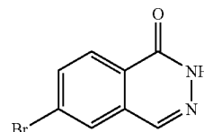
134D: 6-Bromophthalazin-1(2H)-one
