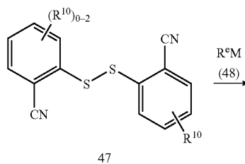
Scheme 14
