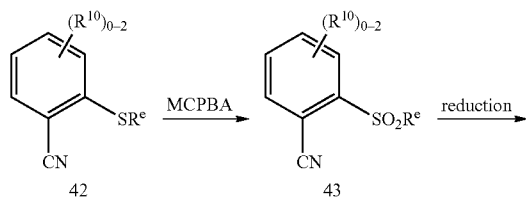
Scheme 12
