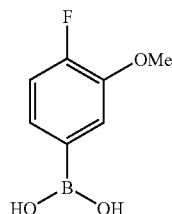
69B: 3-Methoxy-4-fluorophenylboronic acid
