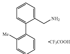
175B: 2-(o-Tolyl)benzylamine trifluoroacetic acid salt
