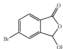
134C: 5-Bromo-3-hydroxyisobenzofuran-1(3H)-one
