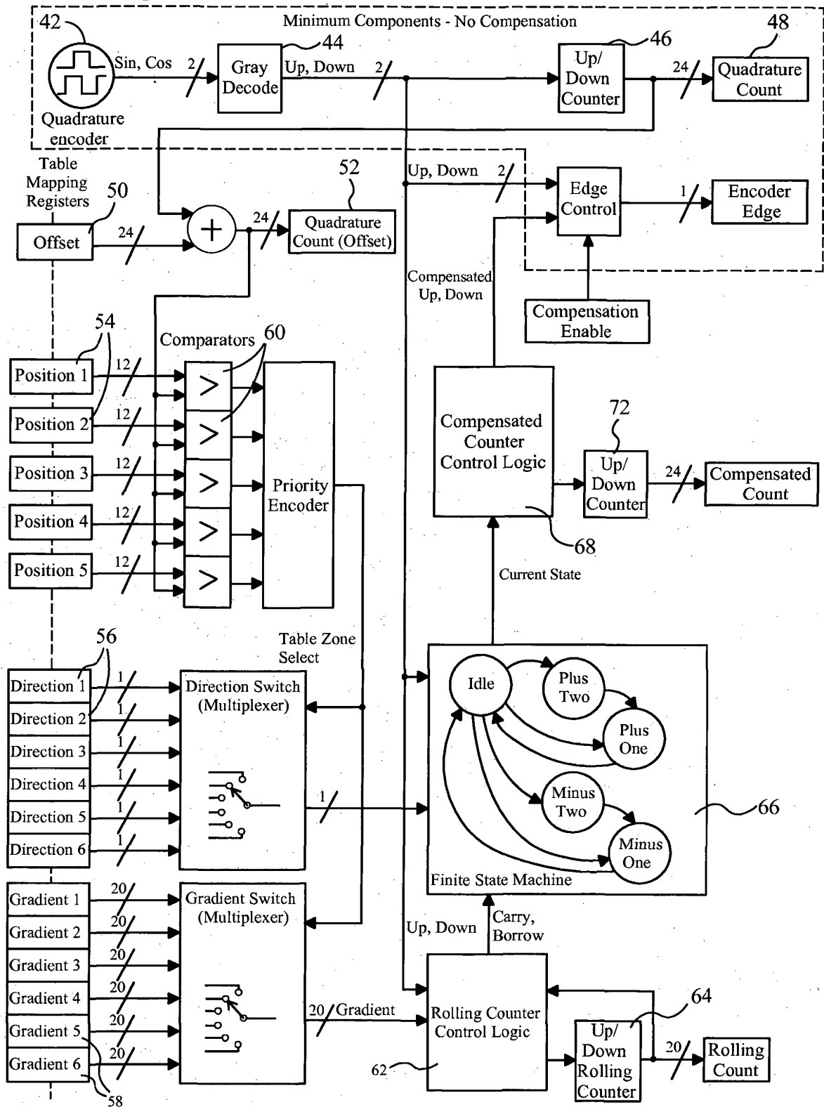
Fig. 2 Encoder Compensation Scheme
