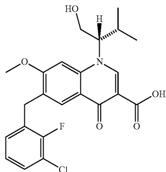
Compound 10, \gamma -form C 23 H 23 ClFNO 5 Mol. Wt.: 447.88
