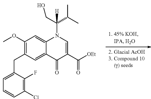
Compound 9a C 25 H 27 ClFNO 5 Mol. Wt.: 475.94
