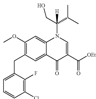
Compound 9a C 25 H 27 ClFNO 5 Mol. Wt.: 475.94
