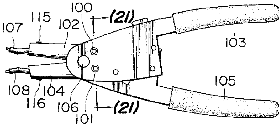
FIG. 20 PRIOR ART
