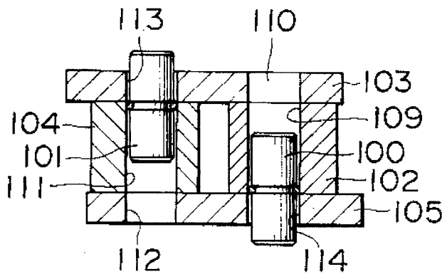
FIG. 21 PRIOR ART
