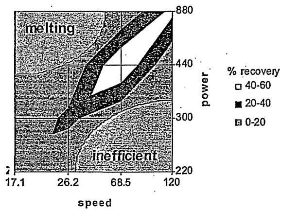
Figure 4 Determining Optimum Power and Speed of Industrial Microwave Unit
