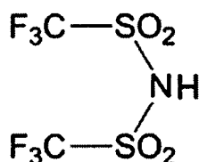
Structural Formula (B)
