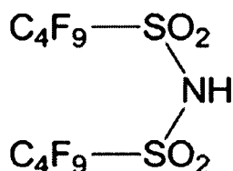
Structural Formula (C)
