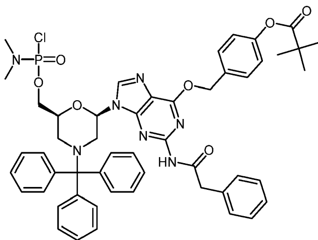
Compound (E1)
