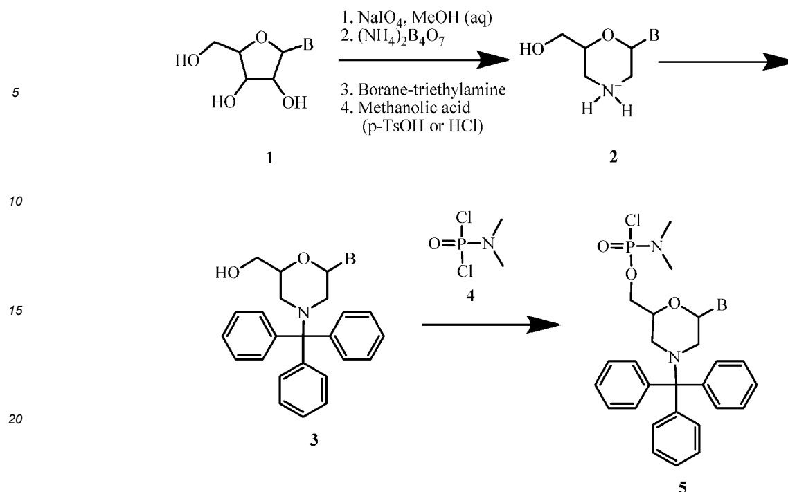
Scheme 1: General synthetic route to PMO Subunits
