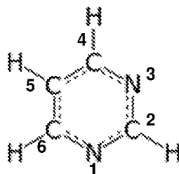
Pyrimidine
