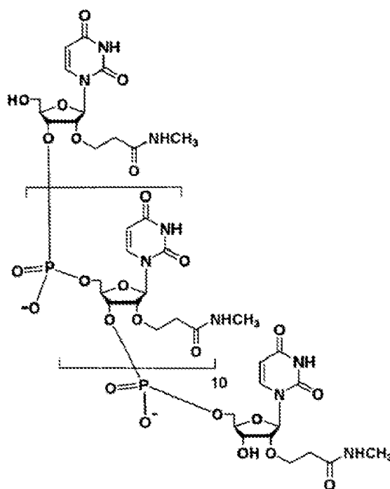
MCE
