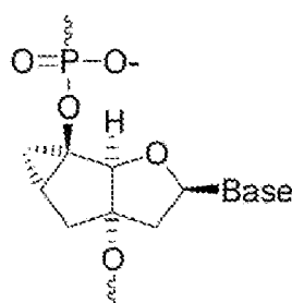
tricyclo-DNA
