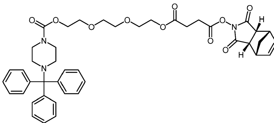
Compound (B)
