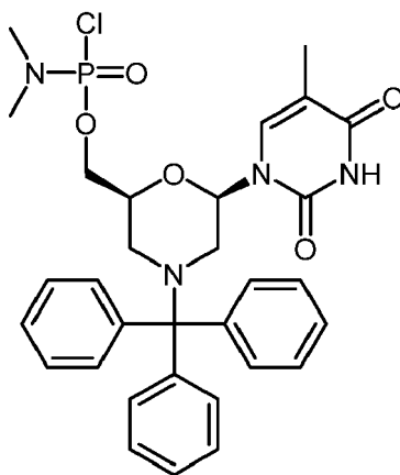
Compound (G1)
