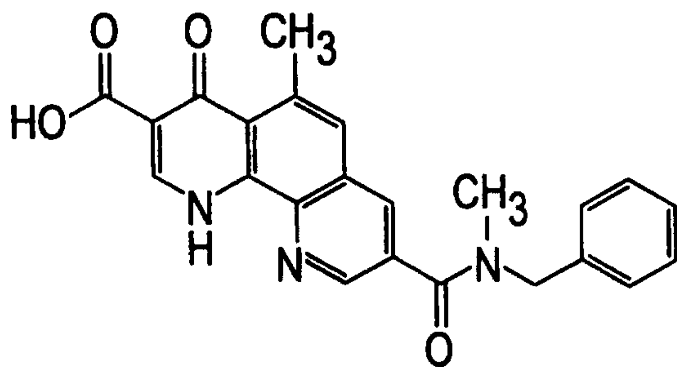
COMPOUND 5 3-Carboxy-8-(N-benzyl-N-methylcarbamoyl)- 5-methyl-4-oxo-3,4-dihydro-1,10-phenanthroline
