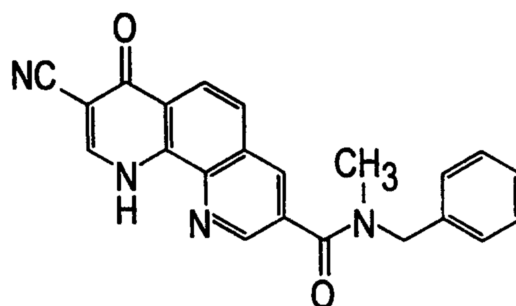
COMPOUND 4 3-Cyano-8-(N-benzyl-N-methylcarbamoyl)- 4-oxo-3,4-dihydro-1,10-phenanthroline
