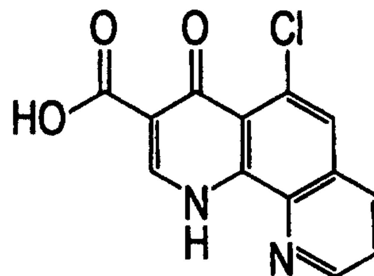
COMPOUND 2 5-Chloro-3-carboxy-4-oxo 3,4-dihydro-1,10-phenanthroline
