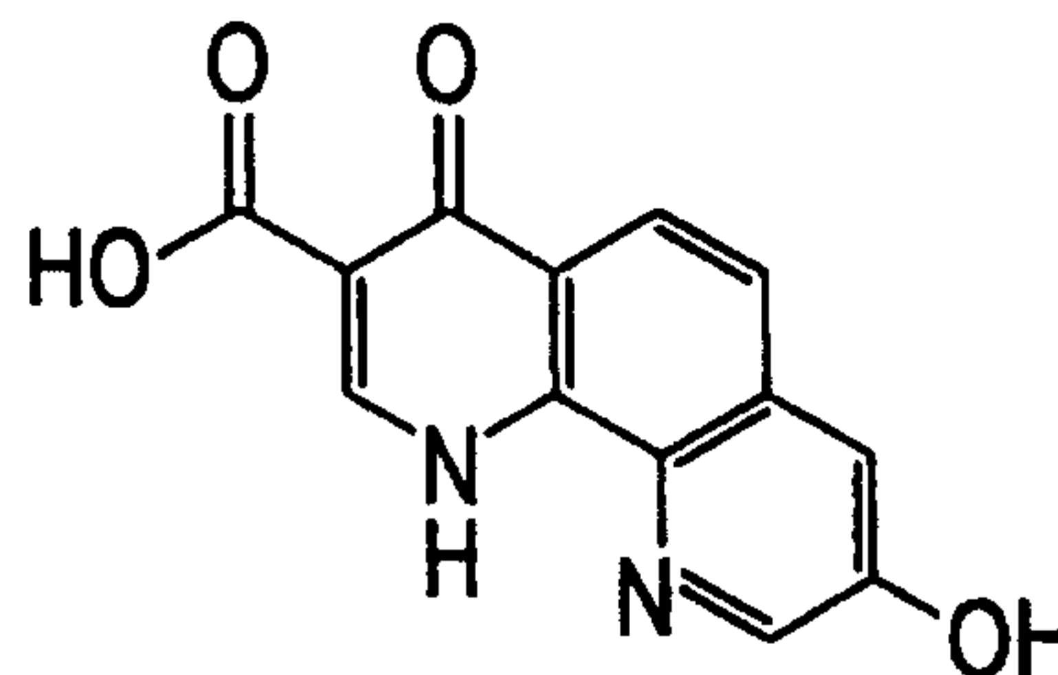
COMPOUND 7 3-Carboxy-8-hydroxy-4-oxo 3,4-dihydro-1,10-phenanthroline
