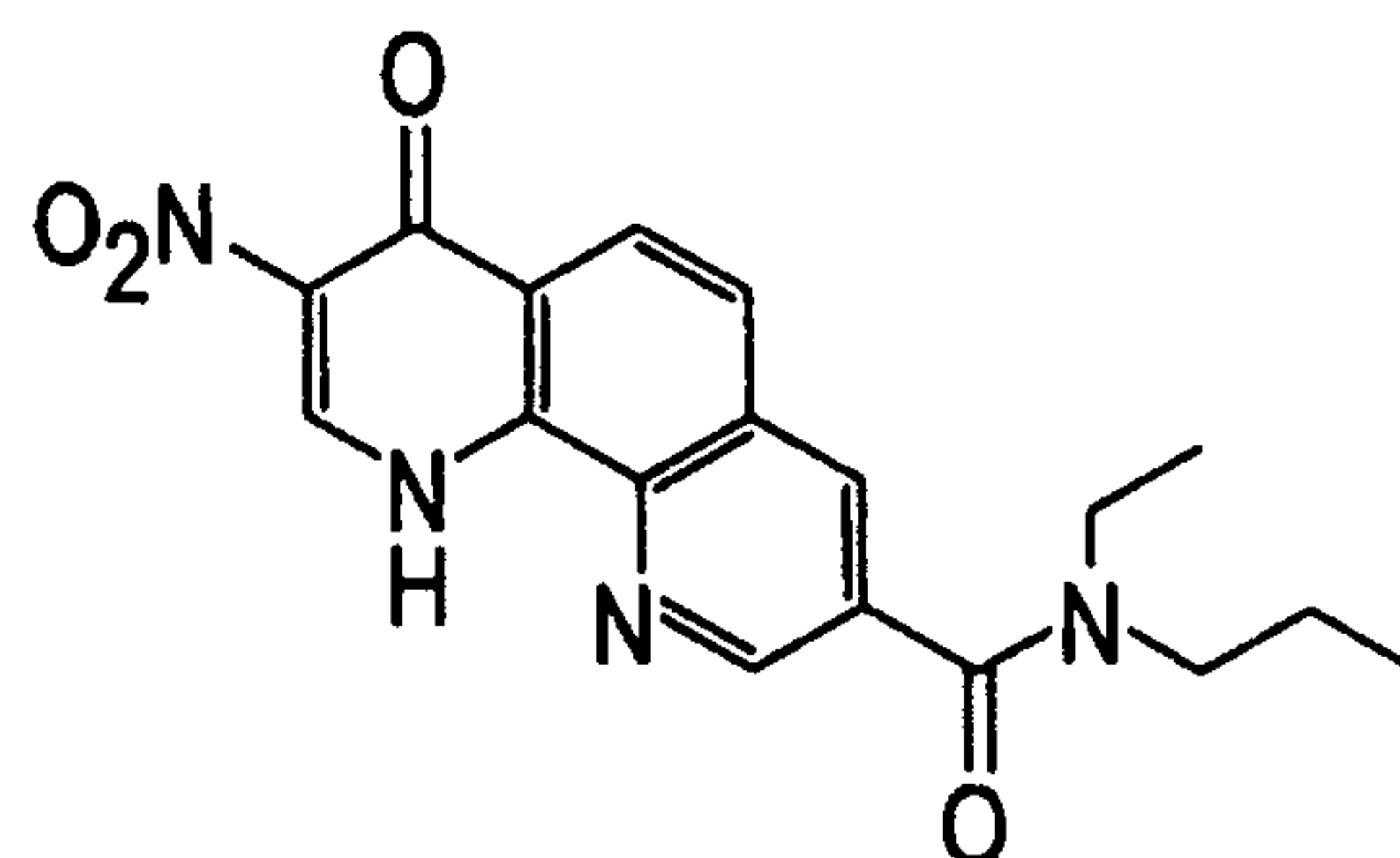
COMPOUND 6 3-Nitro-8-(N-ethyl-N-propylcarbamoyl)-4- oxo-3,4-dihydro-1,10-phenanthroline
