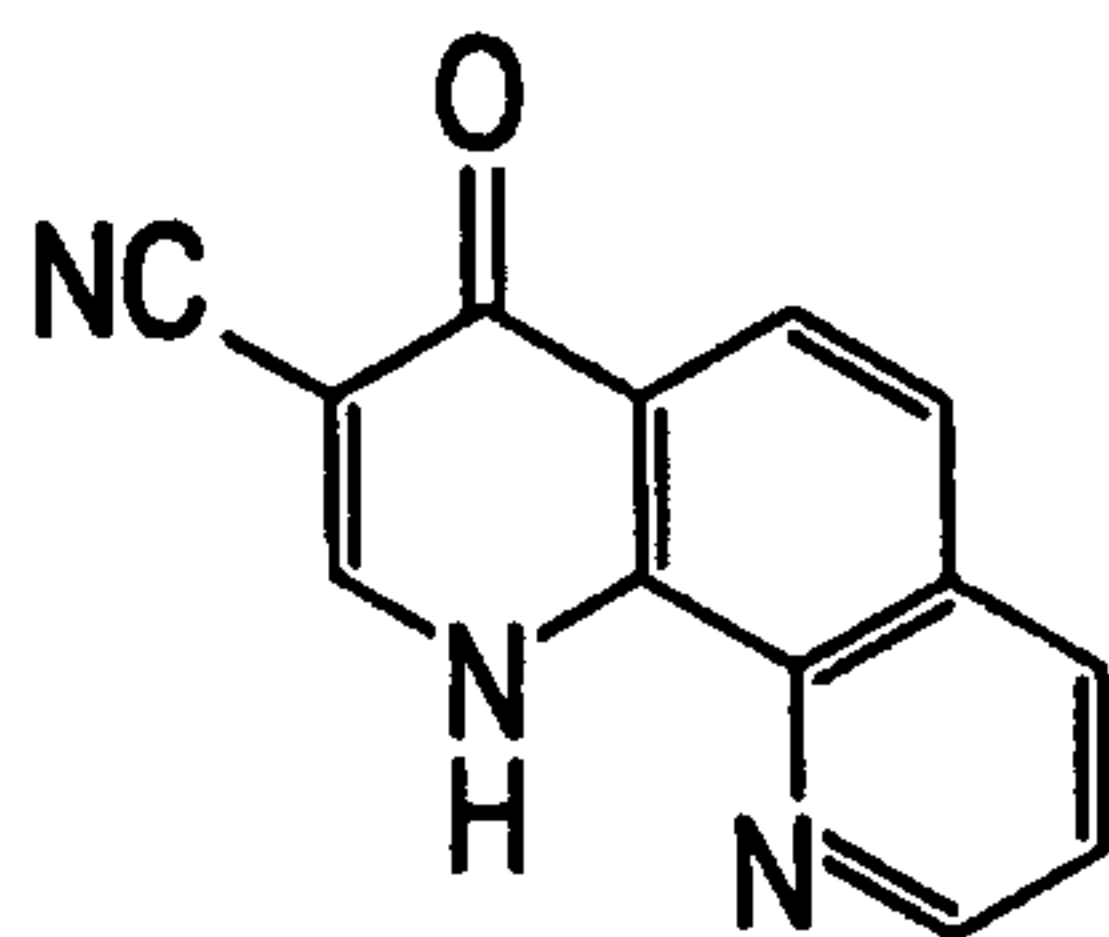
COMPOUND 1 3-Cyano-4-oxo-3,4-dihydro- 1,10-phenanthroline
