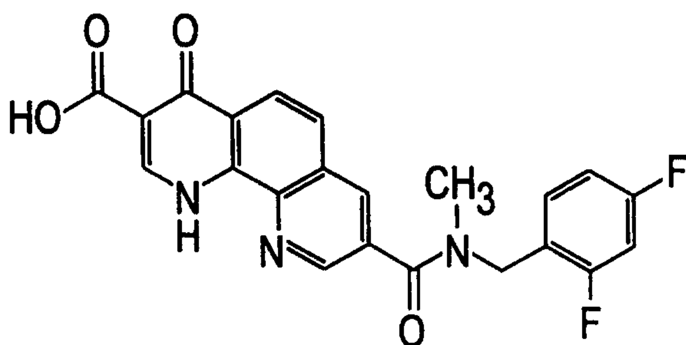
COMPOUND 3 3-Carboxy-8-(N-methyl-N-(2,4-difluorobenzyl)- carbamoyl)-4-oxo-3,4-dihydro-1,10-phenanthroline
