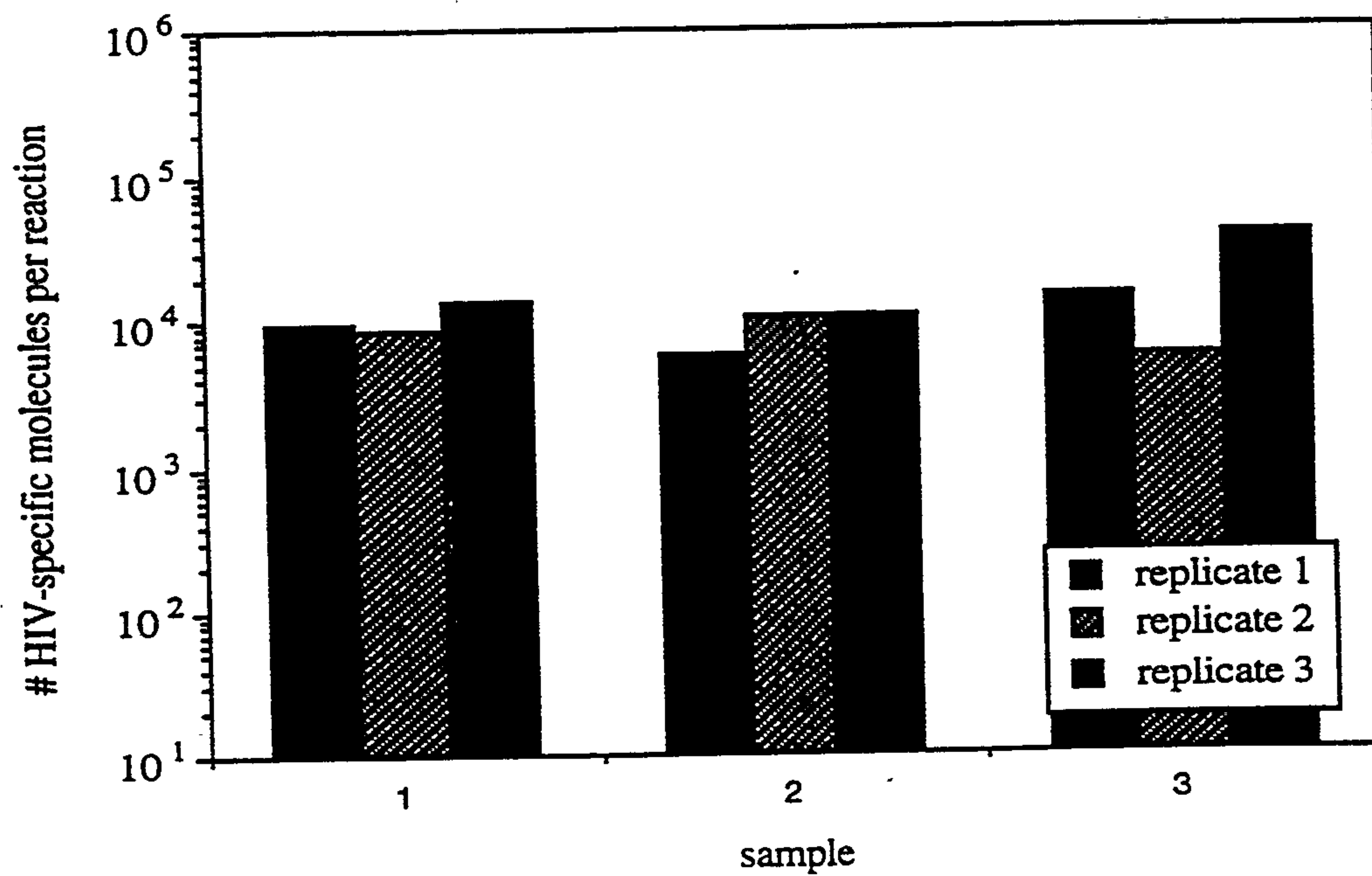
Figure 5c. Determination of number of HIV-specific RNA molecules per poly dT-selected HIV-1 lysate, 1:10 dilution.
