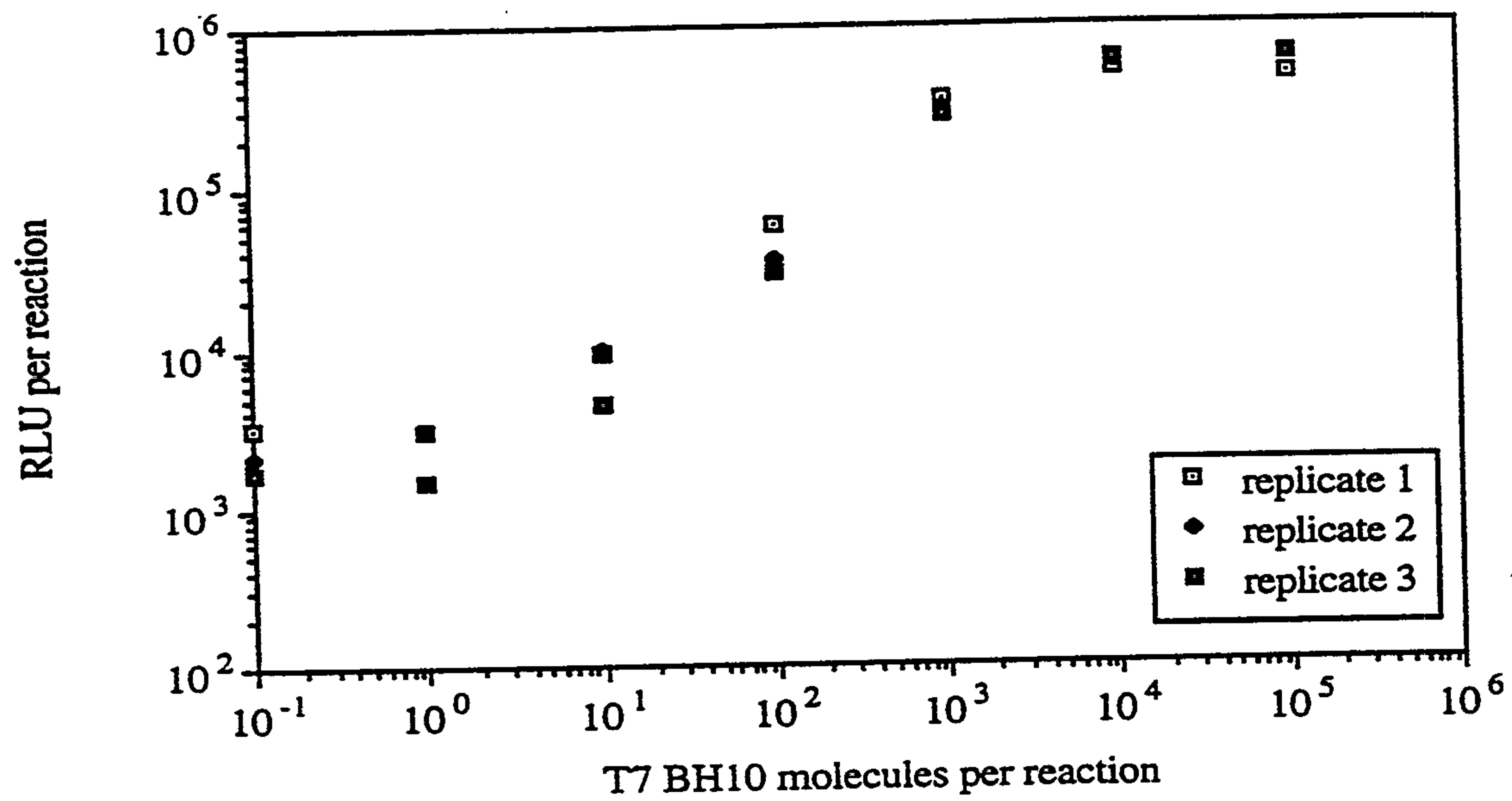
Figure 1c. 20 U T7 RNA polymerase per reaction: T7 BH10 quantitative amplification using multiplex amplification format
