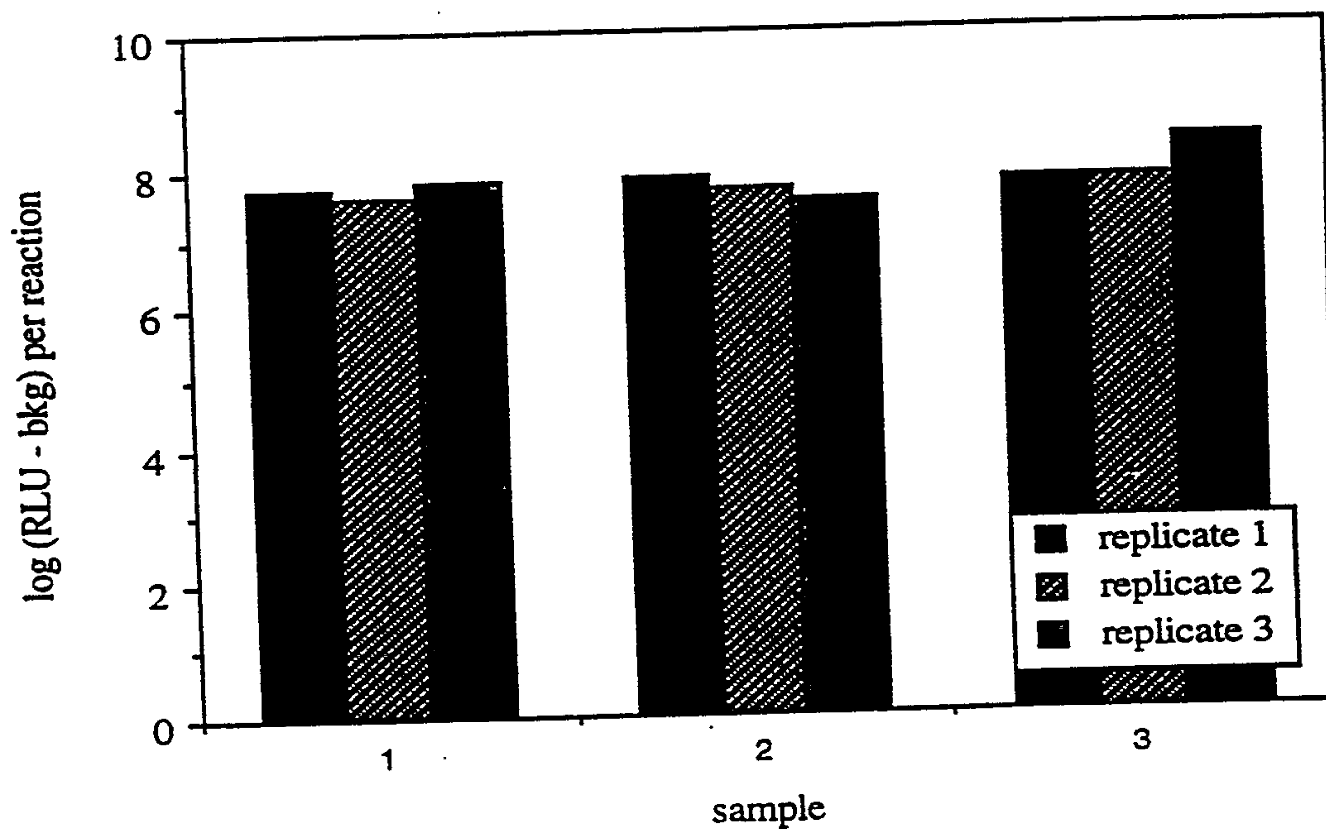
Figure 4b. Quantitative amplification of poly dT-selected HIV-1 lysate.
