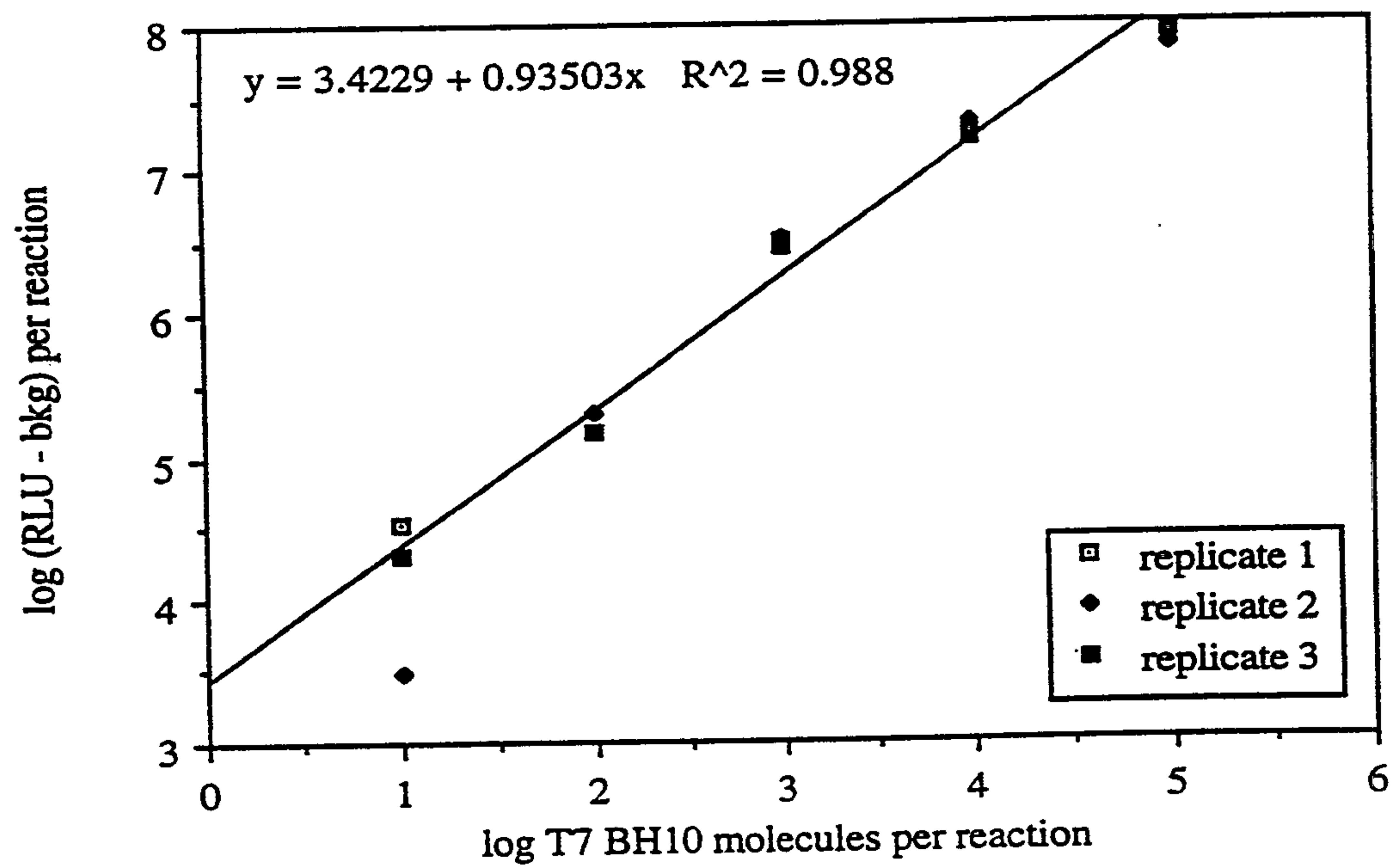
Figure 5a. Amplification of T7 BH10 standard for quantitation of HIV-1 viral lysate.
