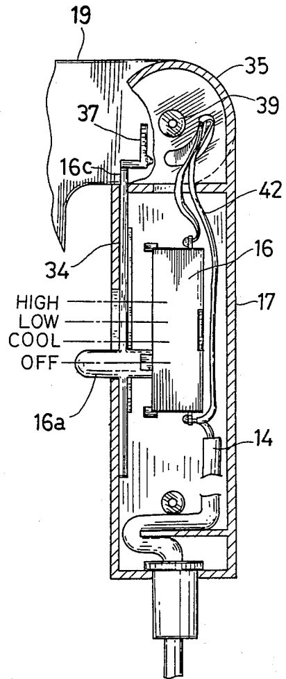
FIG. 6 When the hair dryer head is folded
