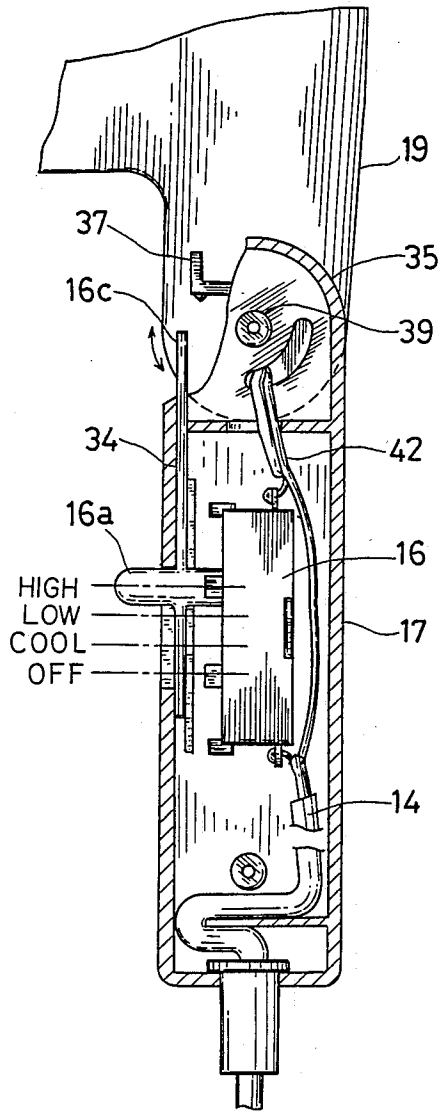
FIG. 5 When the hair dryer is used
