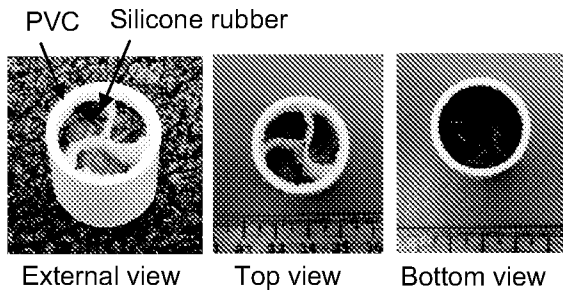
Fig. 2 Photograph of prototype heart valve
