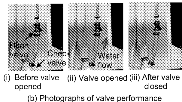
Fig. 3 Schematic of experimental setup and photographs of valve testing results
