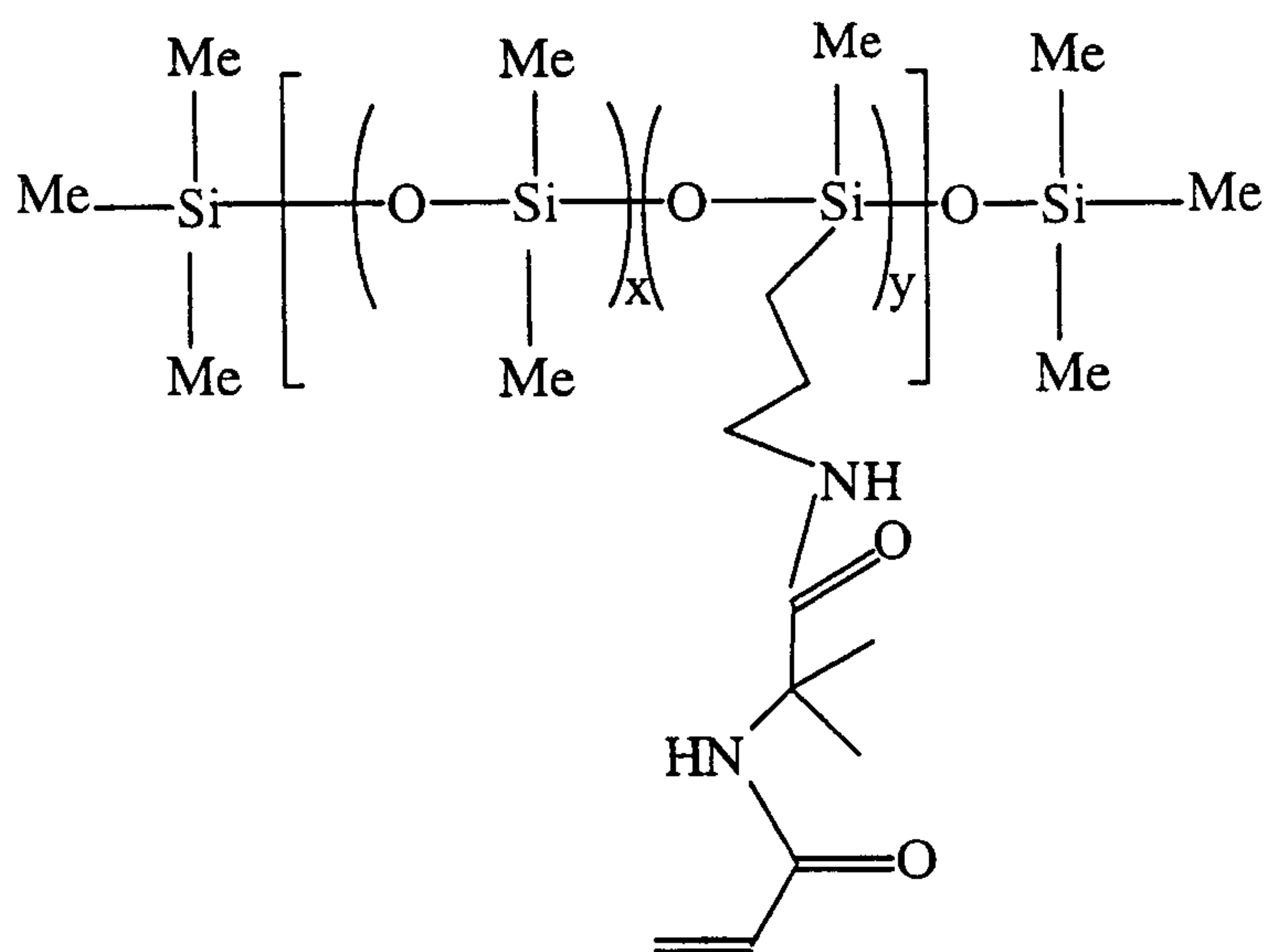
acrylamide-functionalised polydimethyl-aminopropylsiloxane copolymer
