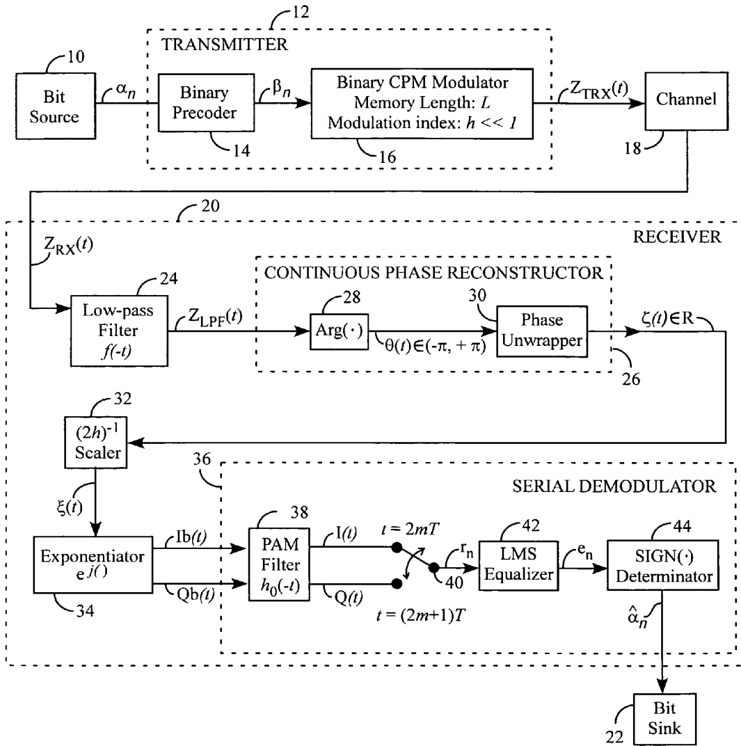
PRE-CODED BINARY CPM DATA DEMODULATOR
