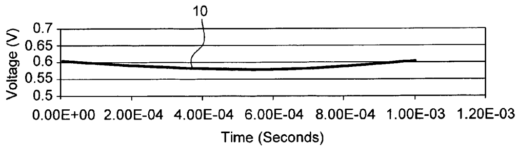
FIG. 2 Terminal Voltage vs. Time Profile
