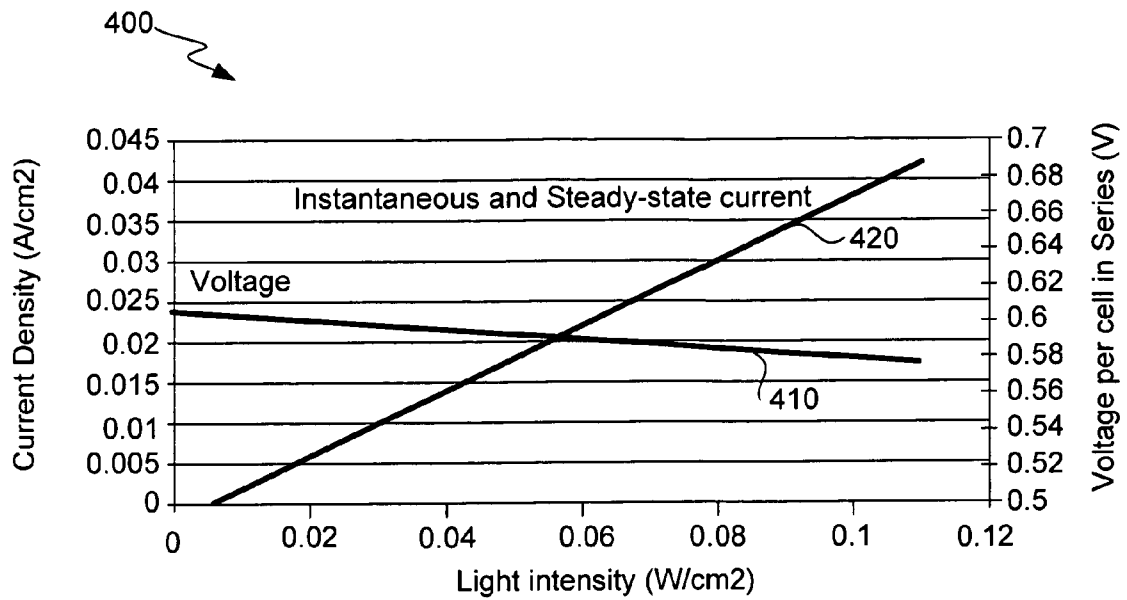
FIG. 5 Current Density vs. Light Intensity
