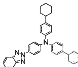
(Compound 8)
