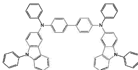
Comparative Compound (2-1)
