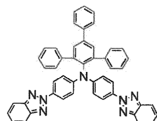
(Compound 45)
