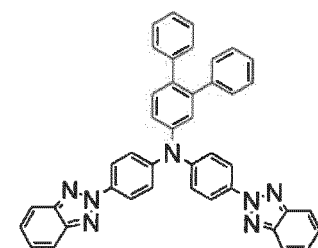
(Compound 42)
