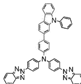
(Compound 54)
