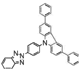
(Compound 23)
