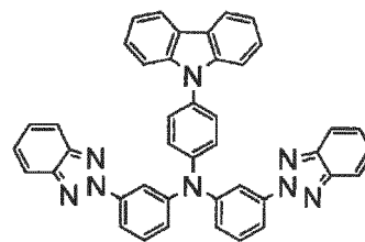
(Compound 81)
