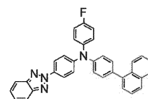
(Compound 9)
