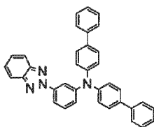
(Compound 68)
