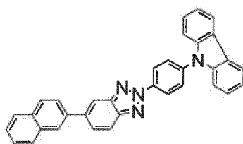
(Compound 22)
