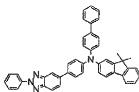
(Compound 31)
