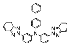
(Compound 75)
