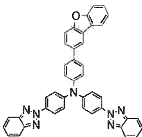
(Compound 52)
