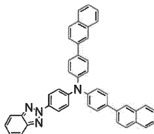
(Compound 14)
