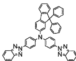
(Compound 48)
