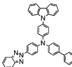
(Compound 15)
