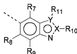
(B - 3)
