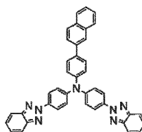
(Compound 43)
