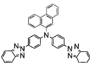
(Compound 40)
