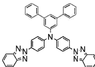
(Compound 41)
