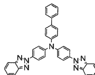
(Compound 39)
