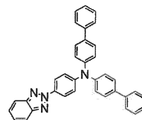
(Compound 6)
