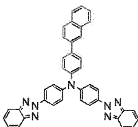
(Compound 43)
