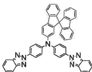
(Compound 49)
