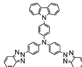
(Compound 51)
