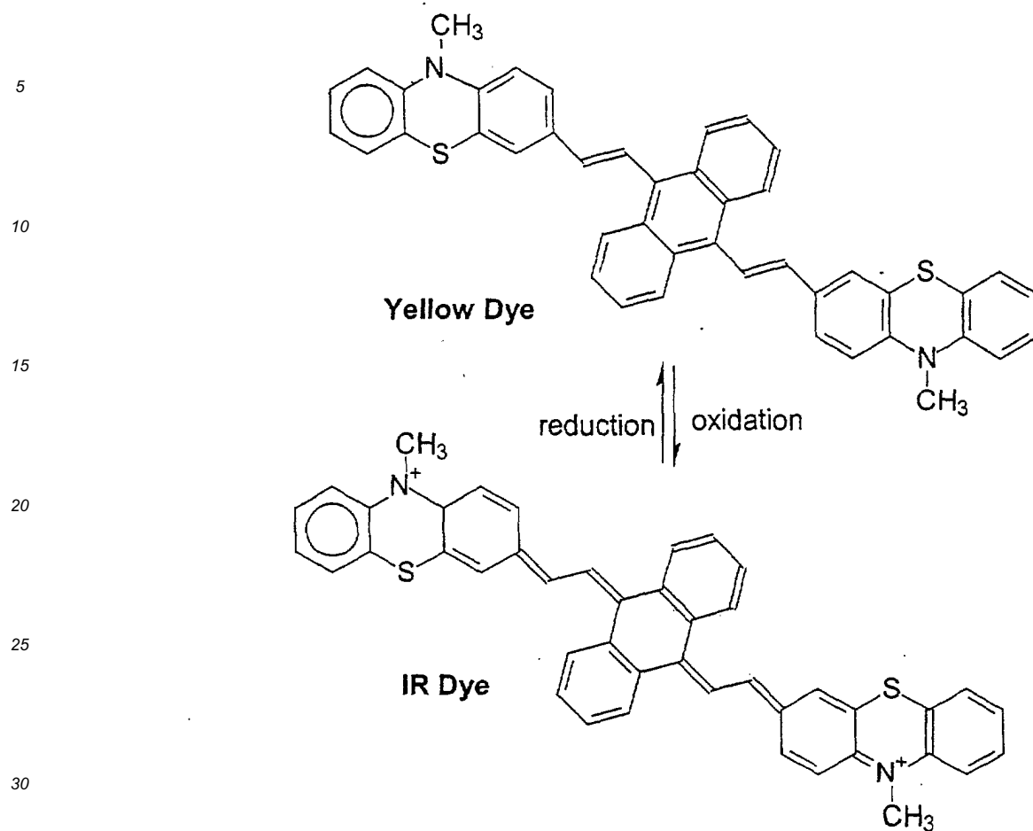
Equation 2
