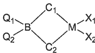
[Chemical Formula 1]
