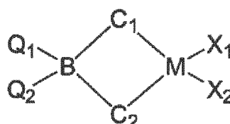
[Chemical Formula 1]
