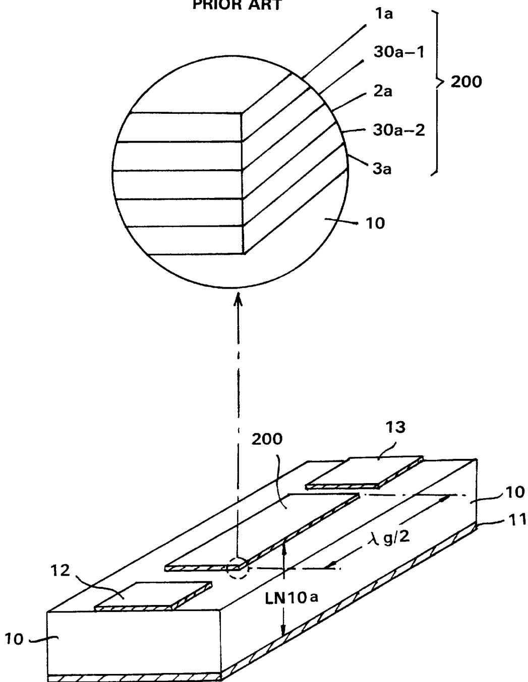
FIG. 4 PRIOR ART
