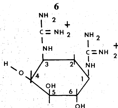
2-deoxystreptidine
