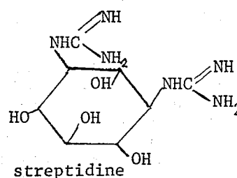
streptidine
