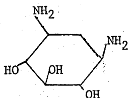
2-deoxystreptamine
