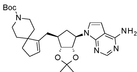
intermediate 530
