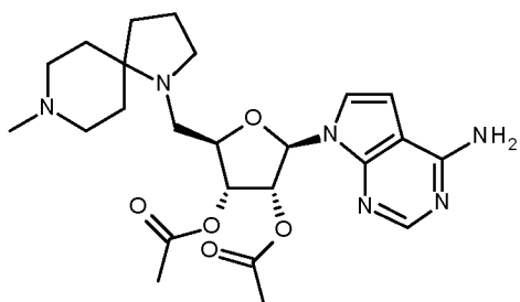
Final compound 98
