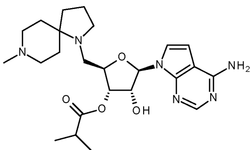
final compound 96
