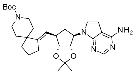
intermediate 531
