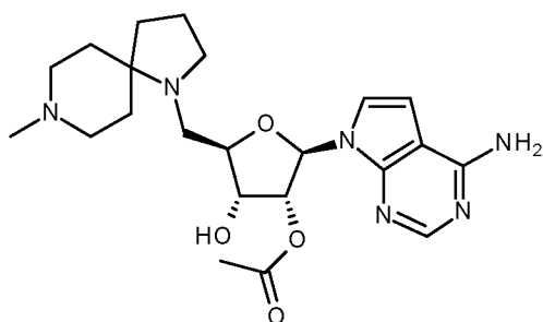
Final compound 100
