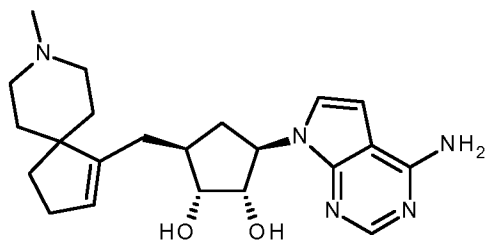
final compound 206
