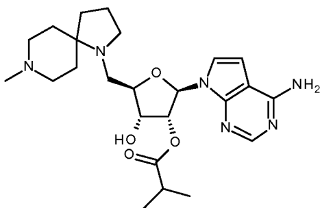
final compound 96
