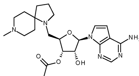
Final compound 99
