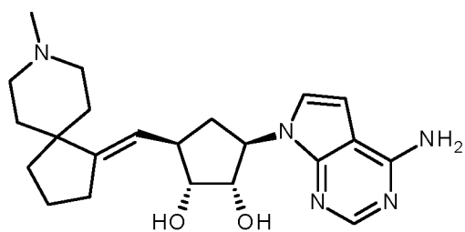
final compound 207
