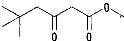
methyl 5,5-dimethyl-3-oxohexanoate, etc.,
