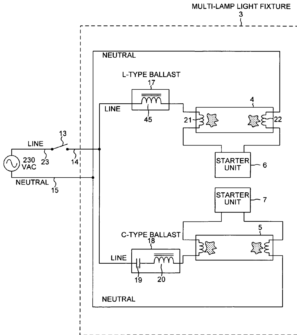
TURN-OFF OF MULTIPLE FLUORESCENT LAMPS
