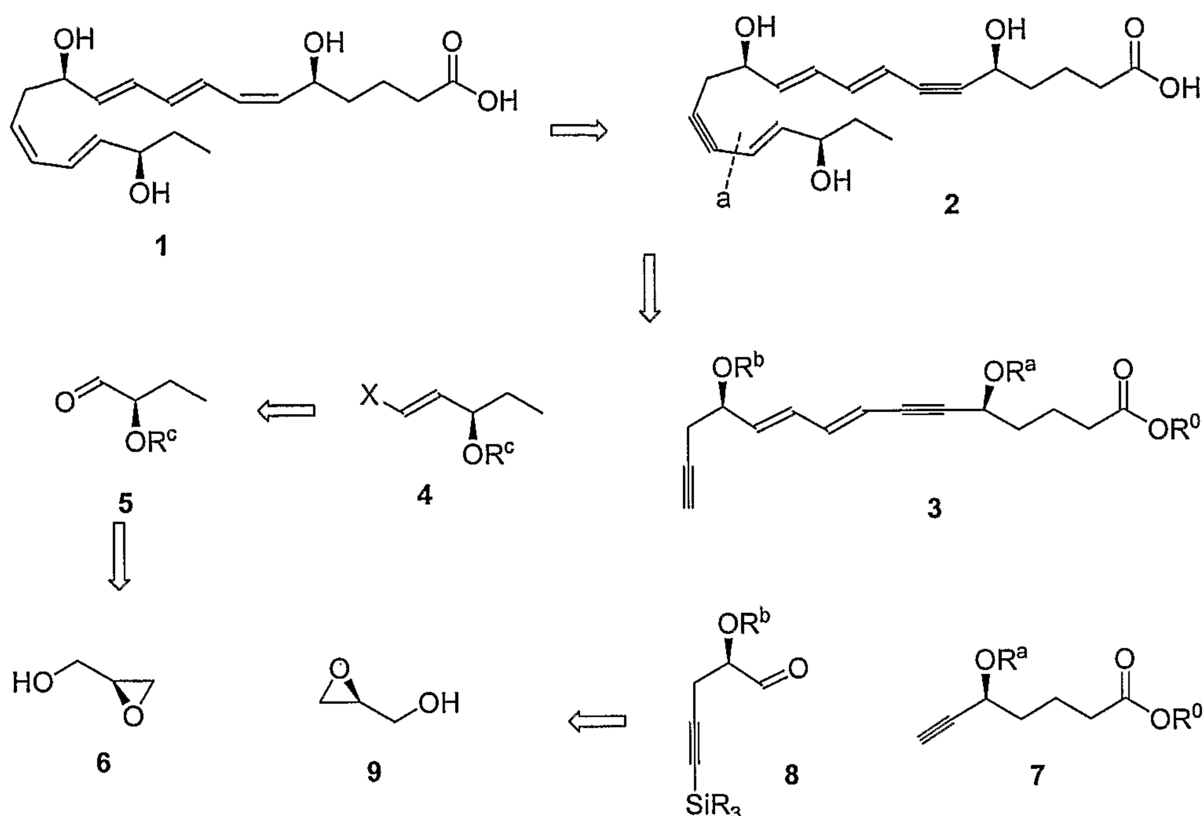
Scheme 1
