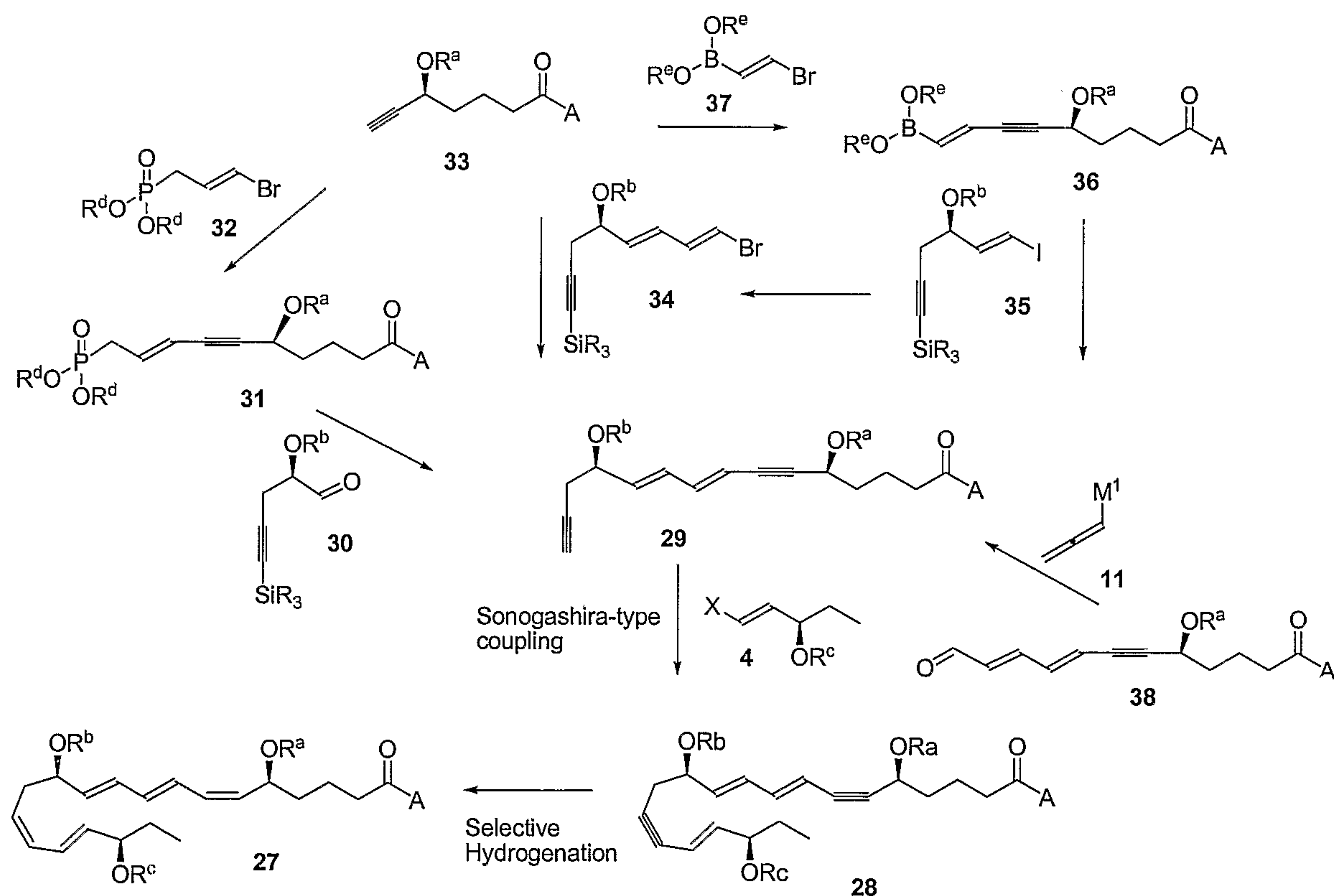
Scheme 12
