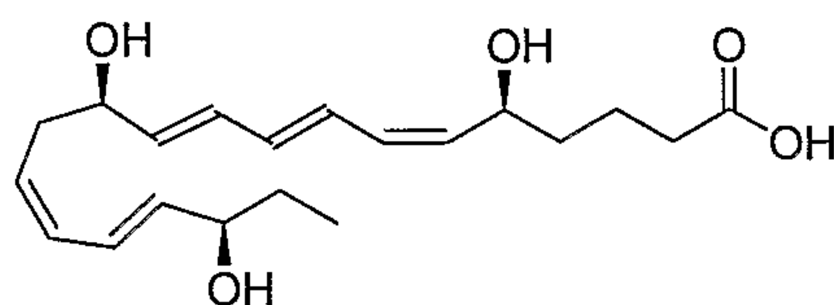
5S, 12R, 18R-triHEPE or Resolvin E1 ( 1 )
