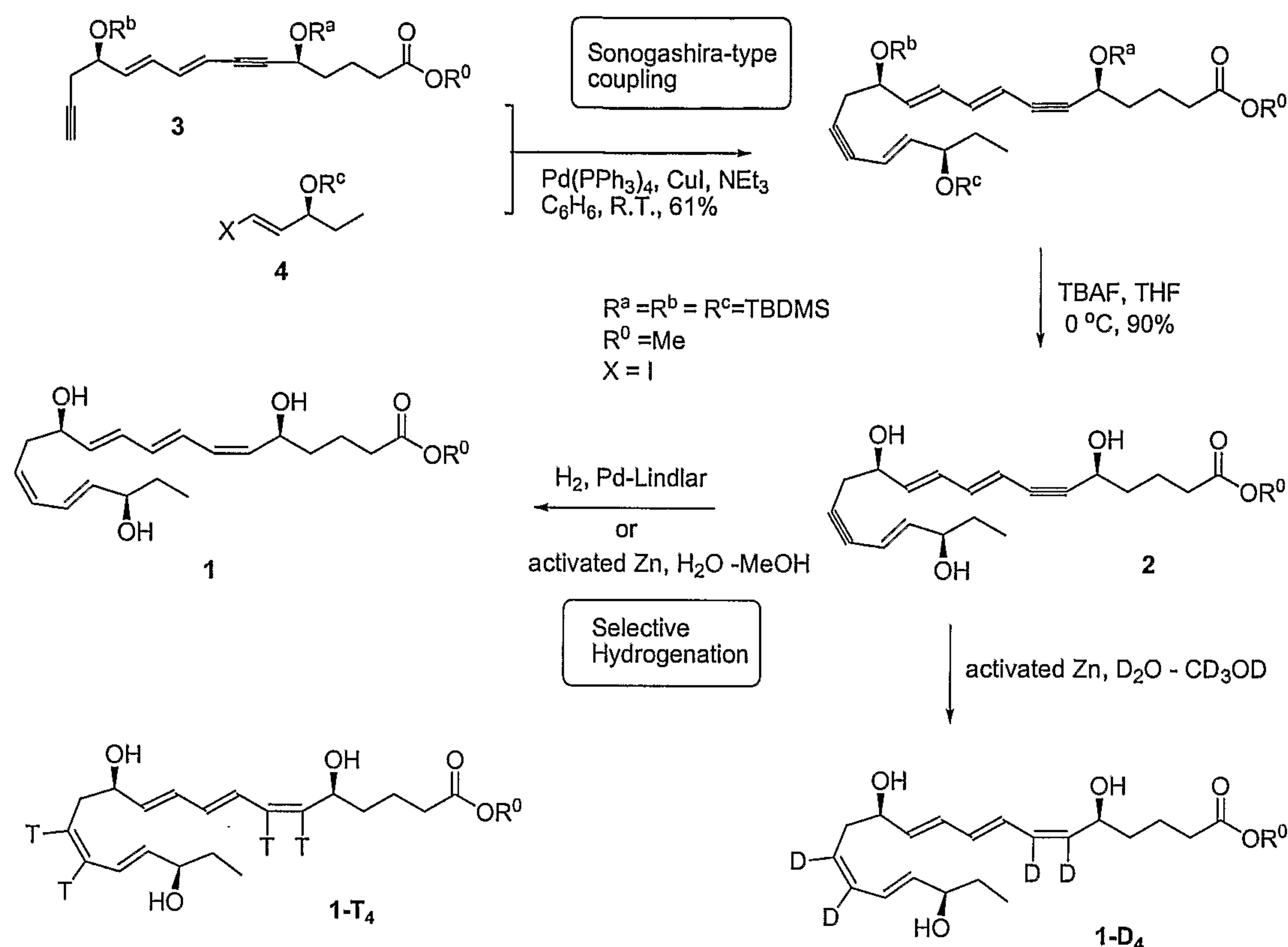
Scheme 11
