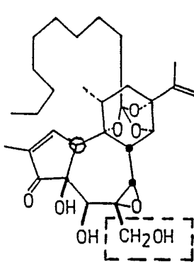
Simplexin
