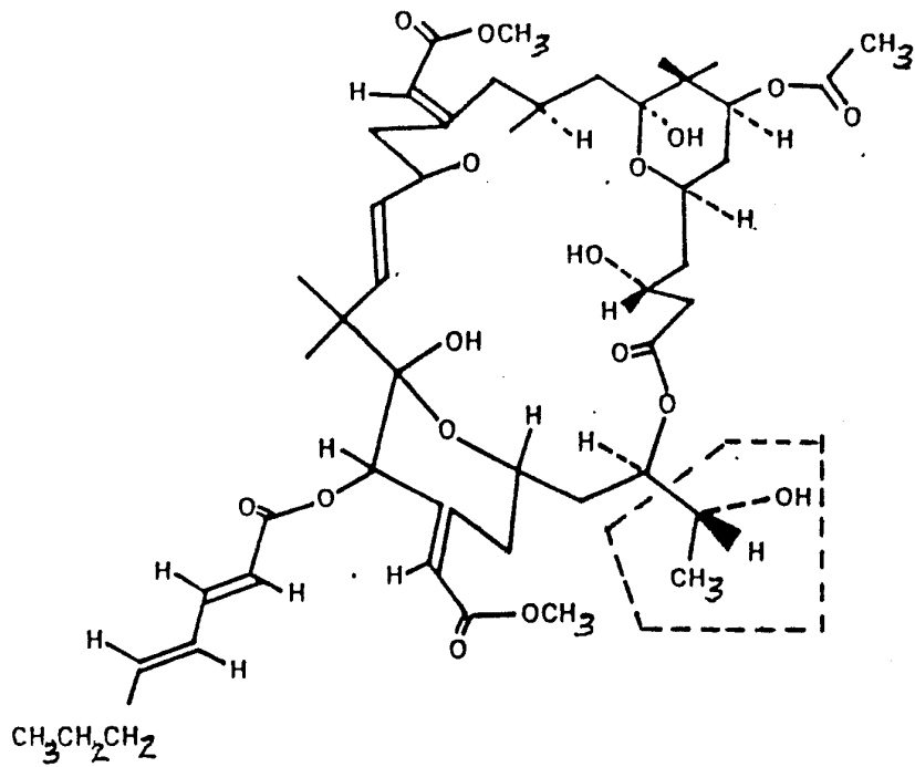
Bryostatin 1
