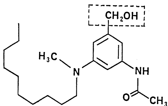
3-Acetylamino-5-(N-decyl-N-methylamino)benzyl Alcohol
