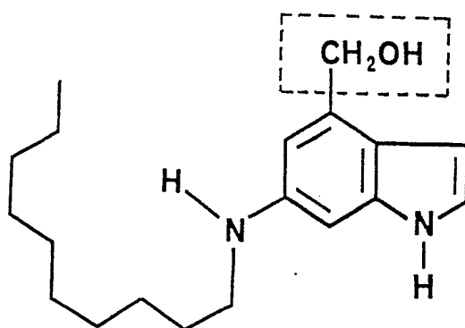
6-(N-decylamino)-4-hydroxymethylindole
