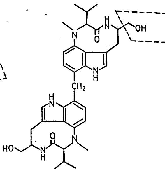
Blastmycetin A
