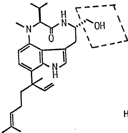
Lyngbyatoxin A
