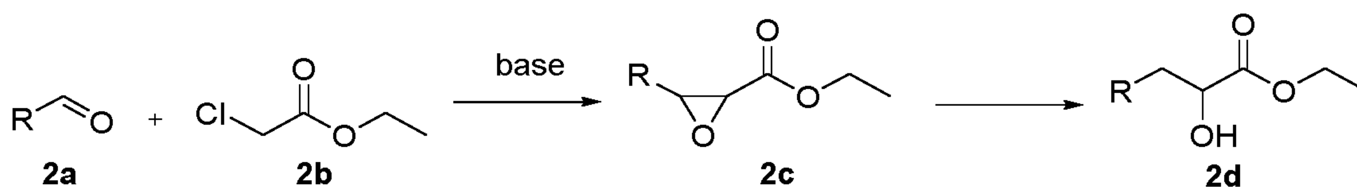
Scheme 3
