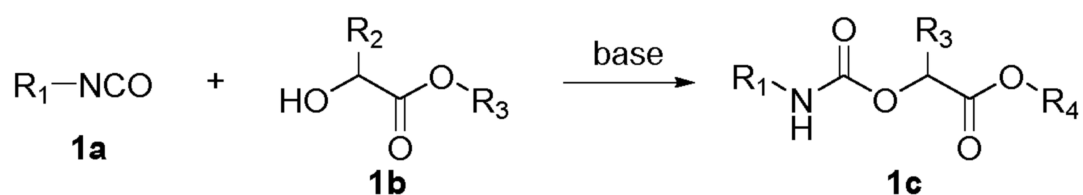
Scheme 1
