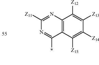
Formula 5-21
