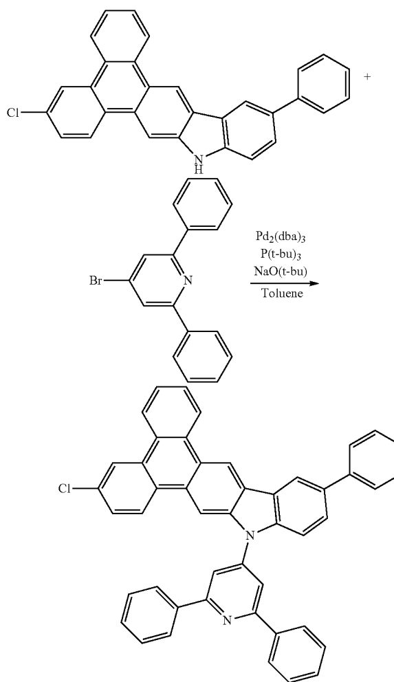
Compound 1
