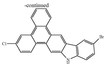
Intermediate 1-2
