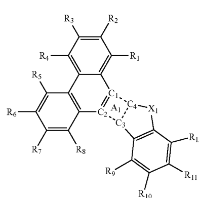
&lt;Formula 1A&gt;
