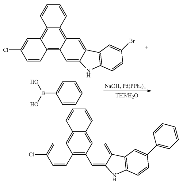
Intermediate 1-3
