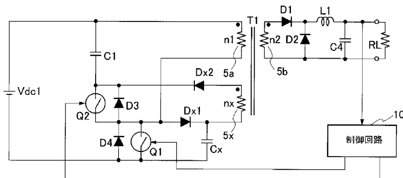
10... CONTROL CIRCUIT
