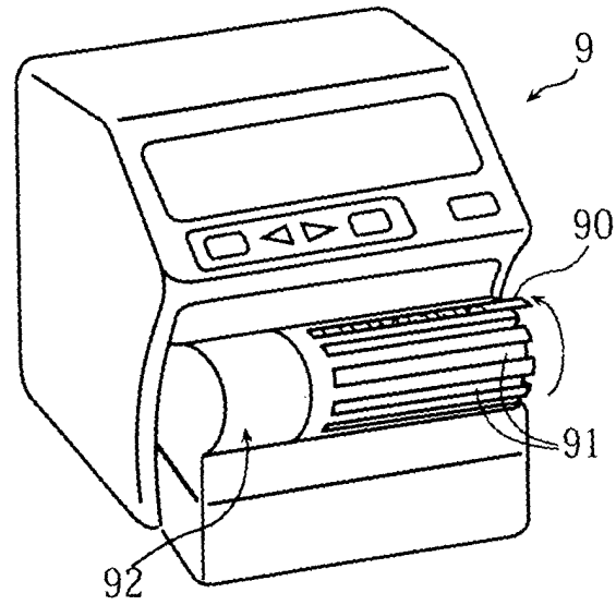
FIG.8 PRIOR ART
