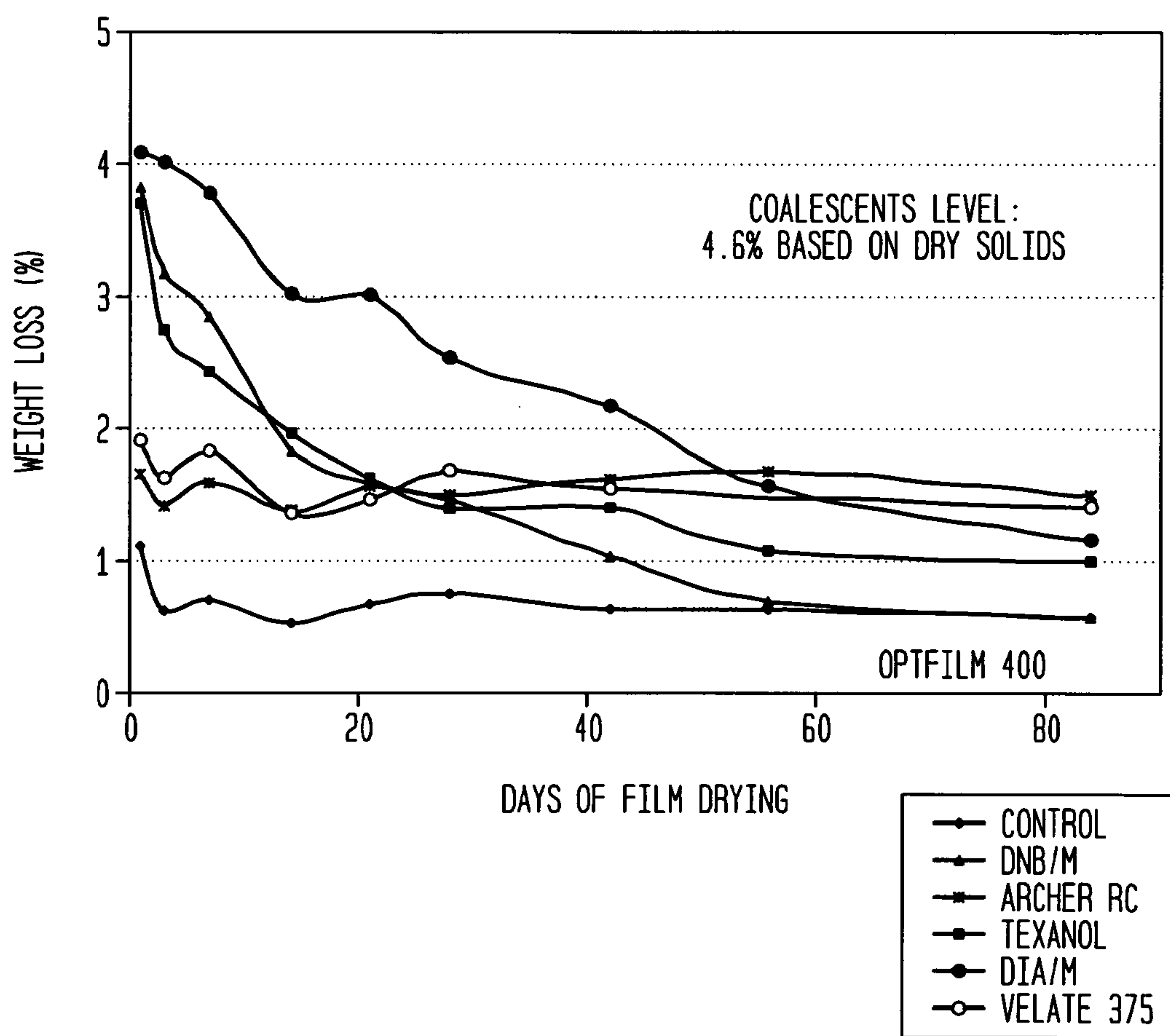
FIG. 10 RESIDUAL COALESCENT IN PAINT FILM - TGA ANALYSIS
