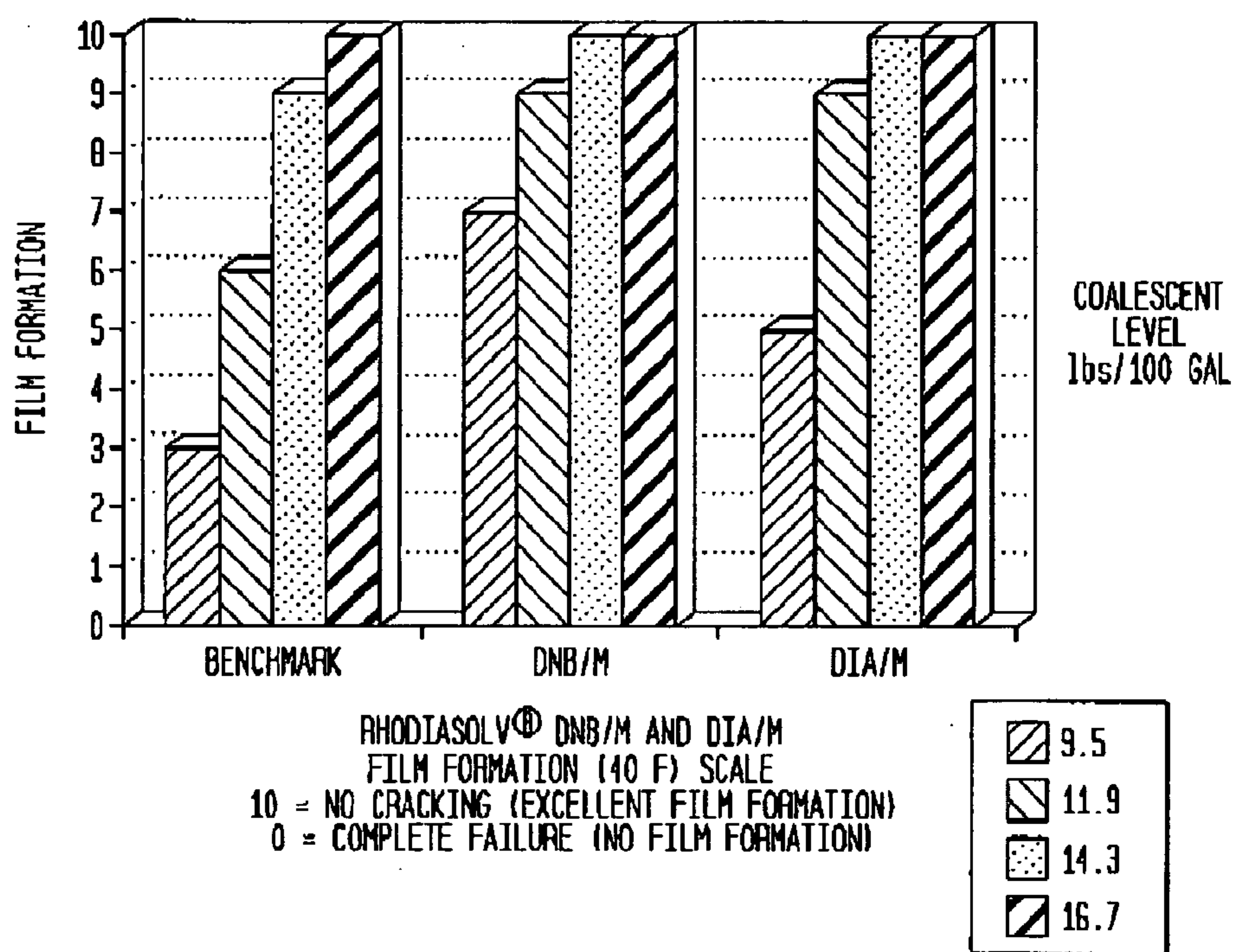
FIG. 8 LOW TEMPERATURE FILM FORMATION - SEMI-GLOSS PAINT
