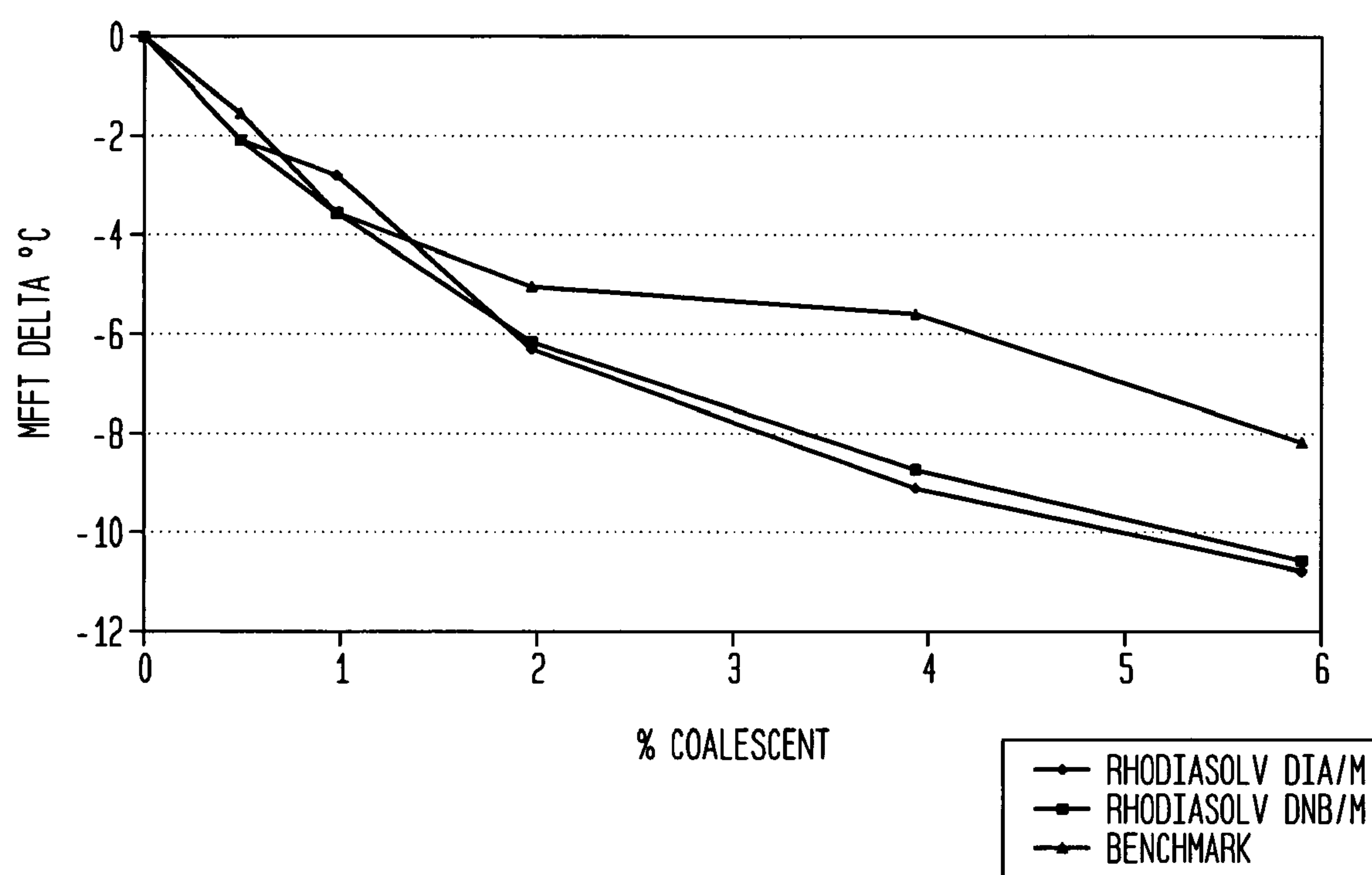
FIG. 7 MFFT RESULTS FOR VINYL-ACRYLIC RESIN
